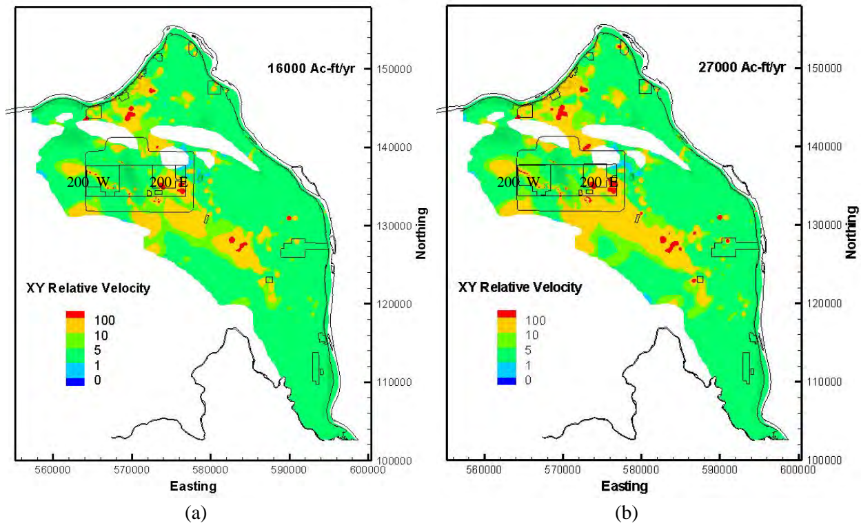
Figure 3.5. X-Y Flow Velocities Relative to the Base Case for a) 16,000 acre-ft/yr and b) 27,000 acre-ft/yr
