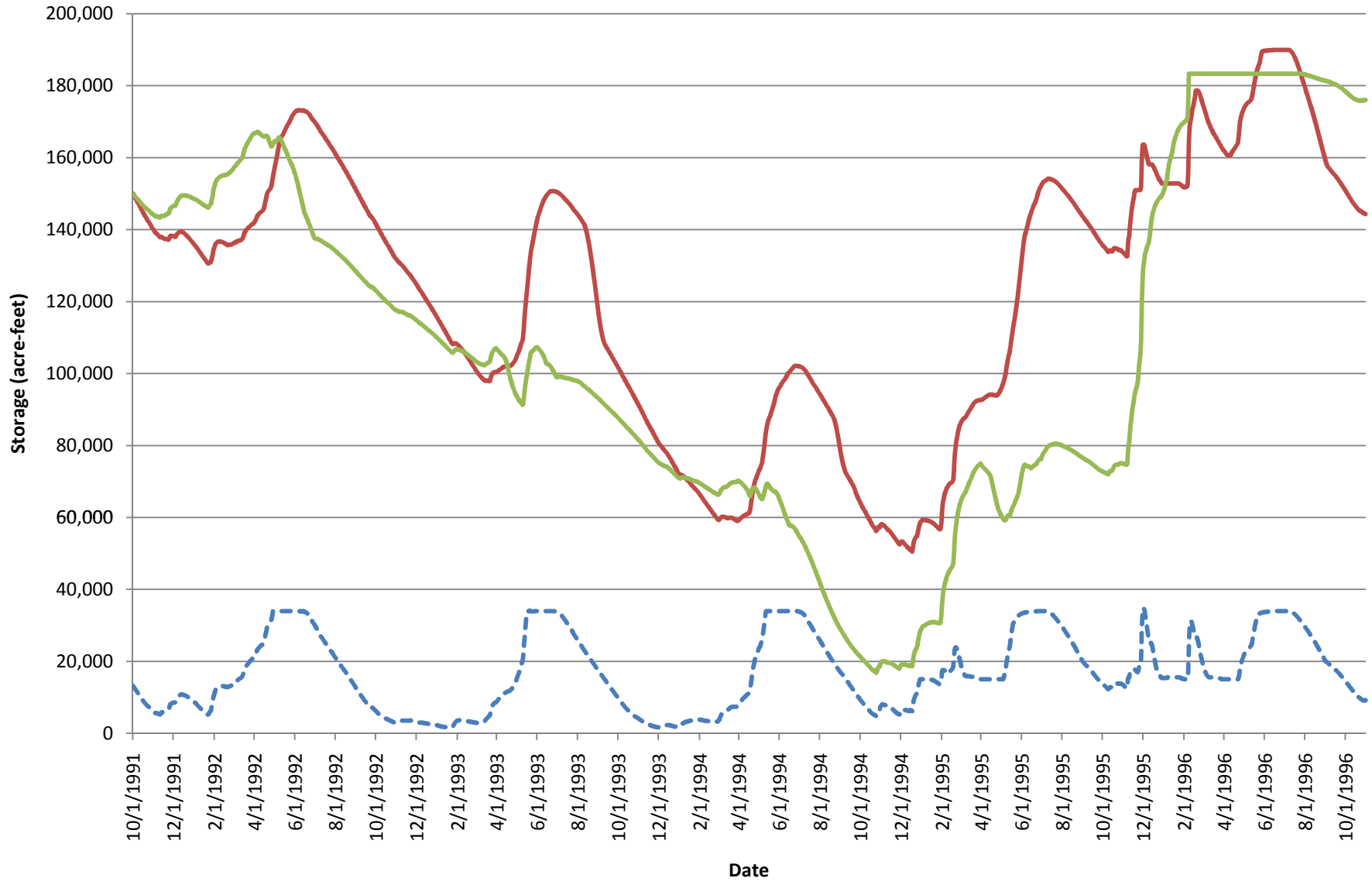
Bumping Reservoir Storage (Water Years 1992-1996)
