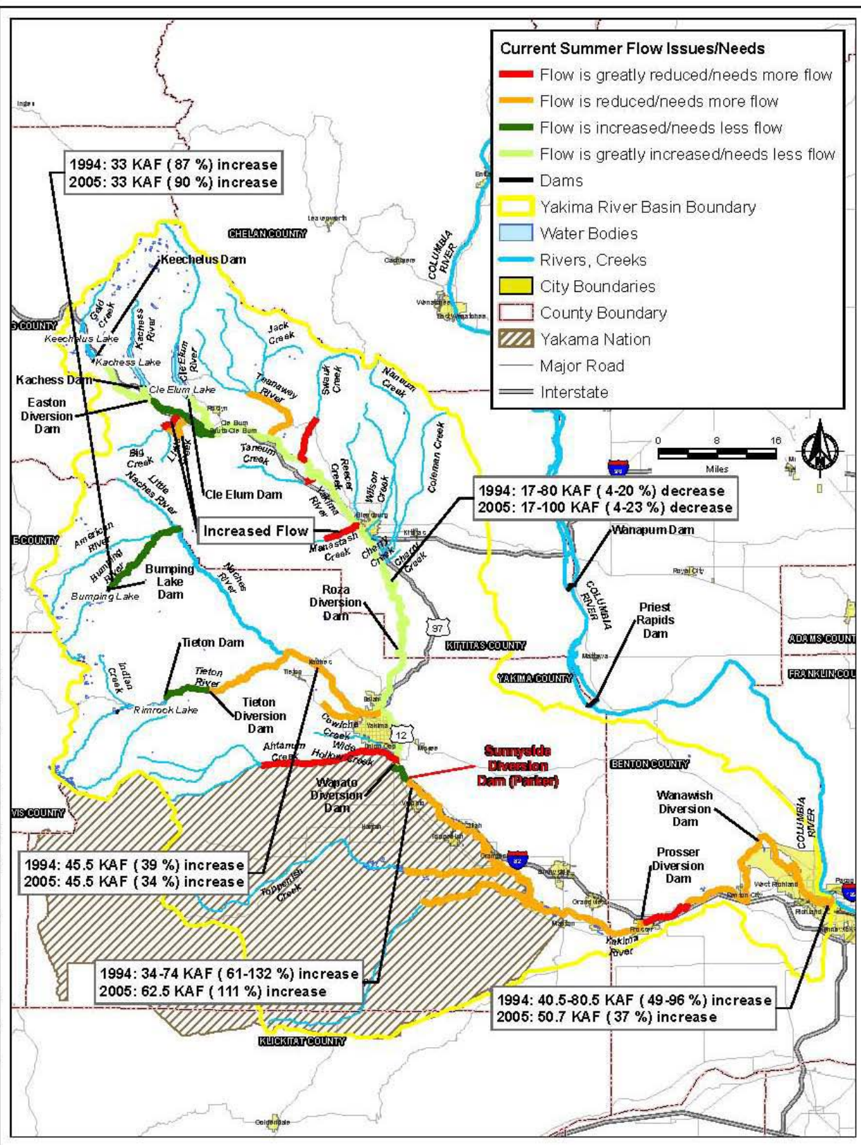
Summer Existing Flow Conditions and Phase I and II Improvements
