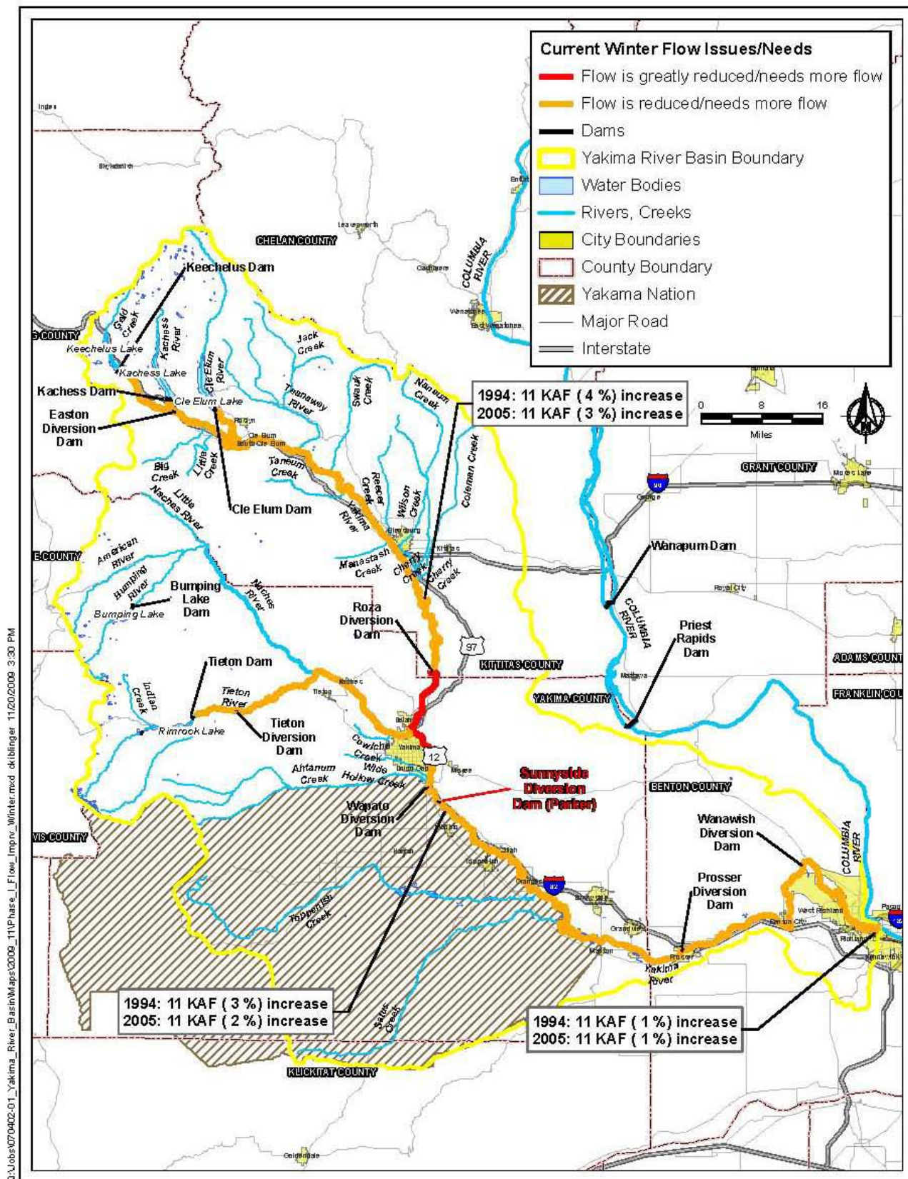
Winter Existing Flow Conditions and Phase I Improvements
