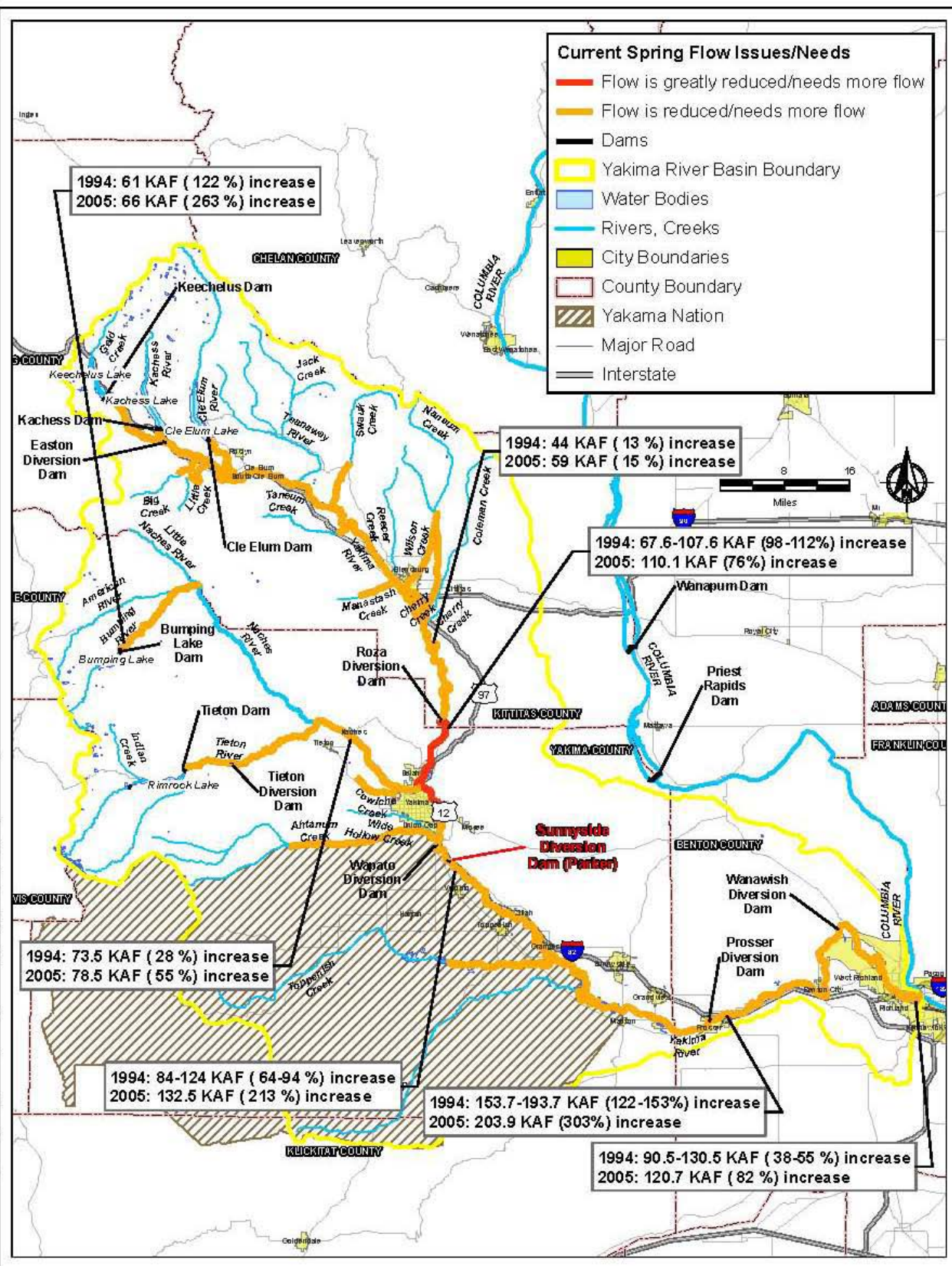
Spring Existing Flow Conditions and Phase I and II Improvements
