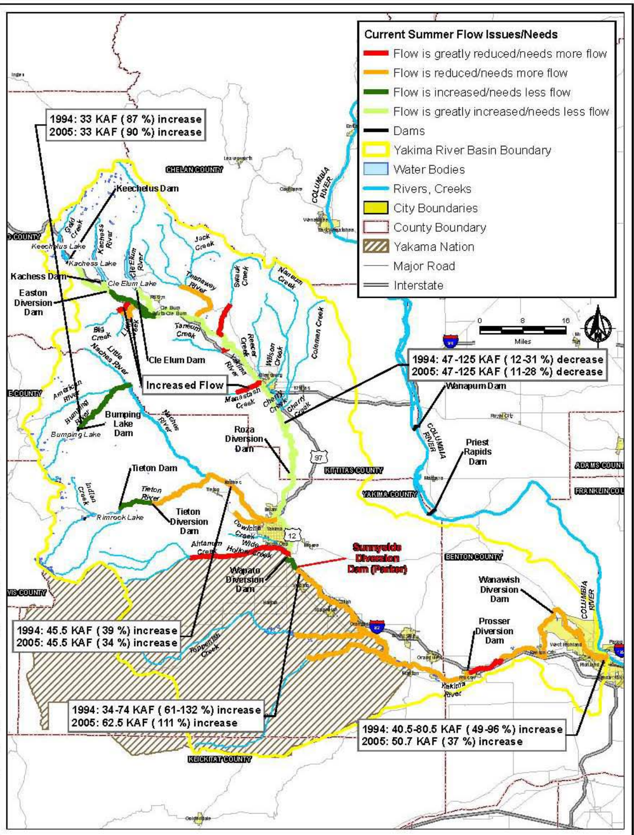
Summer Existing Flow Conditions and Phase I Improvements
