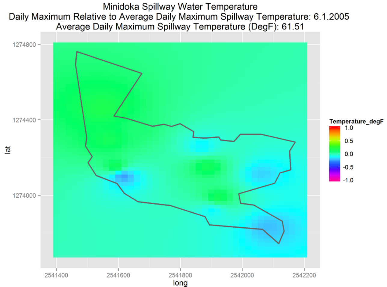
Figure 3-15. June 1, 2005 spatial variation of maximum spillway temperatures.
