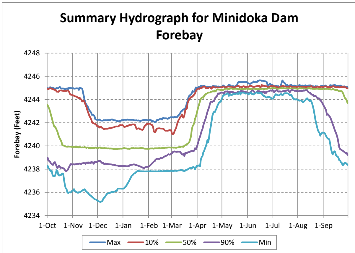
Figure 3-3. Summary hydrograph for Lake Walcott operations.
