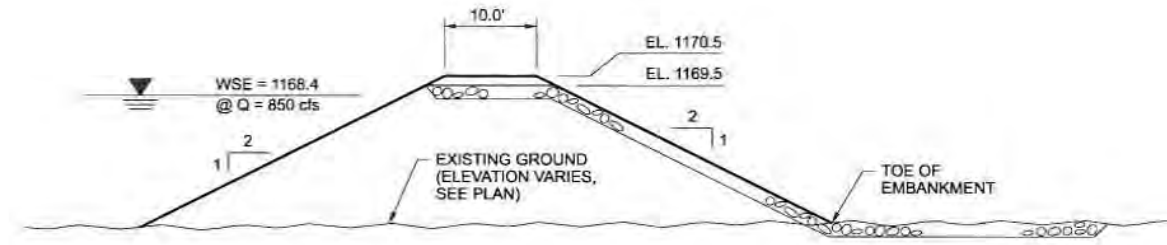
TYPICAL SECTION 1/2"=1'-0"
