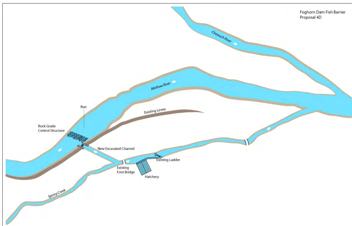
Figure 7. Illustration of proposal 4D to install a structure to augment flow in Spring Creek.
