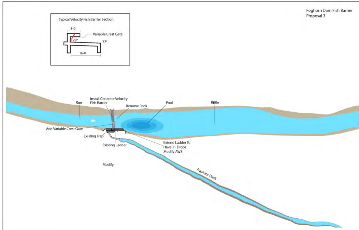
Figure 3. Illustration of a velocity barrier installation at Foghorn Dam, Winthrop, WA.
