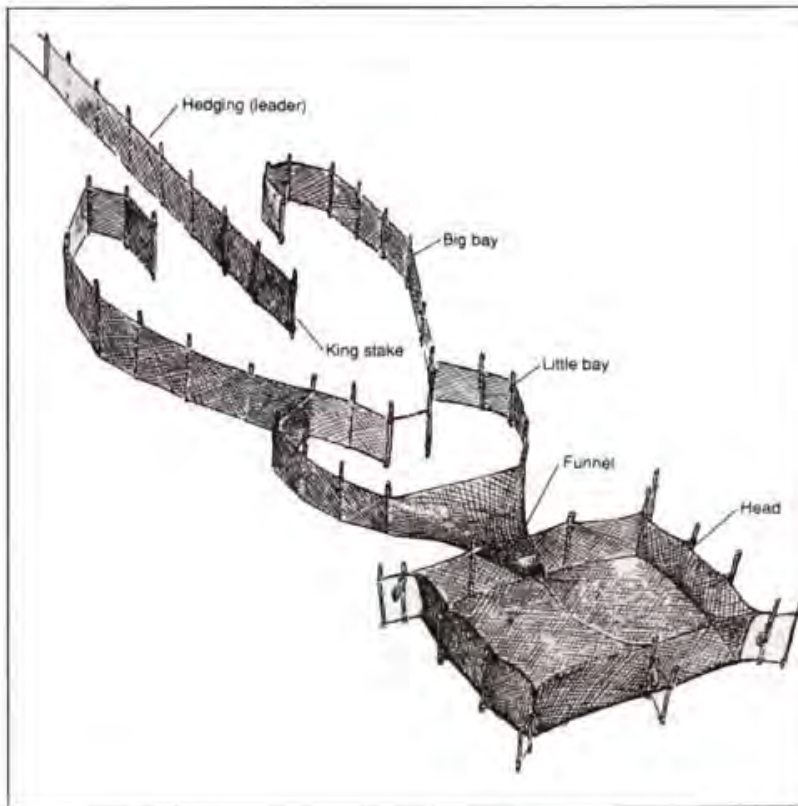
Figure 2. Schematic of typical pound net fish trap.
