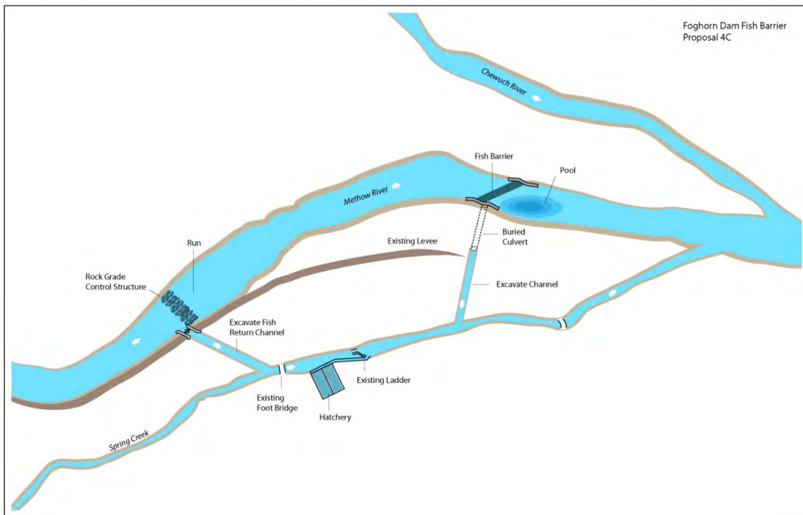
Figure 6. Illustration of Proposal 4 locating a new fixed picket style barrier downstream from Foghorn Dam.
