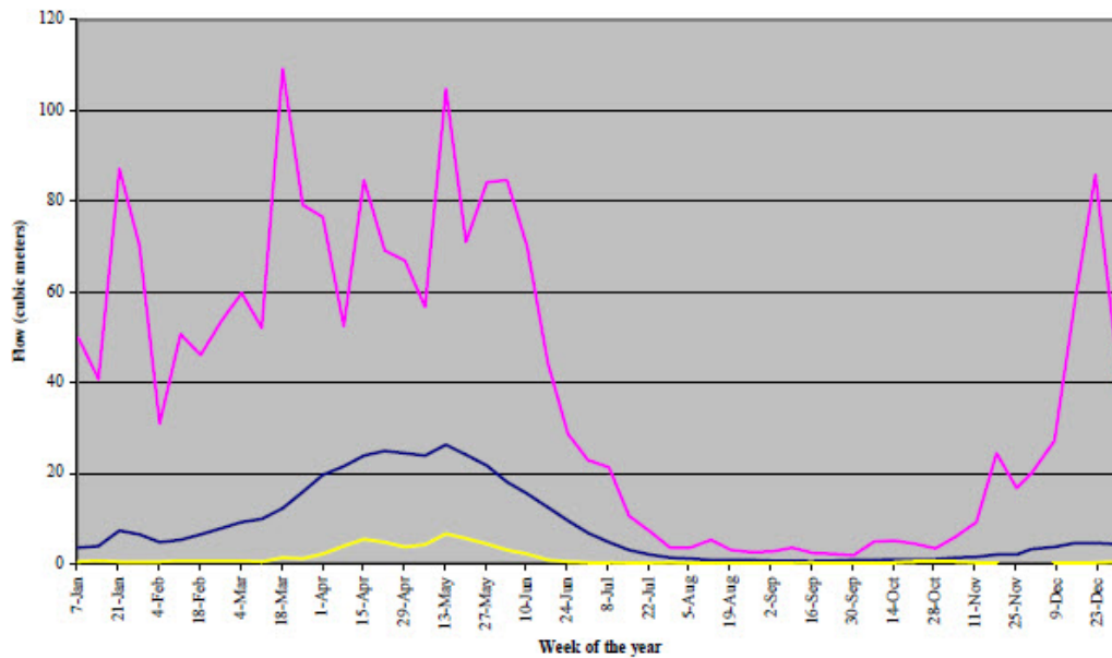
Figure 6. Hydrograph of mean daily flows in the Upper Grande Ronde River near Hilgard 1937-1955 and 1966-1981. The bottom line (yellow) represents minimum; the middle line (blue) mean; and the upper line (purple), maximum flows (NPCC 2004).
