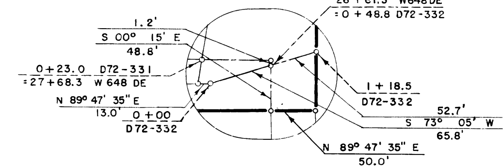
DETAIL "B"
