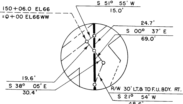
DETAIL "B"
