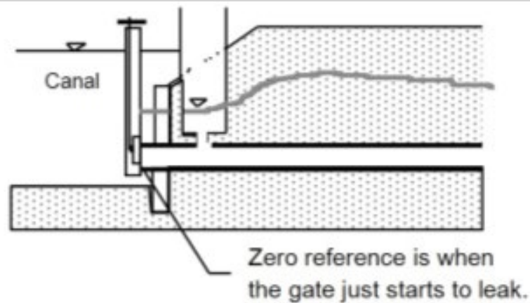
Figure 4. Stilling well used for open channel flow
