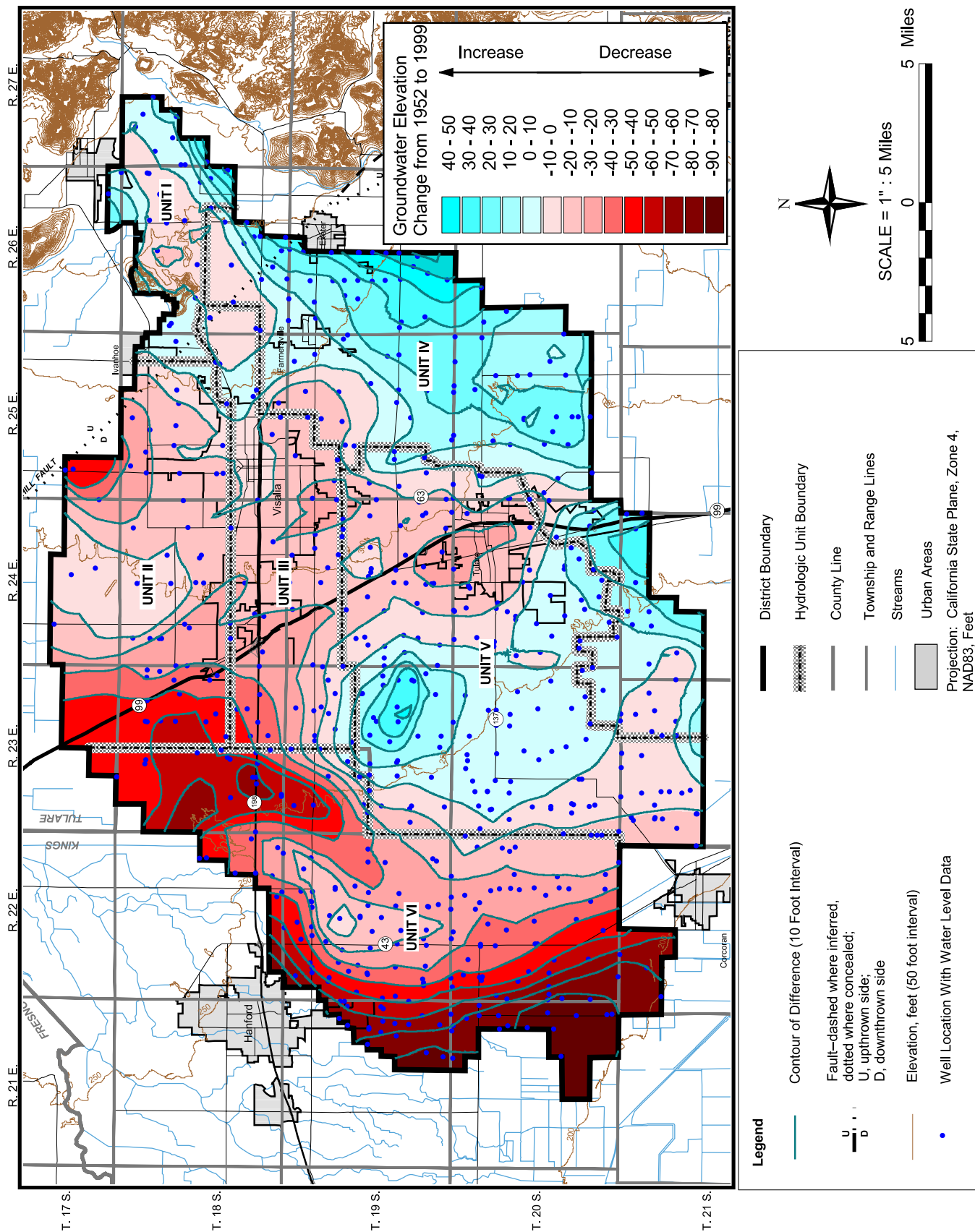
Plate No. 13 Contours of Equal Difference in Water Levels, 1952 to 1999 Kaweah Delta Water Conservation District
