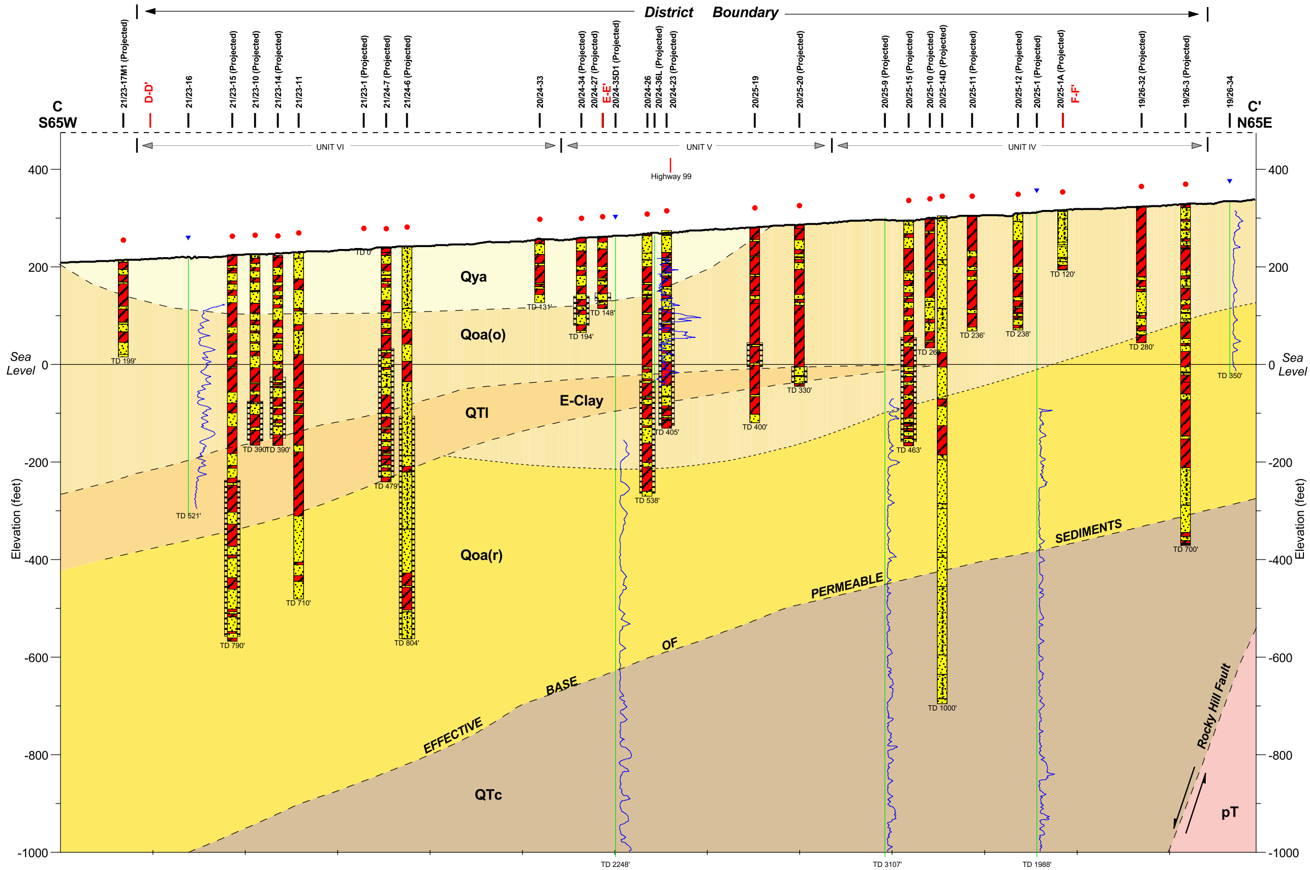
Plate No. 8: Hydrogeologic Section C-C' Kaweah Delta Water Conservation District Kings and Tulare Counties
