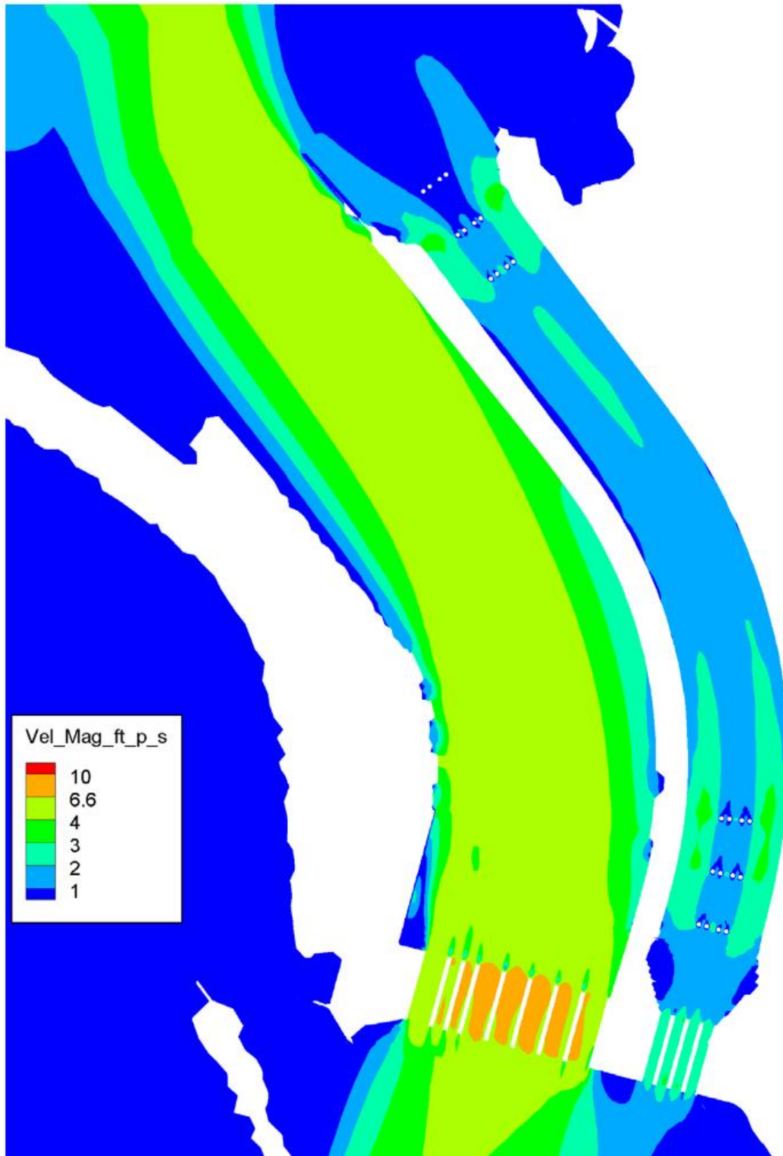
Figure 6. Hydraulic Modeling Scenario J
