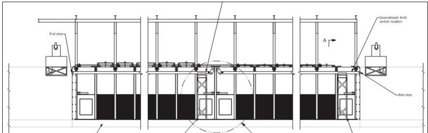
Figure 7. Fish Screen Section View
