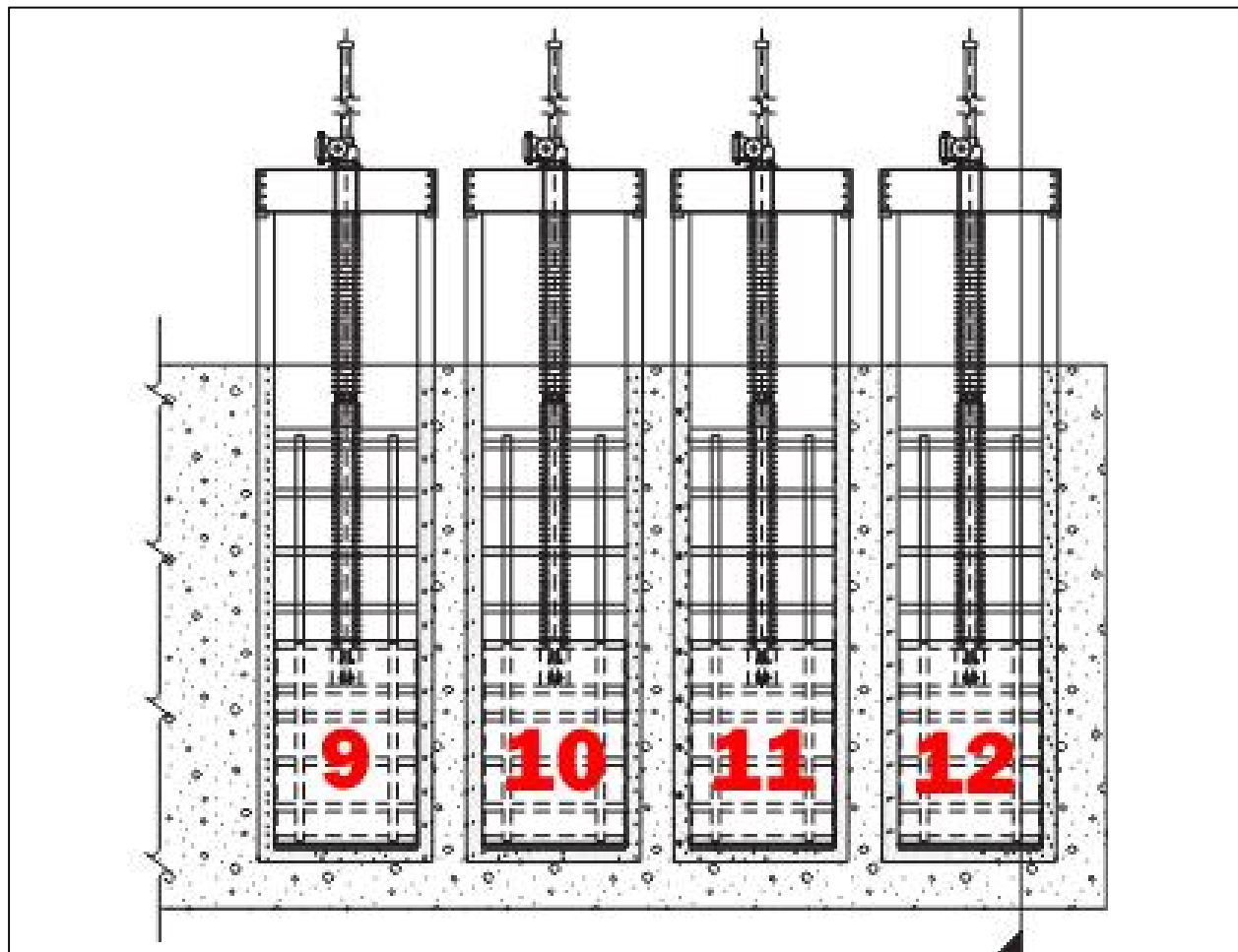
Figure 3. Fish Ramp Headworks Downstream Section View
