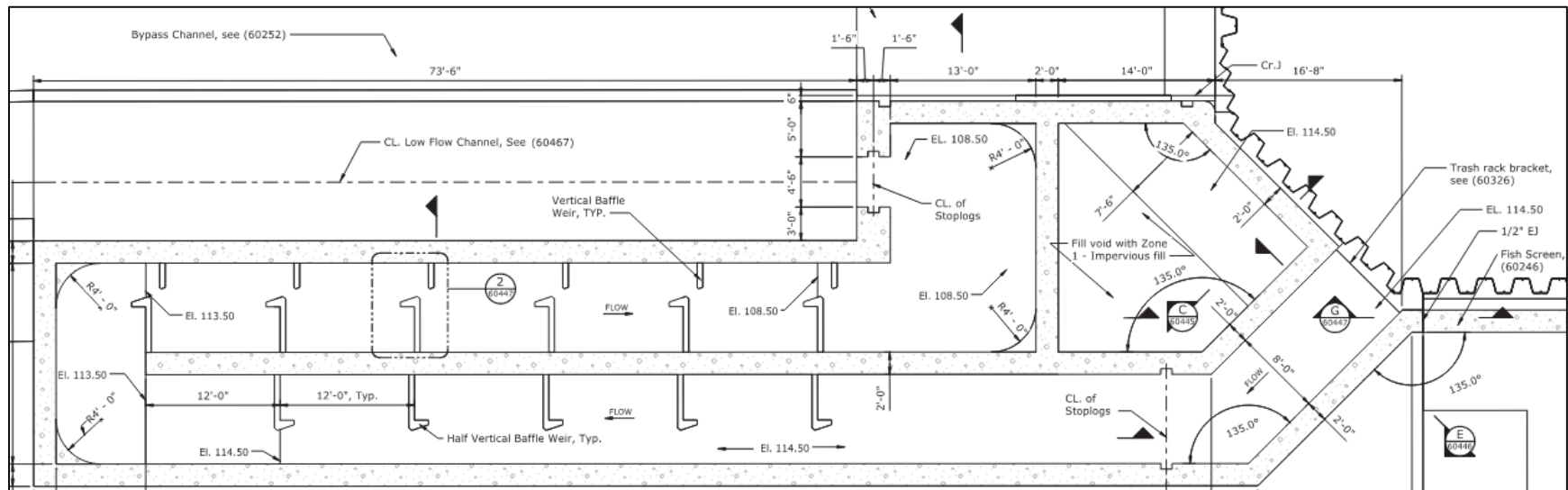
Figure 1. Fish Ladder Plan View
