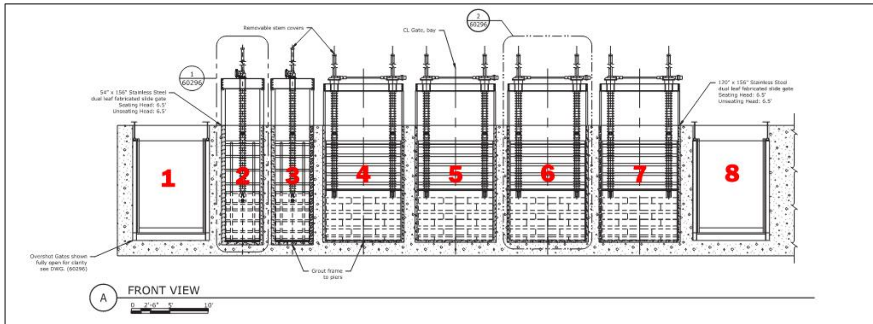
Figure 5. River Bypass Headworks Plan View
