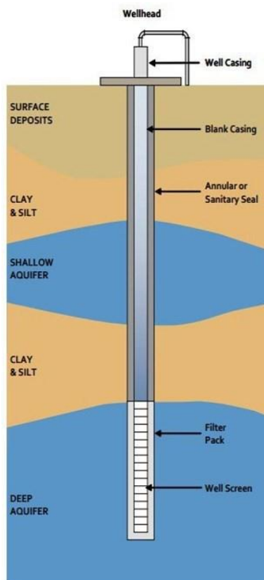
Figure 5. Typical well construction. (CDWR, 2024a)
