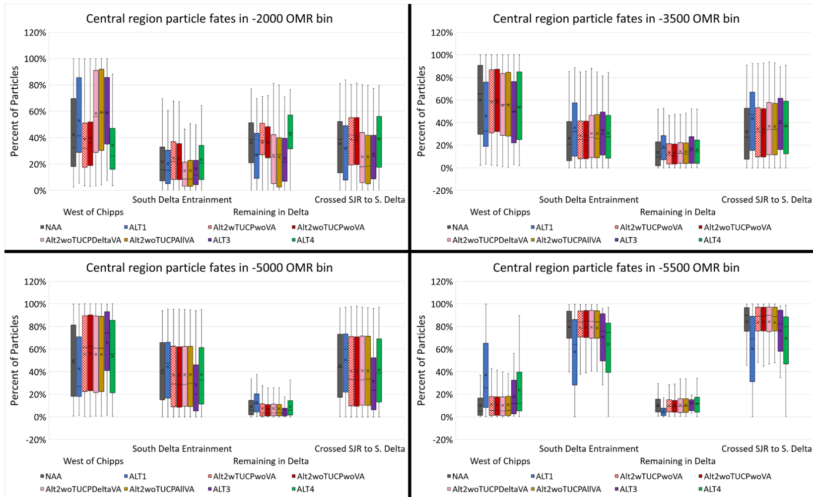
Figure I.8-83. Box and whisker plot of mean December through March particle fate after 45 days by exit location (within each facet from left to right: West of Chipps, South Delta Entrainment, Remaining in Delta, Crossed SJR to S. Delta) for neutrally buoyant particles injected at Central Delta region by OMR Bin (from top left to bottom right: -2,000 cfs, -3,500 cfs, -5,000 cfs, -5,500 cfs) for the No Action Alternative, Alternative 1, four phases of Alternative 2, Alternative 3, and Alternative 4.
