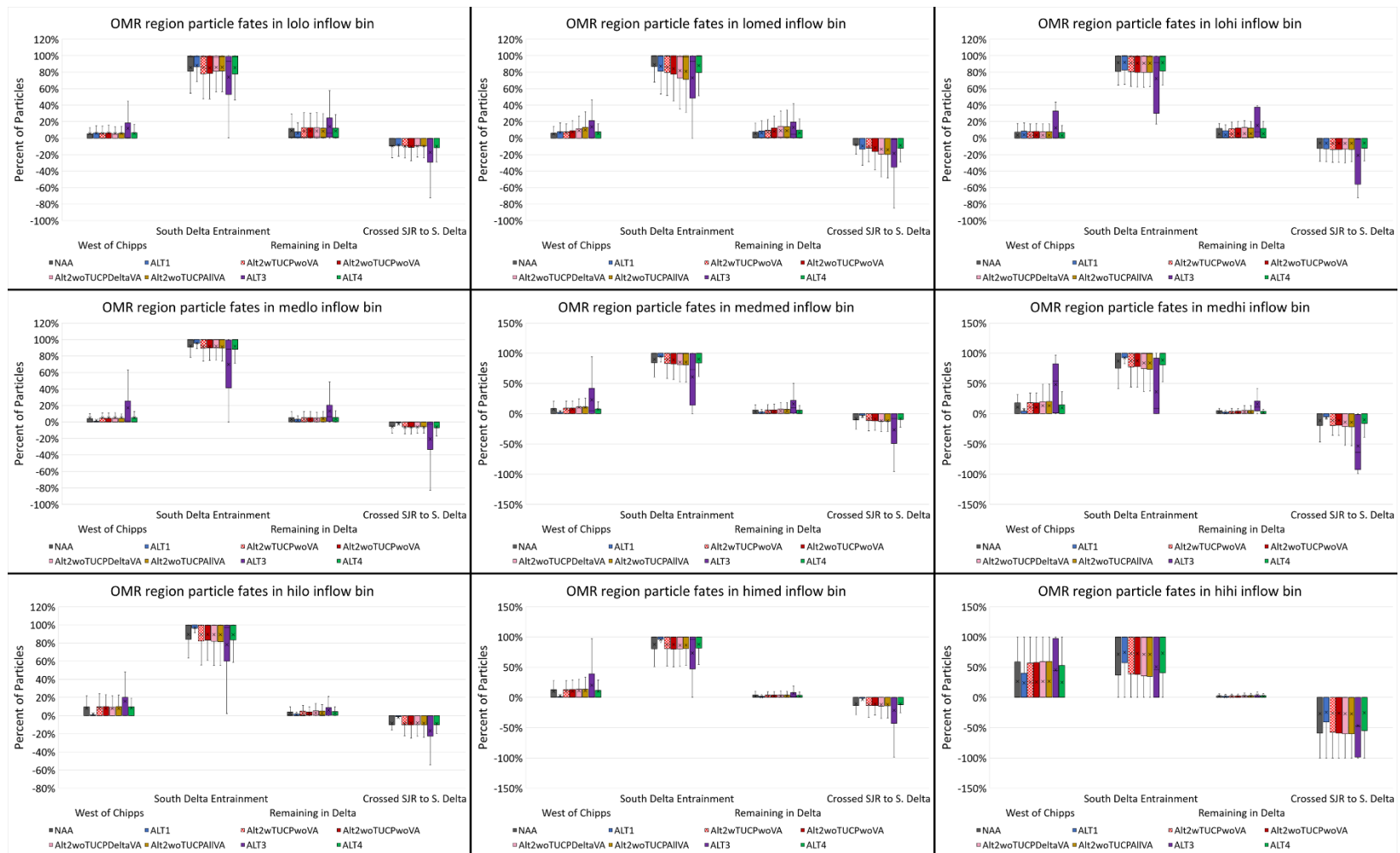
Figure I.8-76. Box and whisker plot of mean December through March particle fate after 45 days by exit location (within each facet from left to right: West of Chipps, South Delta Entrainment, Remaining in Delta, Crossed SJR to S. Delta) for neutrally buoyant particles injected at Old and Middle River region by Inflow Bin (from top left to bottom right: "lolo" to "hihi") for the No Action Alternative, Alternative 1, four phases of Alternative 2, Alternative 3, and Alternative 4.
