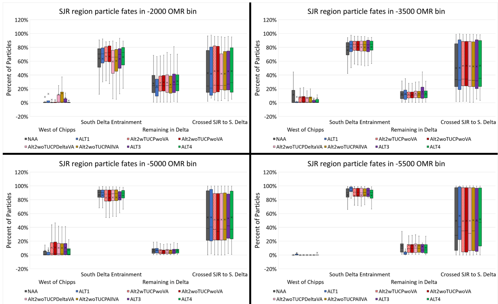
Figure I.8-87. Box and whisker plot of mean December through March particle fate after 45 days by exit location (within each facet from left to right: West of Chipps, South Delta Entrainment, Remaining in Delta, Crossed SJR to S. Delta) for neutrally buoyant particles injected at San Joaquin River region by OMR Bin (from top left to bottom right: -2,000 cfs, -3,500 cfs, -5,000 cfs, -5,500 cfs) for the No Action Alternative, Alternative 1, four phases of Alternative 2, Alternative 3, and Alternative 4.
