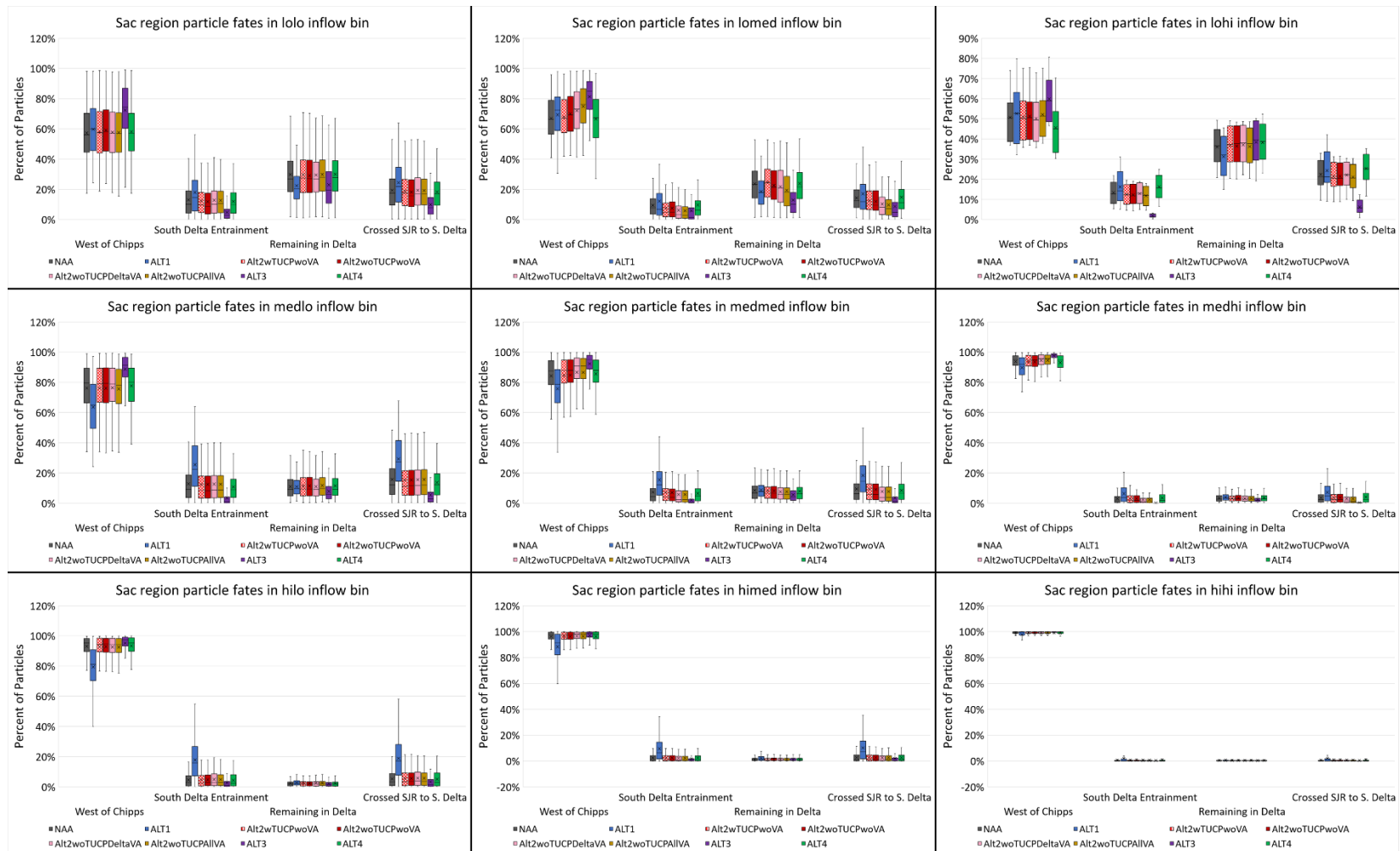
Figure I.8-77. Box and whisker plot of mean December through March particle fate after 45 days by exit location (within each facet from left to right: West of Chipps, South Delta Entrainment, Remaining in Delta, Crossed SJR to S. Delta) for neutrally buoyant particles injected at Sacramento River region by Inflow Bin (from top left to bottom right: "lolo" to "hihi") for the No Action Alternative, Alternative 1, four phases of Alternative 2, Alternative 3, and Alternative 4.
