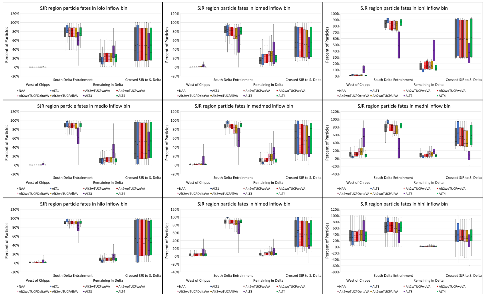
Figure I.8-78. Box and whisker plot of mean December through March particle fate after 45 days by exit location (within each facet from left to right: West of Chipps, South Delta Entrainment, Remaining in Delta, Crossed SJR to S. Delta) for neutrally buoyant particles injected at San Joaquin River region by Inflow Bin (from top left to bottom right: “lolo” to “hihi”) for the No Action Alternative, Alternative 1, four phases of Alternative 2, Alternative 3, and Alternative 4.
