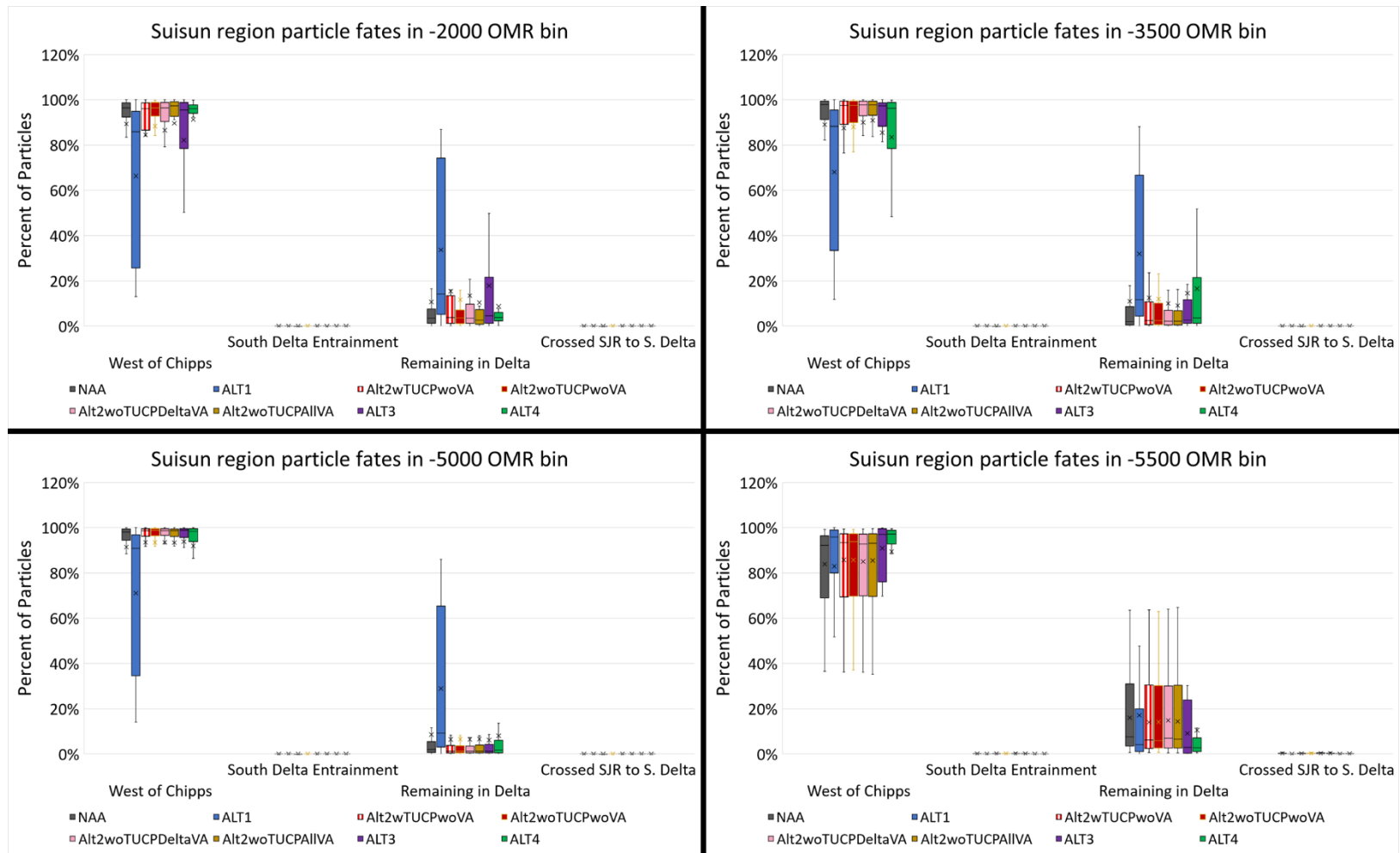
Figure I.8-89. Box and whisker plot of mean December through March particle fate after 45 days by exit location (within each facet from left to right: West of Chipps, South Delta Entrainment, Remaining in Delta, Crossed SJR to S. Delta) for neutrally buoyant particles injected at Suisun region by OMR Bin (from top left to bottom right: -2,000 cfs, -3,500 cfs, -5,000 cfs, -5,500 cfs) for the No Action Alternative, Alternative 1, four phases of Alternative 2, Alternative 3, and Alternative 4.
