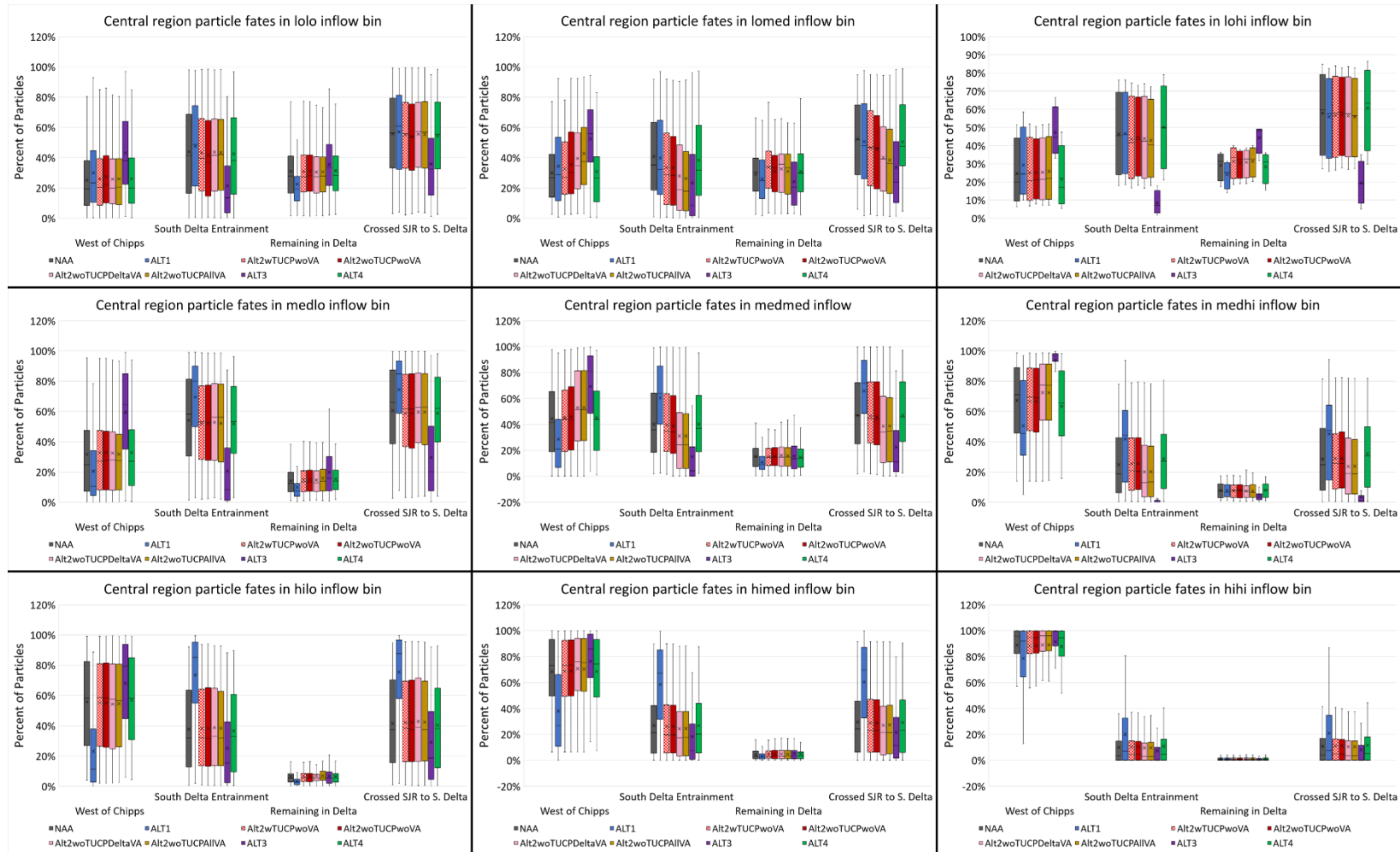
Figure 1.8-74. Box and whisker plot of mean December through March particle fate after 45 days by exit location (within each facet from left to right: West of Chipps, South Delta Entrainment, Remaining in Delta, Crossed SJR to S. Delta) for neutrally buoyant particles injected at Central Delta region by Inflow Bin (from top left to bottom right: "lolo" to "hihi") for the No Action Alternative, Alternative 1, four phases of Alternative 2, Alternative 3, and Alternative 4.
