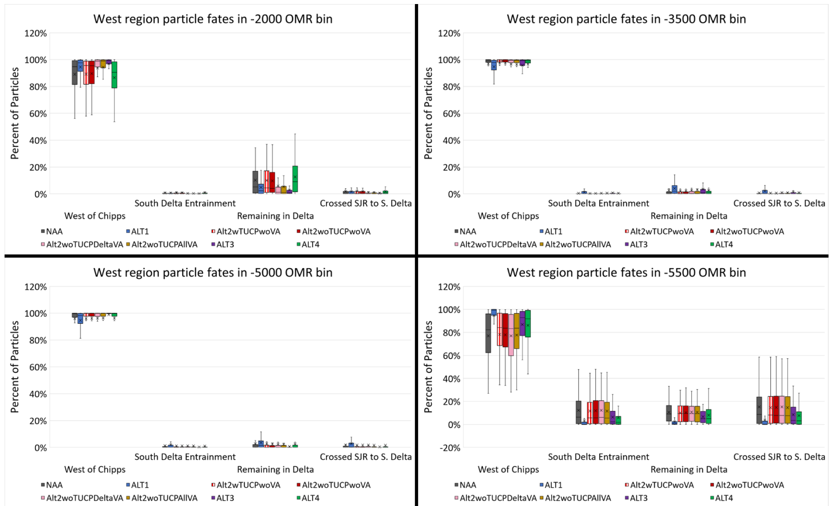
Figure I.8-90. Box and whisker plot of mean December through March particle fate after 45 days by exit location (within each facet from left to right: West of Chipps, South Delta Entrainment, Remaining in Delta, Crossed SJR to S. Delta) for neutrally buoyant particles injected at West Delta region by OMR Bin (from top left to bottom right: -2,000 cfs, -3,500 cfs, -5,000 cfs, -5,500 cfs) for the No Action Alternative, Alternative 1, four phases of Alternative 2, Alternative 3, and Alternative 4.
