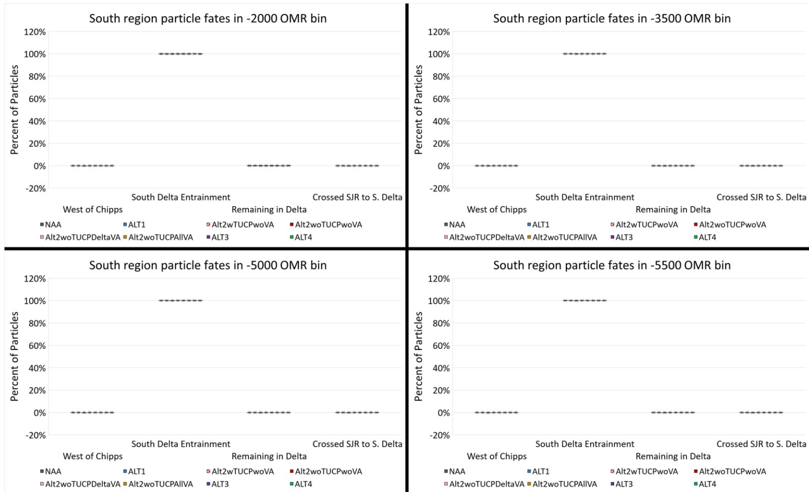
Figure I.8-70. Box and whisker plot of mean December through March particle fate after 45 days by exit location (within each facet from left to right: West of Chipps, South Delta Entrainment, Remaining in Delta, Crossed SJR to S. Delta) for surface oriented particles injected at South Delta region by OMR Bin (from top left to bottom right: -2,000 cfs, -3,500 cfs, -5,000 cfs, -5,500 cfs) for the No Action Alternative, Alternative 1, four phases of Alternative 2, Alternative 3, and Alternative 4.
