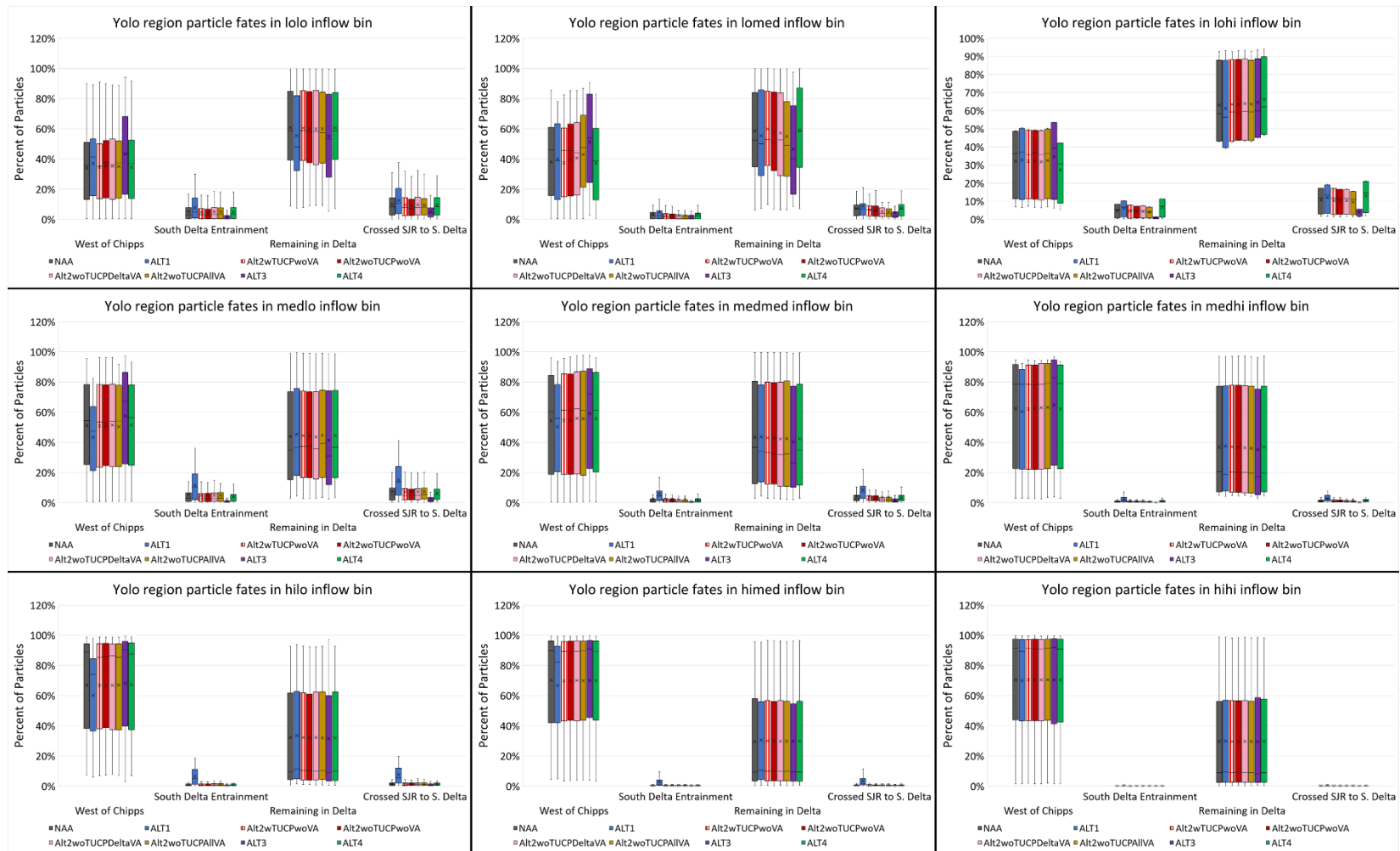
Figure I.8-82. Box and whisker plot of mean December through March particle fate after 45 days by exit location (within each facet from left to right: West of Chipps, South Delta Entrainment, Remaining in Delta, Crossed SJR to S. Delta) for neutrally buoyant particles injected at Yolo region by Inflow Bin (from top left to bottom right: "lolo" to "hihi") for the No Action Alternative, Alternative 1, four phases of Alternative 2, Alternative 3, and Alternative 4.
