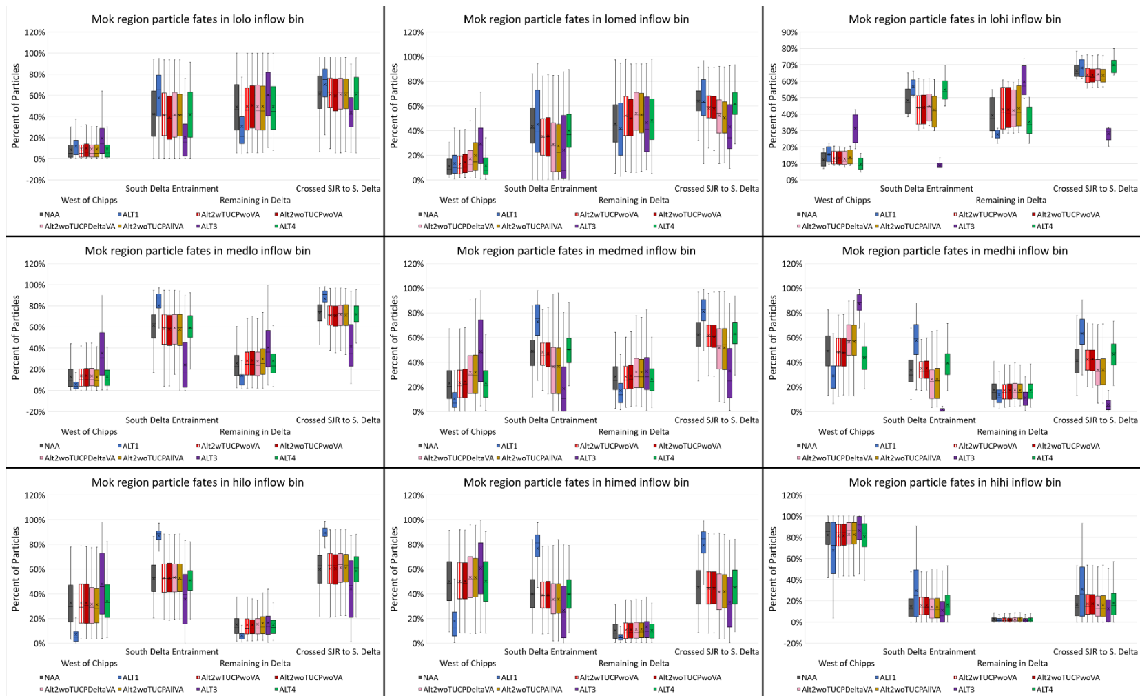
Figure I.8-75. Box and whisker plot of mean December through March particle fate after 45 days by exit location (within each facet from left to right: West of Chipps, South Delta Entrainment, Remaining in Delta, Crossed SJR to S. Delta) for neutrally buoyant particles injected at Mokelumne River region by Inflow Bin (from top left to bottom right: "lolo" to "hihi") for the No Action Alternative, Alternative 1, four phases of Alternative 2, Alternative 3, and Alternative 4.
