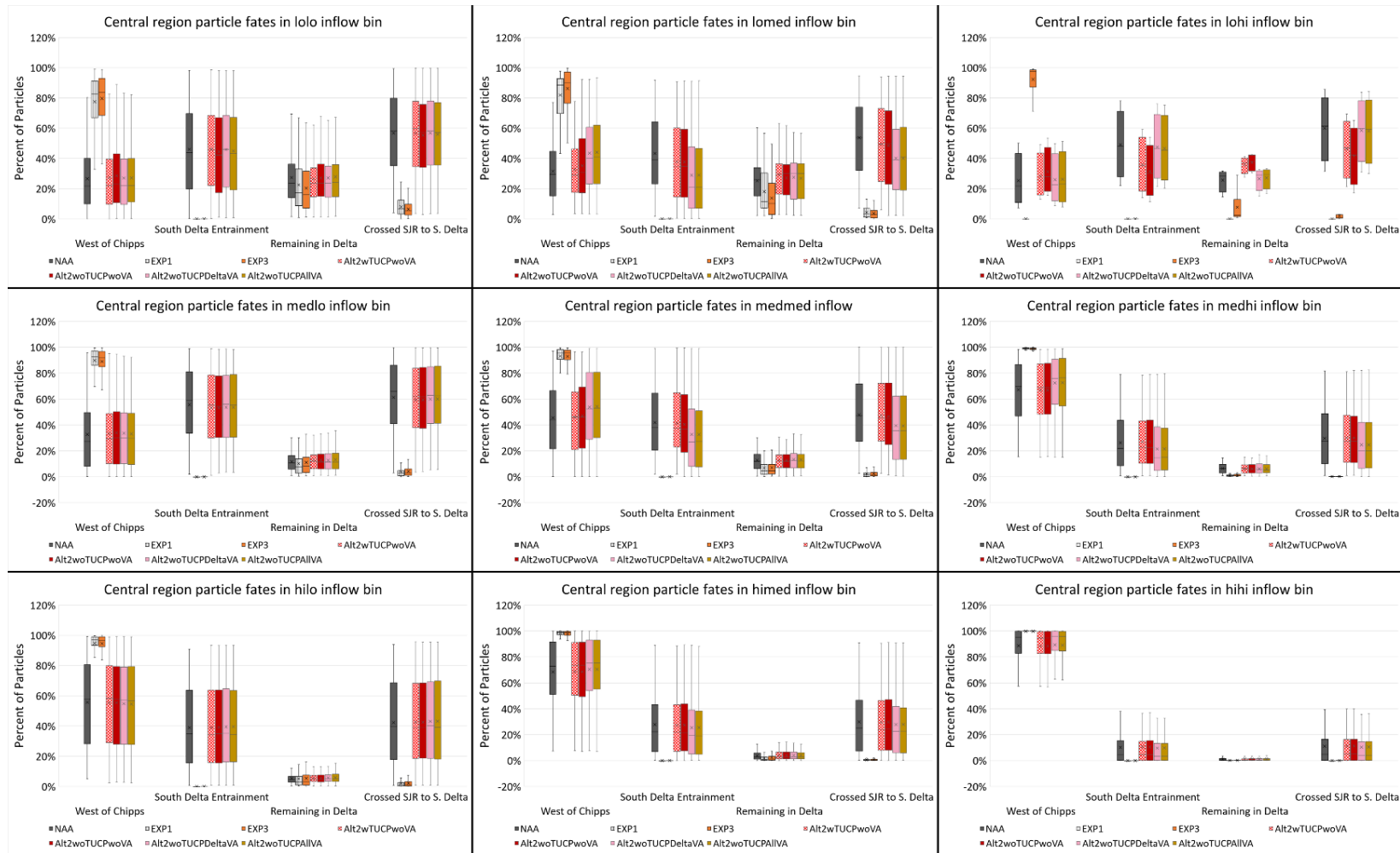
Figure 1.8-20. Box and whisker plot of mean December through March particle fate after 45 days by exit location (within each facet from left to right: West of Chipps, South Delta Entrainment, Remaining in Delta, Crossed SJR to S. Delta) for surface oriented particles injected at Central Delta region by Inflow Bin (from top left to bottom right: "lolo" to "hihi") for the No Action Alternative, EXP 1, EXP 3, and four phases of Alternative 2.
