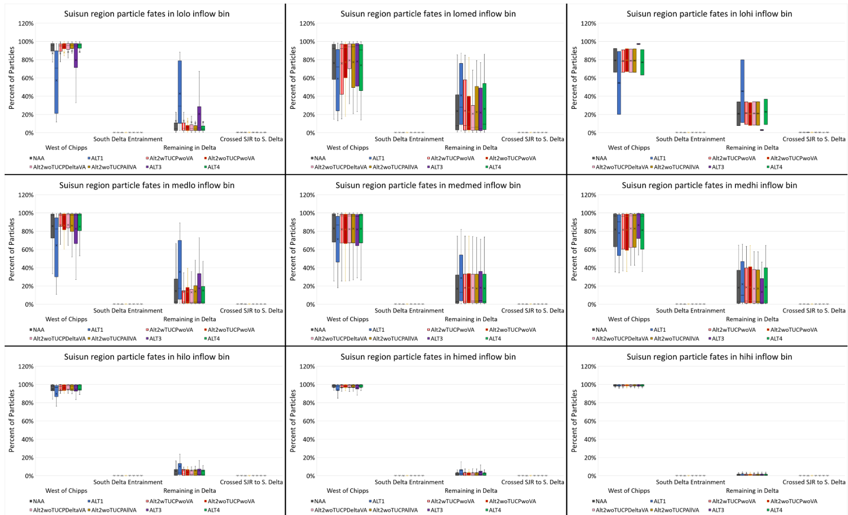
Figure I.8-80. Box and whisker plot of mean December through March particle fate after 45 days by exit location (within each facet from left to right: West of Chipps, South Delta Entrainment, Remaining in Delta, Crossed SJR to S. Delta) for neutrally buoyant particles injected at Suisun region by Inflow Bin (from top left to bottom right: "lolo" to "hihi") for the No Action Alternative, Alternative 1, four phases of Alternative 2, Alternative 3, and Alternative 4.
