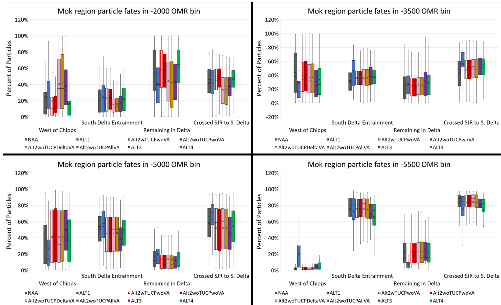
Figure I.8-84. Box and whisker plot of mean December through March particle fate after 45 days by exit location (within each facet from left to right: West of Chipps, South Delta Entrainment, Remaining in Delta, Crossed SJR to S. Delta) for neutrally buoyant particles injected at Mokelumne River region by OMR Bin (from top left to bottom right: -2,000 cfs, -3,500 cfs, -5,000 cfs, -5,500 cfs) for the No Action Alternative, Alternative 1, four phases of Alternative 2, Alternative 3, and Alternative 4.
