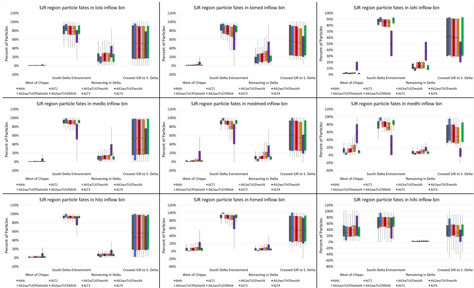
Figure I.8-60. Box and whisker plot of mean December through March particle fate after 45 days by exit location (within each facet from left to right: West of Chipps, South Delta Entrainment, Remaining in Delta, Crossed SJR to S. Delta) for surface oriented particles injected at San Joaquin River region by Inflow Bin (from top left to bottom right: "lolo" to "hihi") for the No Action Alternative, Alternative 1, four phases of Alternative 2, Alternative 3, and Alternative 4.
