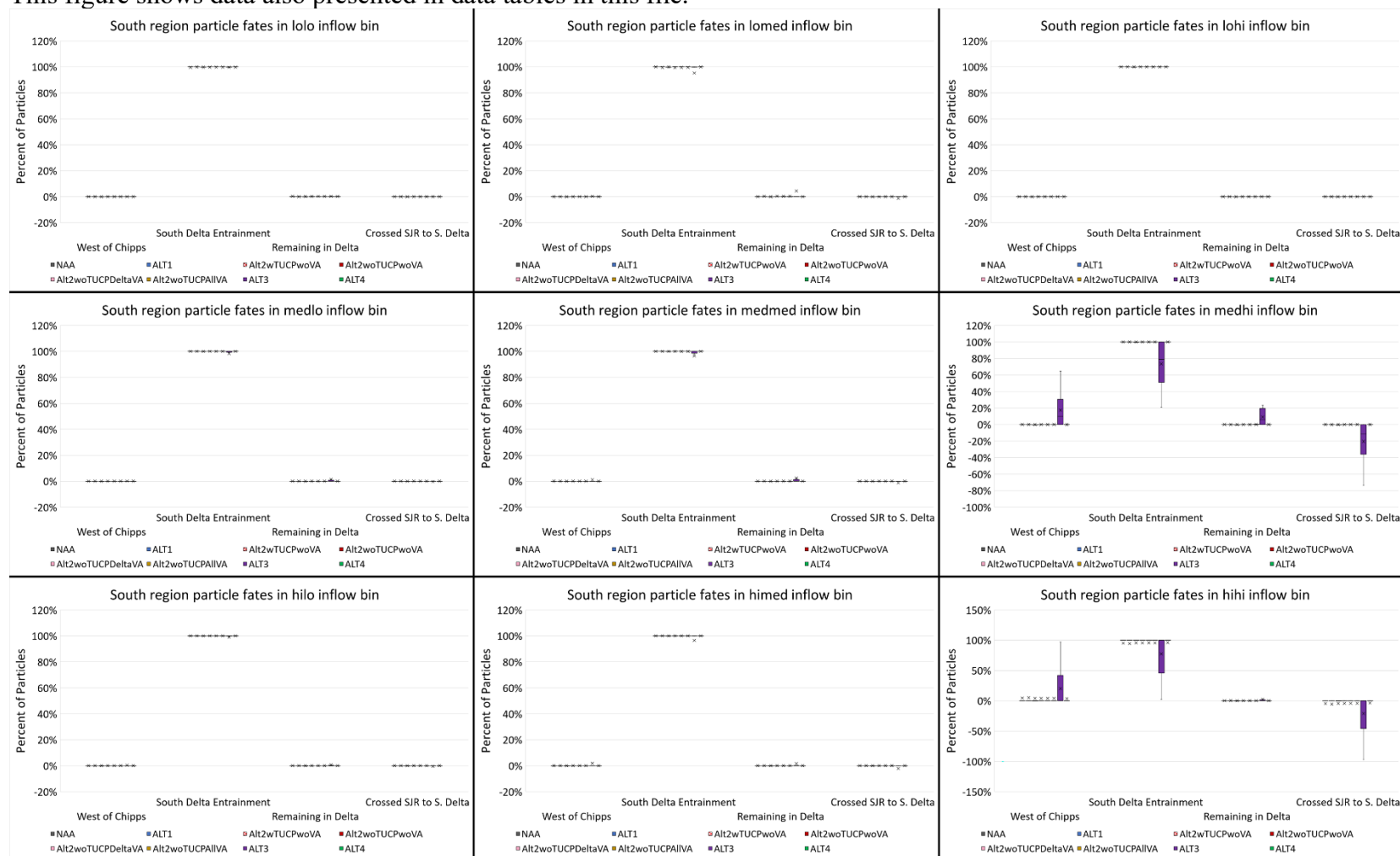
Figure I.8-79. Box and whisker plot of mean December through March particle fate after 45 days by exit location (within each facet from left to right: West of Chipps, South Delta Entrainment, Remaining in Delta, Crossed SJR to S. Delta) for neutrally buoyant particles injected at South Delta region by Inflow Bin (from top left to bottom right: "lolo" to "hihi") for the No Action Alternative, Alternative 1, four phases of Alternative 2, Alternative 3, and Alternative 4.
