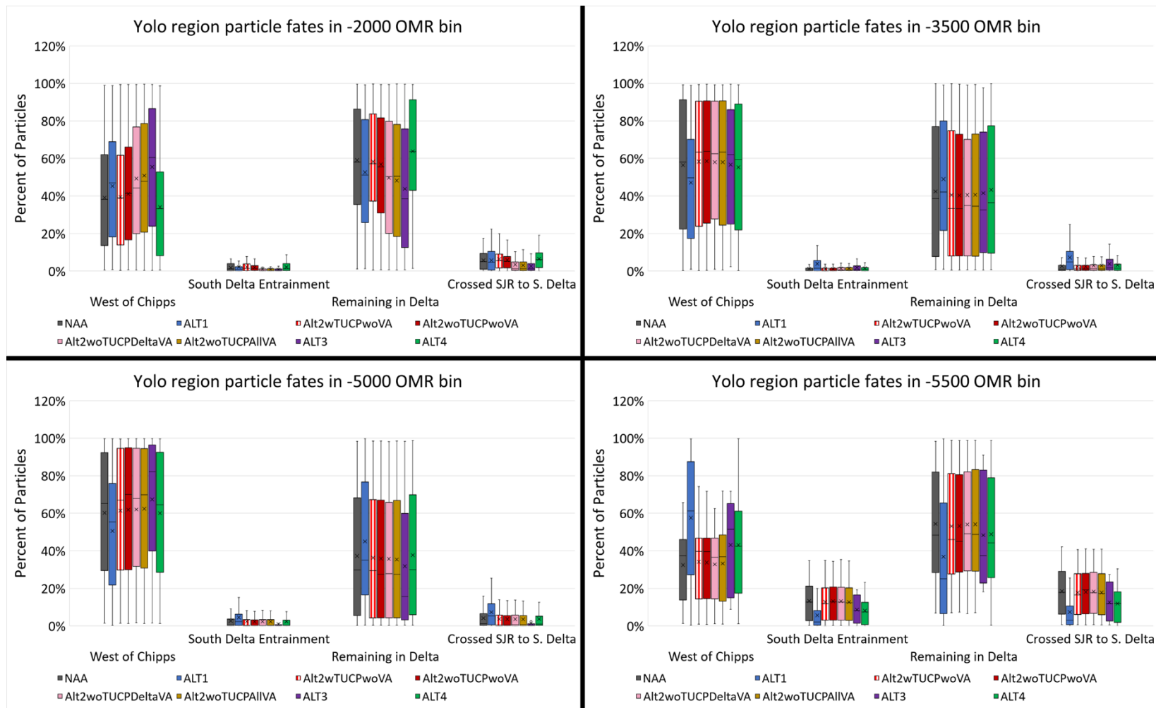
Figure I.8-91. Box and whisker plot of mean December through March particle fate after 45 days by exit location (within each facet from left to right: West of Chipps, South Delta Entrainment, Remaining in Delta, Crossed SJR to S. Delta) for neutrally buoyant particles injected at Yolo region by OMR Bin (from top left to bottom right: -2,000 cfs, -3,500 cfs, -5,000 cfs, -5,500 cfs) for the No Action Alternative, Alternative 1, four phases of Alternative 2, Alternative 3, and Alternative 4.
