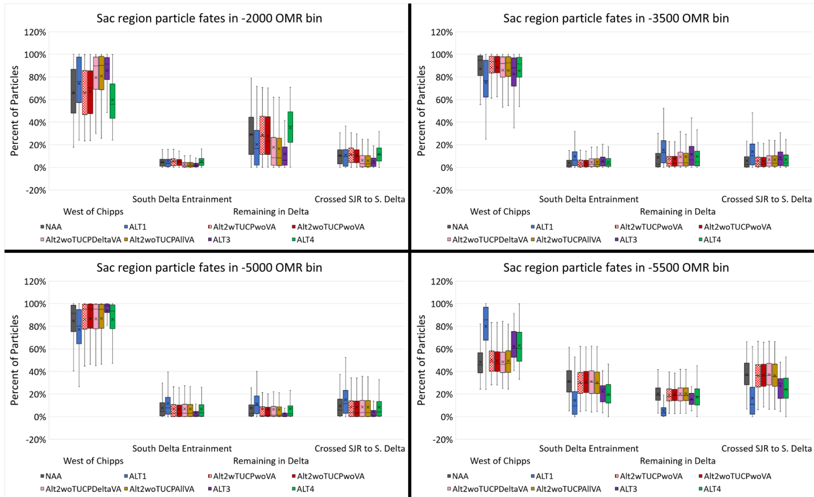
Figure I.8-86. Box and whisker plot of mean December through March particle fate after 45 days by exit location (within each facet from left to right: West of Chipps, South Delta Entrainment, Remaining in Delta, Crossed SJR to S. Delta) for neutrally buoyant particles injected at Sacramento River region by OMR Bin (from top left to bottom right: -2,000 cfs, -3,500 cfs, -5,000 cfs, -5,500 cfs) for the No Action Alternative, Alternative 1, four phases of Alternative 2, Alternative 3, and Alternative 4.
