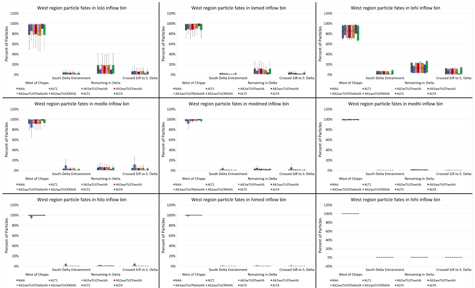
Figure I.8-81. Box and whisker plot of mean December through March particle fate after 45 days by exit location (within each facet from left to right: West of Chipps, South Delta Entrainment, Remaining in Delta, Crossed SJR to S. Delta) for neutrally buoyant particles injected at West Delta region by Inflow Bin (from top left to bottom right: "lolo" to "hihi") for the No Action Alternative, Alternative 1, four phases of Alternative 2, Alternative 3, and Alternative 4.
