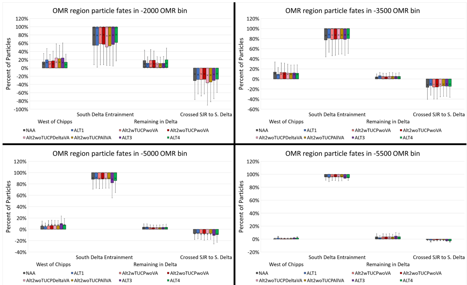
Figure I.8-85. Box and whisker plot of mean December through March particle fate after 45 days by exit location (within each facet from left to right: West of Chipps, South Delta Entrainment, Remaining in Delta, Crossed SJR to S. Delta) for neutrally buoyant particles injected at Old and Middle River region by OMR Bin (from top left to bottom right: -2,000 cfs, -3,500 cfs, -5,000 cfs, -5,500 cfs) for the No Action Alternative, Alternative 1, four phases of Alternative 2, Alternative 3, and Alternative 4.
