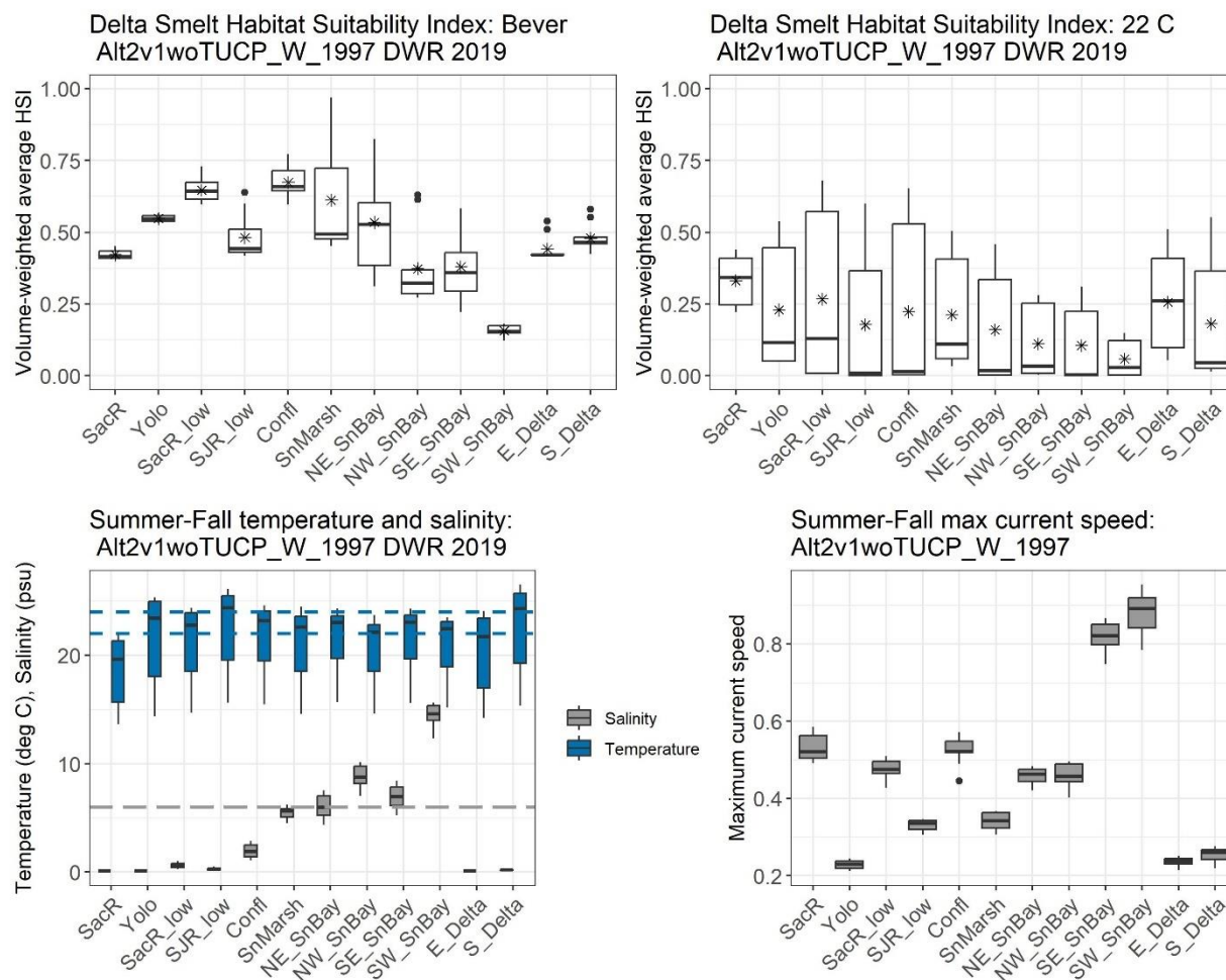
Figure K.1-40. Top left graph: Bever et al. (2016) habitat suitability indices for each subregion. Top right graph: Bever et al. (2016) habitat suitability indices and indices modified by a 22-degree Celsius threshold for each subregion. Lower left graph: temperature (in blue) and salinity (in gray) for each subregion; the dashed gray line indicates the 6 ppt salinity threshold; the dashed blue lines indicate the 22° and 24° C temperature thresholds. Lower right graph: maximum current speed for each subregion. In all graphs, data for the July 1 – November 18 in the wet water year (1997) are shown for alternative 2 without temporary urgency change, without Voluntary Agreements (Alt2v1woTUCP), using DWR 2019 air inputs. The median is shown as the horizontal line, the mean is shown with an asterisk (HSI graphs only), the box indicates the 25th and 75th percentiles, the vertical lines indicate the 25th and 75th percentiles plus 1.5 times the interquartile range, and the dots indicate potential outliers.
