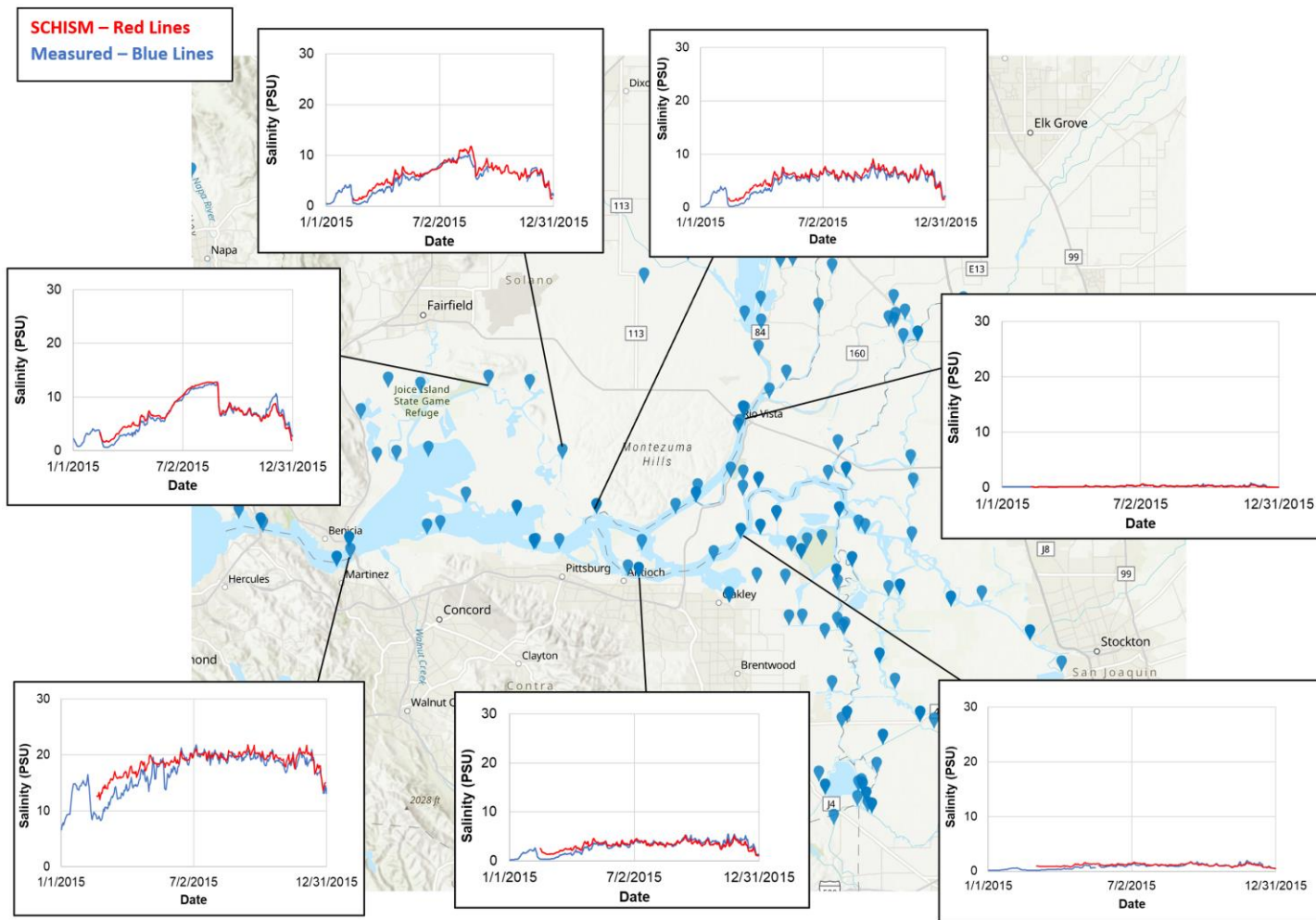
Figure K.1-14. Visual comparison between tidally-averaged measured and SCHISM-predicted stream salinities at select monitoring stations across the model domain for 2015.
