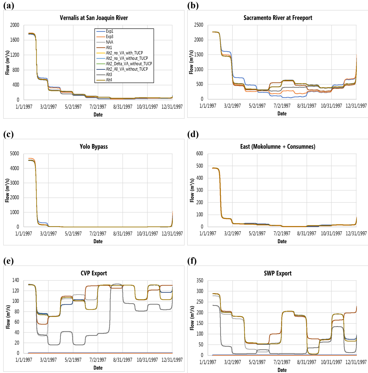
Figure K.1-3. Summary of major inflow and export boundary conditions for W year (1997) for all alternatives at (a) Vernalis at San Joaquin River (inflow); (b) Sacramento River at Freeport (inflow); (c) Yolo Bypass (inflow); (d) Mokolumne and Consumnes (inflow); (e) CVP (export), and; (f) SWP (export)
