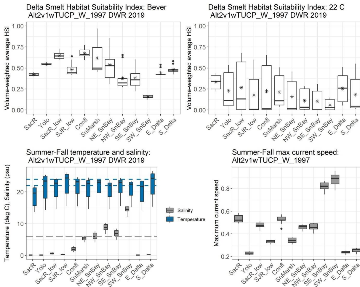
Figure K.1-39. Top left graph: Bever et al. (2016) habitat suitability indices for each subregion. Top right graph: Bever et al. (2016) habitat suitability indices and indices modified by a 22-degree Celsius threshold for each subregion. Lower left graph: temperature (in blue) and salinity (in gray) for each subregion; the dashed gray line indicates the 6 ppt salinity threshold; the dashed blue lines indicate the 22° and 24° C temperature thresholds. Lower right graph: maximum current speed for each subregion. In all graphs, data for the July 1 – November 18 in the wet water year (1997) are shown for alternative 2 with temporary urgency change, without Voluntary Agreements (Alt2v1wTUCP), using DWR 2019 air inputs. The median is shown as the horizontal line, the mean is shown with an asterisk (HSI graphs only), the box indicates the 25th and 75th percentiles, the vertical lines indicate the 25th and 75th percentiles plus 1.5 times the interquartile range, and the dots indicate potential outliers.
