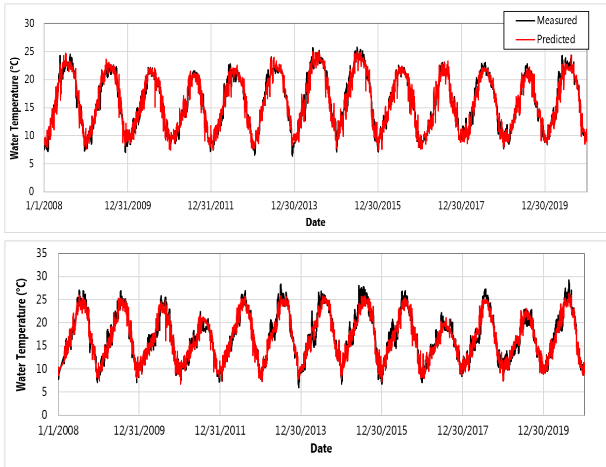
Figure K.1-7. Measured and ANN-predicted stream water temperatures from 2008 to 2020 at: (a) Sacramento River at Freeport, and (b) San Joaquin River at Vernalis
