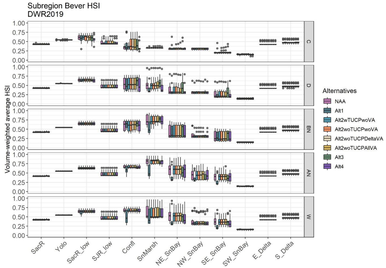
Figure K.1-32. Bever et al. (2016) habitat suitability indices for each alternative and water year type for July 1 – November 18. The median is shown as the horizontal line, the box indicates the 25th and 75th percentiles, the vertical lines indicate the 25th and 75th percentiles plus 1.5 times the interquartile range, and the dots indicate potential outliers. The alternatives, from left to right are: no action alternative (NAA); alternative 1 (Alt1); alternative 2 with temporary urgency change, without Voluntary Agreements (Alt2wTUCPwoVA); alternative 2 without temporary urgency change, without Voluntary Agreements (Alt2woTUCPwoVA); alternative 2 without temporary urgency change, with Delta Voluntary Agreements (Alt2woTUCPDeltaVA); alternative 2 without temporary urgency change, with all Voluntary Agreements (Alt2woTUCPAIIVA); alternative 3 (Alt3); alternative 4 (Alt4). Water year types presented from top to bottom panels are: critical (C); dry (D); below normal (BN); above normal (AN); wet (W).
