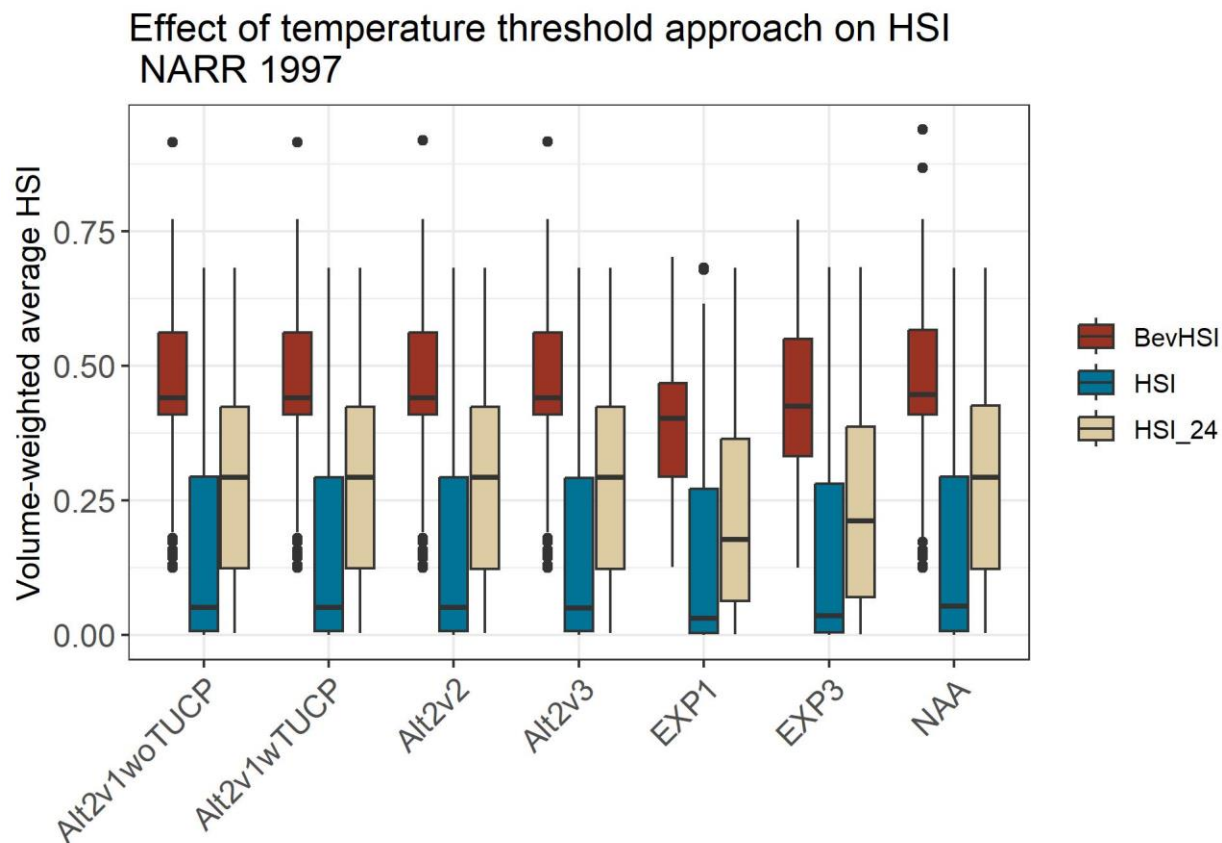
Figure K.1-86. Habitat suitability index (HSI) from July 1 – November 18 calculated using Bever et al. (2016) and Bever et al. (2016) modified by the 22°C and 24°C thresholds and using the NARR 1997 air temperature for each alternative for the 1997 wet water year. The median is shown as the horizontal line, the box indicates the 25th and 75th percentiles, the vertical lines indicate the the 25th and 75th percentiles plus 1.5 times the interquartile range, and the dots indicate potential outliers. The HSI calculations, from left to right are: BevHSI = Bever et al. (2016); HSI = Bever et al. (2016) modified by the 22°C threshold; and HSI_24 = Bever et al. (2016) modified by the 24°C threshold.
