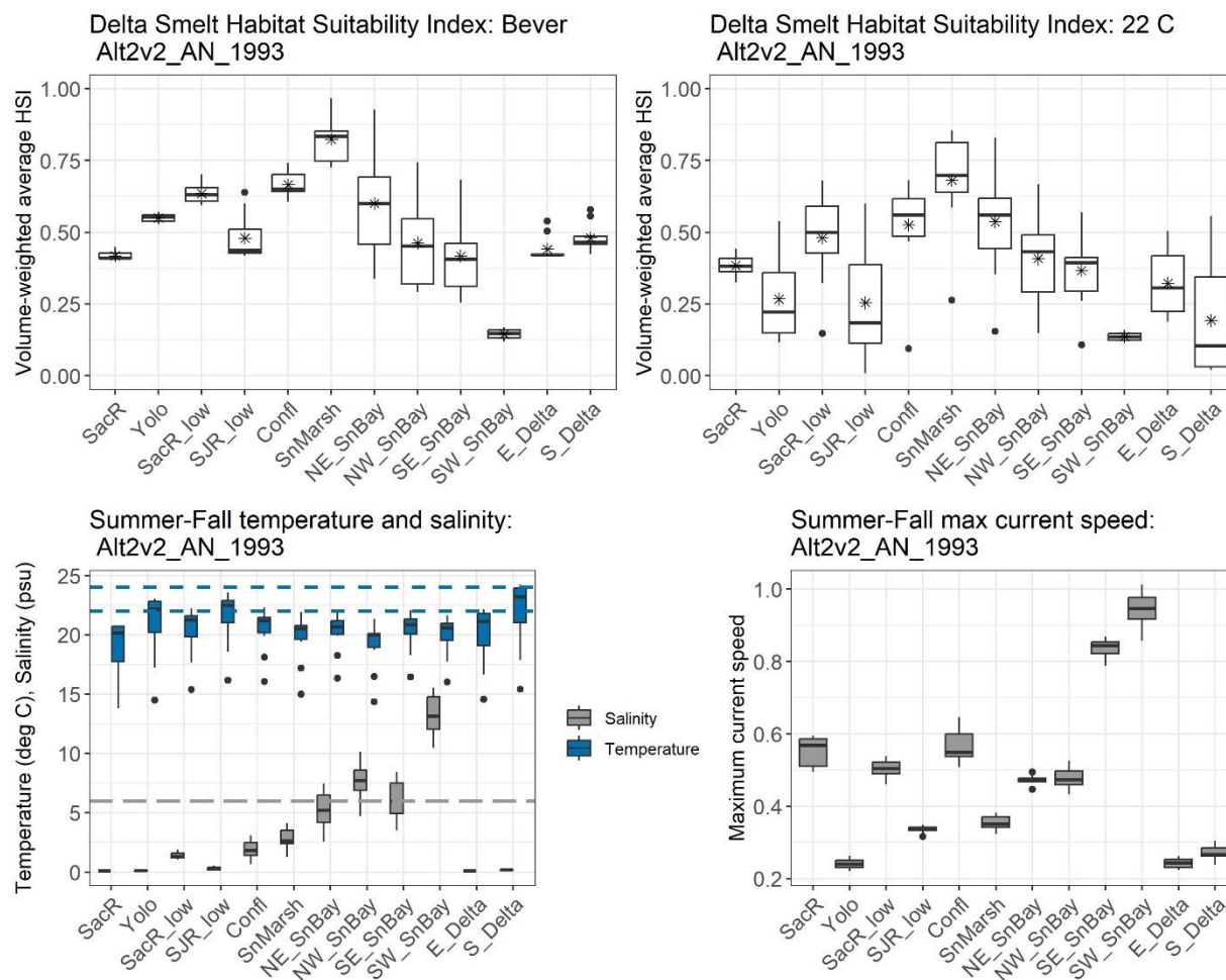
Figure K.1-51. Top left graph: Bever et al. (2016) habitat suitability indices for each subregion. Top right graph: Bever et al. (2016) habitat suitability indices and indices modified by a 22-degree Celsius threshold for each subregion. Lower left graph: temperature (in blue) and salinity (in gray) for each subregion; the dashed gray line indicates the 6 ppt salinity threshold; the dashed blue lines indicate the 22° and 24° C temperature thresholds. Lower right graph: maximum current speed for each subregion. In all graphs, data for the July 1 – November 18 in the above normal water year (1993) are shown for alternative 2 without temporary urgency change, with Delta Voluntary Agreements (Alt2v2), using DWR 2010 air inputs. The median is shown as the horizontal line, the mean is shown with an asterisk (HSI graphs only), the box indicates the 25th and 75th percentiles, the vertical lines indicate the 25th and 75th percentiles plus 1.5 times the interquartile range, and the dots indicate potential outliers.
