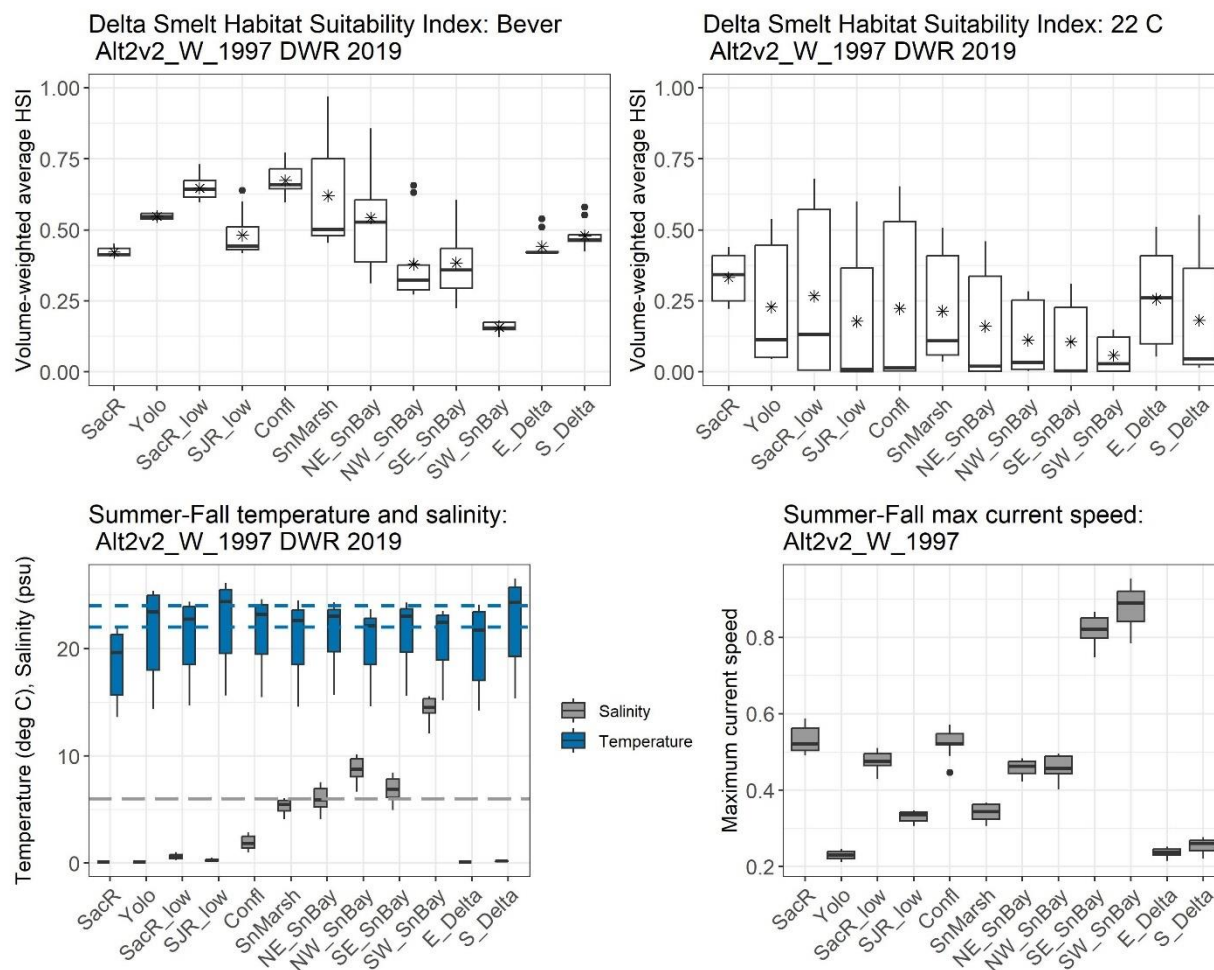
Figure K.1-41. Top left graph: Bever et al. (2016) habitat suitability indices for each subregion. Top right graph: Bever et al. (2016) habitat suitability indices and indices modified by a 22-degree Celsius threshold for each subregion. Lower left graph: temperature (in blue) and salinity (in gray) for each subregion; the dashed gray line indicates the 6 ppt salinity threshold; the dashed blue lines indicate the 22° and 24° C temperature thresholds. Lower right graph: maximum current speed for each subregion. In all graphs, data for the July 1 – November 18 in the wet water year (1997) are shown for alternative 2 without temporary urgency change, with Delta Voluntary Agreements (Alt2v2), using DWR 2019 air inputs. The median is shown as the horizontal line, the mean is shown with an asterisk (HSI graphs only), the box indicates the 25th and 75th percentiles, the vertical lines indicate the 25th and 75th percentiles plus 1.5 times the interquartile range, and the dots indicate potential outliers.
