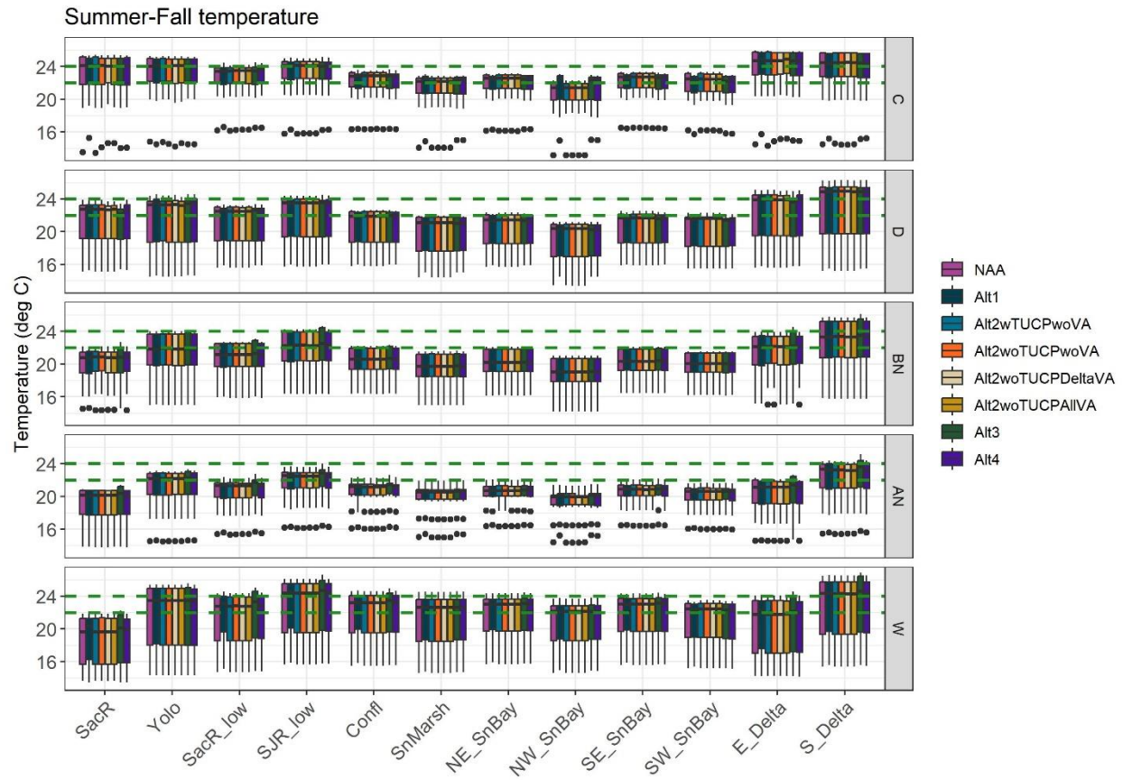
Figure K.1-16. Delta subregion temperatures (degrees Celsius [°C]) from July 1 – November 18 for each alternative and water year. The median is shown as the horizontal line, the box indicates the 25th and 75th percentiles, the vertical lines indicate the 25th and 75th percentiles plus 1.5 times the interquartile range, and the dots indicate potential outliers. The alternatives, from left to right are: no action alternative (NAA); alternative 1 (Alt1); alternative 2 with temporary urgency change, without Voluntary Agreements (Alt2wTUCPwoVA); alternative 2 without temporary urgency change, without Voluntary Agreements (Alt2woTUCPwoVA); alternative 2 without temporary urgency change, with Delta Voluntary Agreements (Alt2woTUCPDeltaVA); alternative 2 without temporary urgency change, with all Voluntary Agreements (Alt2woTUCPAIIVA); alternative 3 (Alt3); and alternative 4 (Alt4). The green dashed lines indicate the 22 C and 24 C temperature thresholds that have been used to modify the Bever et al. (2016) Delta Smelt habitat suitability index. Water year types presented from top to bottom panels are: critical (C); dry (D); below normal (BN); above normal (AN); wet (W).
