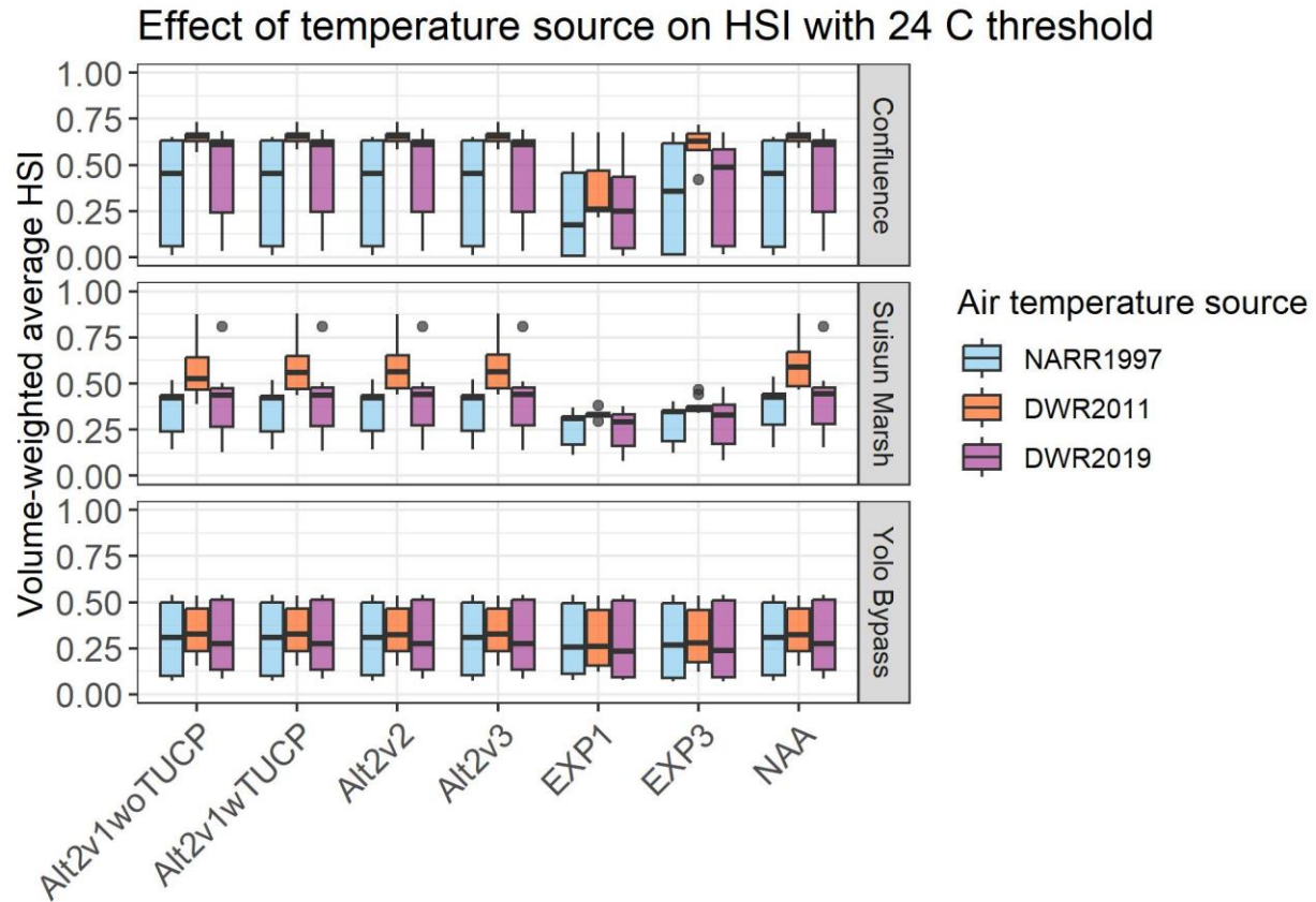
Figure K.1-91. Bever et al. (2016) modified by a 24-degree Celsius threshold from July 1 – November 18 using the NARR 1997, DWR 2011, and DWR 2019 air inputs for each alternative for the 1997 wet water year. The median is shown as the horizontal line, the box indicates the 25th and 75th percentiles, the vertical lines indicate the 25th and 75th percentiles plus 1.5 times the interquartile range, and the dots indicate potential outliers.
