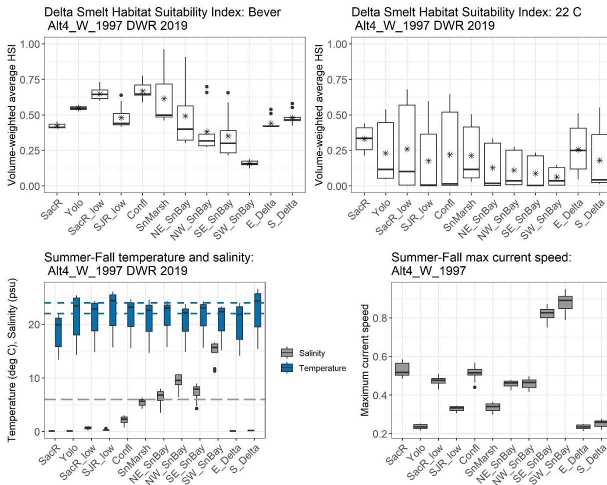
Figure K.1-44. Top left graph: Bever et al. (2016) habitat suitability indices for each subregion. Top right graph: Bever et al. (2016) habitat suitability indices and indices modified by a 22-degree Celsius threshold for each subregion. Lower left graph: temperature (in blue) and salinity (in gray) for each subregion; the dashed gray line indicates the 6 ppt salinity threshold; the dashed blue lines indicate the 22° and 24° C temperature thresholds. Lower right graph: maximum current speed for each subregion. In all graphs, data for the July 1 – November 18 in the wet water year (1997) are shown for alternative 4 (Alt4), using DWR 2019 air inputs. The median is shown as the horizontal line, the mean is shown with an asterisk (HSI graphs only), the box indicates the 25th and 75th percentiles, the vertical lines indicate the 25th and 75th percentiles plus 1.5 times the interquartile range, and the dots indicate potential outliers.
