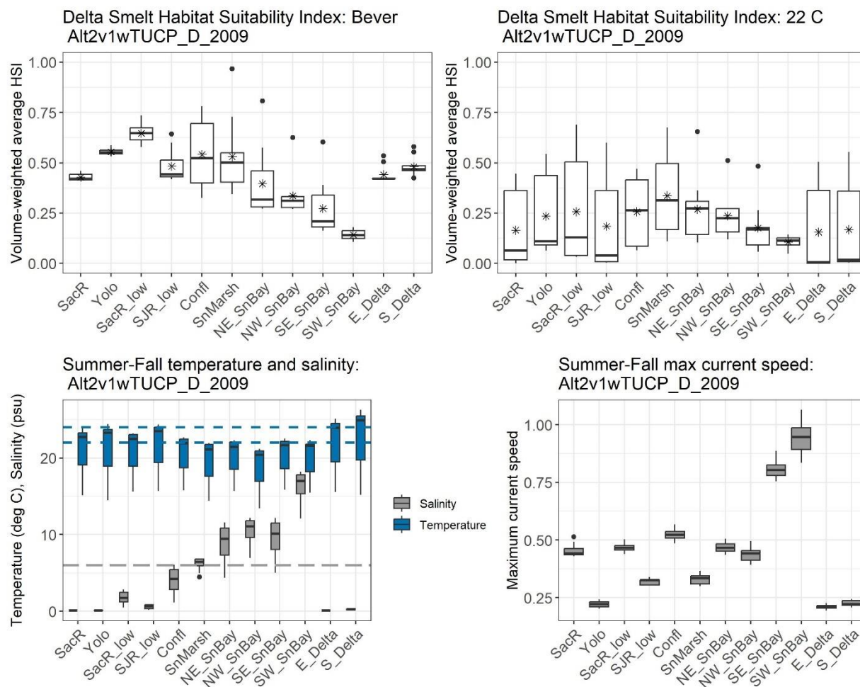
Figure K.1-69. Top left graph: Bever et al. (2016) habitat suitability indices for each subregion. Top right graph: Bever et al. (2016) habitat suitability indices and indices modified by a 22-degree Celsius threshold for each subregion. Lower left graph: temperature (in blue) and salinity (in gray) for each subregion; the dashed gray line indicates the 6 ppt salinity threshold; the dashed blue lines indicate the 22° and 24° C temperature thresholds. Lower right graph: maximum current speed for each subregion. In all graphs, data for the July 1 – November 18 in the dry water year (2009) are shown for alternative 2 with temporary urgency change, without Voluntary Agreements (Alt2v1wTUCP). The median is shown as the horizontal line, the mean is shown with an asterisk (HSI graphs only), the box indicates the 25th and 75th percentiles, the vertical lines indicate the 25th and 75th percentiles plus 1.5 times the interquartile range, and the dots indicate potential outliers.
