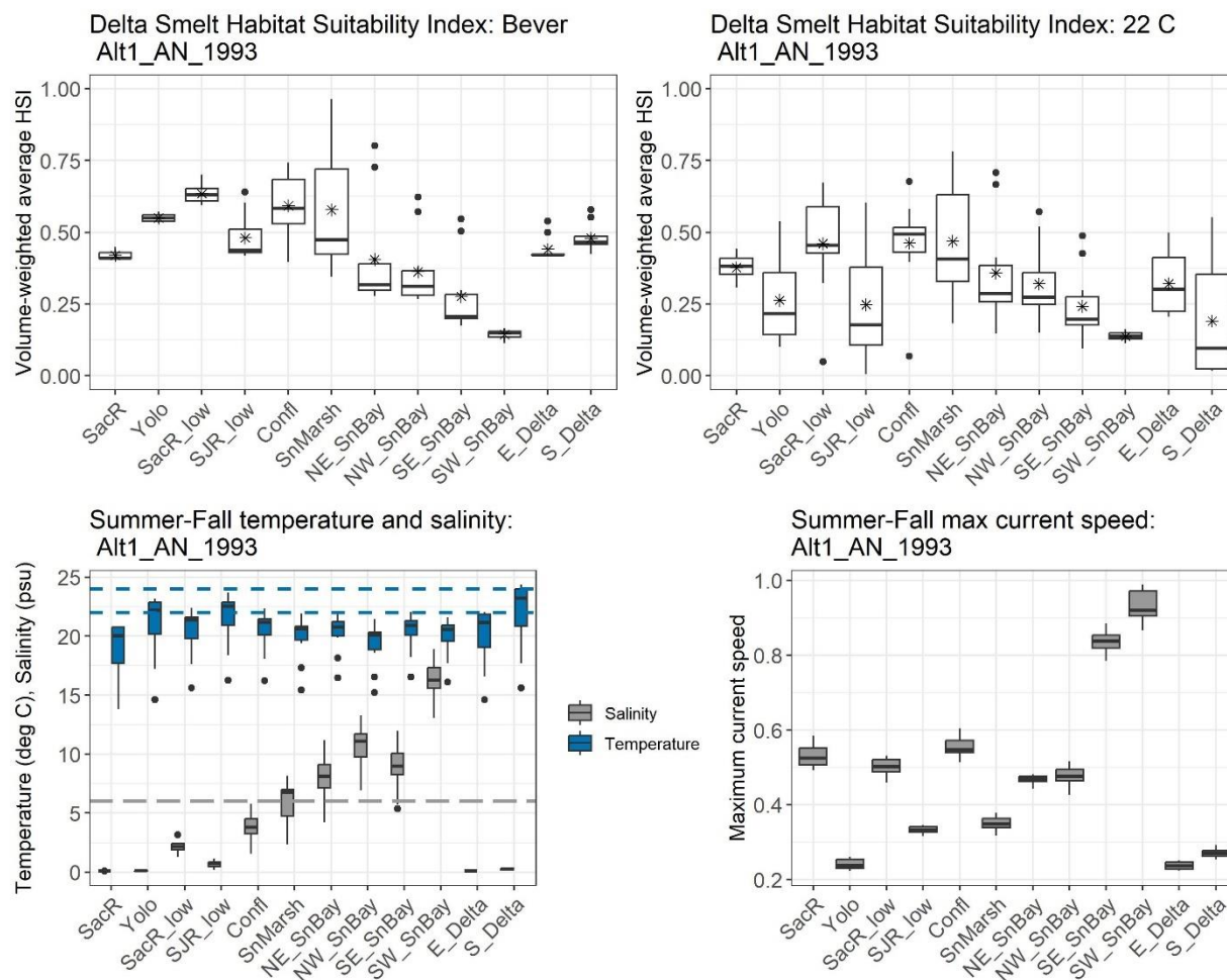
Figure K.1-48. Top left graph: Bever et al. (2016) habitat suitability indices for each subregion. Top right graph: Bever et al. (2016) habitat suitability indices and indices modified by a 22-degree Celsius threshold for each subregion. Lower left graph: temperature (in blue) and salinity (in gray) for each subregion; the dashed gray line indicates the 6 ppt salinity threshold; the dashed blue lines indicate the 22° and 24° C temperature thresholds. Lower right graph: maximum current speed for each subregion. In all graphs, data for the July 1 – November 18 in the above normal water year (1993) are shown for Alternative 1 (Alt1), using DWR 2010 air inputs. The median is shown as the horizontal line, the mean is shown with an asterisk (HSI graphs only), the box indicates the 25th and 75th percentiles, the vertical lines indicate the 25th and 75th percentiles plus 1.5 times the interquartile range, and the dots indicate potential outliers.
