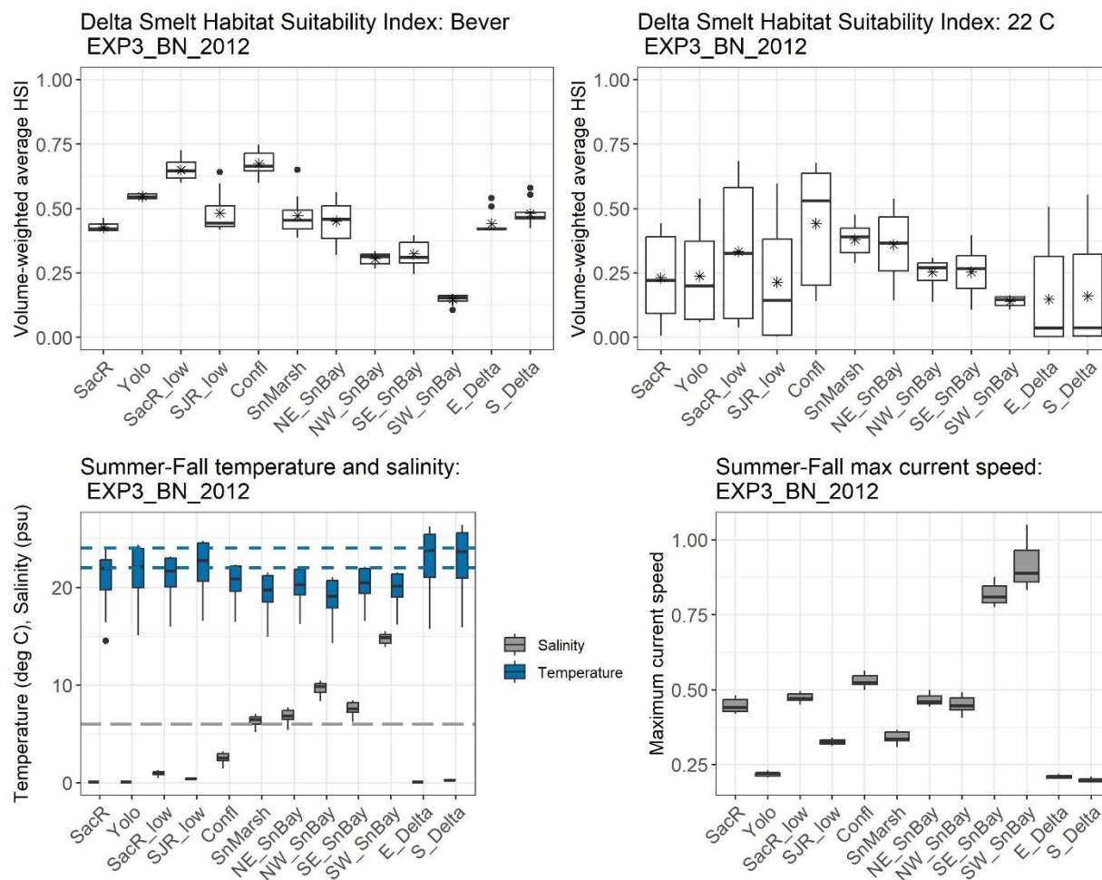
Figure K.1-56. Top left graph: Bever et al. (2016) habitat suitability indices for each subregion. Top right graph: Bever et al. (2016) habitat suitability indices and indices modified by a 22-degree Celsius threshold for each subregion. Lower left graph: temperature (in blue) and salinity (in gray) for each subregion; the dashed gray line indicates the 6 ppt salinity threshold; the dashed blue lines indicate the 22° and 24° C temperature thresholds. Lower right graph: maximum current speed for each subregion. In all graphs, data for the July 1 – November 18 in the below normal water year (2012) are shown for exploratory 3 (EXP3). The median is shown as the horizontal line, the mean is shown with an asterisk (HSI graphs only), the box indicates the 25th and 75th percentiles, the vertical lines indicate the 25th and 75th percentiles plus 1.5 times the interquartile range, and the dots indicate potential outliers.
