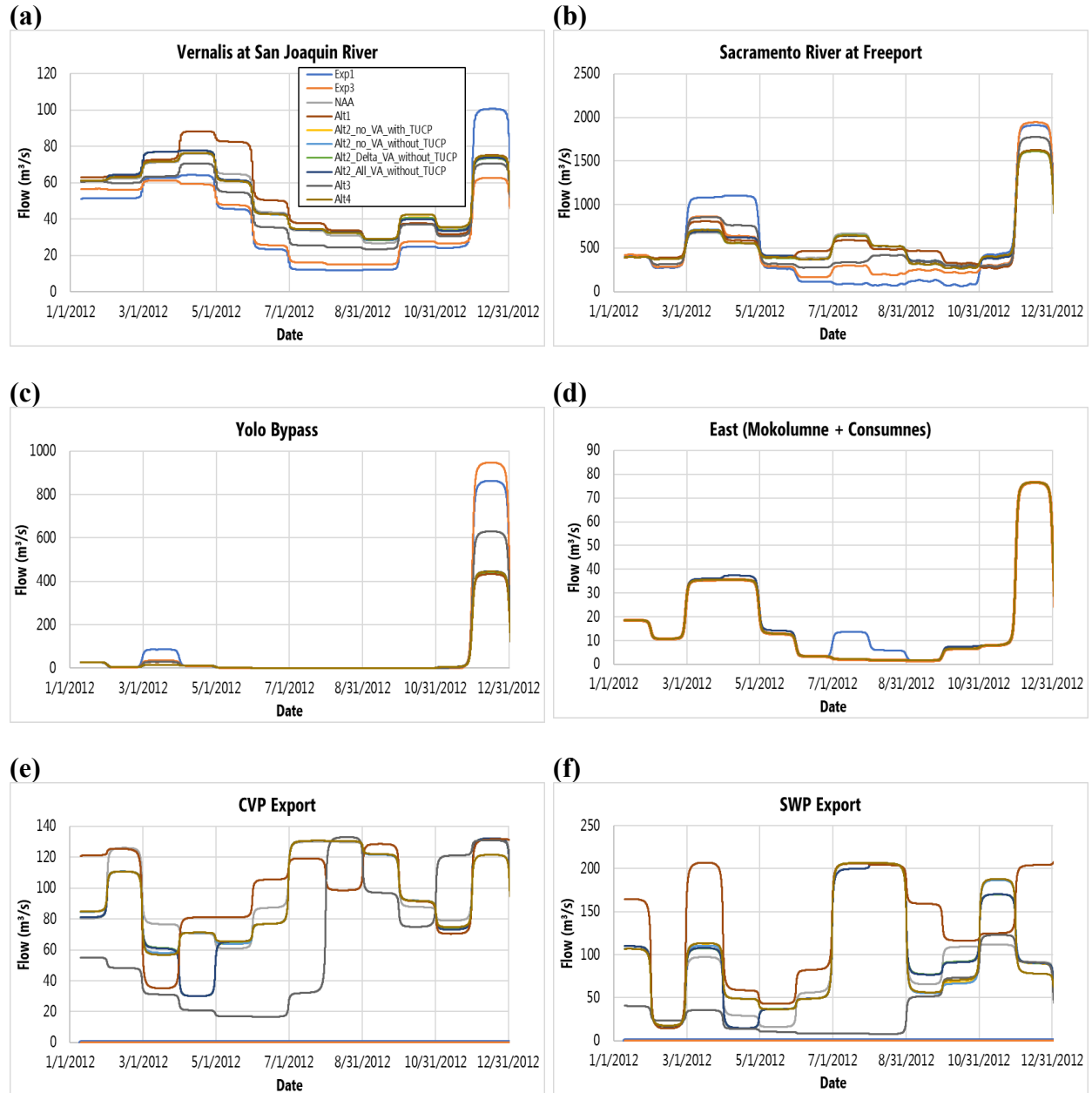
Figure K.1-5. Summary of major inflow and export boundary conditions for BN year (2012) for all alternatives at (a) Vernalis at San Joaquin River (inflow); (b) Sacramento River at Freeport (inflow); (c) Yolo Bypass (inflow); (d) Mokolumne and Consumnes (inflow); (e) CVP (export), and; (f) SWP (export)
