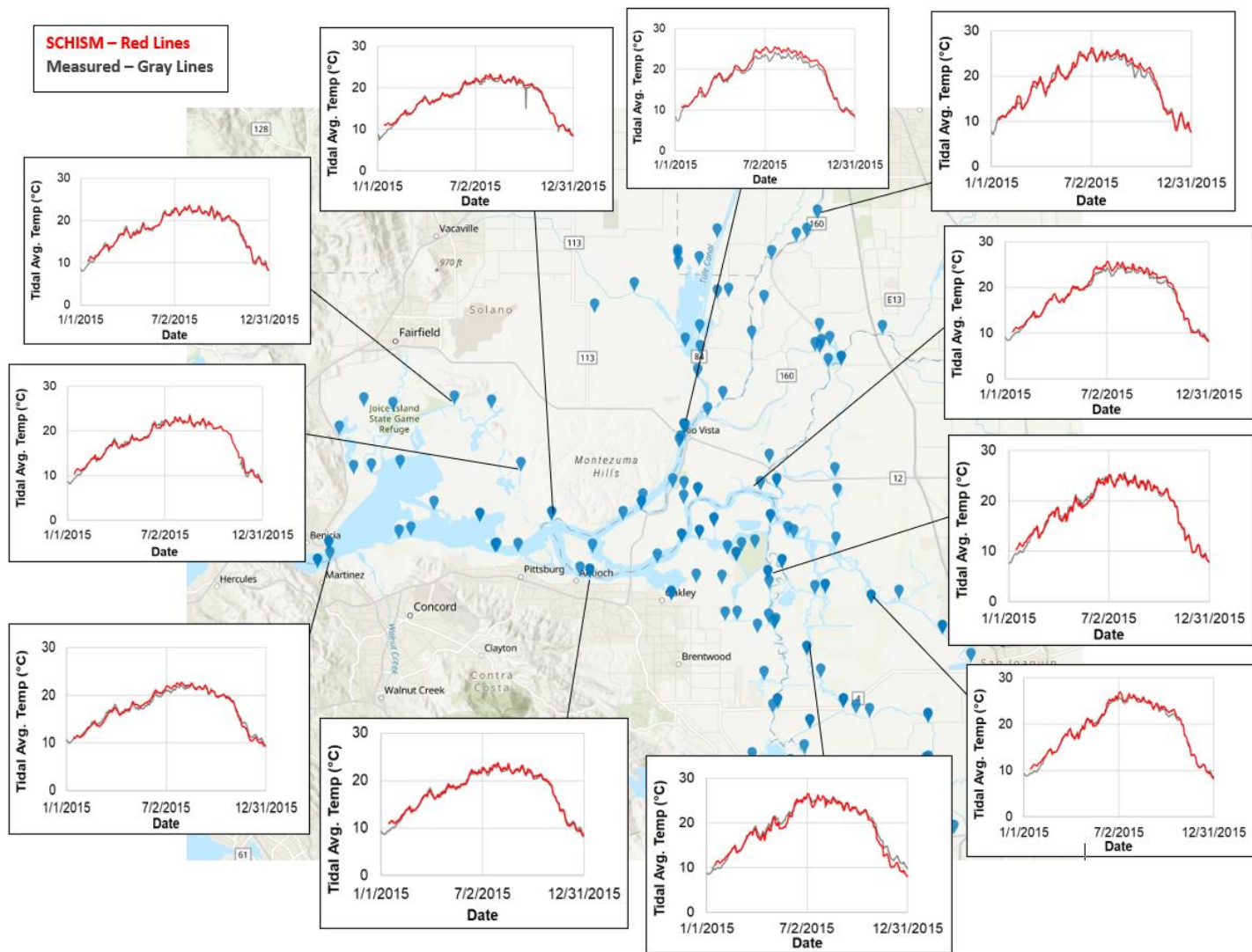
Figure K.1-11. Visual comparison between tidally-averaged measured stream temperature and tidally-averaged SCHISM-predicted stream temperatures at select monitoring stations across the model domain for 2015.
