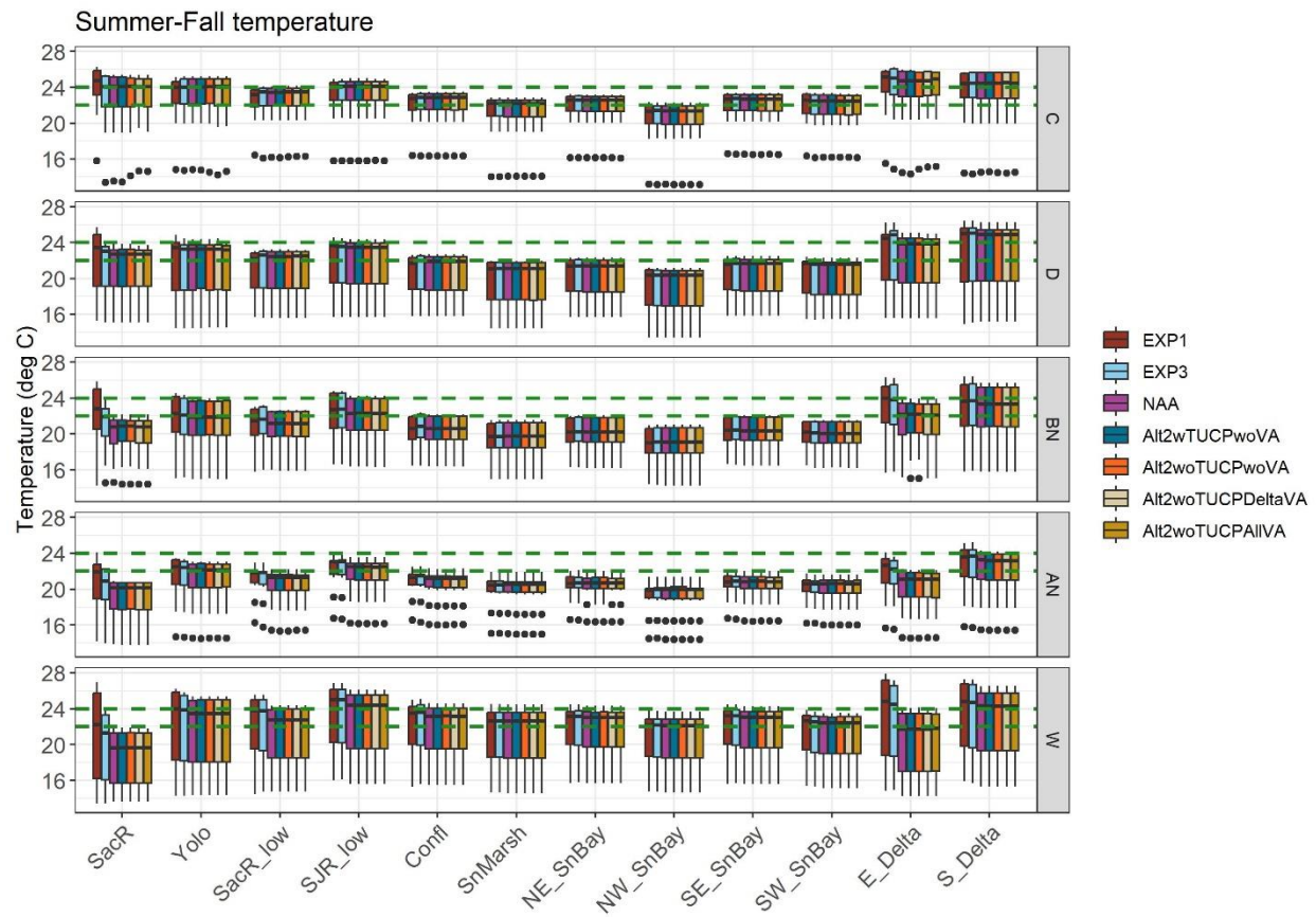
Figure K.1-15. Delta subregion temperatures (degrees Celsius [°C]) from July 1 – November 18 for each alternative and water year. The median is shown as the horizontal line, the box indicates the 25th and 75th percentiles, the vertical lines indicate the 25th and 75th percentiles plus 1.5 times the interquartile range, and the dots indicate potential outliers. The alternatives, from left to right are: exploratory 1 (EXP1); exploratory 3 (EXP3); no action alternative (NAA); alternative 2 with temporary urgency change, without Voluntary Agreements (Alt2wTUCPwoVA); alternative 2 without temporary urgency change, without Voluntary Agreements (Alt2wTUCPwoVA); alternative 2 without temporary urgency change, with Delta Voluntary Agreements (Alt2wTUCPDeltaVA); alternative 2 without temporary urgency change, with all Voluntary Agreements (Alt2wTUCPAIIVA). Water year types presented from top to bottom panels are: critical (C); dry (D); below normal (BN); above normal (AN); wet (W). The green dashed lines indicate the 22 C and 24 C temperature thresholds that have been used to modify the Bever et al. (2016) Delta Smelt habitat suitability index.
