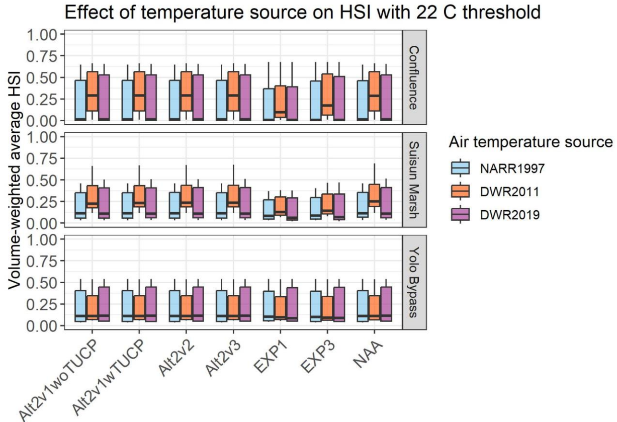
Figure K.1-90. Bever et al. (2016) modified by a 22-degree Celsius threshold from July 1 – November 18 using the NARR 1997, DWR 2011, and DWR 2019 air inputs for each alternative for the 1997 wet water year. The median is shown as the horizontal line, the box indicates the 25th and 75th percentiles, the vertical lines indicate the 25th and 75th percentiles plus 1.5 times the interquartile range, and the dots indicate potential outliers.
