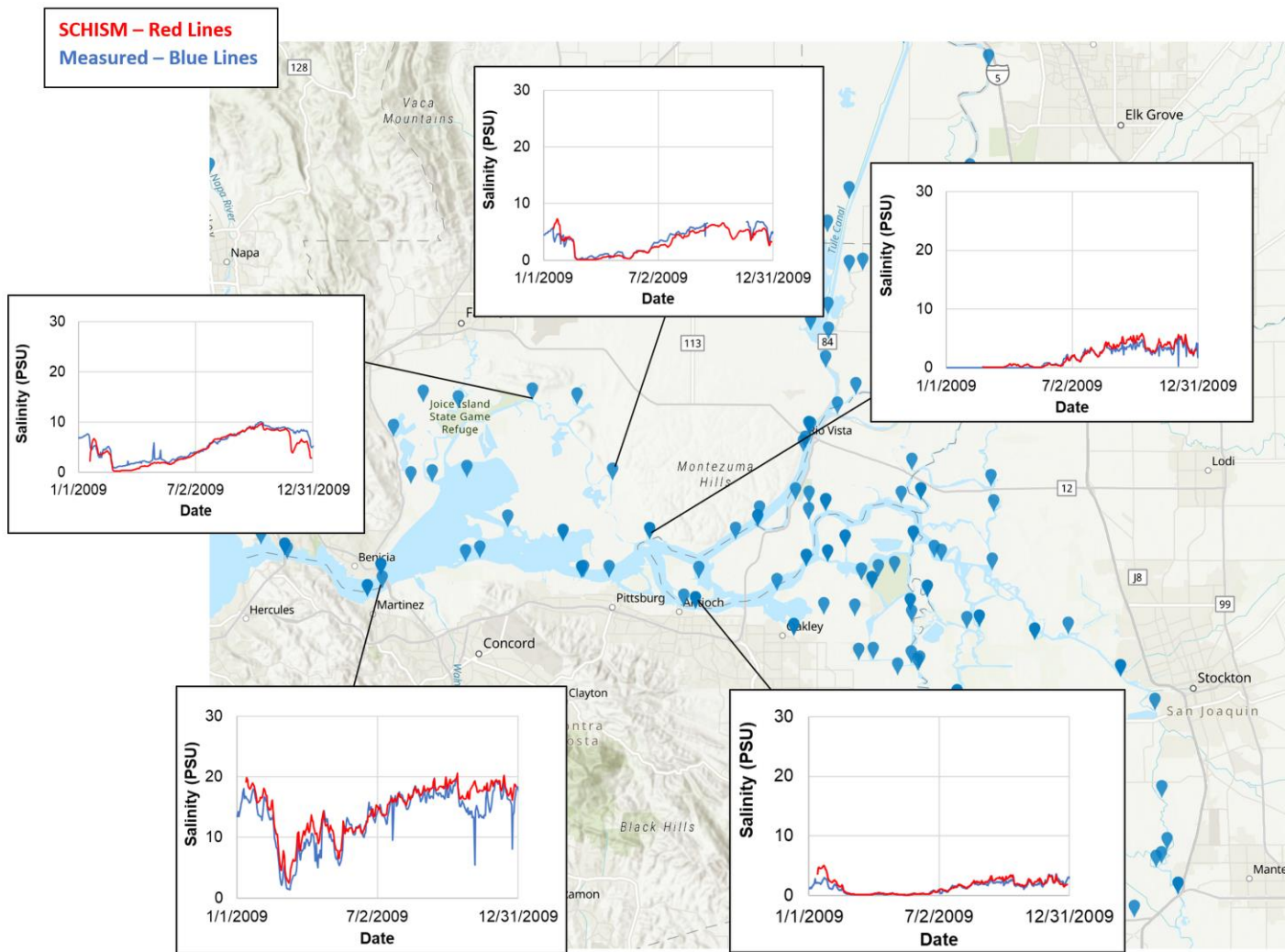
Figure K.1-12. Visual comparison between tidally-averaged measured and SCHISM-predicted stream salinities at select monitoring stations across the model domain for 2009.
