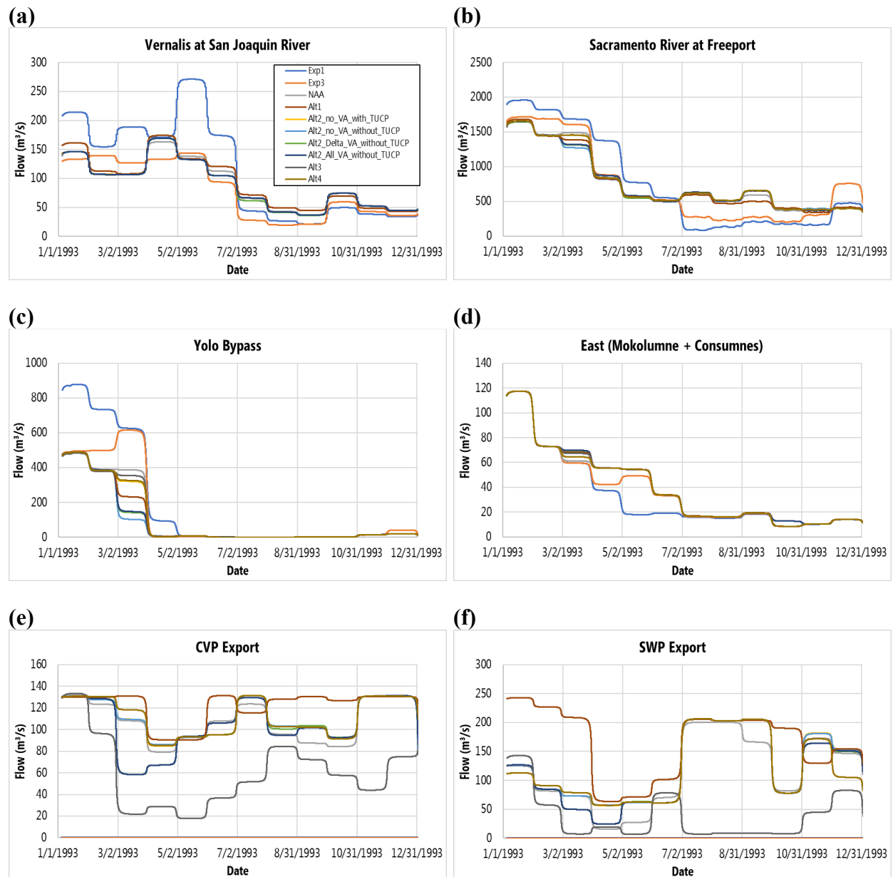
Figure K.1-2. Summary of major inflow and export boundary conditions for AN year (1993) for all alternatives at (a) Vernalis at San Joaquin River (inflow); (b) Sacramento River at Freeport (inflow); (c) Yolo Bypass (inflow); (d) Mokolumne and Consumnes (inflow); (e) CVP (export), and; (f) SWP (export)
