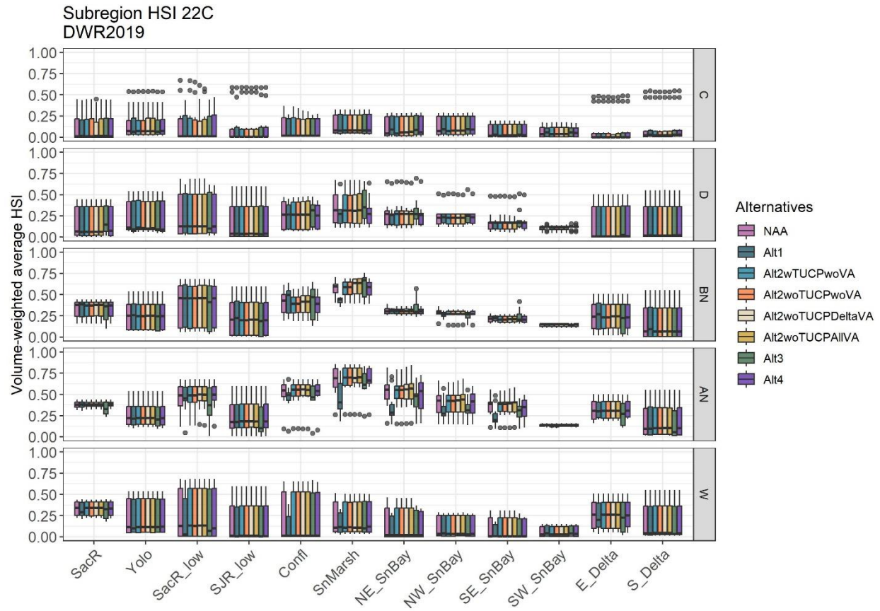
Figure K.1-34. Bever et al. (2016) habitat suitability indices modified by a 22-degree Celsius threshold for each alternative and water year type for July 1 – November 18. The median is shown as the horizontal line, the box indicates the 25th and 75th percentiles, the vertical lines indicate the 25th and 75th percentiles plus 1.5 times the interquartile range, and the dots indicate potential outliers. The alternatives, from left to right are: no action alternative (NAA); alternative 1 (Alt1); alternative 2 with temporary urgency change, without Voluntary Agreements (Alt2wTUCPwoVA); alternative 2 without temporary urgency change, without Voluntary Agreements (Alt2woTUCPwoVA); alternative 2 without temporary urgency change, with Delta Voluntary Agreements (Alt2woTUCPDeltaVA); alternative 2 without temporary urgency change, with all Voluntary Agreements (Alt2woTUCPAIIVA); alternative 3 (Alt3); alternative 4 (Alt4). Water year types presented from top to bottom panels are: critical (C); dry (D); below normal (BN); above normal (AN); wet (W).
