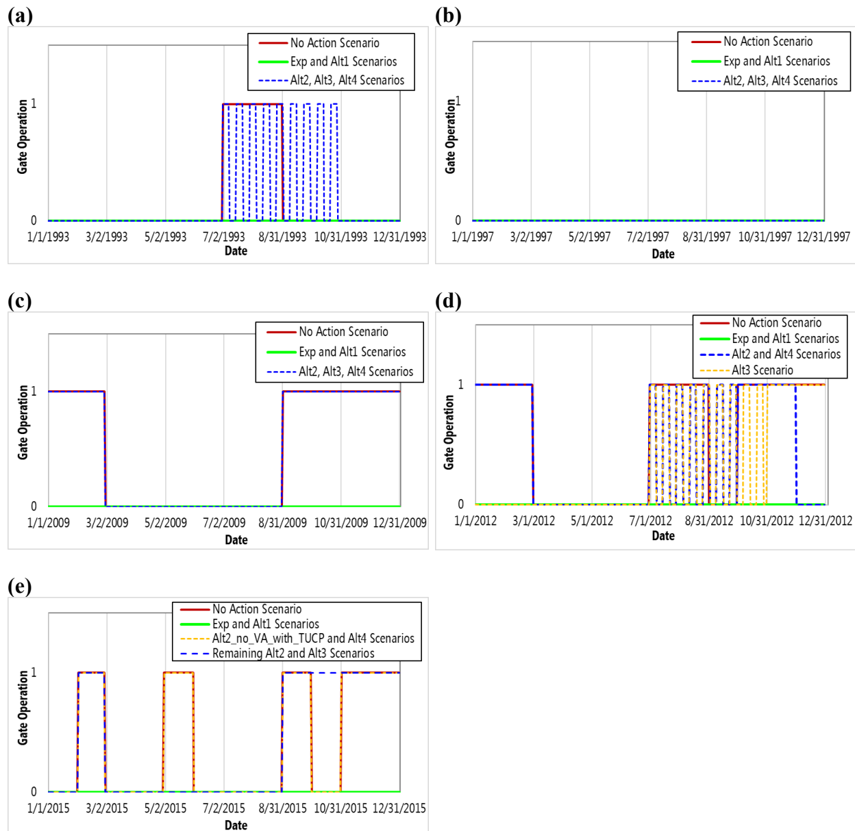
Figure K.1-8. Suisun Marsh Salinity Control Gate Operation: 1 indicates mode in which gates are being tidally operated and 0 is when the gates are fully open. Plots are shown for: (a) Above Normal – 1993; (b) Wet – 1997; (c) Dry – 2009; (d) Below Normal – 2012, and; (e) Critical water years – 2015.
