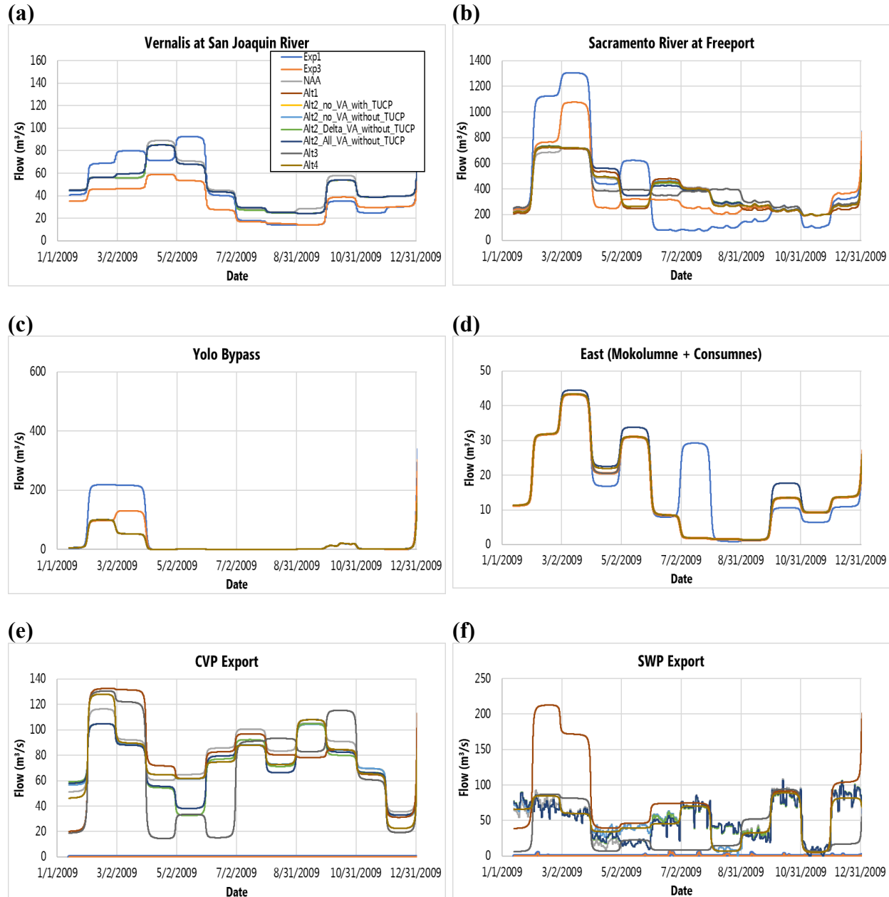
Figure K.1-4. Summary of major inflow and export boundary conditions for D year (2009) for all alternatives at (a) Vernalis at San Joaquin River (inflow); (b) Sacramento River at Freeport (inflow); (c) Yolo Bypass (inflow); (d) Mokolumne and Consumnes (inflow); (e) CVP (export), and; (f) SWP (export)
