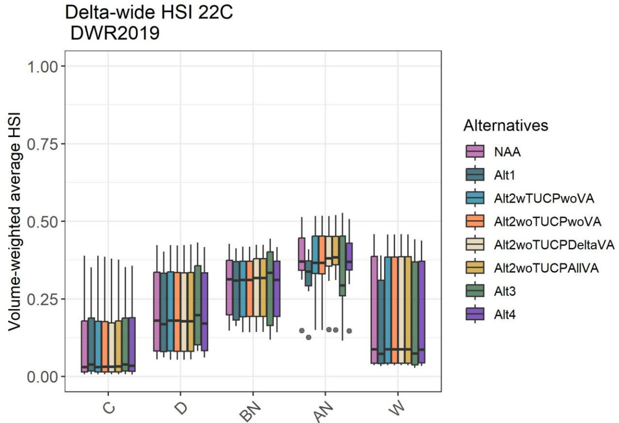
Figure K.1-26. Bever et al. (2016) Delta-wide habitat suitability indices modified by a 22-degree Celsius threshold for each alternative and water year type for July 1 – November 18. The median is shown as the horizontal line, the box indicates the 25th and 75th percentiles, the vertical lines indicate the 25th and 75th percentiles plus 1.5 times the interquartile range, and the dots indicate potential outliers. Water year types presented from left to right are: critical (C); dry (D); below normal (BN); above normal (AN); wet (W). The alternatives, from left to right for each water year type are: no action alternative (NAA); alternative 1 (Alt1); alternative 2 with temporary urgency change, without Voluntary Agreements (Alt2wTUCPwoVA); alternative 2 without temporary urgency change, without Voluntary Agreements (Alt2woTUCPwoVA); alternative 2 without temporary urgency change, with Delta Voluntary Agreements (Alt2woTUCPDeltaVA); alternative 2 without temporary urgency change, with all Voluntary Agreements (Alt2woTUCPAIIVA); alternative 3 (Alt3); alternative 4 (Alt4).
