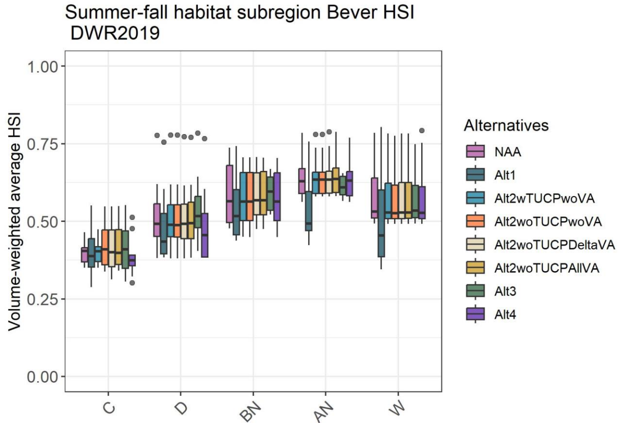
Figure K.1-28. Bever et al. (2016) habitat suitability indices in the summer and fall habitat arc for each alternative and water year type for July 1 – November 18. The arc includes subregions Confluence, Lower Sacramento River, northwest Suisun Bay, and Suisun Marsh. The median is shown as the horizontal line, the box indicates the 25th and 75th percentiles, the vertical lines indicate the 25th and 75th percentiles plus 1.5 times the interquartile range, and the dots indicate potential outliers. Water year types presented from left to right are: critical (C); dry (D); below normal (BN); above normal (AN); wet (W). The alternatives, from left to right for each water year type are: no action alternative (NAA); alternative 1 (Alt1); alternative 2 with temporary urgency change, without Voluntary Agreements (Alt2wTUCPwoVA); alternative 2 without temporary urgency change, without Voluntary Agreements (Alt2woTUCPwoVA); alternative 2 without temporary urgency change, with Delta Voluntary Agreements (Alt2woTUCPDeltaVA); alternative 2 without temporary urgency change, with all Voluntary Agreements (Alt2woTUCPAIIVA); alternative 3 (Alt3); alternative 4 (Alt4).
