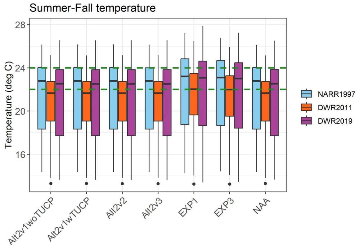
Figure K.1-89. Water temperatures (degrees Celsius [°C]) from July 1 – November 18 using the NARR 1997, DWR 2011, and DWR 2019 air inputs for each alternative for the 1997 wet water year. The median is shown as the horizontal line, the box indicates the 25th and 75th percentiles, the vertical lines indicate the 25th and 75th percentiles plus 1.5 times the interquartile range, and the dots indicate potential outliers.
