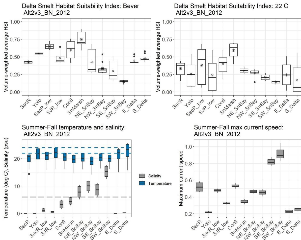
Figure K.1-62. Top left graph: Bever et al. (2016) habitat suitability indices for each subregion. Top right graph: Bever et al. (2016) habitat suitability indices and indices modified by a 22-degree Celsius threshold for each subregion. Lower left graph: temperature (in blue) and salinity (in gray) for each subregion; the dashed gray line indicates the 6 ppt salinity threshold; the dashed blue lines indicate the 22° and 24° C temperature thresholds. Lower right graph: maximum current speed for each subregion. In all graphs, data for the July 1 – November 18 in the below normal water year (2012) are shown for alternative 2 without temporary urgency change, with all Voluntary Agreements (Alt2v3). The median is shown as the horizontal line, the mean is shown with an asterisk (HSI graphs only), the box indicates the 25th and 75th percentiles, the vertical lines indicate the 25th and 75th percentiles plus 1.5 times the interquartile range, and the dots indicate potential outliers.
