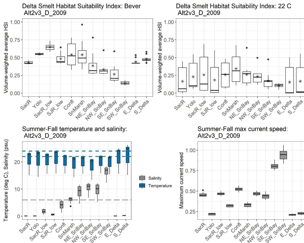
Figure K.1-72. Top left graph: Bever et al. (2016) habitat suitability indices for each subregion. Top right graph: Bever et al. (2016) habitat suitability indices and indices modified by a 22-degree Celsius threshold for each subregion. Lower left graph: temperature (in blue) and salinity (in gray) for each subregion; the dashed gray line indicates the 6 ppt salinity threshold; the dashed blue lines indicate the 22° and 24° C temperature thresholds. Lower right graph: maximum current speed for each subregion. In all graphs, data for the July 1 – November 18 in the dry water year (2009) are shown for alternative 2 without temporary urgency change, with all Voluntary Agreements (Alt2v3). The median is shown as the horizontal line, the mean is shown with an asterisk (HSI graphs only), the box indicates the 25th and 75th percentiles, the vertical lines indicate the 25th and 75th percentiles plus 1.5 times the interquartile range, and the dots indicate potential outliers.
