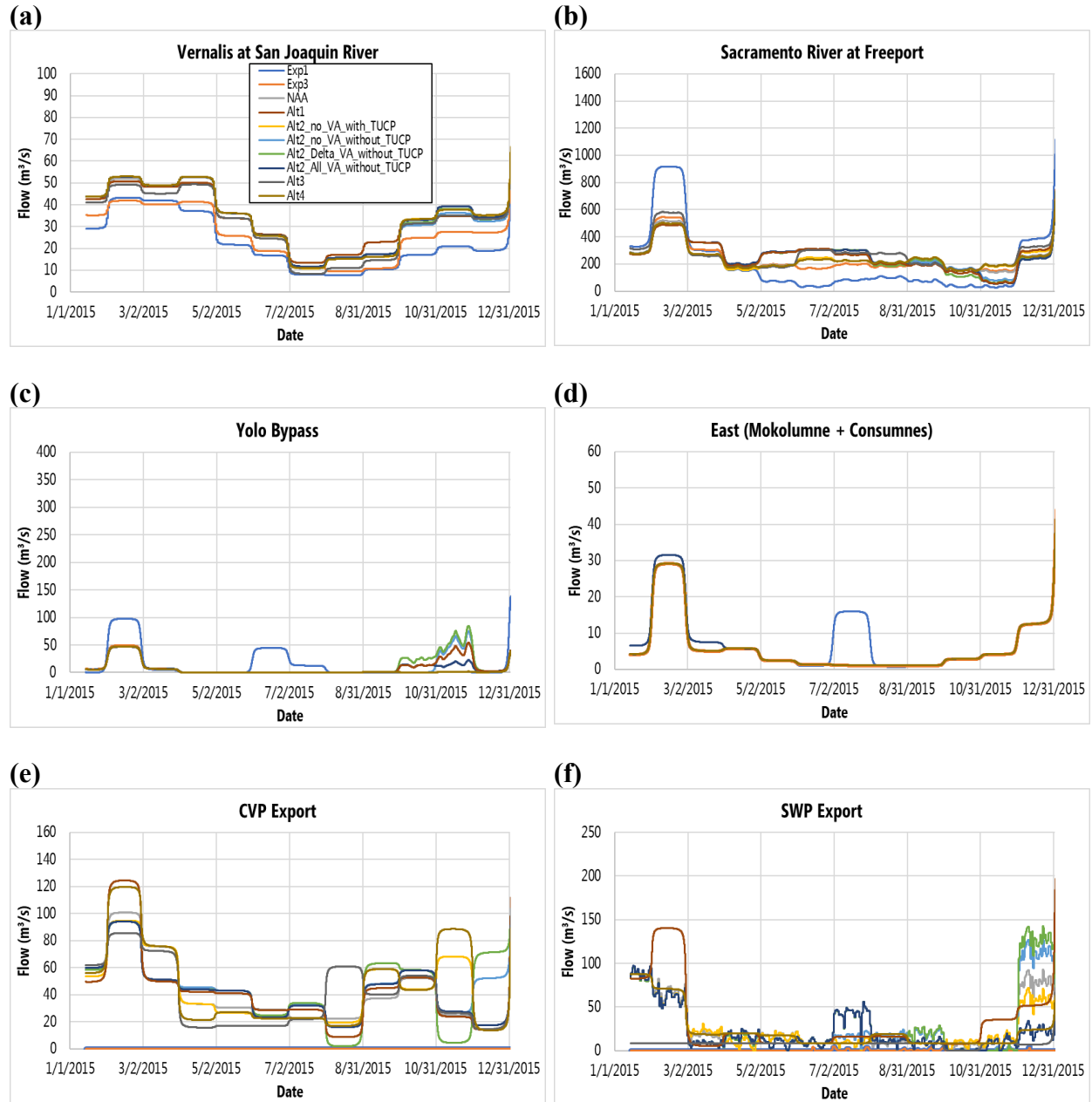
Figure K.1-6. Summary of major inflow and export boundary conditions for C year (2015) for all alternatives at (a) Vernalis at San Joaquin River (inflow); (b) Sacramento River at Freeport (inflow); (c) Yolo Bypass (inflow); (d) Mokolumne and Consumnes (inflow); (e) CVP (export), and; (f) SWP (export)
