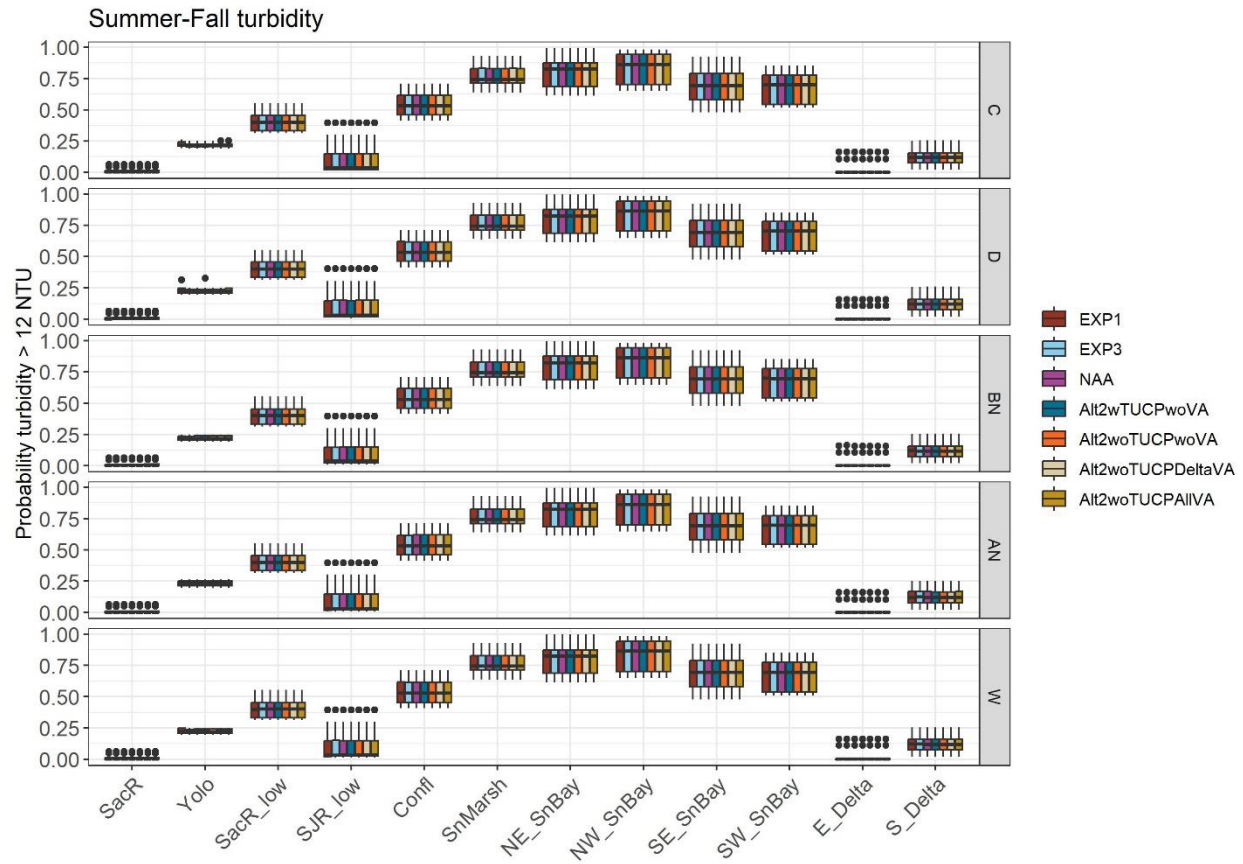
Figure K.1-21. Delta subregion probability of turbidity greater than 12 Nephelometric Units (NTU) from July 1 – November 18. The threshold of 12 NTU is from the Bever et al. (2016) Delta Smelt habitat suitability index. The median is shown as the horizontal line, the box indicates the 25th and 75th percentiles, the vertical lines indicate the 25th and 75th percentiles plus 1.5 times the interquartile range, and the dots indicate potential outliers. The alternatives, from left to right are: exploratory 1 (EXP1); exploratory 3 (EXP3); no action alternative (NAA); alternative 2 with temporary urgency change, without Voluntary Agreements (Alt2wTUCPwoVA); alternative 2 without temporary urgency change, without Voluntary Agreements (Alt2woTUCPwoVA); alternative 2 without temporary urgency change, with Delta Voluntary Agreements (Alt2woTUCPDeltaVA); alternative 2 without temporary urgency change, with all Voluntary Agreements (Alt2woTUCPAIIVA). Water year types presented from top to bottom panels are: critical (C); dry (D); below normal (BN); above normal (AN); wet (W).
