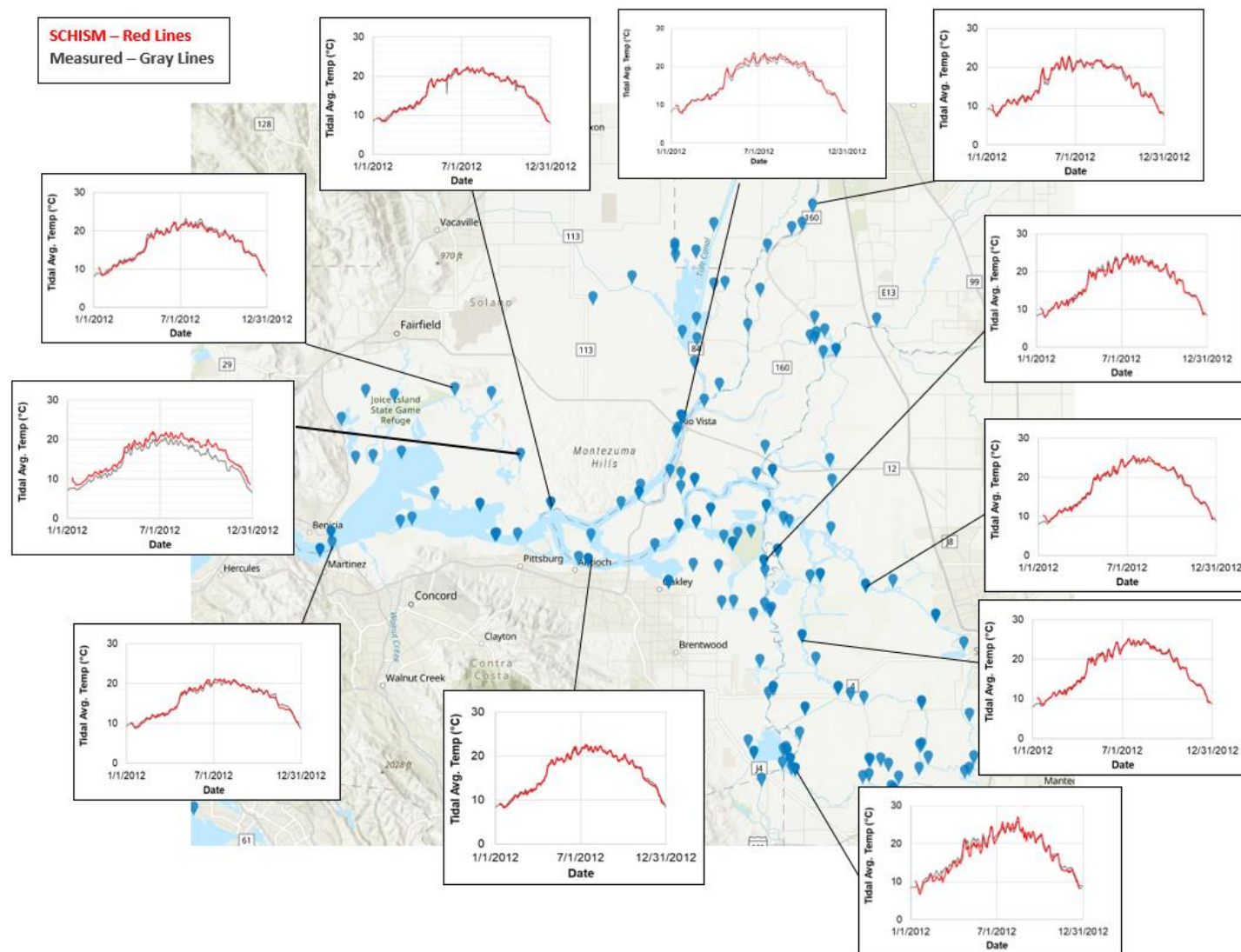
Figure K.1-9. Visual comparison between tidally-averaged measured stream temperatures and tidally-averaged SCHISM-predicted stream temperatures at select monitoring stations across the model domain for 2012.
