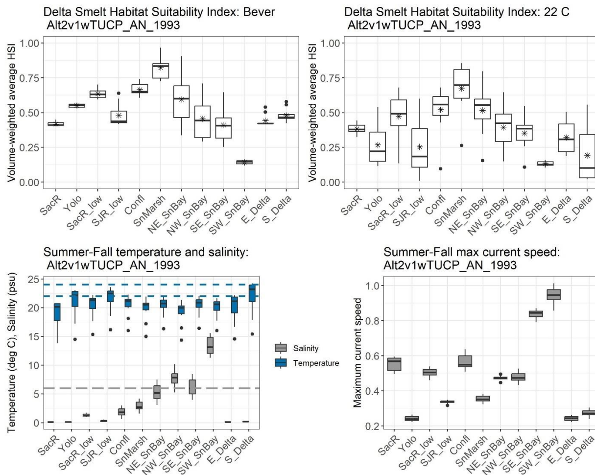
Figure K.1-49. Top left graph: Bever et al. (2016) habitat suitability indices for each subregion. Top right graph: Bever et al. (2016) habitat suitability indices and indices modified by a 22-degree Celsius threshold for each subregion. Lower left graph: temperature (in blue) and salinity (in gray) for each subregion; the dashed gray line indicates the 6 ppt salinity threshold; the dashed blue lines indicate the 22° and 24° C temperature thresholds. Lower right graph: maximum current speed for each subregion. In all graphs, data for the July 1 – November 18 in the above normal water year (1993) are shown for alternative 2 with temporary urgency change, without Voluntary Agreements (Alt2v1wTUCP), using DWR 2010 air inputs. The median is shown as the horizontal line, the mean is shown with an asterisk (HSI graphs only), the box indicates the 25th and 75th percentiles, the vertical lines indicate the 25th and 75th percentiles plus 1.5 times the interquartile range, and the dots indicate potential outliers.
