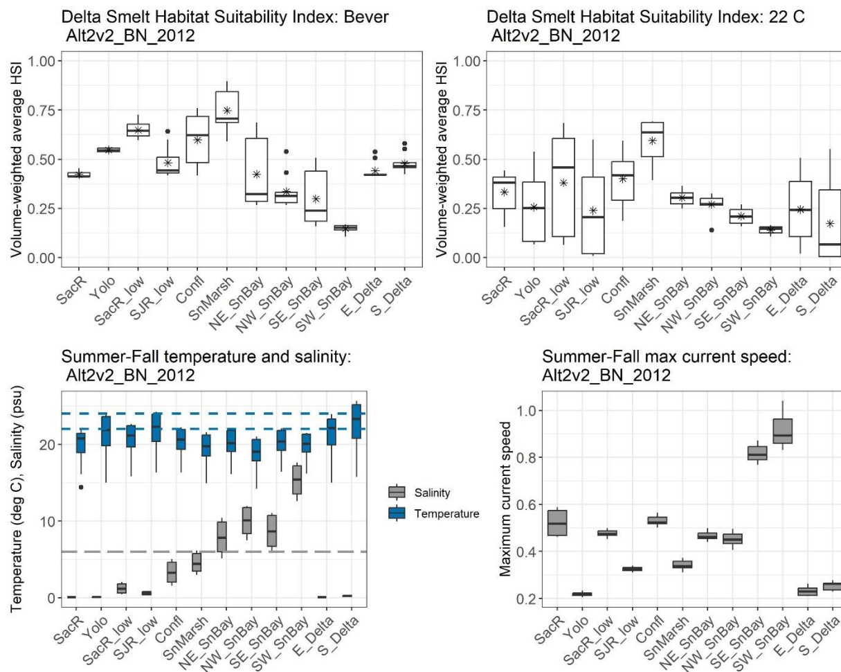
Figure K.1-61. Top left graph: Bever et al. (2016) habitat suitability indices for each subregion. Top right graph: Bever et al. (2016) habitat suitability indices and indices modified by a 22-degree Celsius threshold for each subregion. Lower left graph: temperature (in blue) and salinity (in gray) for each subregion; the dashed gray line indicates the 6 ppt salinity threshold; the dashed blue lines indicate the 22° and 24° C temperature thresholds. Lower right graph: maximum current speed for each subregion. In all graphs, data for the July 1 – November 18 in the below normal water year (2012) are shown for alternative 2 without temporary urgency change, with Delta Voluntary Agreements (Alt2v2). The median is shown as the horizontal line, the mean is shown with an asterisk (HSI graphs only), the box indicates the 25th and 75th percentiles, the vertical lines indicate the 25th and 75th percentiles plus 1.5 times the interquartile range, and the dots indicate potential outliers.
