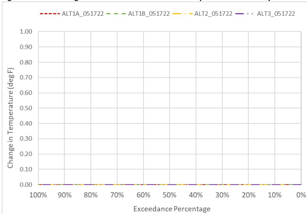
Figure 6D2-8-5. Changes to Sacramento River Water Temperature in February
