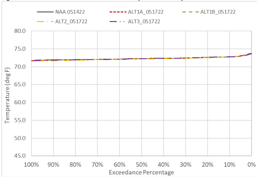
Figure 6D2-7-10. Sacramento River Water Temperature in July
