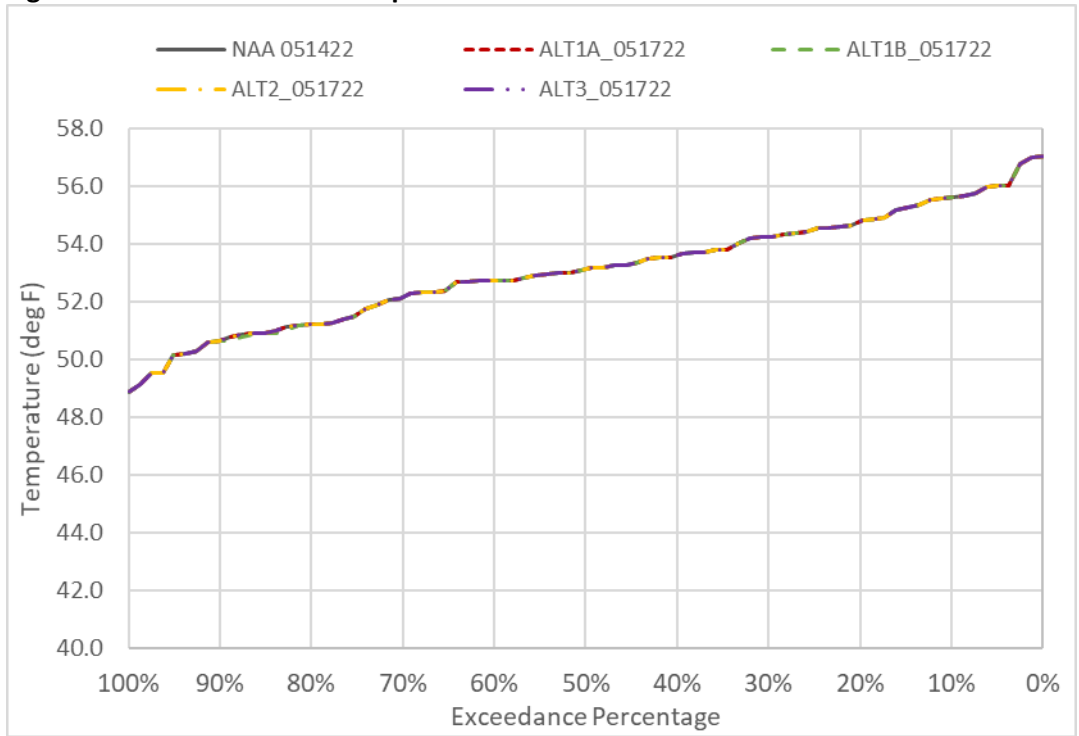
Figure 6D2-3-6. GCC Water Temperature in March
