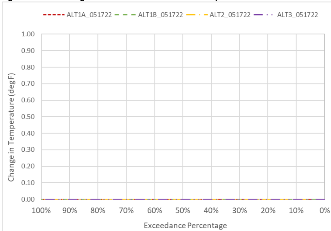
Figure 6D2-8-6. Changes to Sacramento River Water Temperature in March
