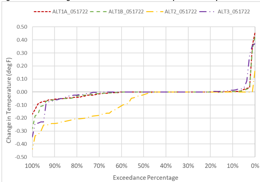
Figure 6D2-8-10. Changes to Sacramento River Water Temperature in July
