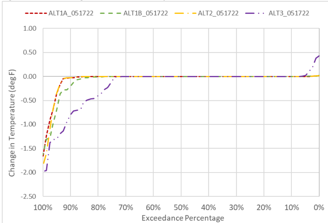
Figure 6D2-4-9. Changes to GCC Water Temperature in June
