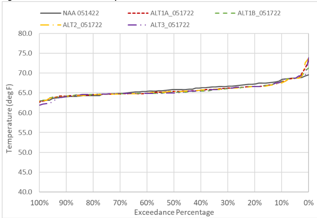
Figure 6D2-1-9. TCC Water Temperature in June
