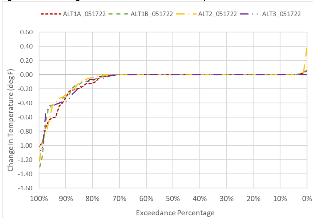
Figure 6D2-8-2. Changes to Sacramento River Water Temperature in November
