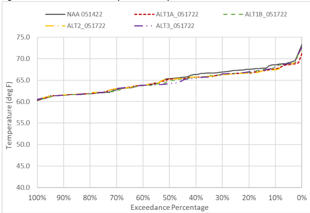
Figure 6D2-3-12. GCC Water Temperature in September
