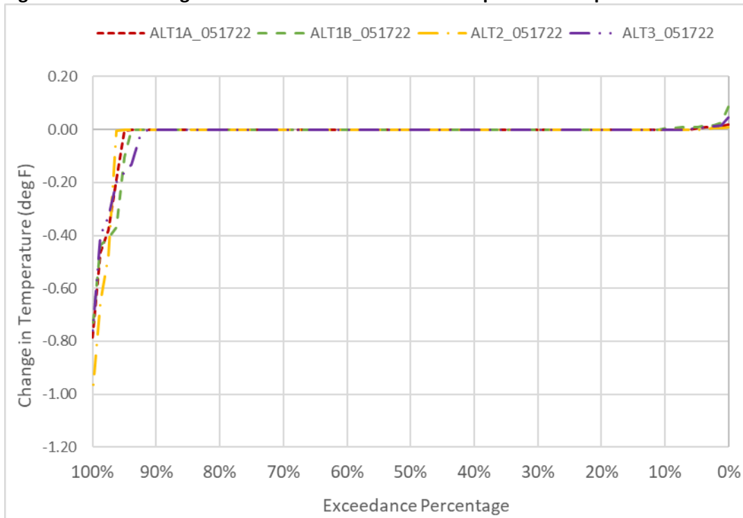
Figure 6D2-8-7. Changes to Sacramento River Water Temperature in April
