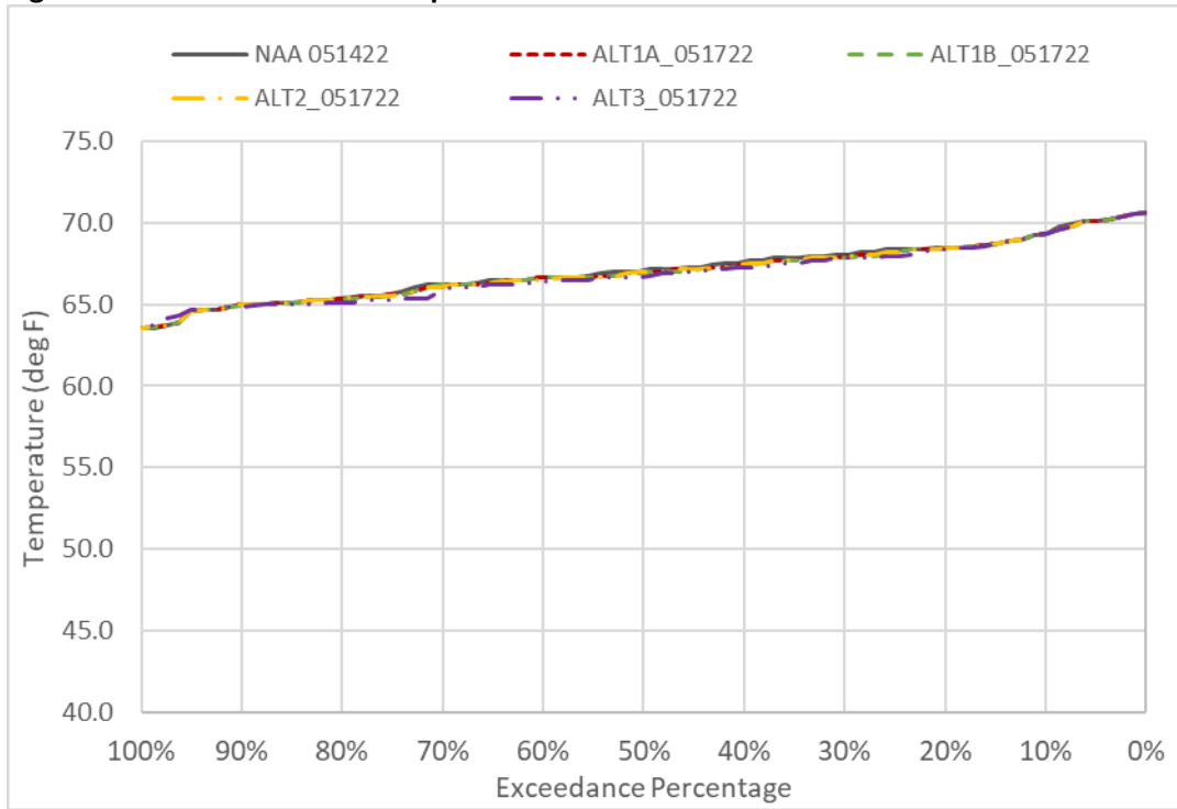
Figure 6D2-3-9. GCC Water Temperature in June
