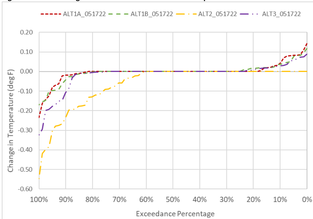
Figure 6D2-8-9. Changes to Sacramento River Water Temperature in June
