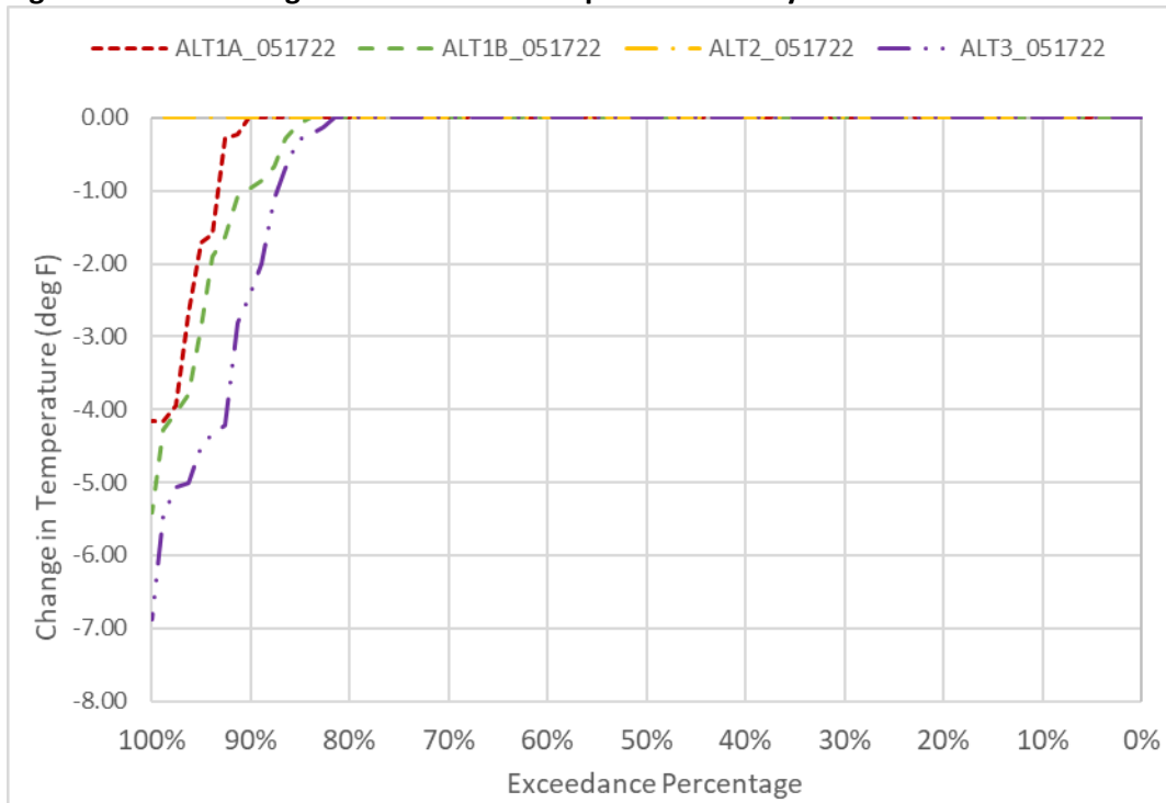
Figure 6D2-6-8. Changes to CBD Water Temperature in May
