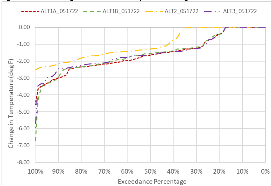
Figure 6D2-6-11. Changes to CBD Water Temperature in August
