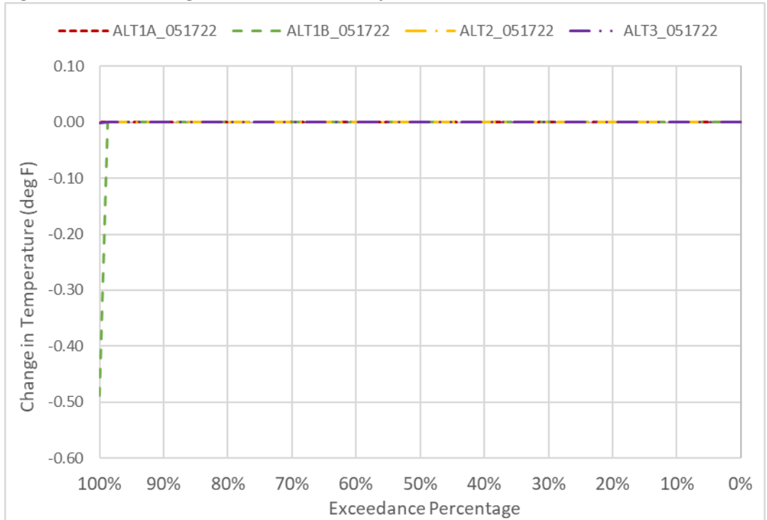
Figure 6D2-4-6. Changes to GCC Water Temperature in March
