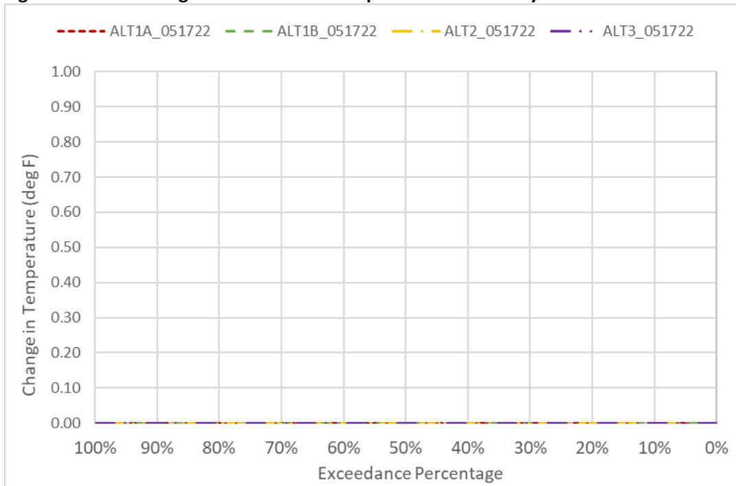
Figure 6D2-6-5. Changes to CBD Water Temperature in February
