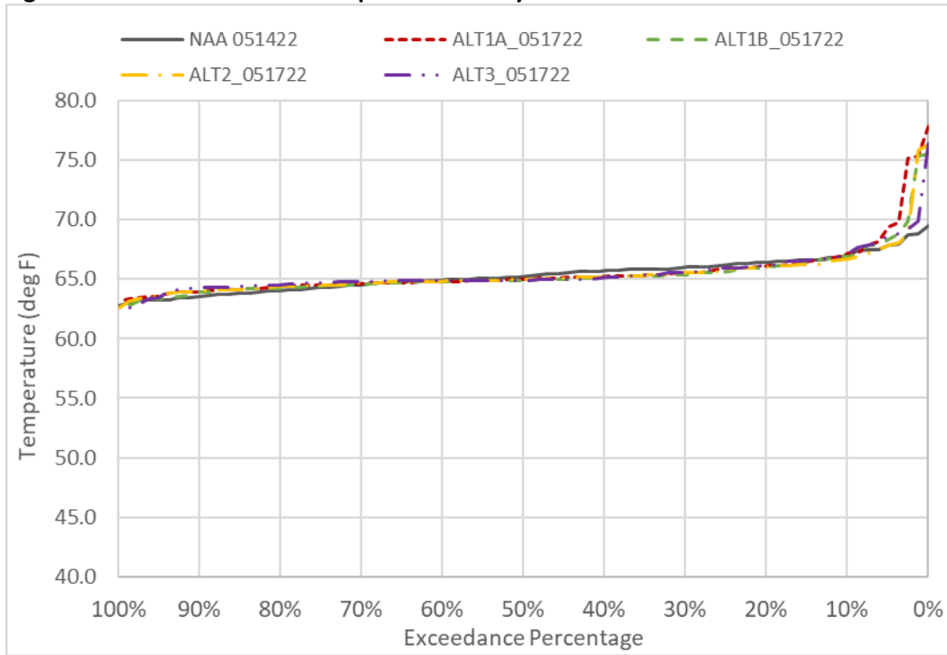
Figure 6D2-1-10. TCC Water Temperature in July
