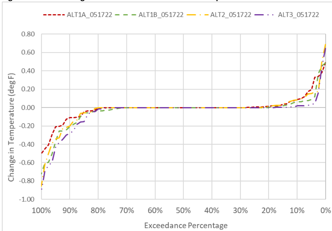
Figure 6D2-8-1. Changes to Sacramento River Water Temperature in October
