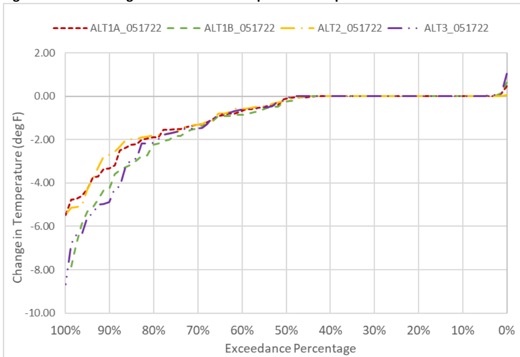
Figure 6D2-2-7. Changes to TCC Water Temperature in April
