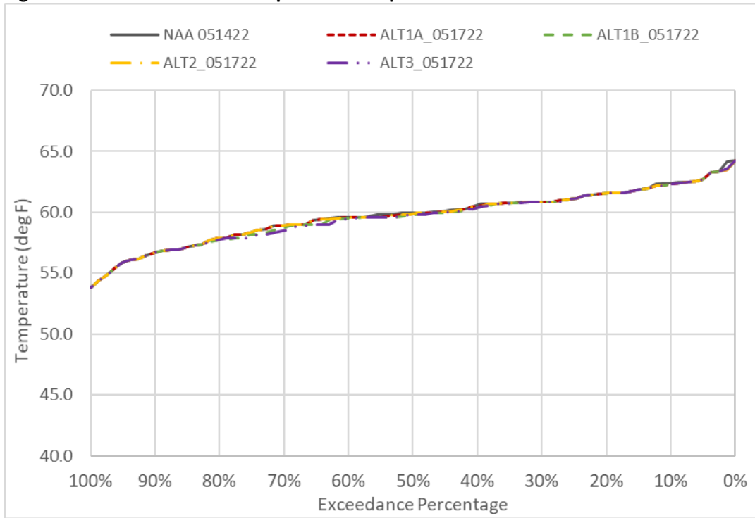
Figure 6D2-3-7. GCC Water Temperature in April
