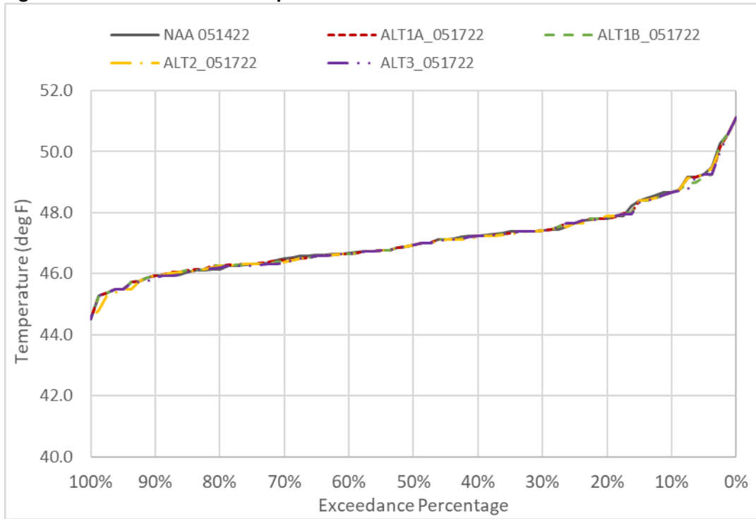
Figure 6D2-3-3. GCC Water Temperature in December
