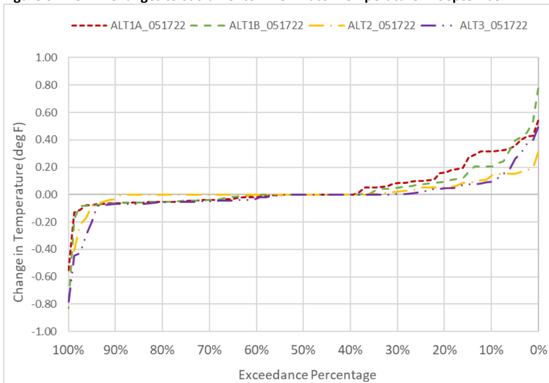
Figure 6D2-8-12. Changes to Sacramento River Water Temperature in September
