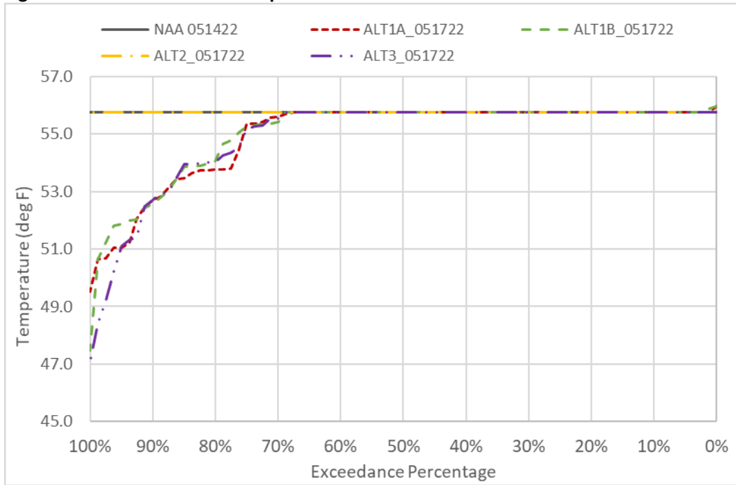
Figure 6D2-5-2. CBD Water Temperature in November
