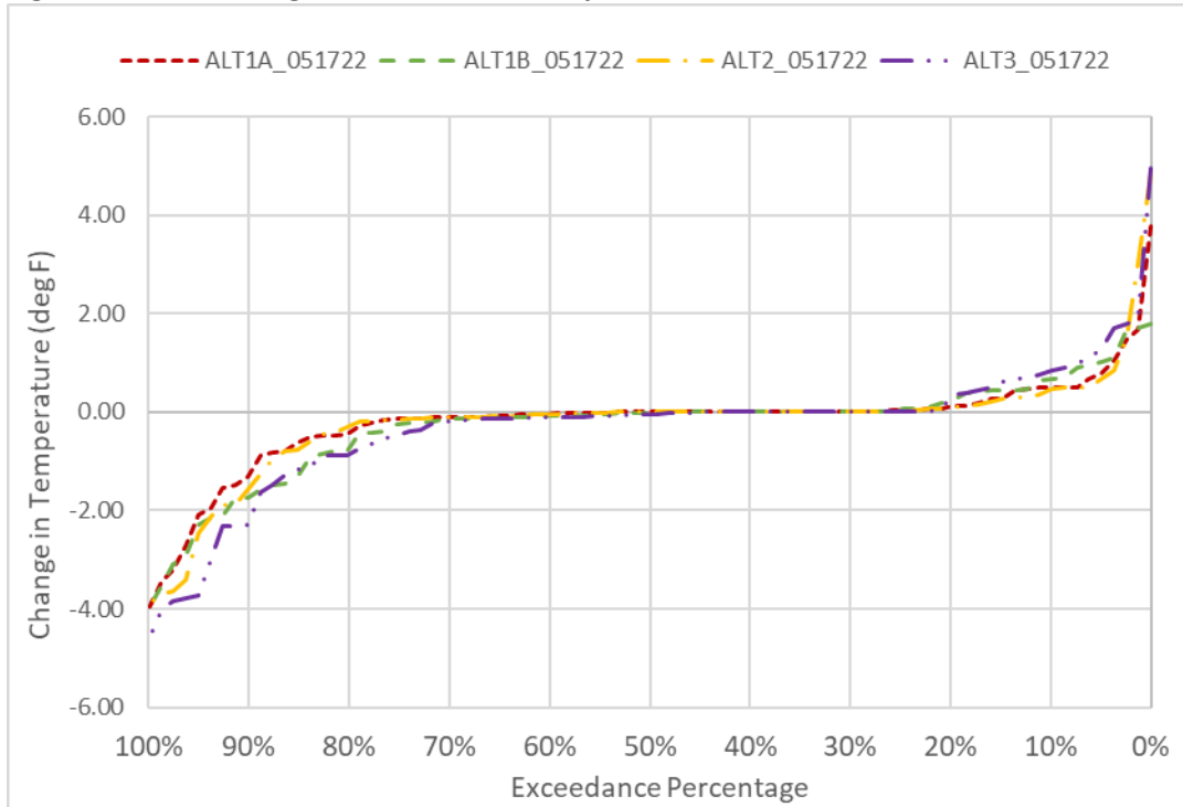
Figure 6D2-2-9. Changes to TCC Water Temperature in June
