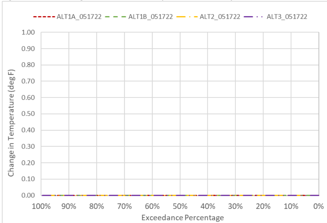
Figure 6D2-2-4. Changes to TCC Water Temperature in January
