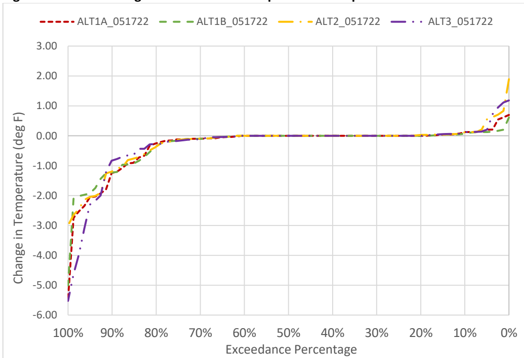
Figure 6D2-4-12. Changes to GCC Water Temperature in September
