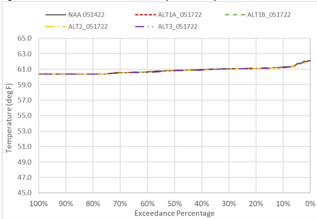
Figure 6D2-7-7. Sacramento River Water Temperature in April
