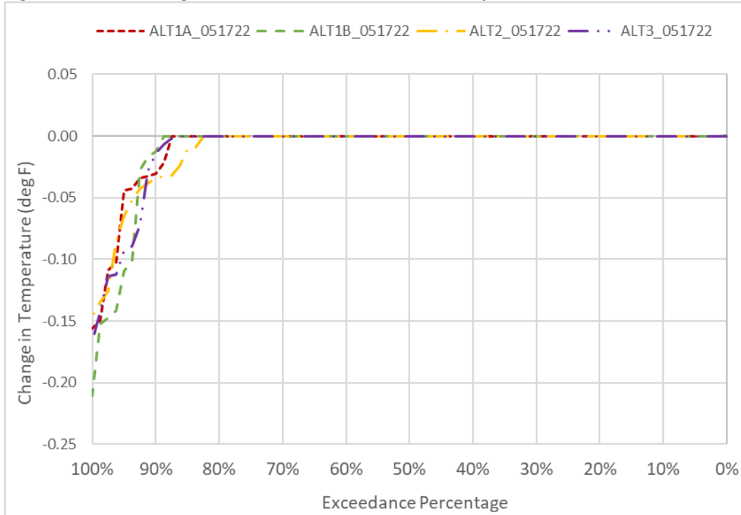
Figure 6D2-8-3. Changes to Sacramento River Water Temperature in December
