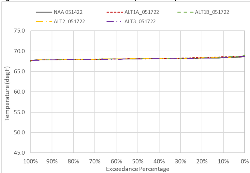
Figure 6D2-7-12. Sacramento River Water Temperature in September
