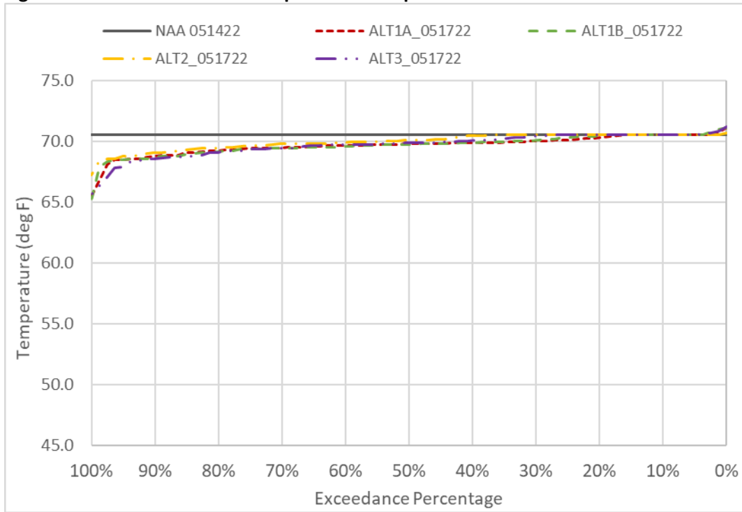
Figure 6D2-5-12. CBD Water Temperature in September
