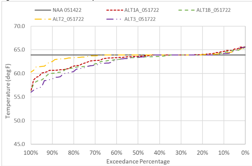
Figure 6D2-5-1. CBD Water Temperature in October
