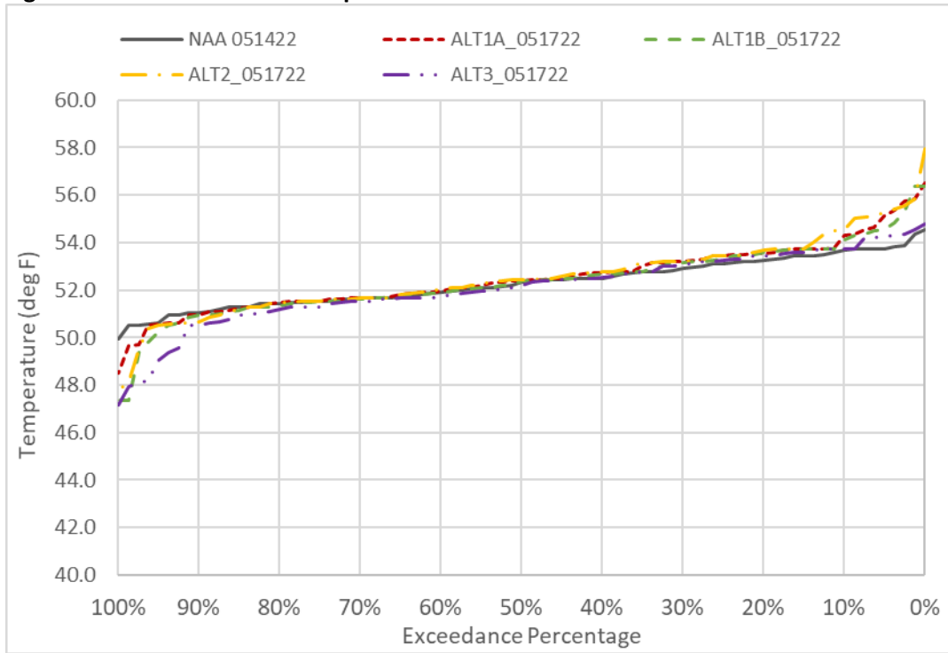
Figure 6D2-1-2. TCC Water Temperature in November
