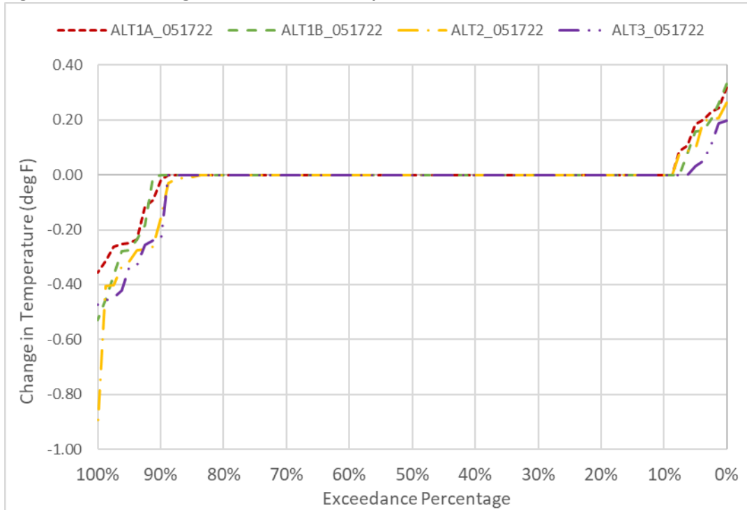
Figure 6D2-4-3. Changes to GCC Water Temperature in December
