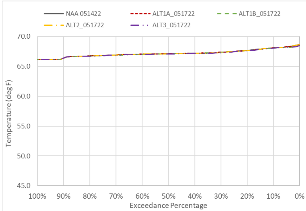
Figure 6D2-7-8. Sacramento River Water Temperature in May
