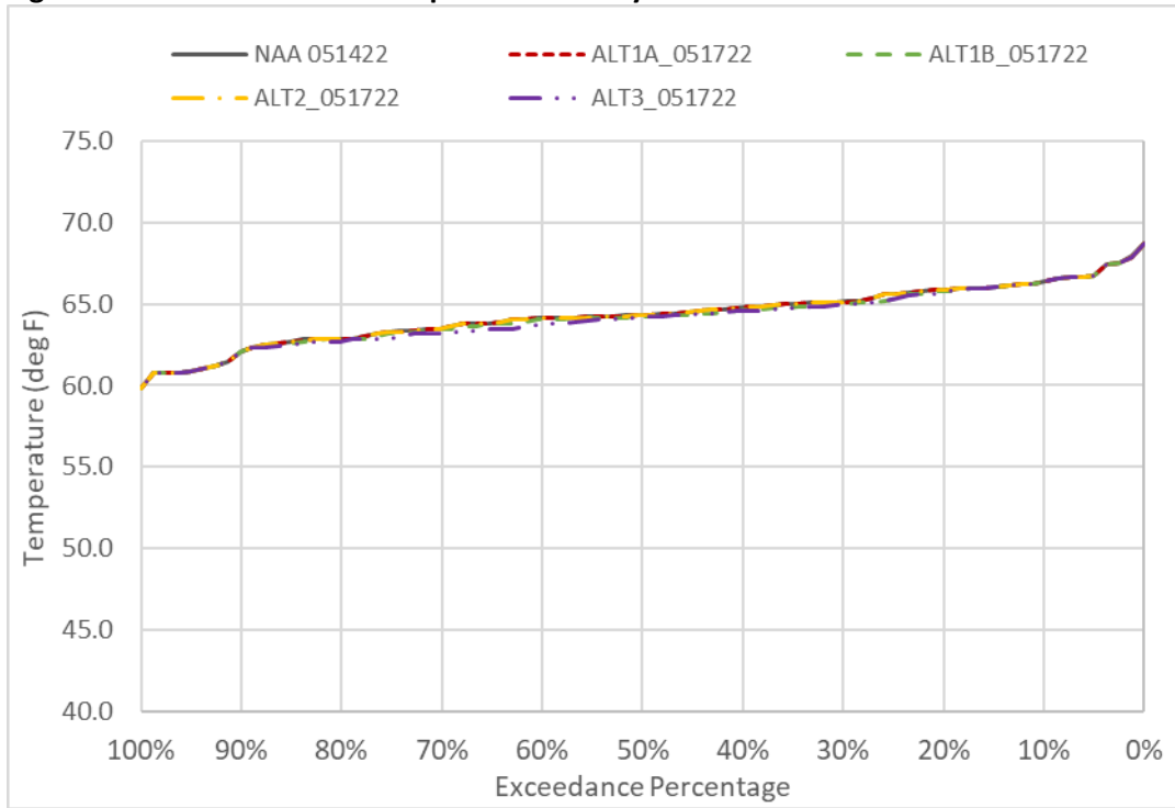
Figure 6D2-3-8. GCC Water Temperature in May
