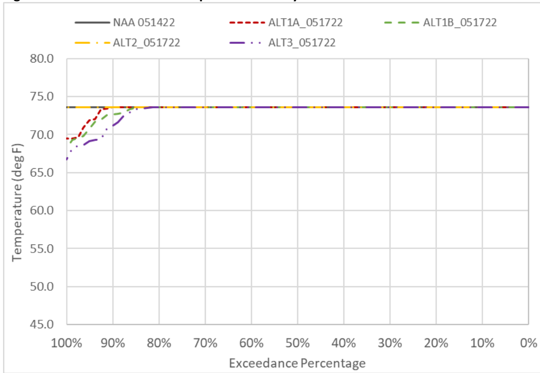
Figure 6D2-5-8. CBD Water Temperature in May
