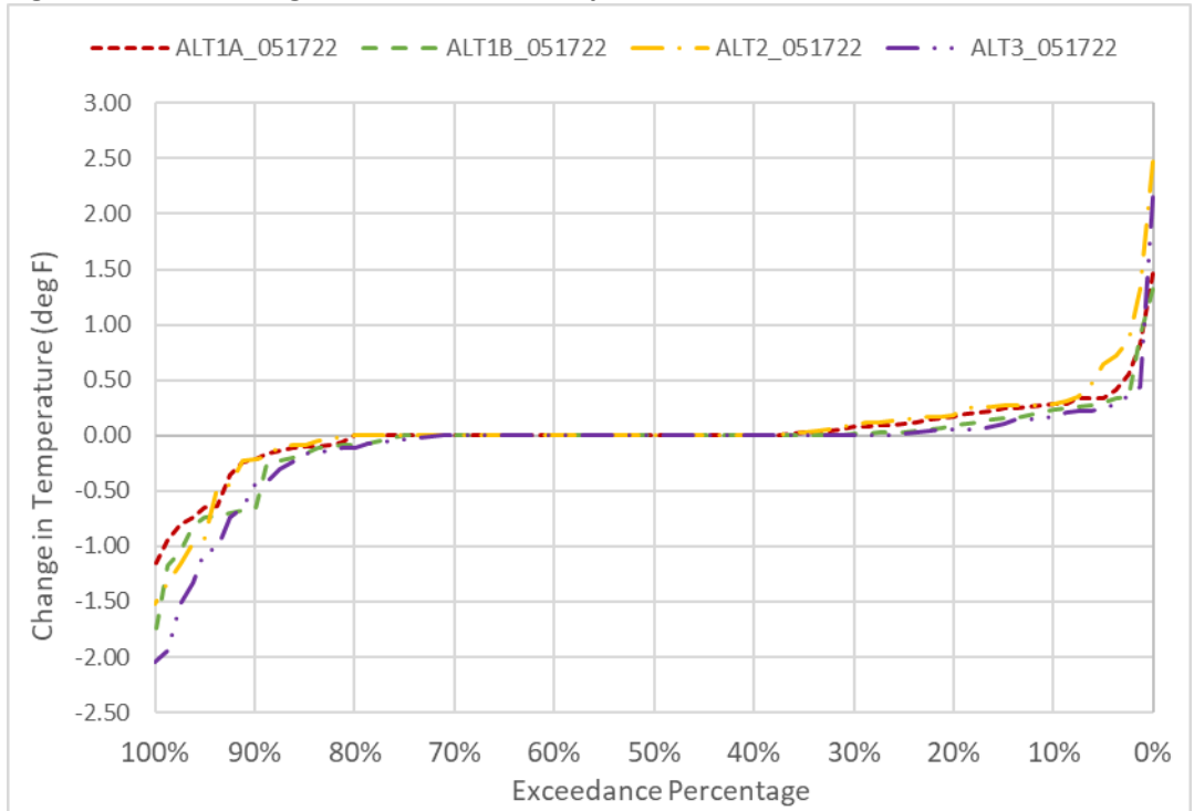
Figure 6D2-4-1. Changes to GCC Water Temperature in October
