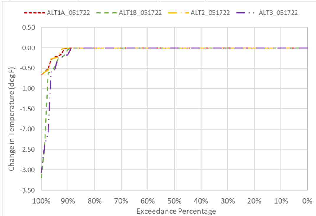
Figure 6D2-4-7. Changes to GCC Water Temperature in April
