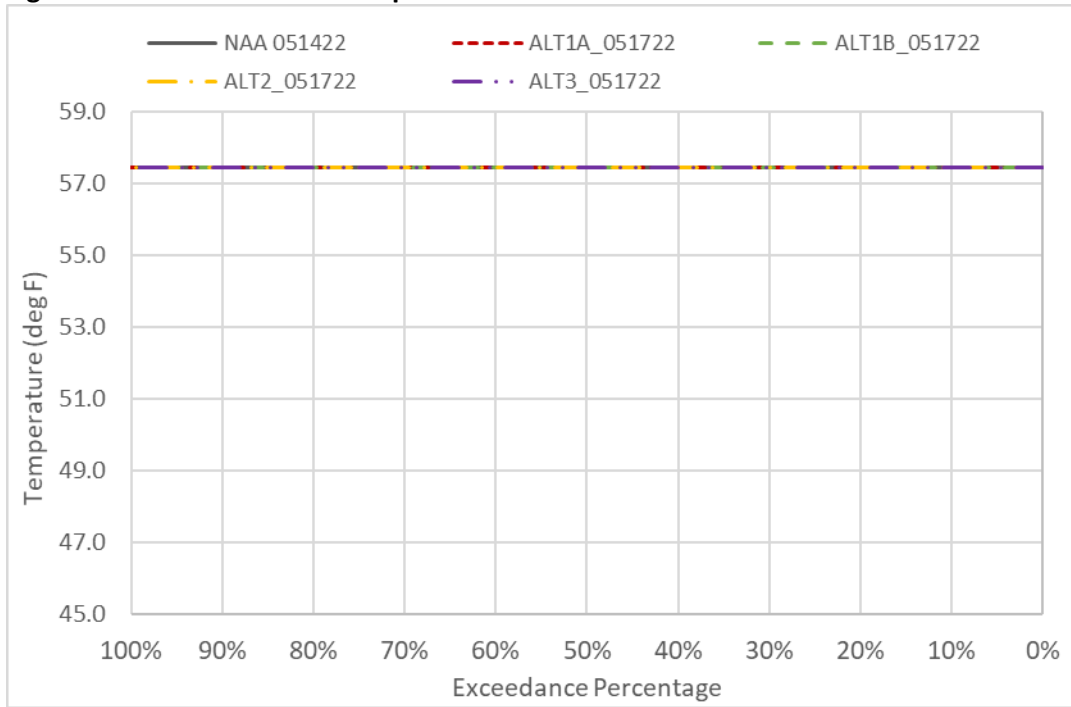
Figure 6D2-5-6. CBD Water Temperature in March
