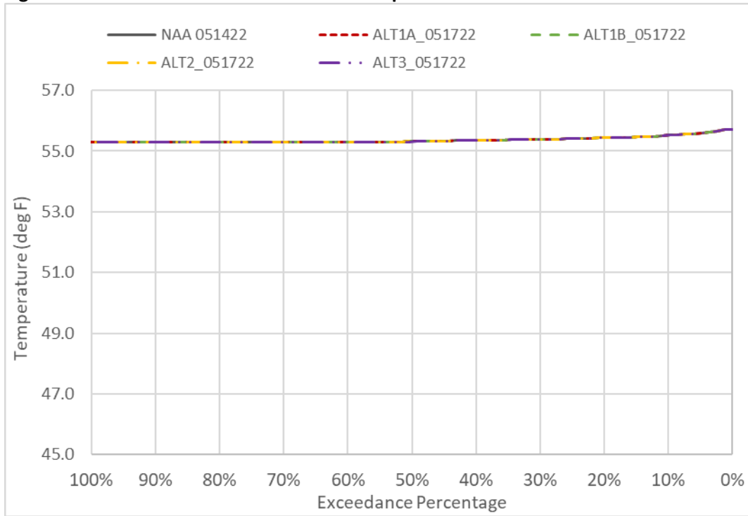
Figure 6D2-7-6. Sacramento River Water Temperature in March
