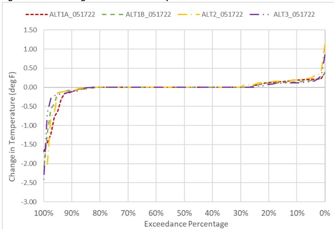
Figure 6D2-4-2. Changes to GCC Water Temperature in November
