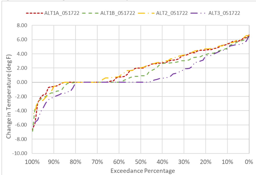
Figure 6D2-2-1. Changes to TCC Water Temperature in October
