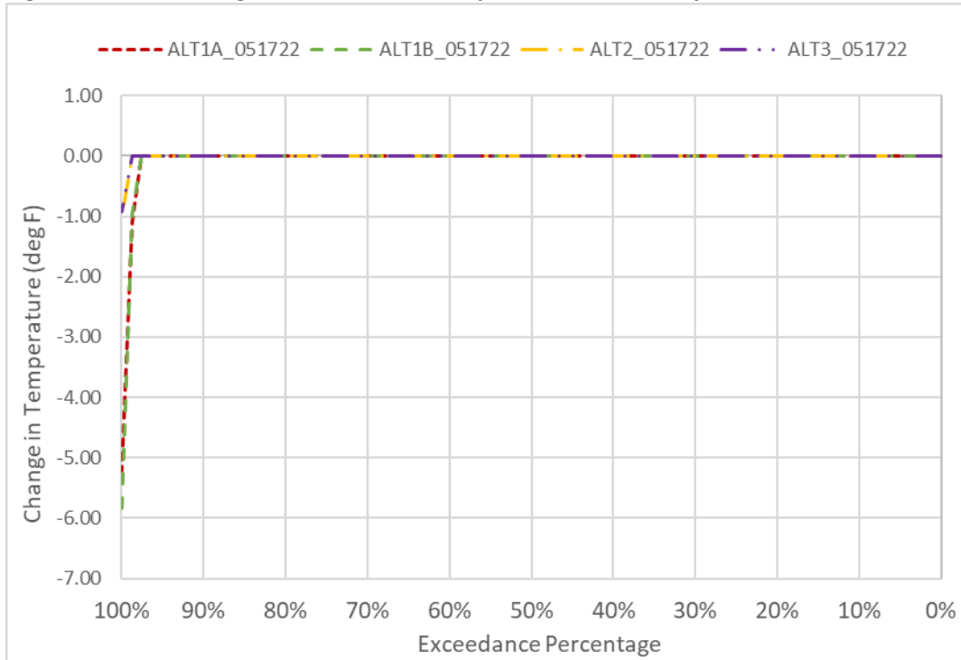
Figure 6D2-2-5. Changes to TCC Water Temperature in February
