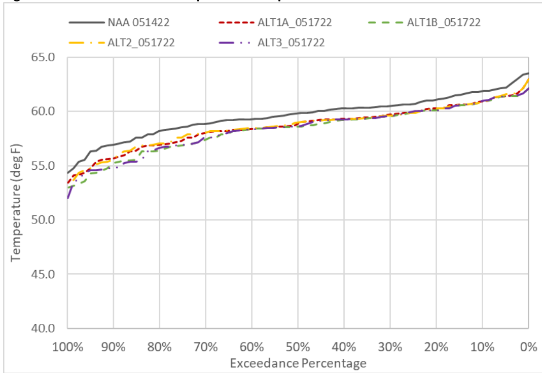
Figure 6D2-1-7. TCC Water Temperature in April
