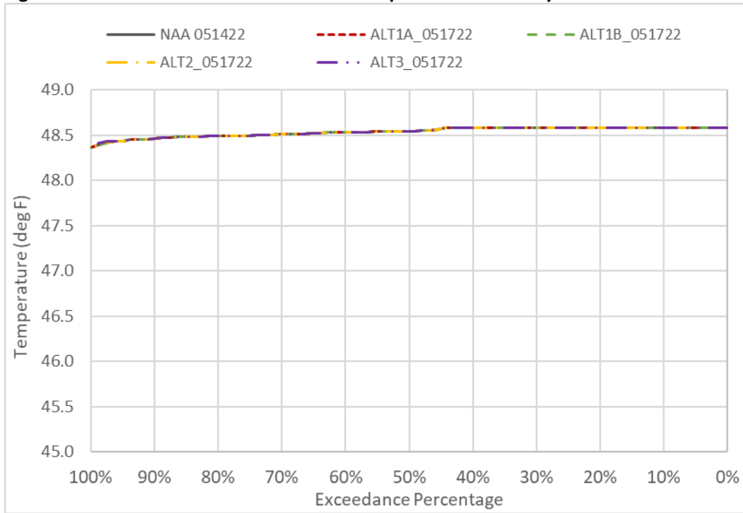
Figure 6D2-7-4. Sacramento River Water Temperature in January
