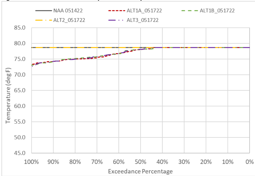
Figure 6D2-5-10. CBD Water Temperature in July
