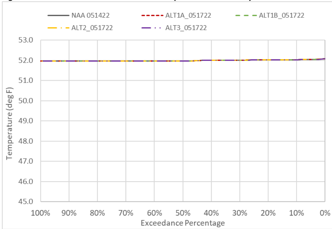
Figure 6D2-7-5. Sacramento River Water Temperature in February
