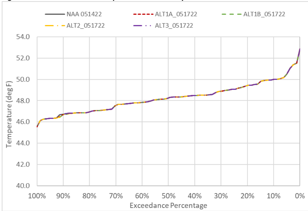
Figure 6D2-3-5. GCC Water Temperature in February
