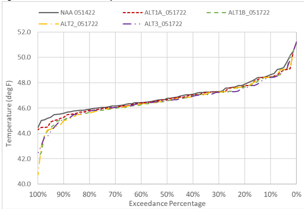
Figure 6D2-1-3. TCC Water Temperature in December
