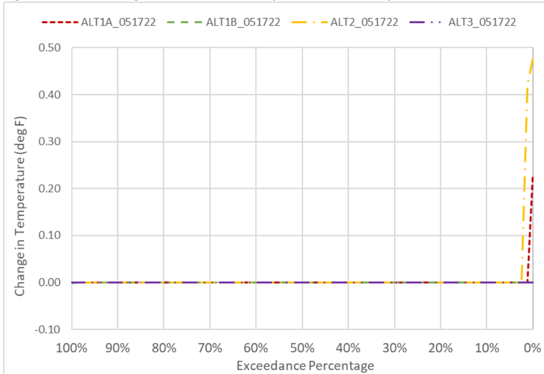
Figure 6D2-4-4. Changes to GCC Water Temperature in January
