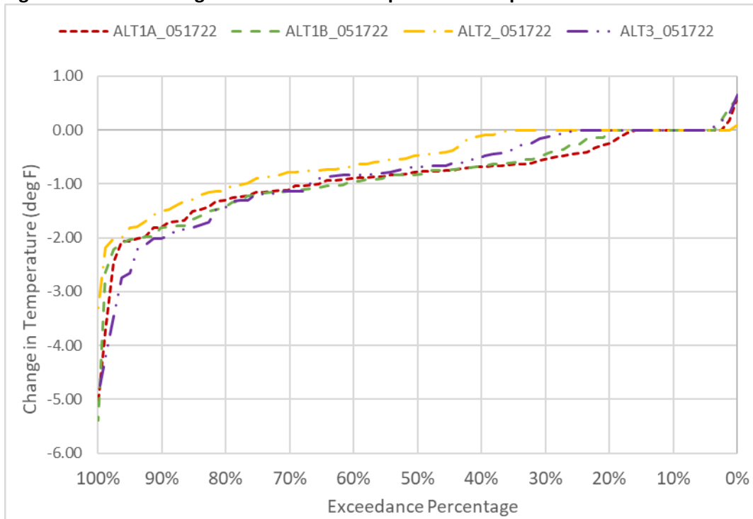
Figure 6D2-6-12. Changes to CBD Water Temperature in September
