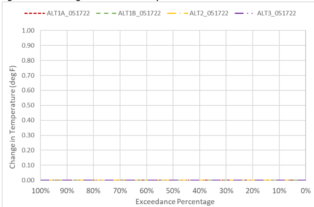
Figure 6D2-6-6. Changes to CBD Water Temperature in March
