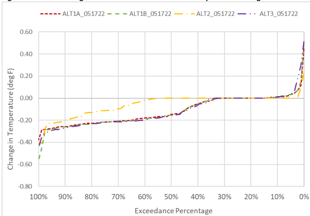
Figure 6D2-8-11. Changes to Sacramento River Water Temperature in August
