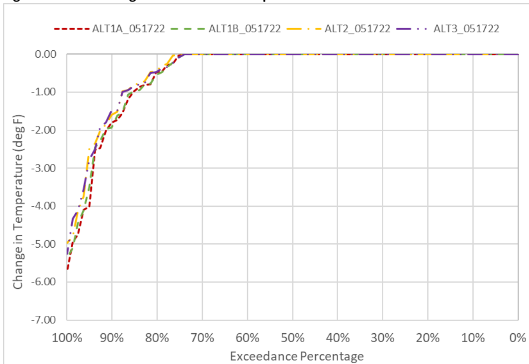
Figure 6D2-2-6. Changes to TCC Water Temperature in March
