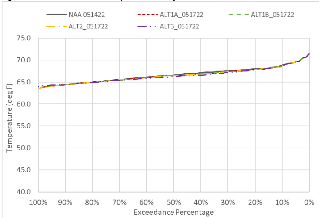
Figure 6D2-3-10. GCC Water Temperature in July
