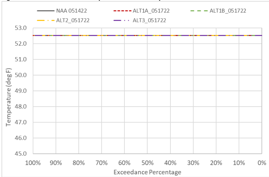
Figure 6D2-5-5. CBD Water Temperature in February
