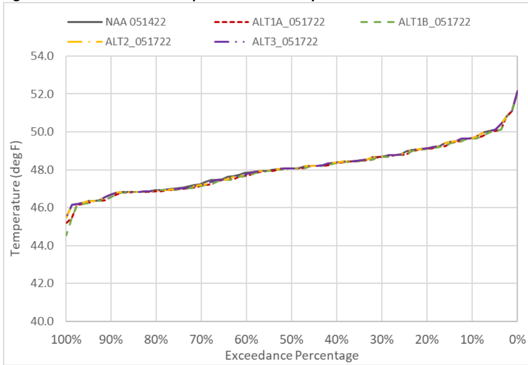
Figure 6D2-1-5. TCC Water Temperature in February
