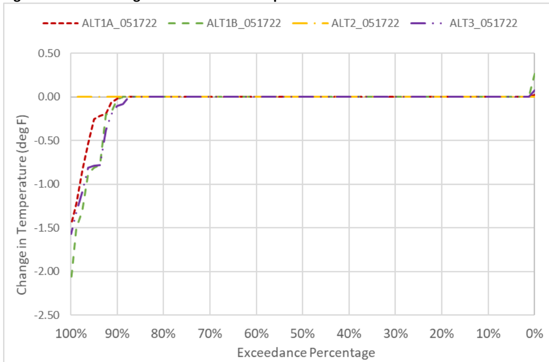
Figure 6D2-6-3. Changes to CBD Water Temperature in December
