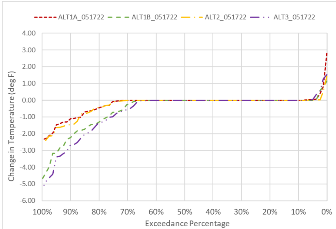
Figure 6D2-2-8. Changes to TCC Water Temperature in May
