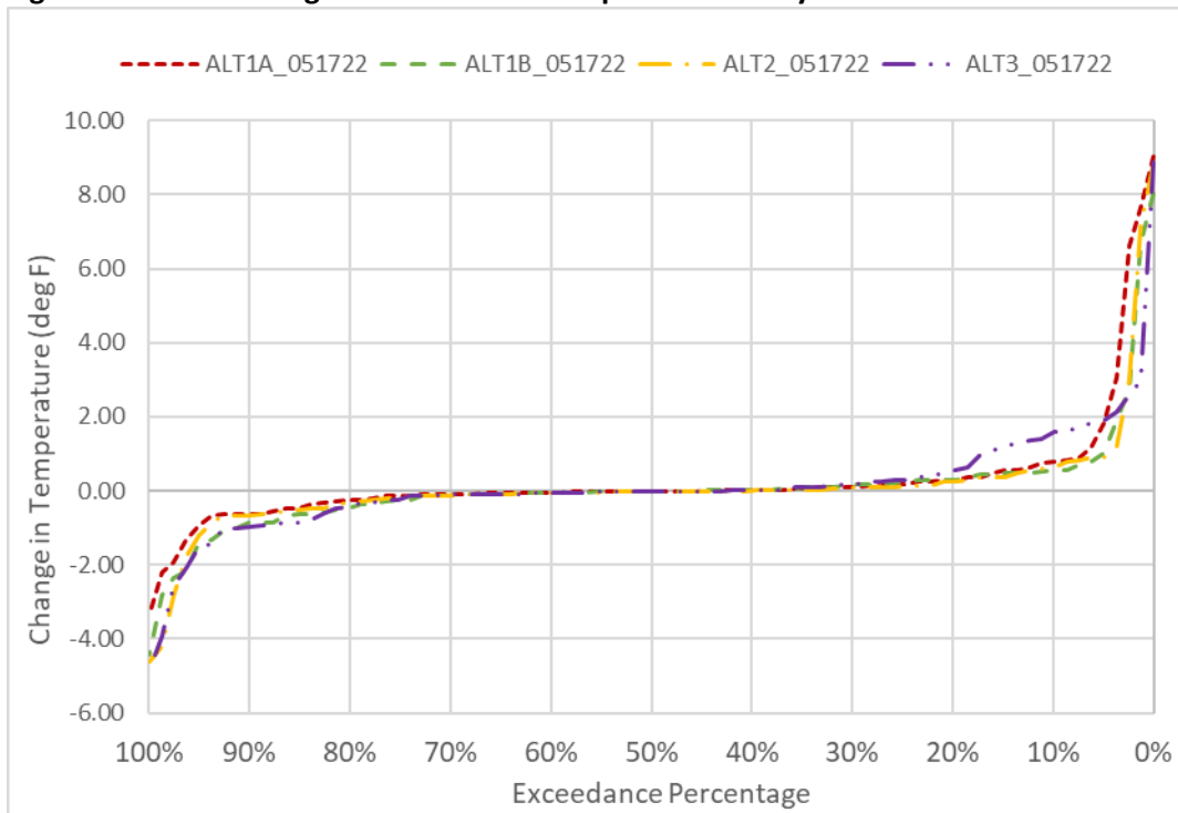
Figure 6D2-2-10. Changes to TCC Water Temperature in July
