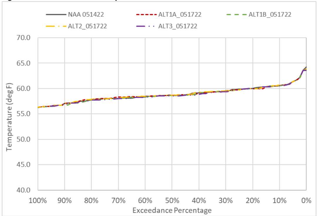
Figure 6D2-3-1. GCC Water Temperature in October
