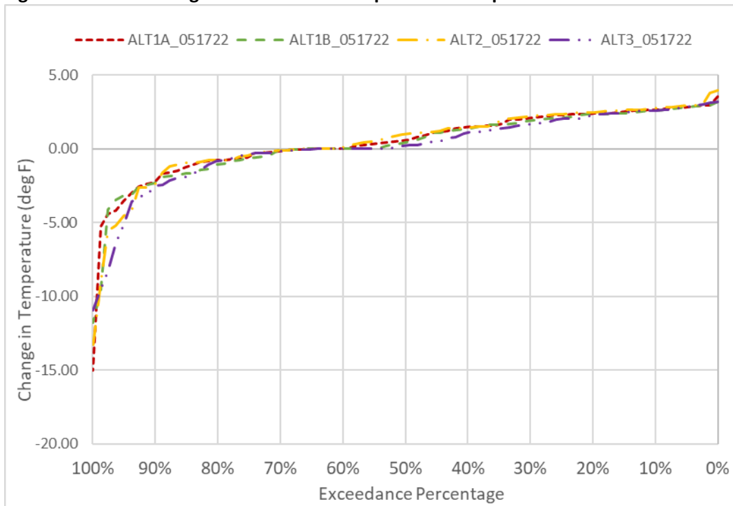
Figure 6D2-2-12. Changes to TCC Water Temperature in September
