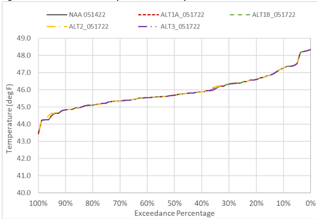
Figure 6D2-3-4. GCC Water Temperature in January
