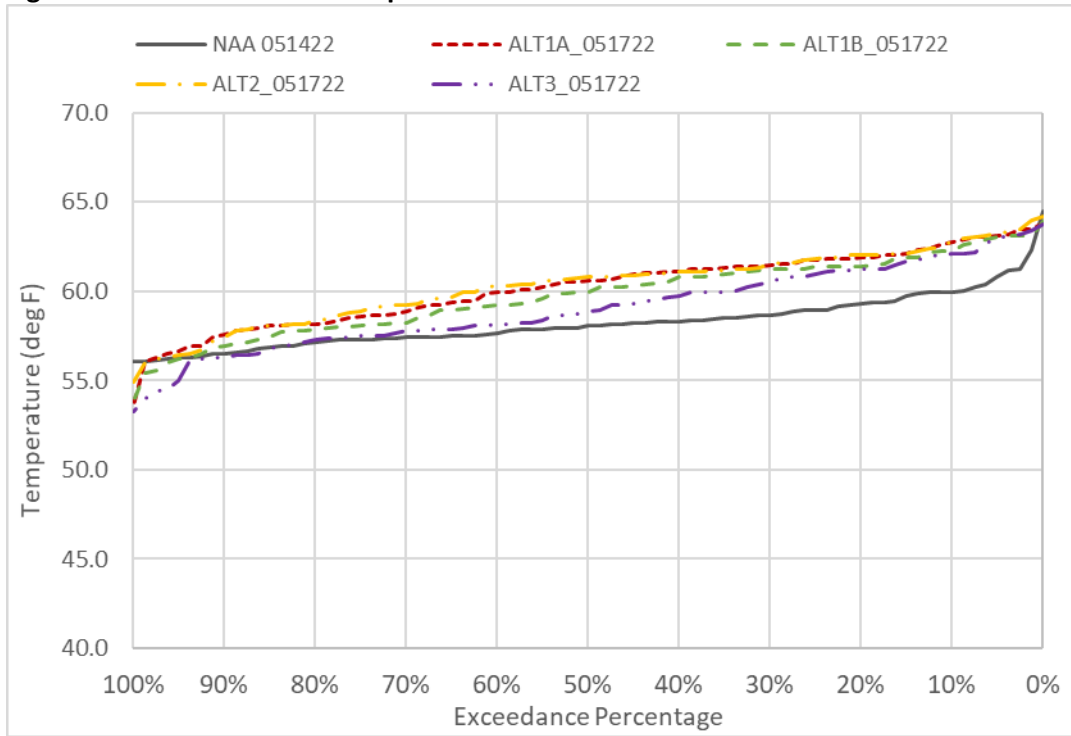
Figure 6D2-1-1. TCC Water Temperature in October
