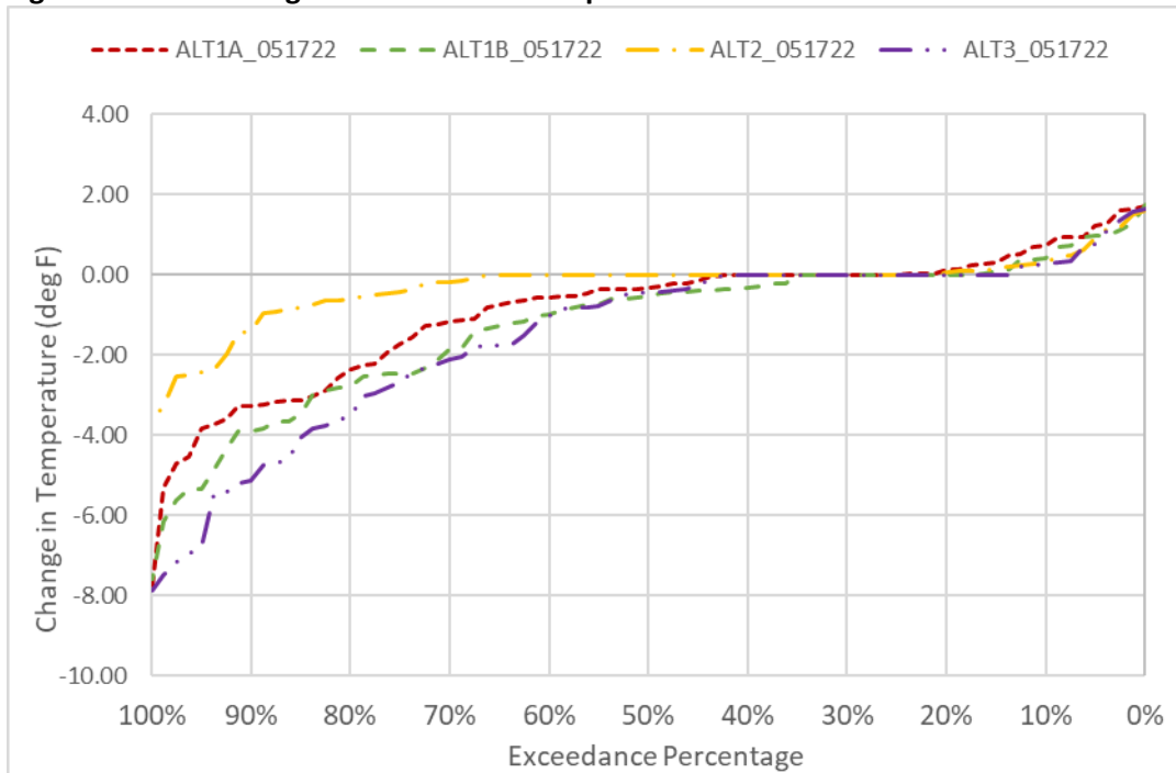
Figure 6D2-6-1. Changes to CBD Water Temperature in October
