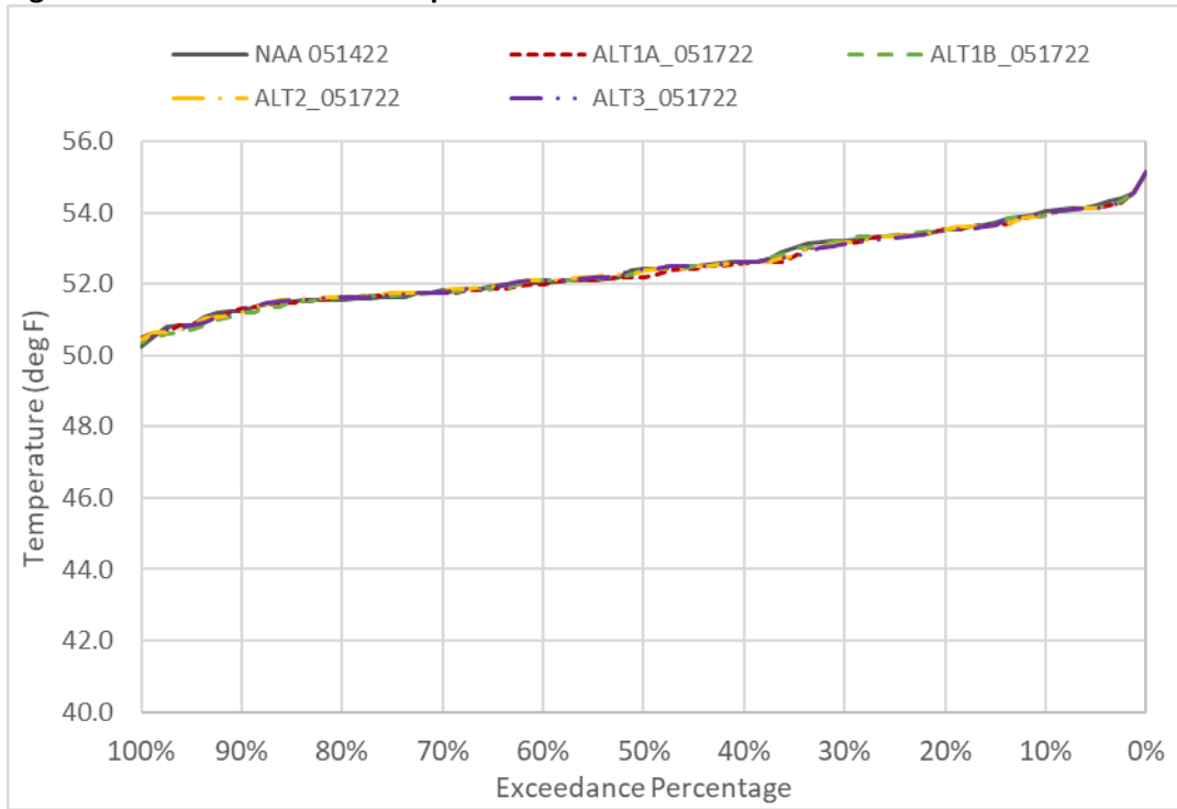
Figure 6D2-3-2. GCC Water Temperature in November
