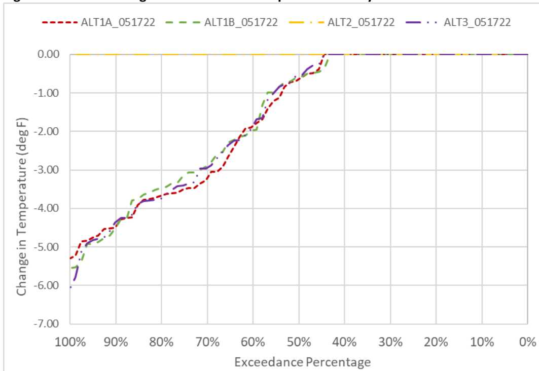
Figure 6D2-6-10. Changes to CBD Water Temperature in July
