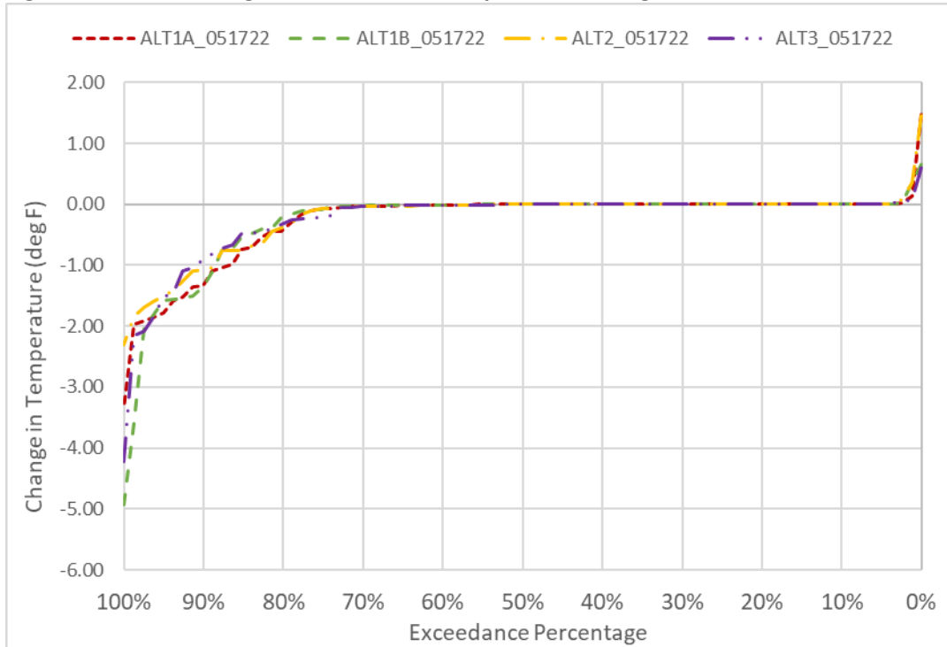
Figure 6D2-4-11. Changes to GCC Water Temperature in August
