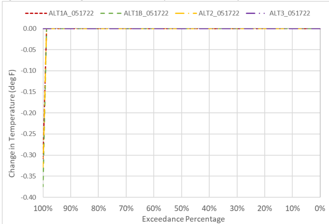
Figure 6D2-4-5. Changes to GCC Water Temperature in February
