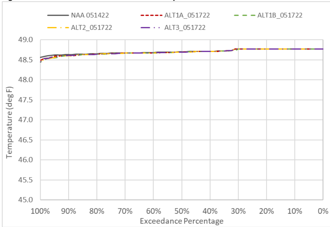
Figure 6D2-7-3. Sacramento River Water Temperature in December
