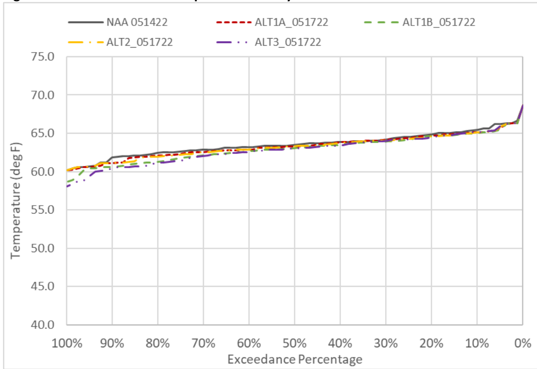
Figure 6D2-1-8. TCC Water Temperature in May
