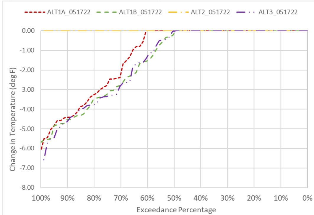
Figure 6D2-6-9. Changes to CBD Water Temperature in June
