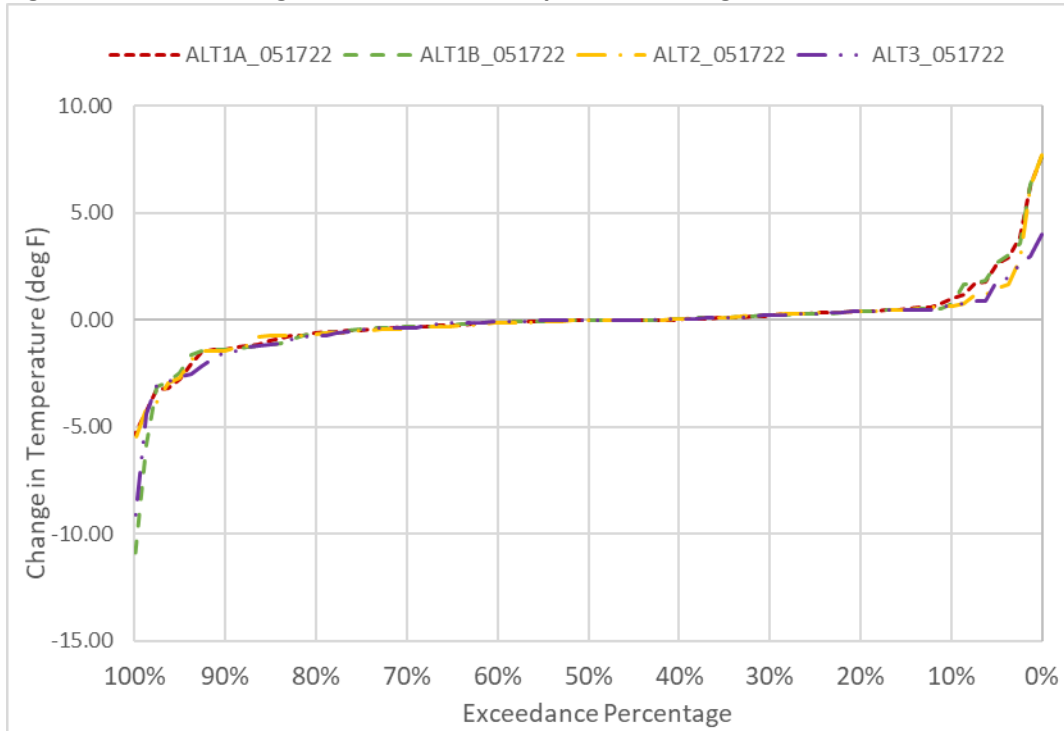
Figure 6D2-2-11. Changes to TCC Water Temperature in August
