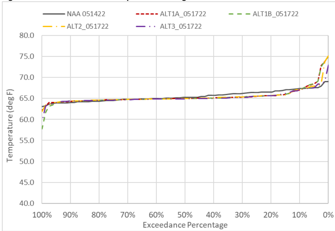
Figure 6D2-1-11. TCC Water Temperature in August
