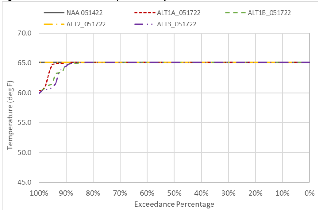
Figure 6D2-5-7. CBD Water Temperature in April
