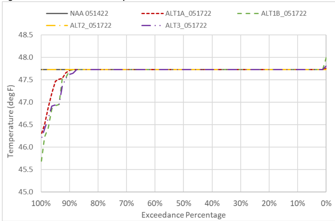
Figure 6D2-5-3. CBD Water Temperature in December
