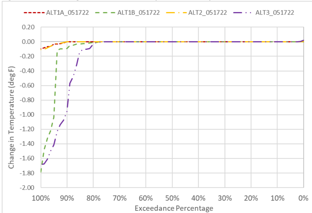
Figure 6D2-4-8. Changes to GCC Water Temperature in May
