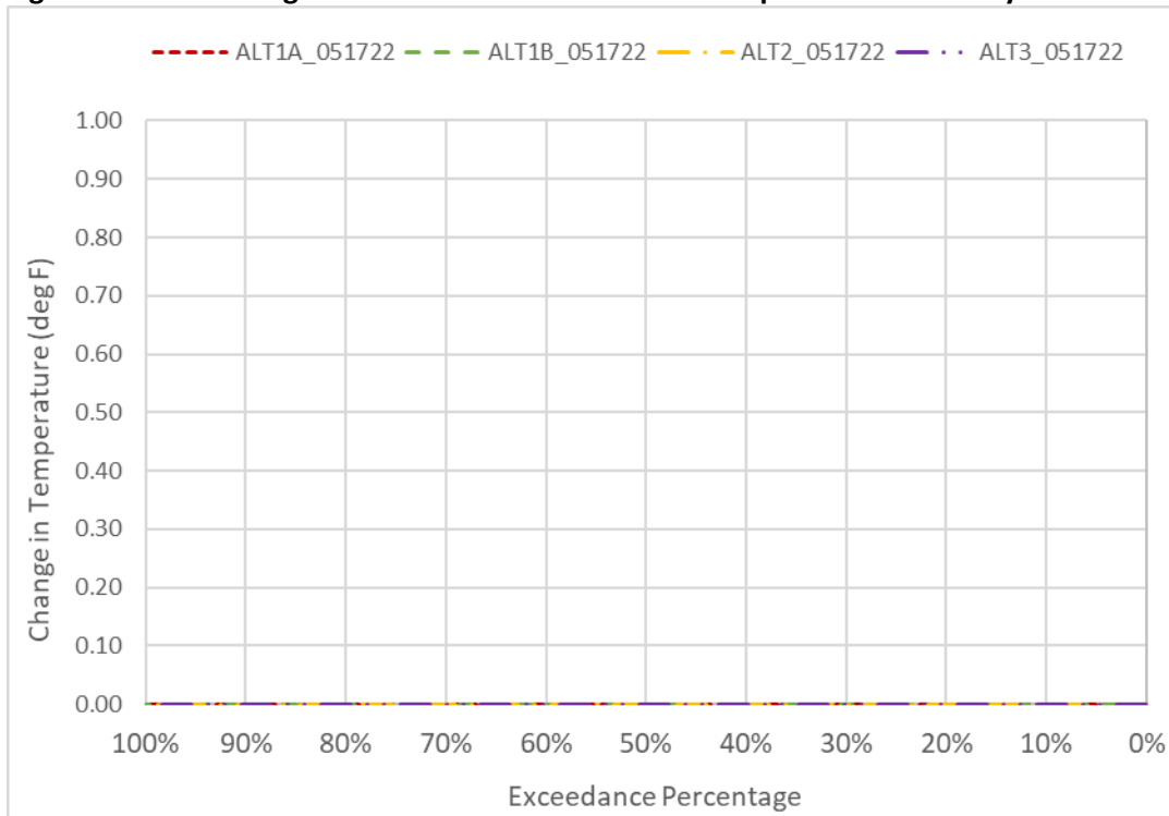
Figure 6D2-8-4. Changes to Sacramento River Water Temperature in January
