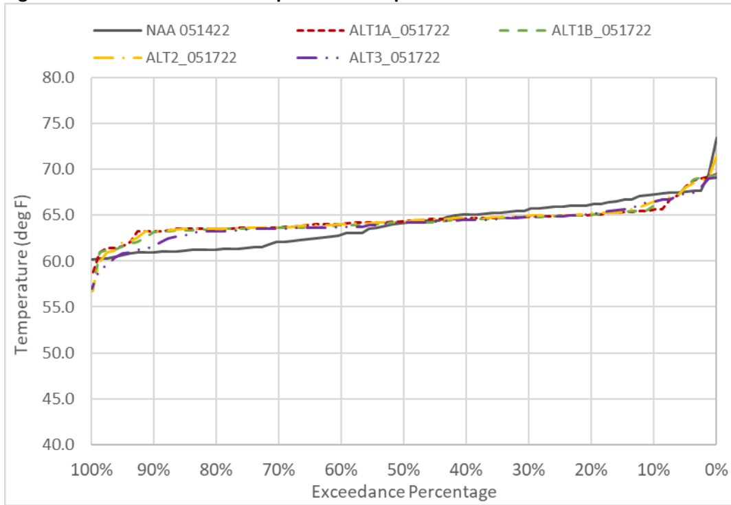
Figure 6D2-1-12. TCC Water Temperature in September
