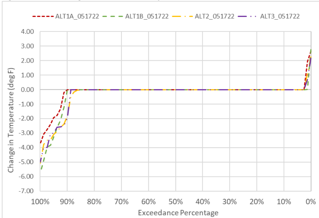
Figure 6D2-2-3. Changes to TCC Water Temperature in December
