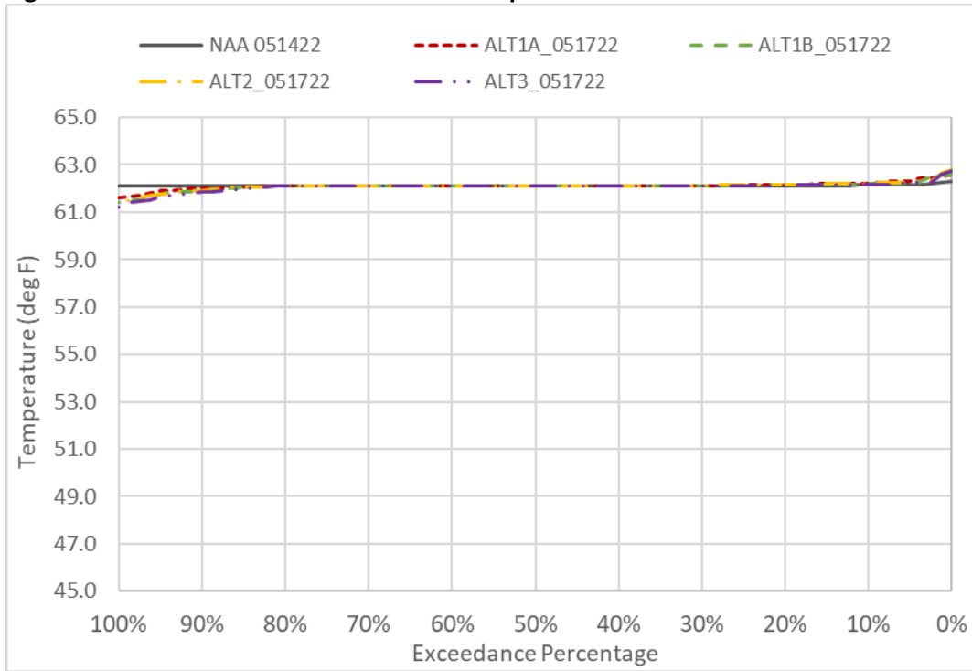
Figure 6D2-7-1. Sacramento River Water Temperature in October
