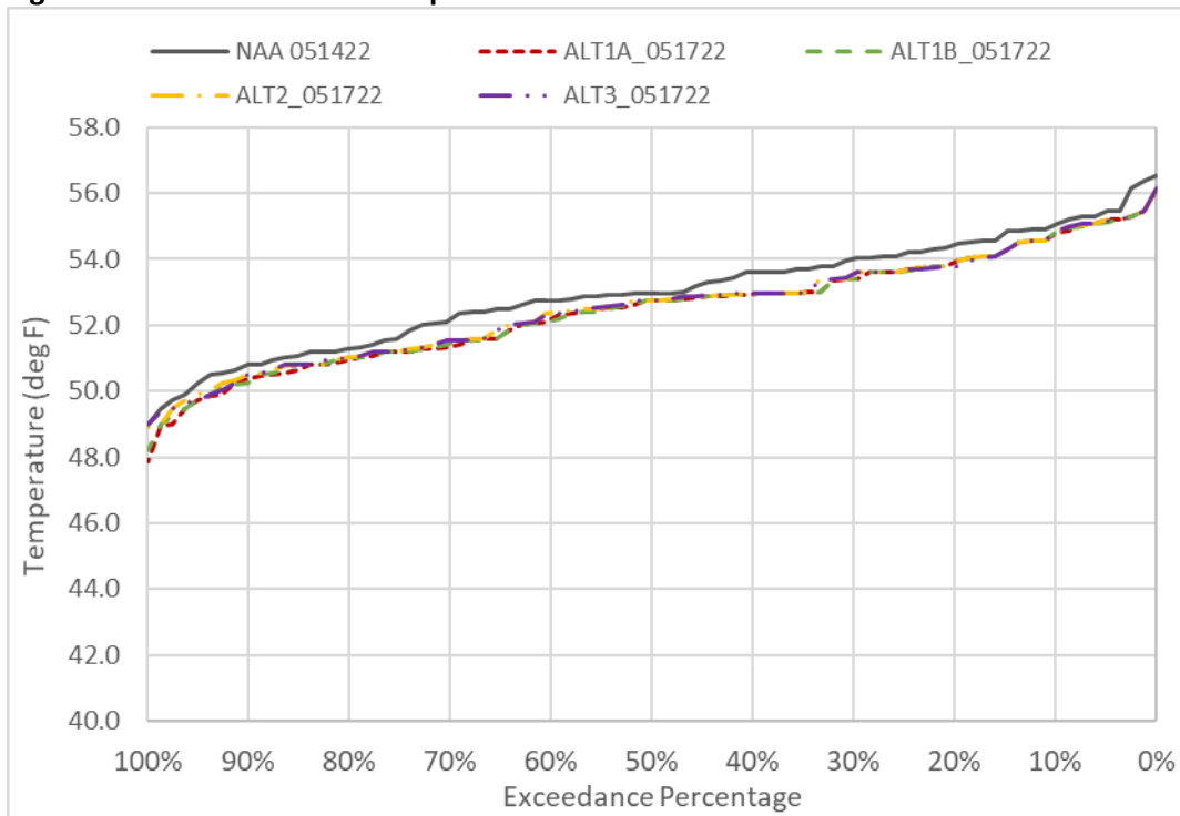
Figure 6D2-1-6. TCC Water Temperature in March
