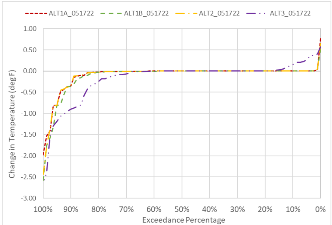
Figure 6D2-4-10. Changes to GCC Water Temperature in July
