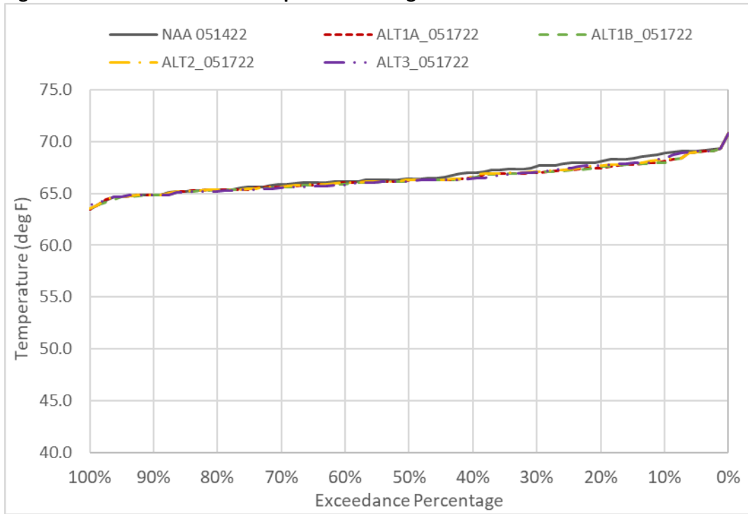
Figure 6D2-3-11. GCC Water Temperature in August
