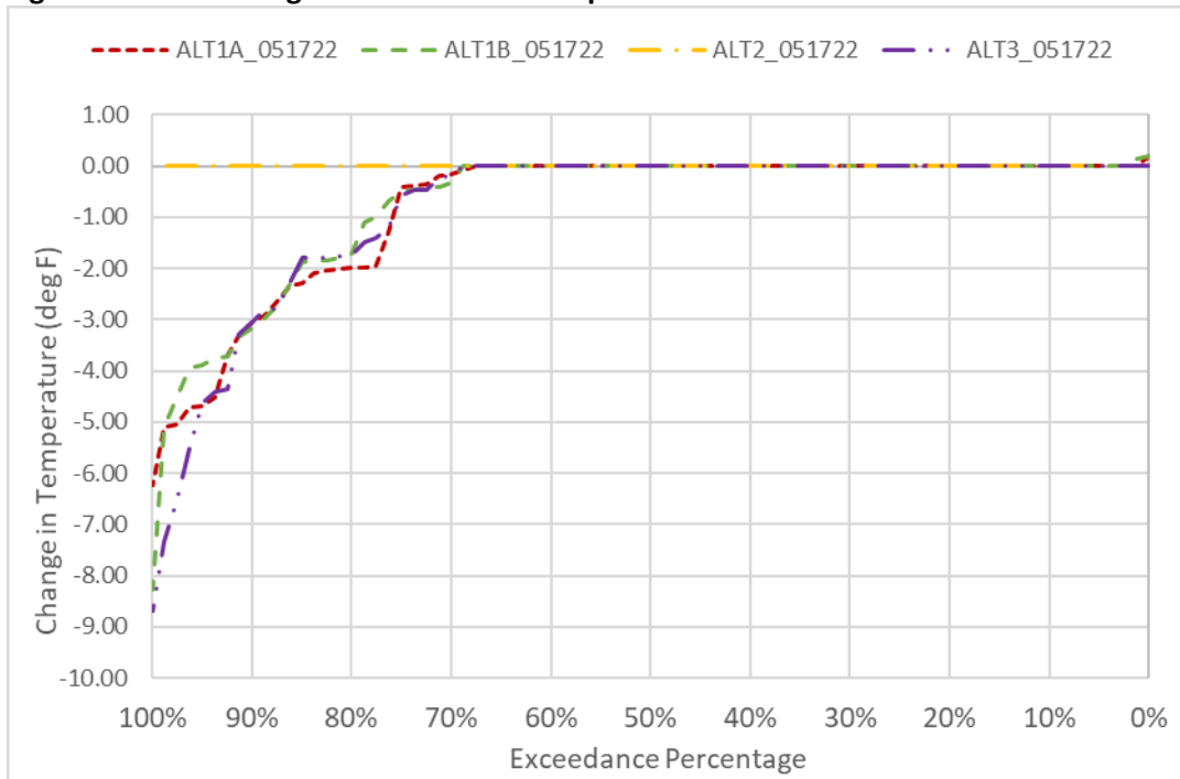
Figure 6D2-6-2. Changes to CBD Water Temperature in November
