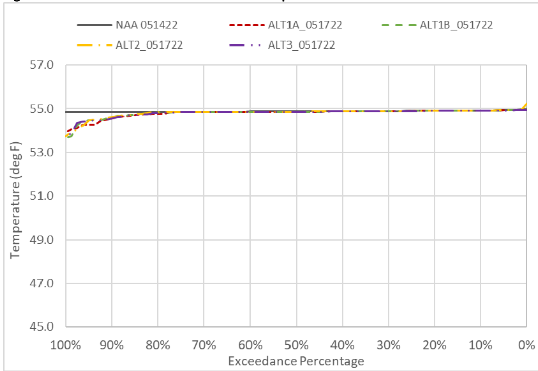
Figure 6D2-7-2. Sacramento River Water Temperature in November
