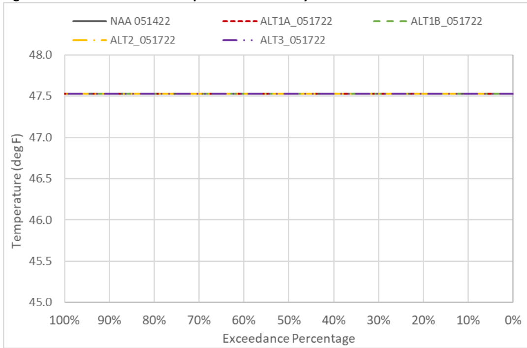
Figure 6D2-5-4. CBD Water Temperature in January
