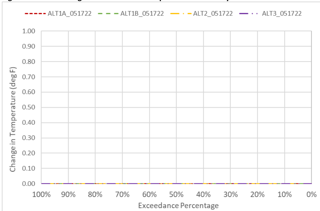
Figure 6D2-6-4. Changes to CBD Water Temperature in January
