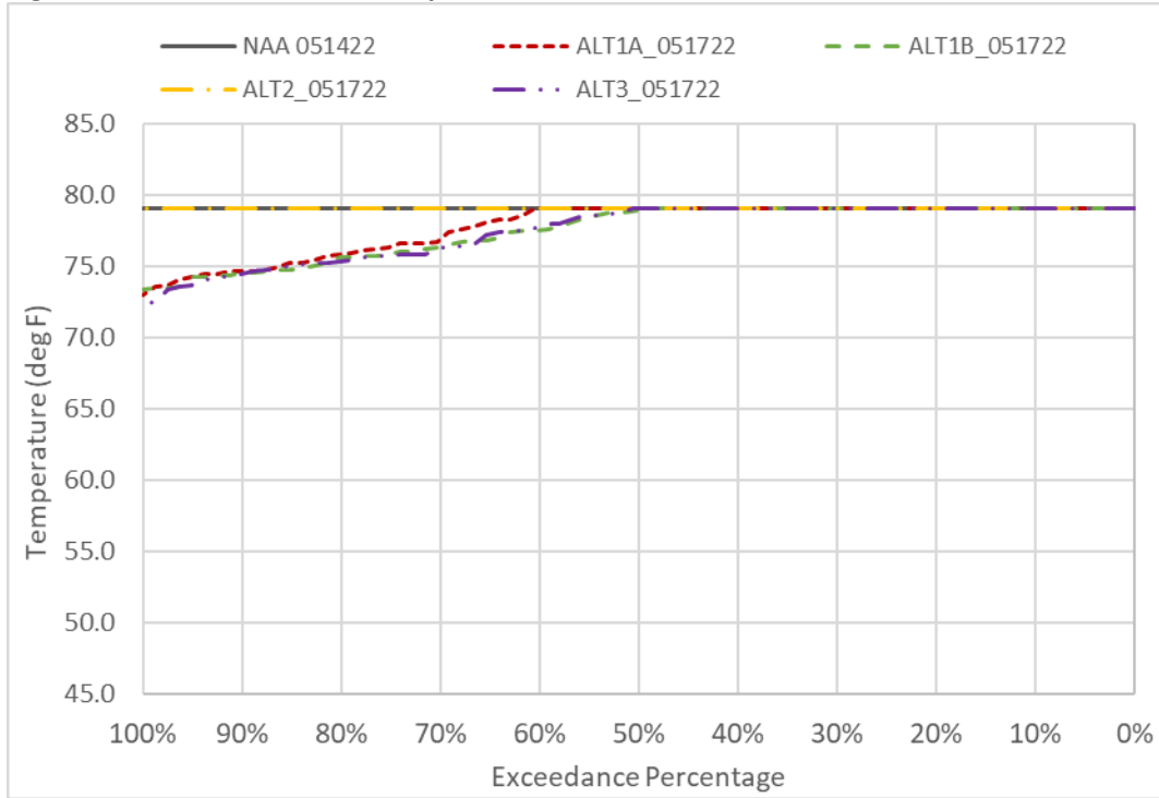
Figure 6D2-5-9. CBD Water Temperature in June
