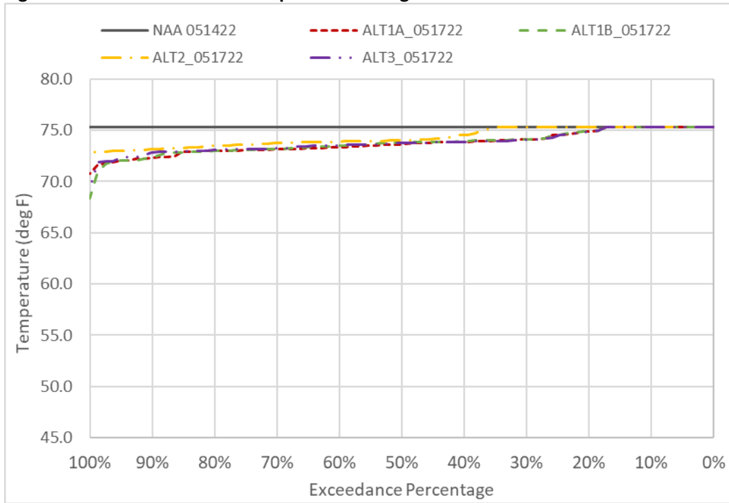
Figure 6D2-5-11. CBD Water Temperature in August
