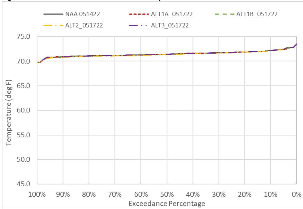
Figure 6D2-7-9. Sacramento River Water Temperature in June
