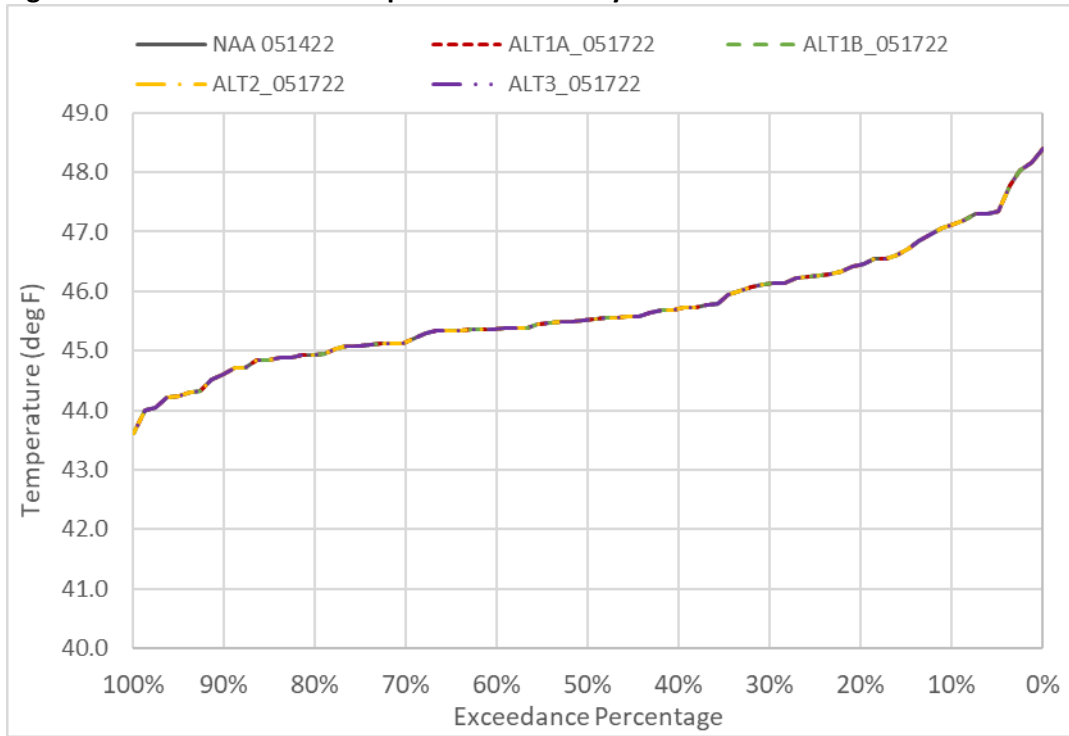
Figure 6D2-1-4. TCC Water Temperature in January
