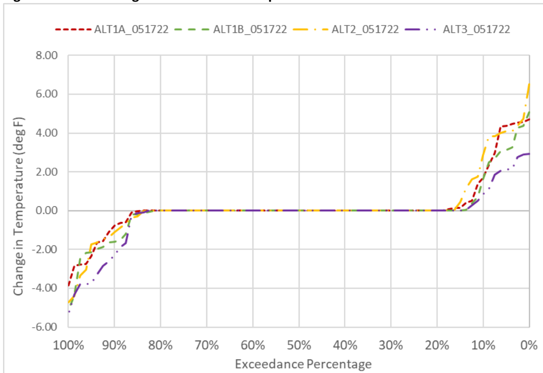
Figure 6D2-2-2. Changes to TCC Water Temperature in November
