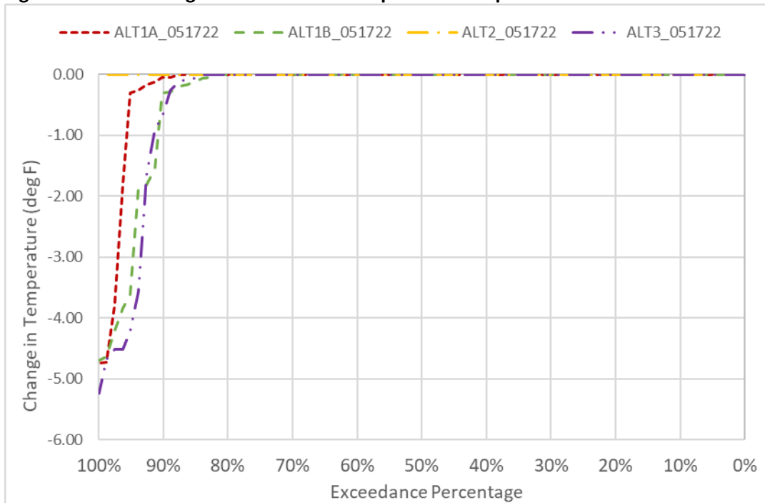
Figure 6D2-6-7. Changes to CBD Water Temperature in April
