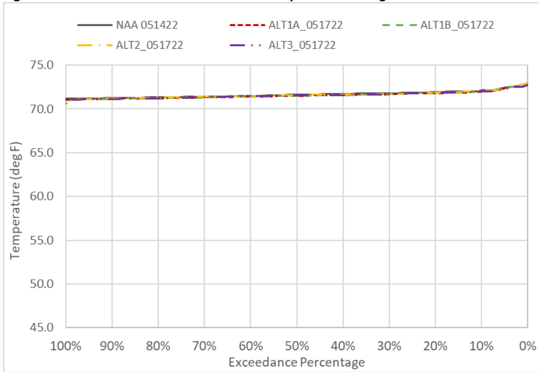
Figure 6D2-7-11. Sacramento River Water Temperature in August
