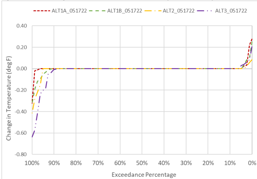
Figure 6D2-8-8. Changes to Sacramento River Water Temperature in May
