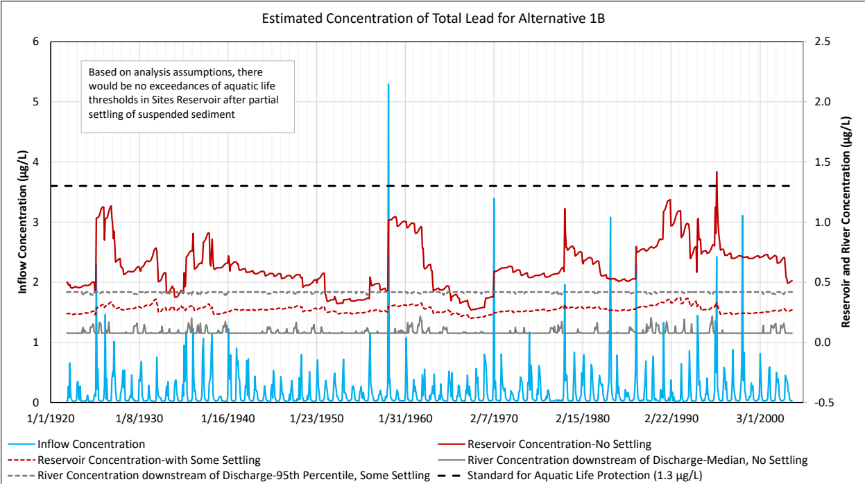
Figure 6-12. Estimated Total Lead Concentration in Inflow to Sites Reservoir, in Sites Reservoir, and in the Sacramento River at the Sites Discharge Location
