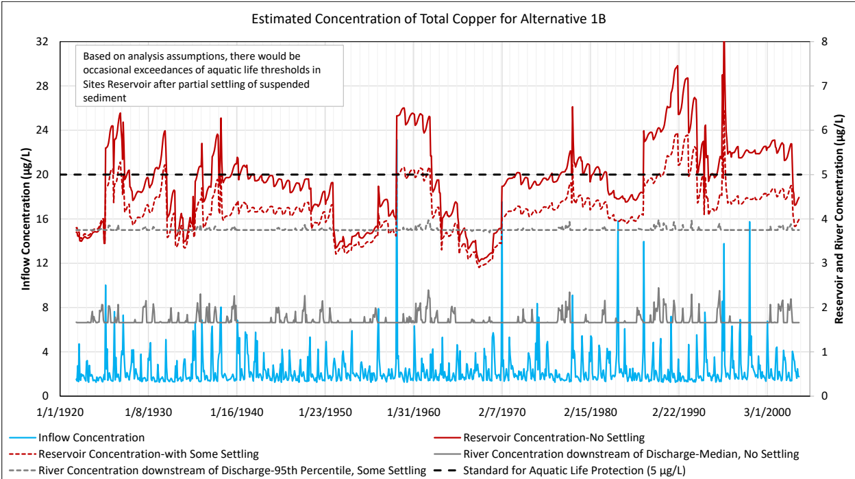
Figure 6-10. Estimated Total Copper Concentration in Inflow to Sites Reservoir, in Sites Reservoir, and in the Sacramento River at the Sites Discharge Location.
