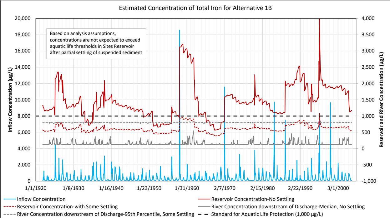
Figure 6-11. Estimated Total Iron Concentration in Inflow to Sites Reservoir, in Sites Reservoir, and in the Sacramento River at the Sites Discharge Location.
