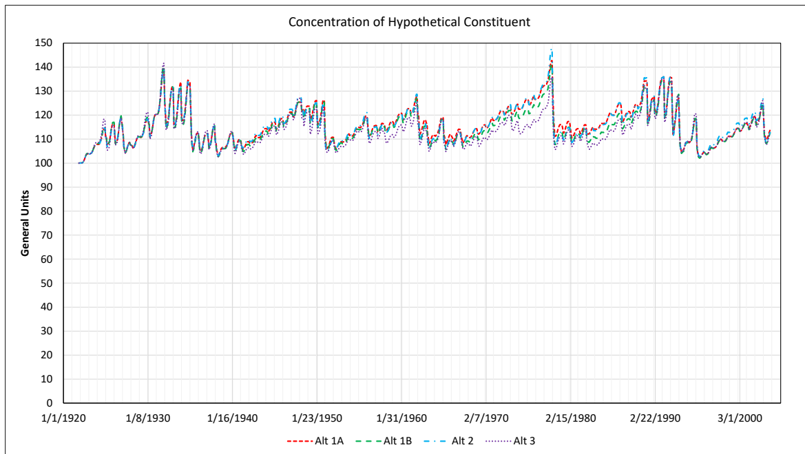
Figure 6-2. Estimated Effect of Evaporation from Sites Reservoir on a Hypothetical Constituent through Time as Derived from CALSIM Results
