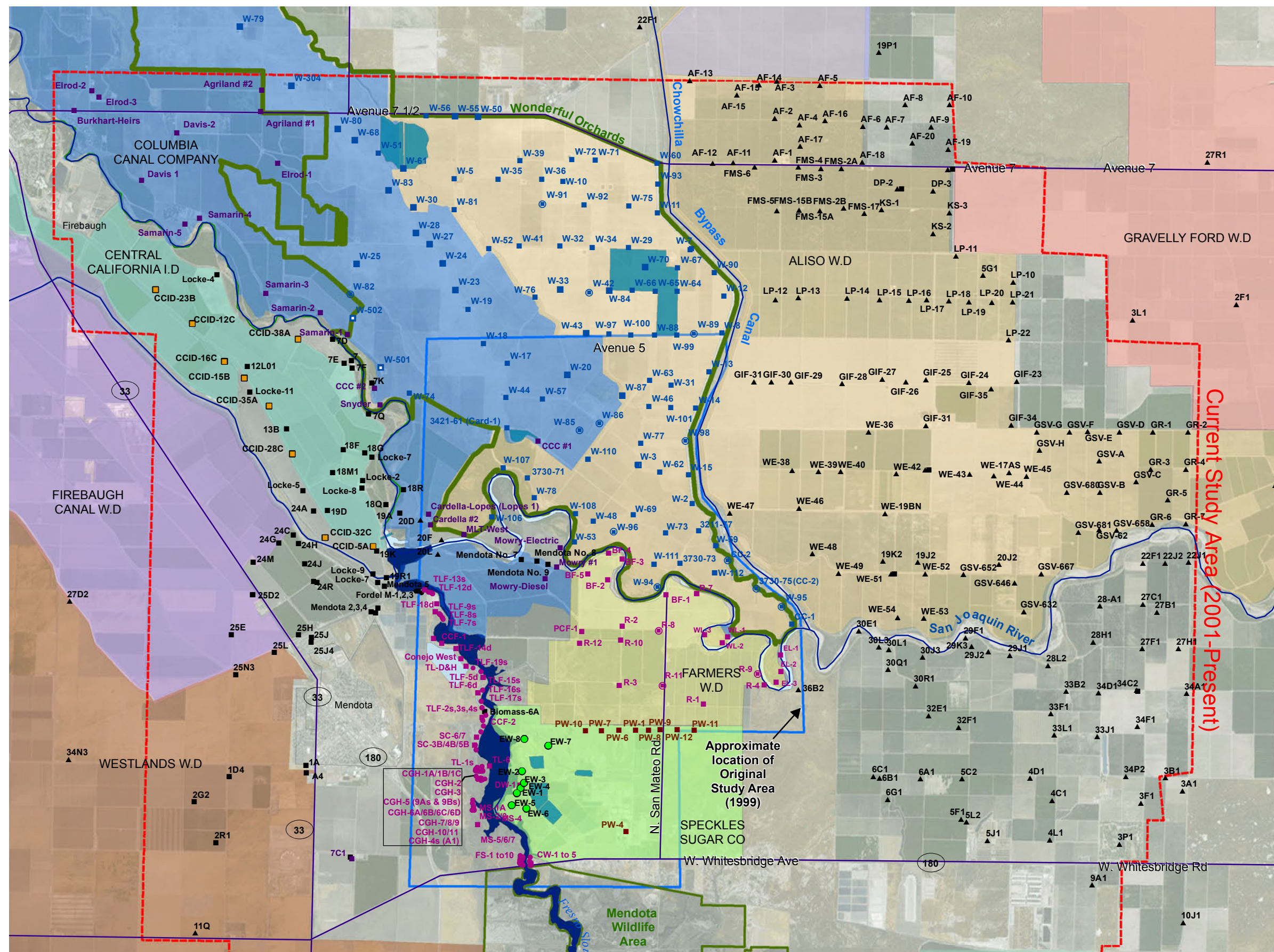
Figure 1-3 Production Wells in Mendota Area
