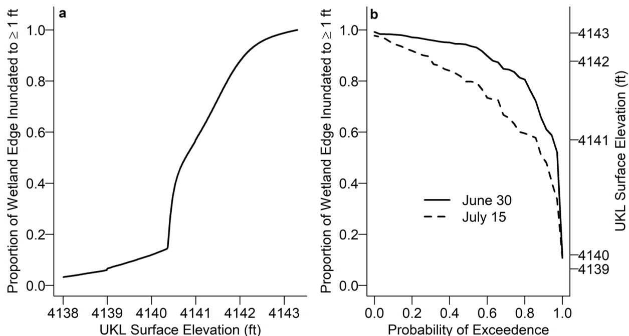
Figure 7-4. a) Relationship between UKL surface elevation and the proportion of emergent wetland edge habitat that is inundated to at least 1 ft (reproduced from Hereford and Roberts 2019 p. 9). b) The probability of exceedance for the proportion of emergent wetland edge habitat inundated to at least 1 ft on June 30 (solid line) and July 15 (dashed line) expected under the PA based on the model output from the period of record.
