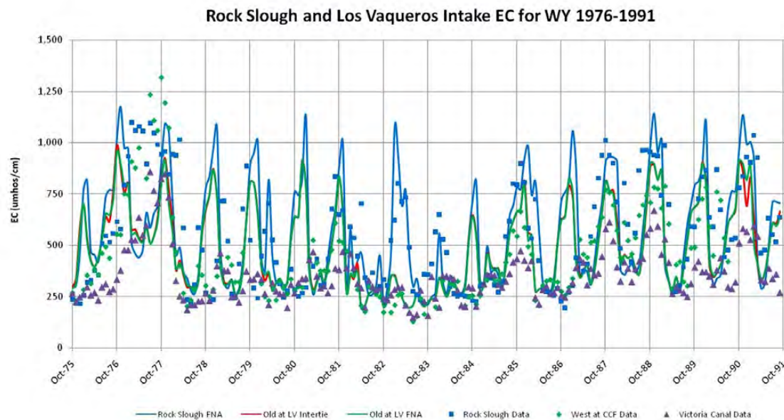
Figure 3.3-6. Comparison of Historical and Simulated No Action and Intertie EC at Rock Slough and Los Vaqueros Intake for Water Years 1976–1991
