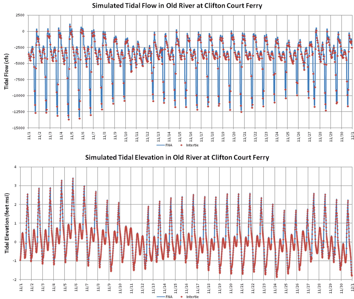
Figure 3.2-3 Comparison of DSM2-Simulated Tidal Elevations and Tidal Flows for the Intertie (4,600 cfs CVP Pumping) and No Action Alternative (4,250 cfs CVP Pumping) in Old River at Clifton Court Ferry for November 1975
