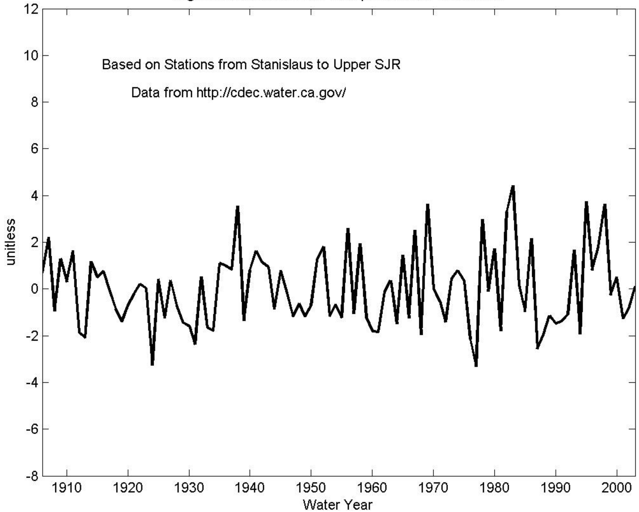
Fig.H1-Observed Annual Precip Index C2: 1906-2003
