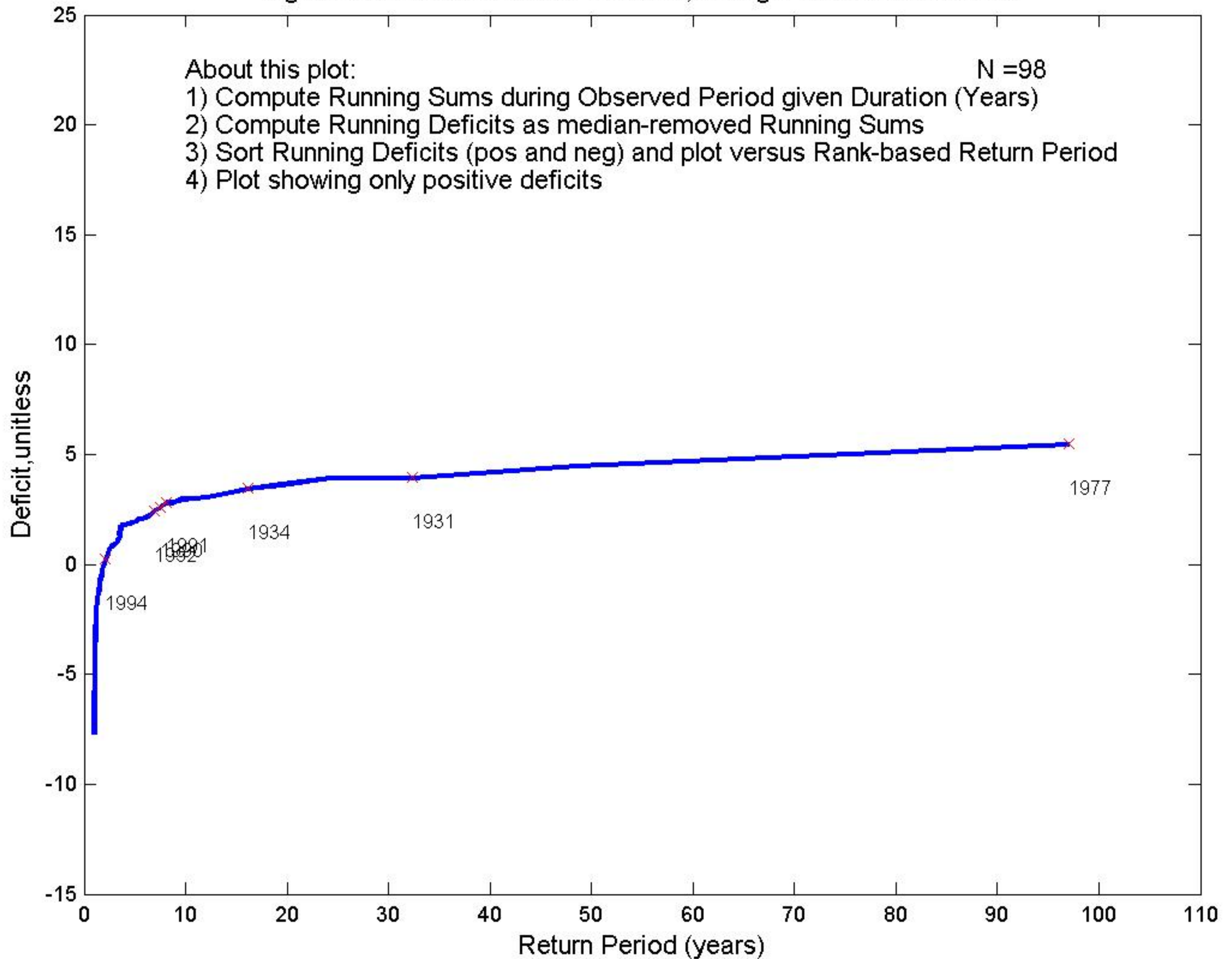
Fig.H2-Observed:Two-Year Duration, Drought End-Years Labeled
