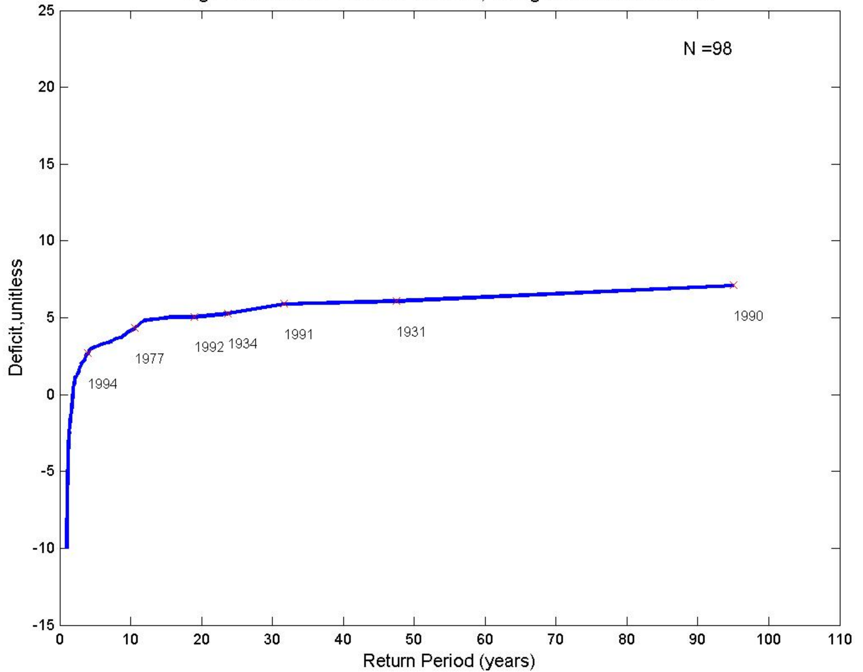
Fig.H4-Observed:Four-Year Duration, Drought End-Years Labeled
