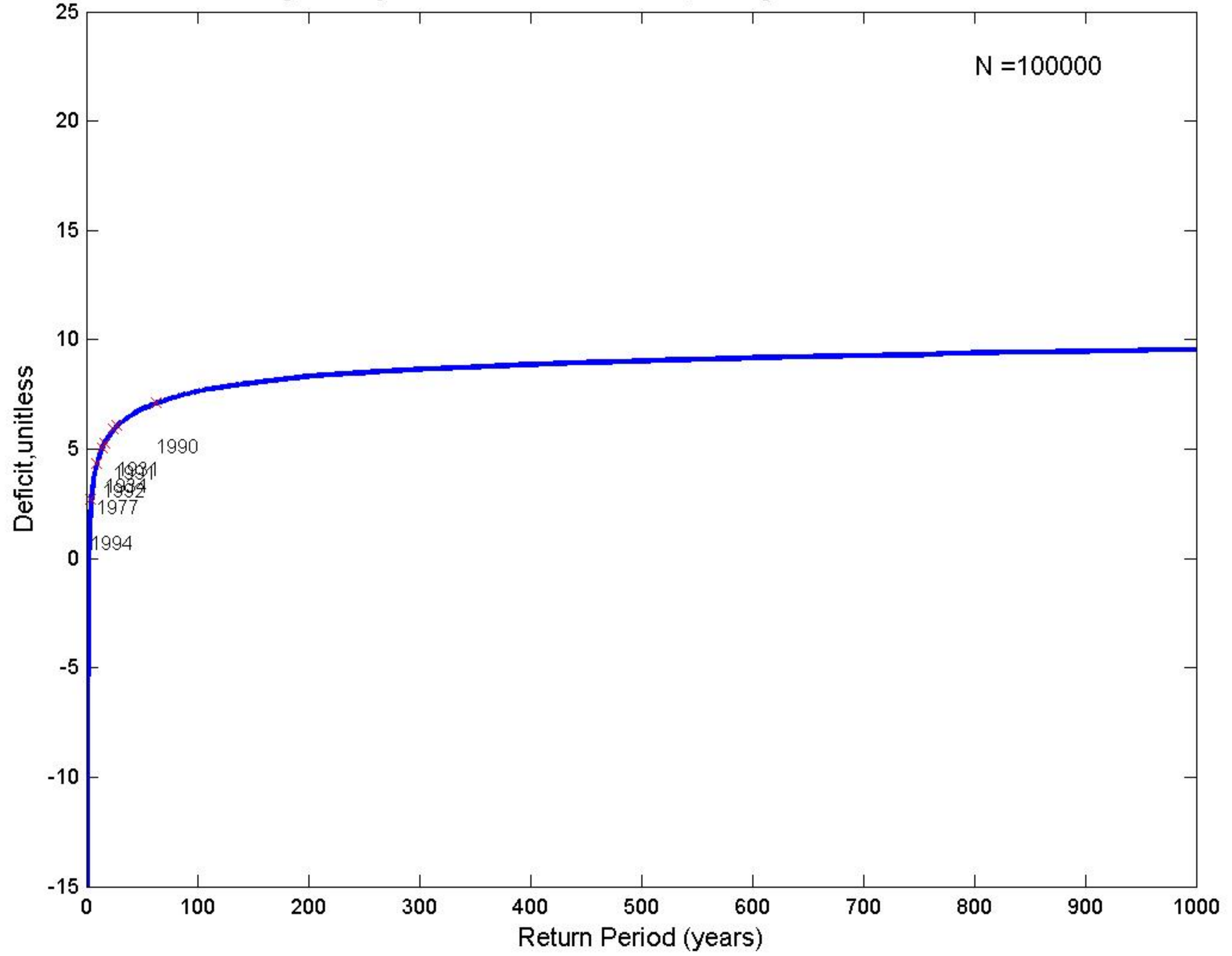
Fig.H17-Synthetic:Four-Year Duration, Drought End-Years Labeled
