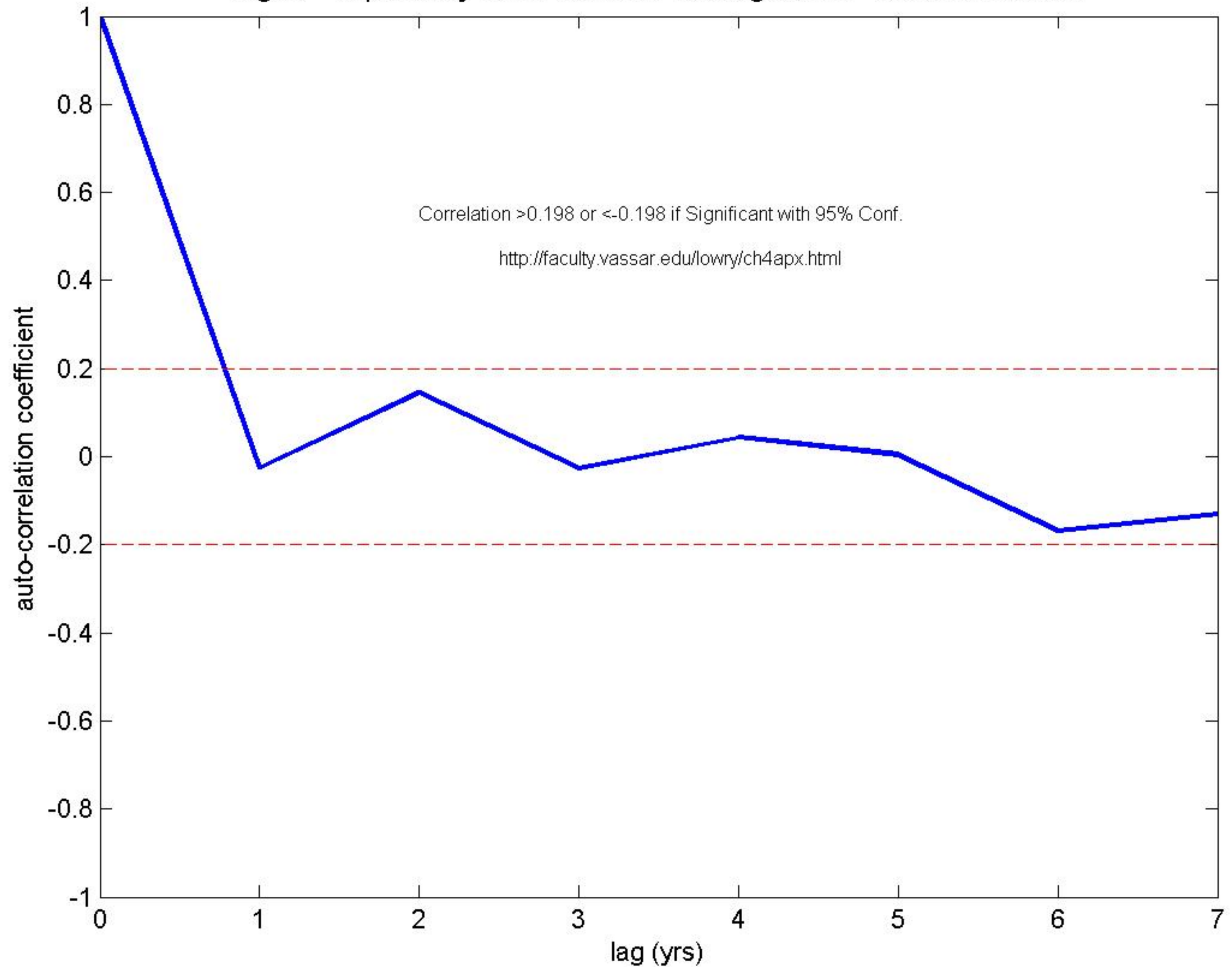
Fig.H7 - Explanatory Term: Consider Autoregression - Check Correlation
