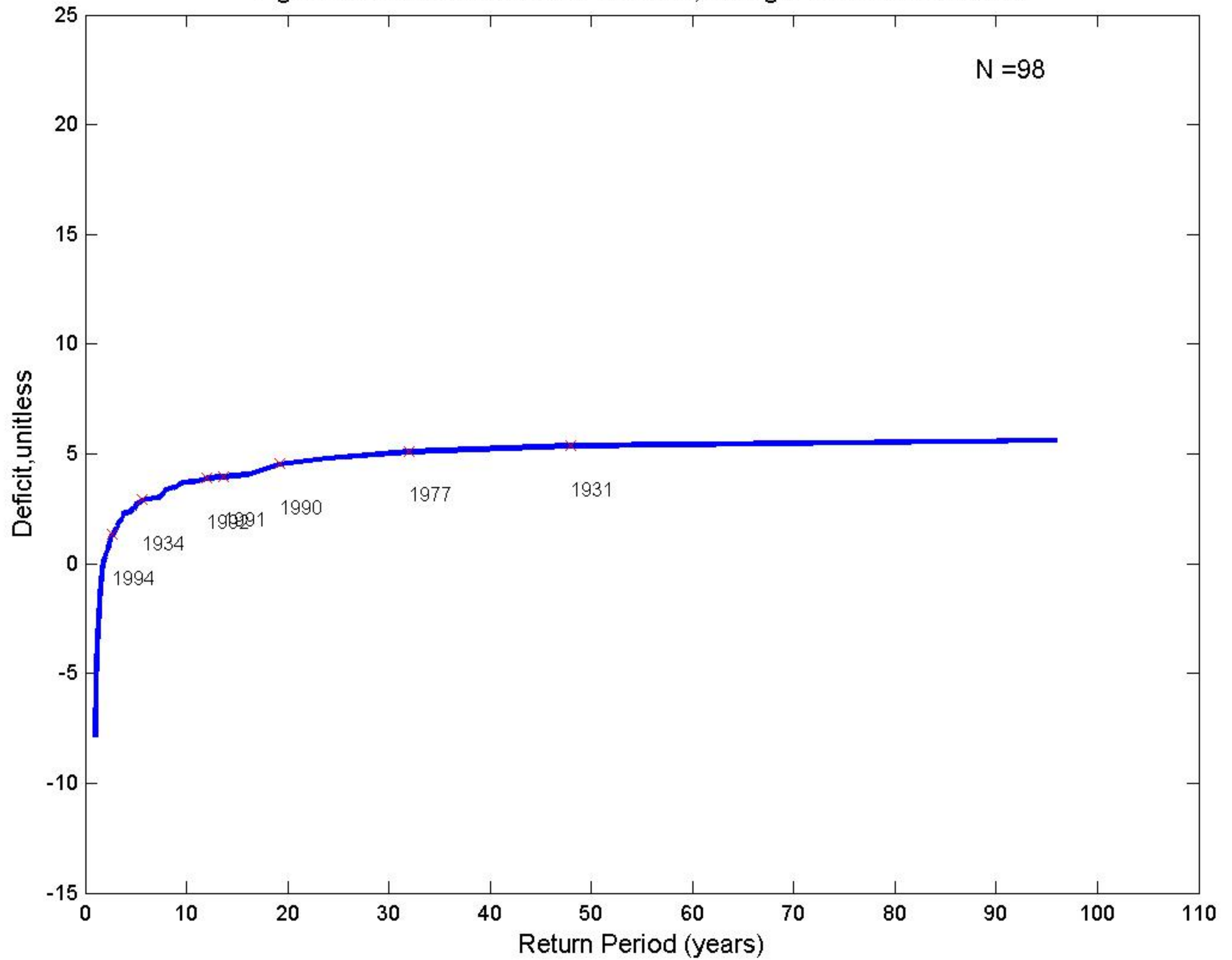
Fig.H3-Observed:Three-Year Duration, Drought End-Years Labeled
