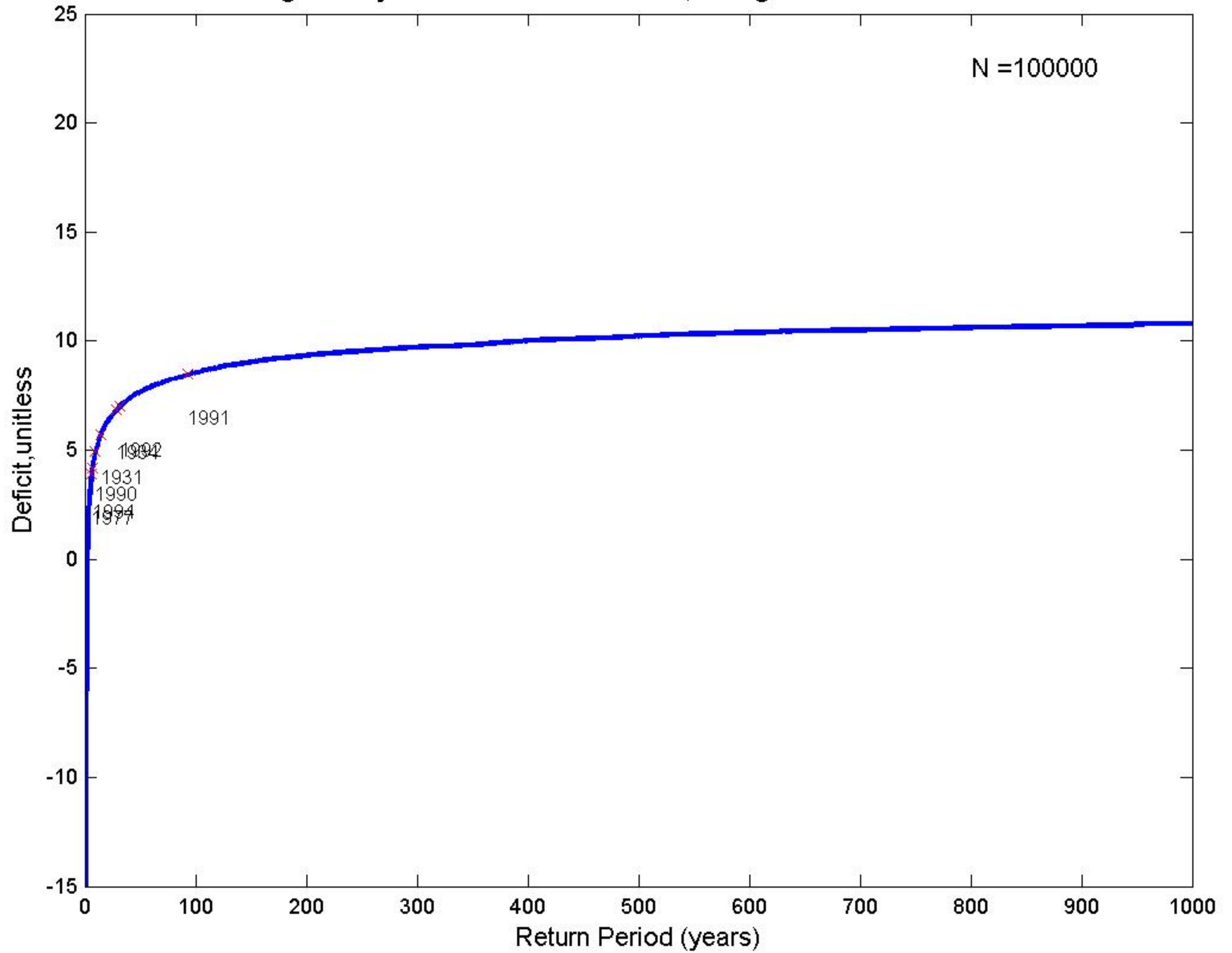
Fig.H18-Synthetic:Five-Year Duration, Drought End-Years Labeled
