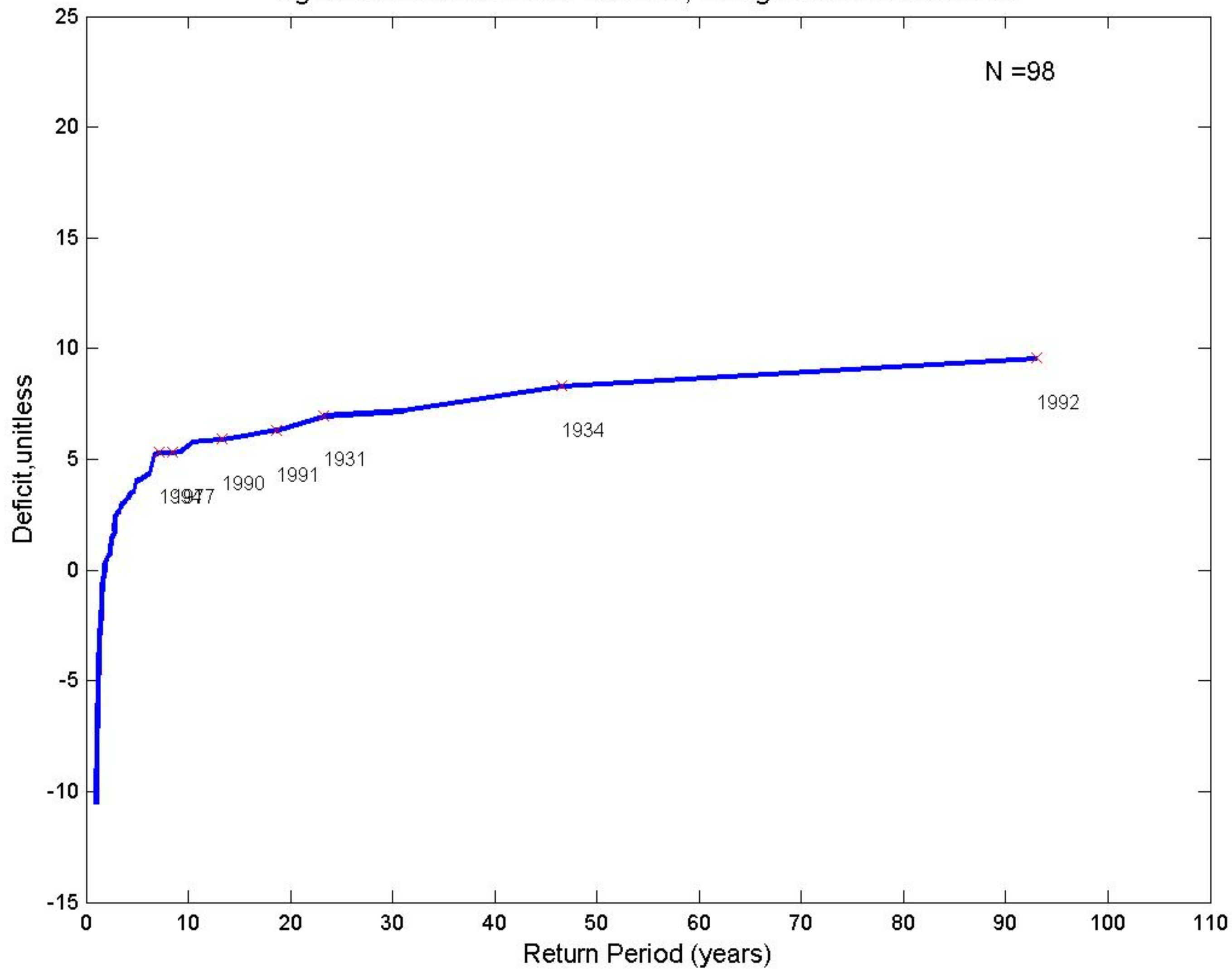
Fig.H6-Observed:Six-Year Duration, Drought End-Years Labeled
