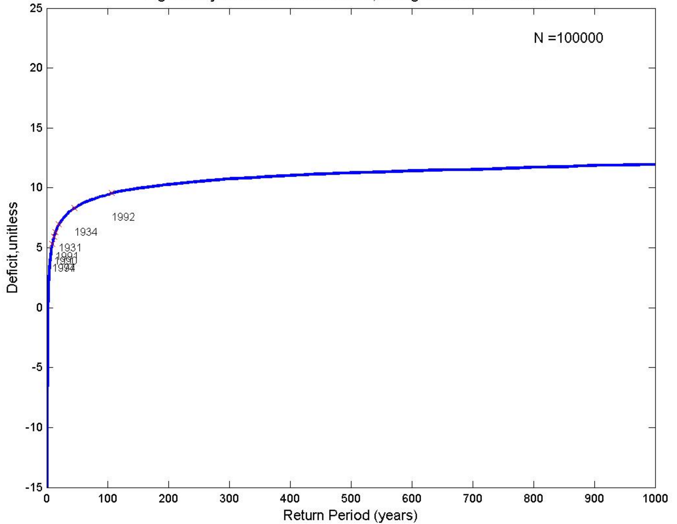
Fig.H19-Synthetic:Six-Year Duration, Drought End-Years Labeled
