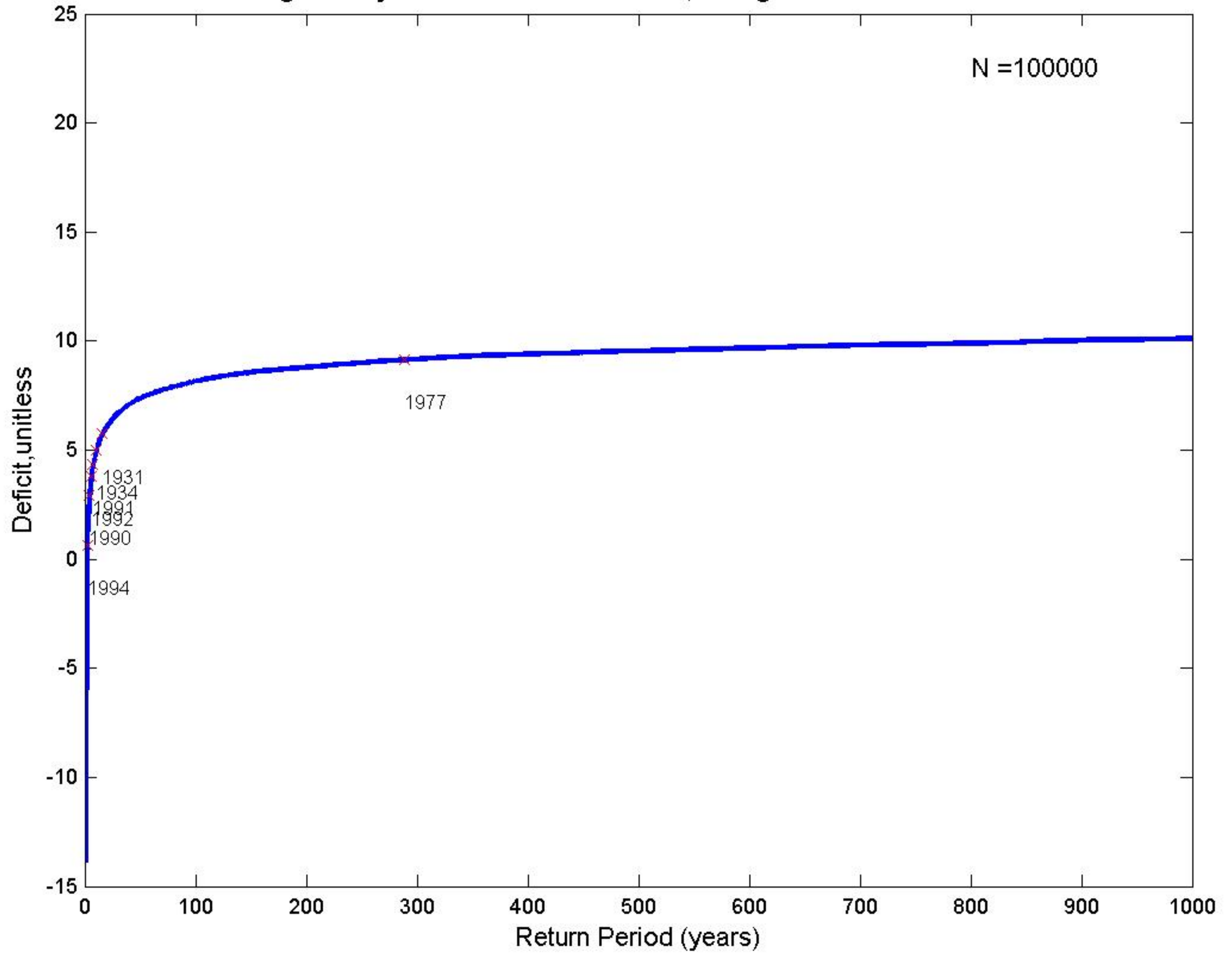
Fig.G15-Synthetic:Two-Year Duration, Drought End-Years Labeled
