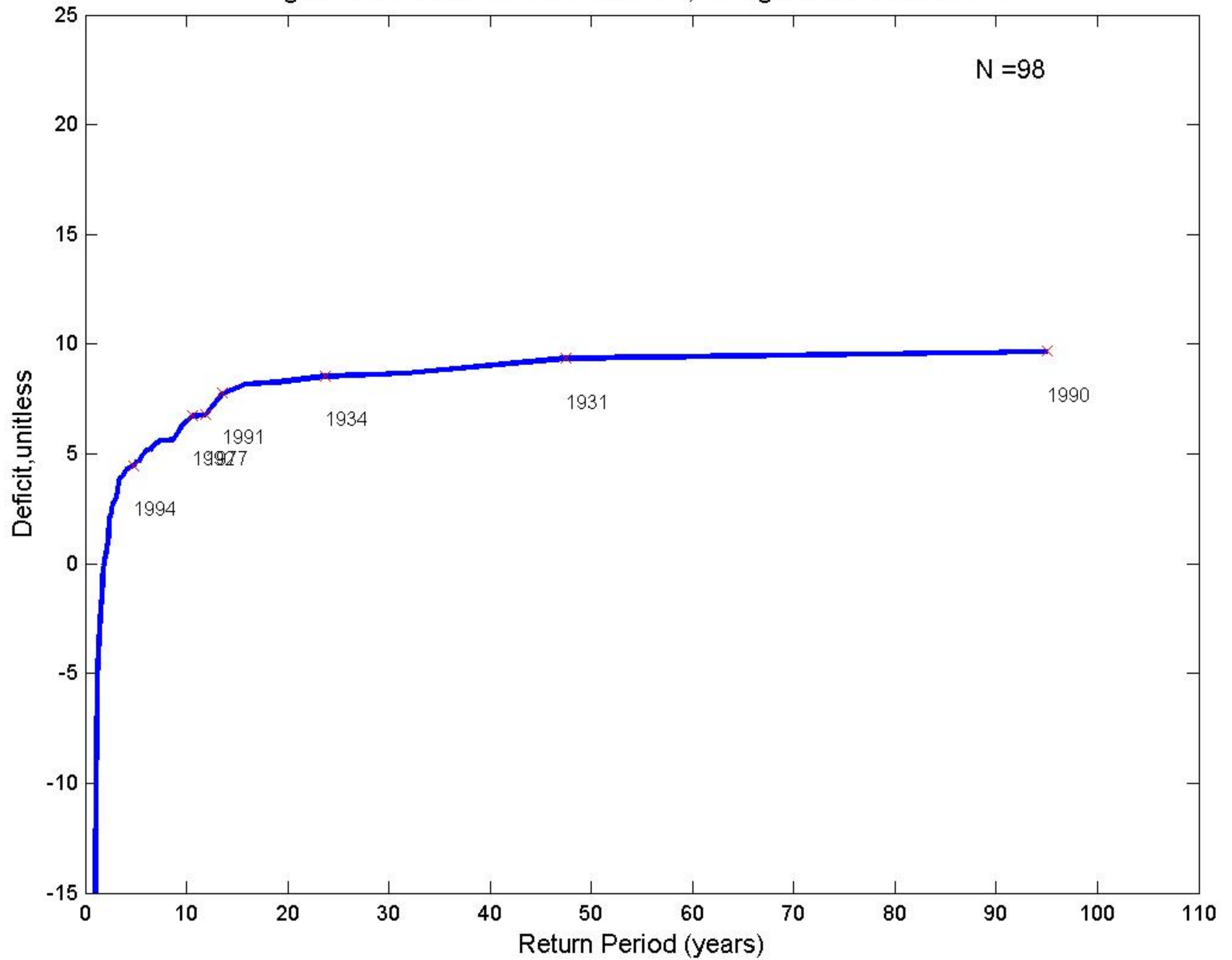
Fig.G4-Observed:Four-Year Duration, Drought End-Years Labeled
