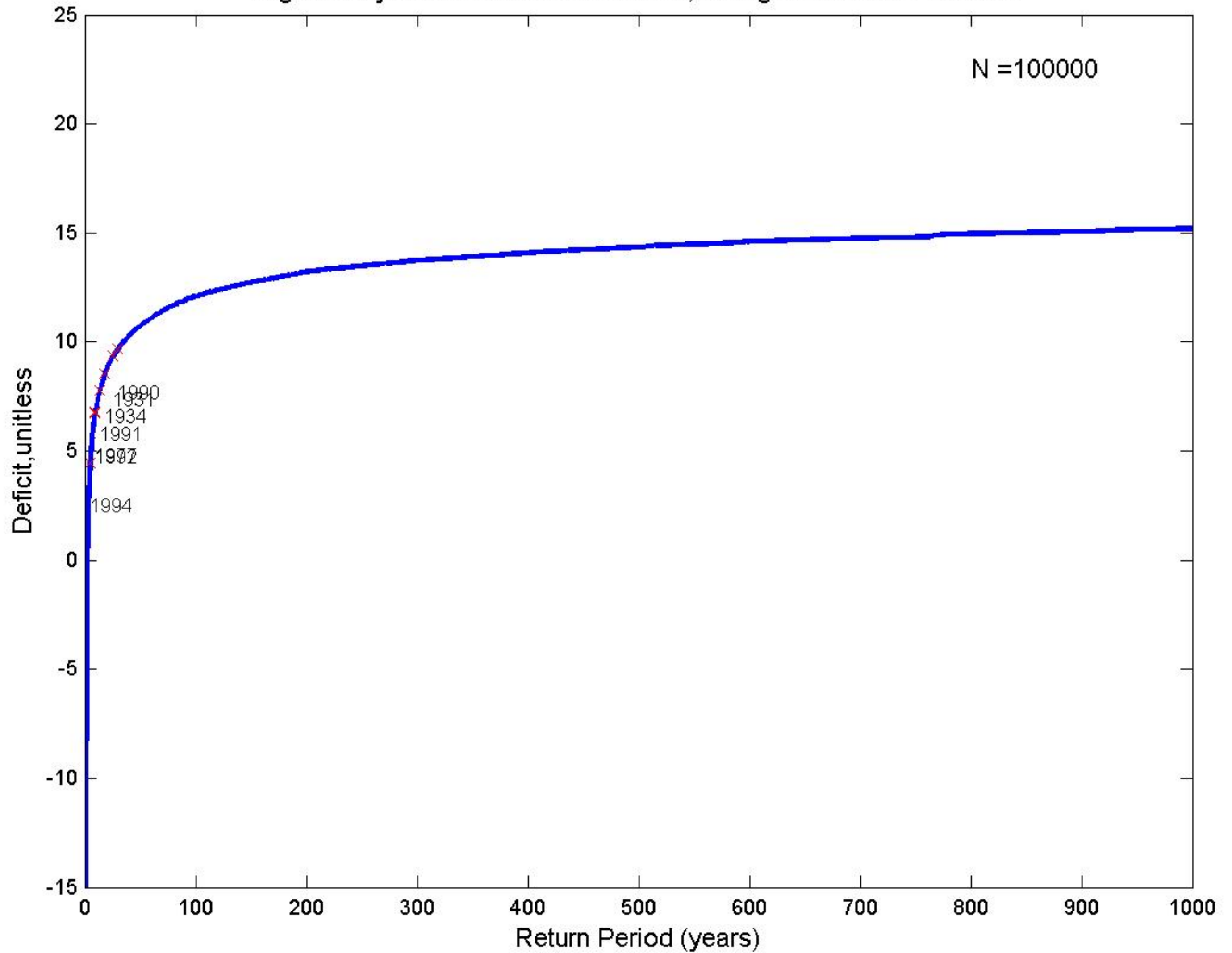
Fig.G17-Synthetic:Four-Year Duration, Drought End-Years Labeled
