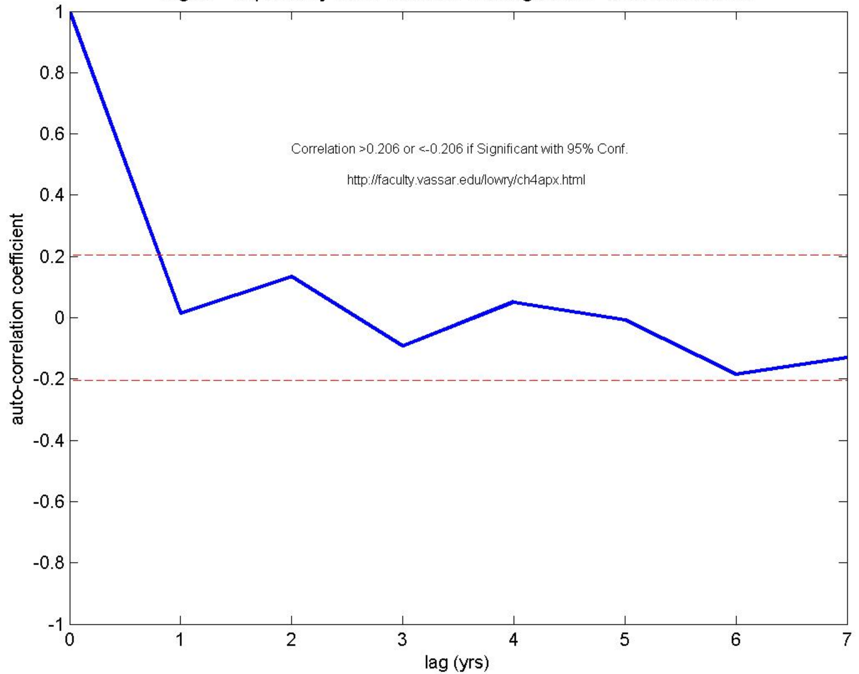
Fig.G7 - Explanatory Term: Consider Autoregression - Check Correlation
