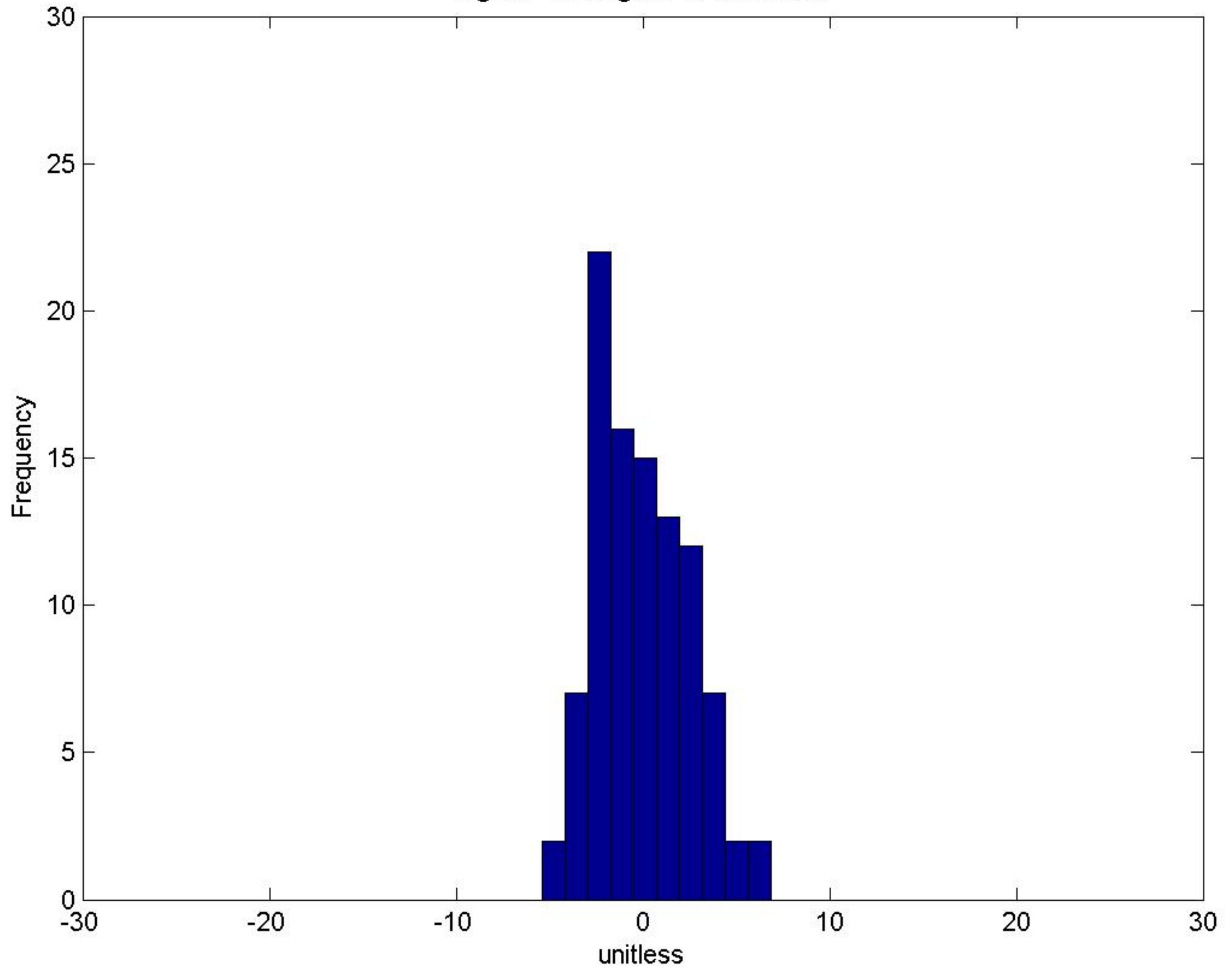
Fig.G9 - Histogram of Observed
