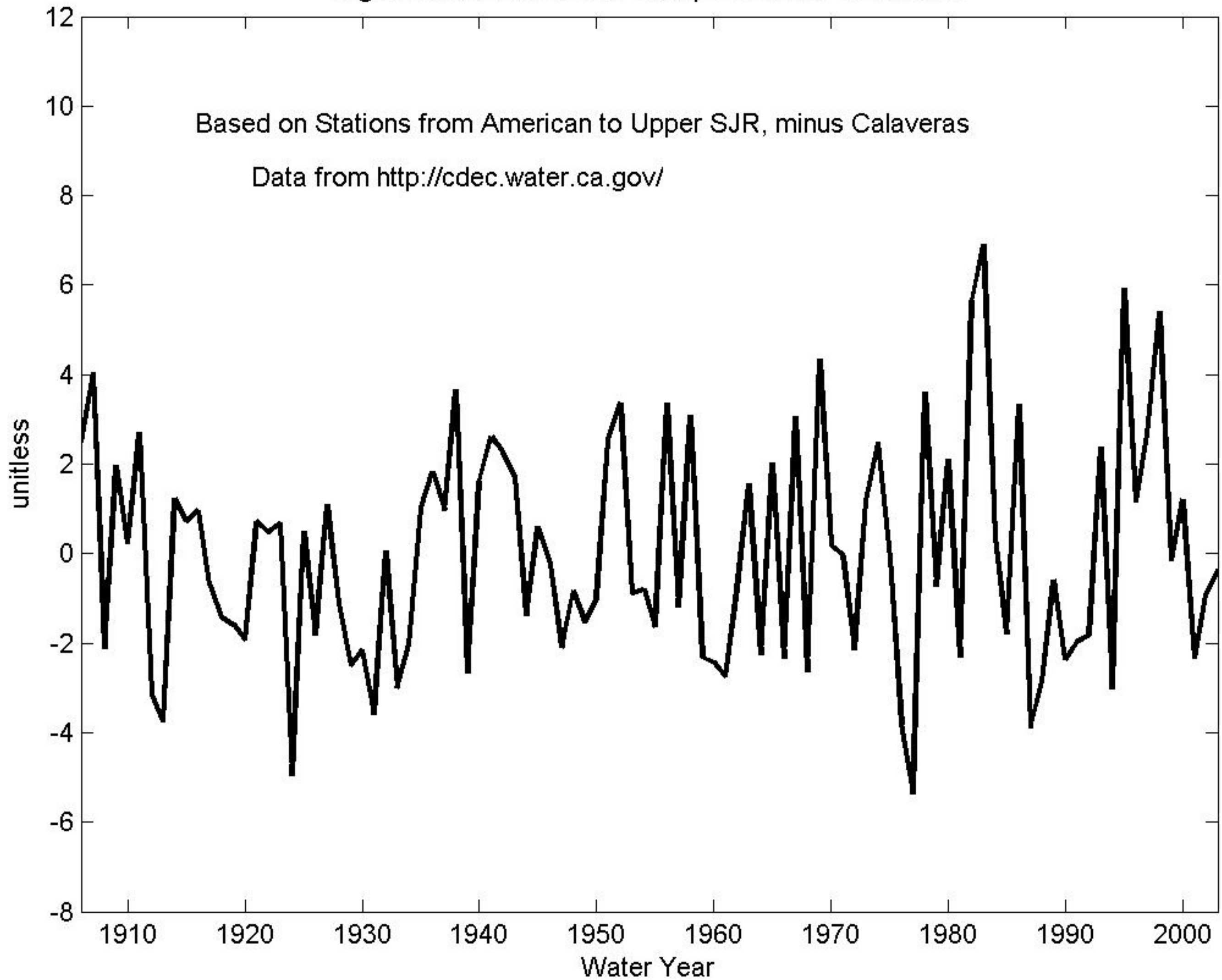
Fig.G1-Observed Annual Precip Index B2: 1906-2003
