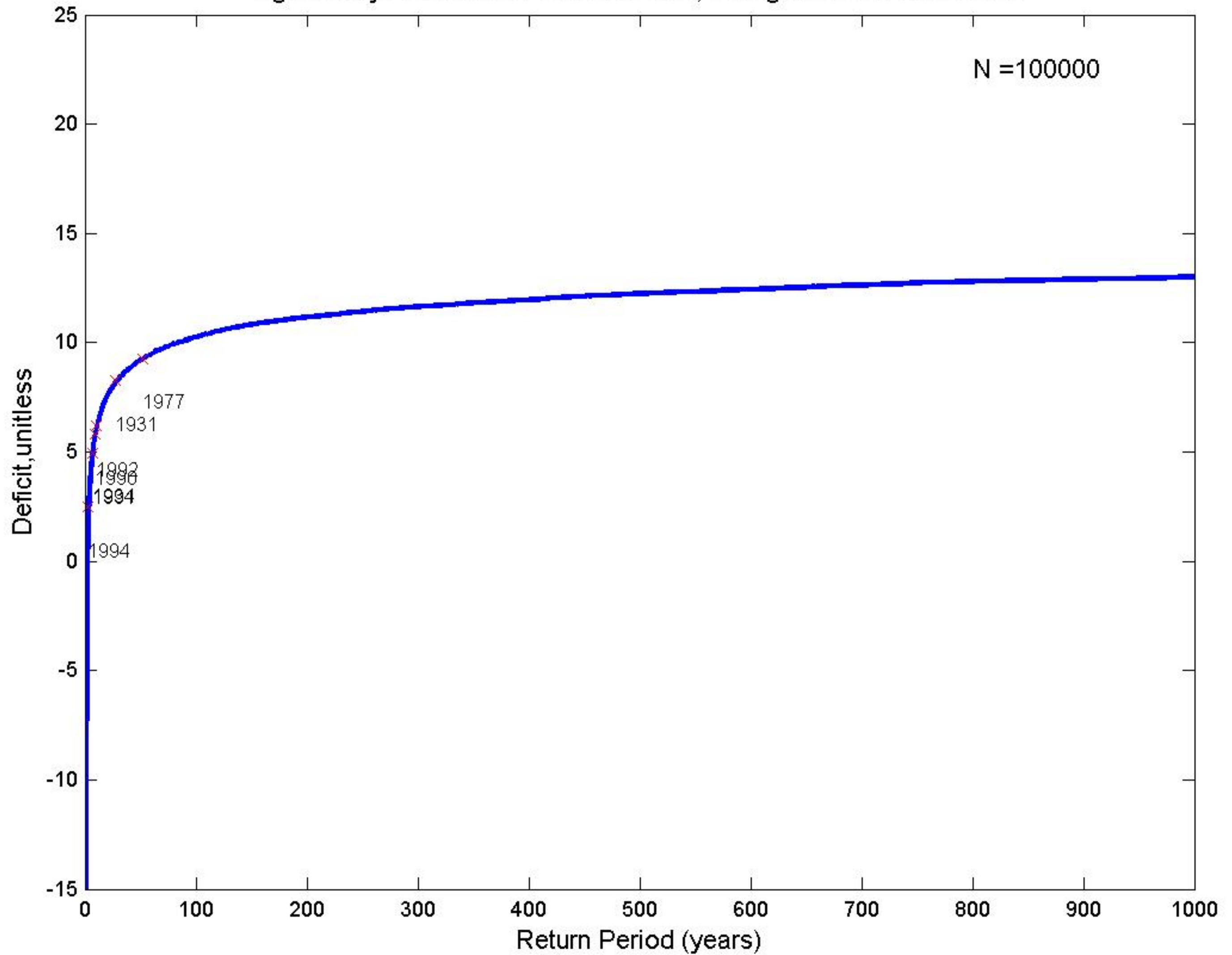
Fig.G16-Synthetic: Three-Year Duration, Drought End-Years Labeled
