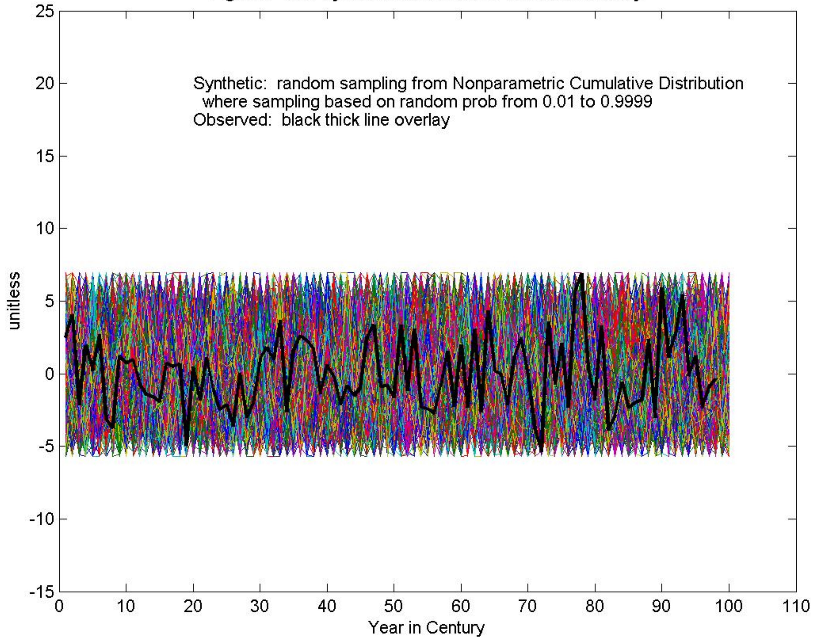
Fig.G12 - 200 Synthetic Centuries and Observed Overlay
