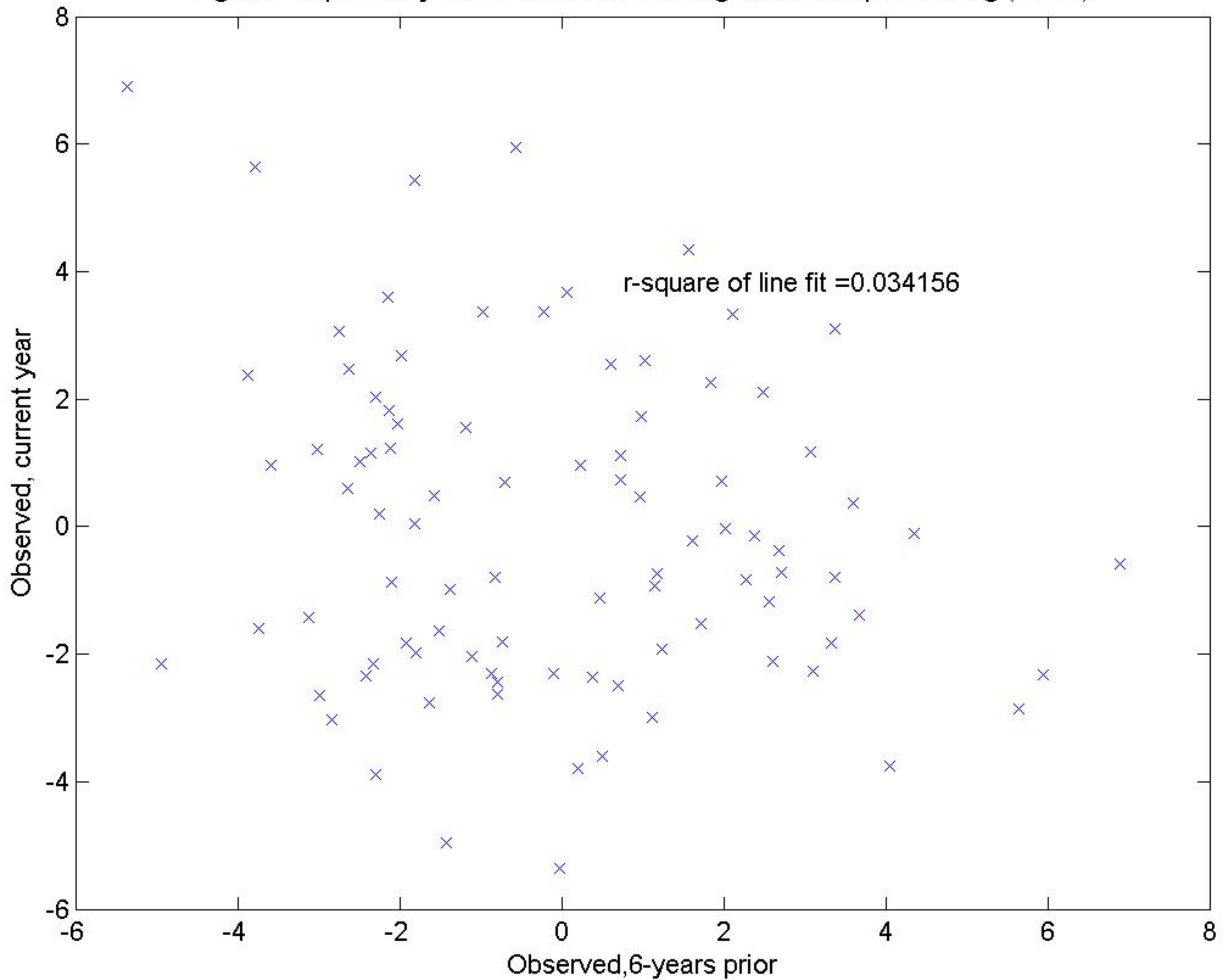
Fig.G8 - Explanatory Term: Consider Autoregression at specified lag (x-axis)
