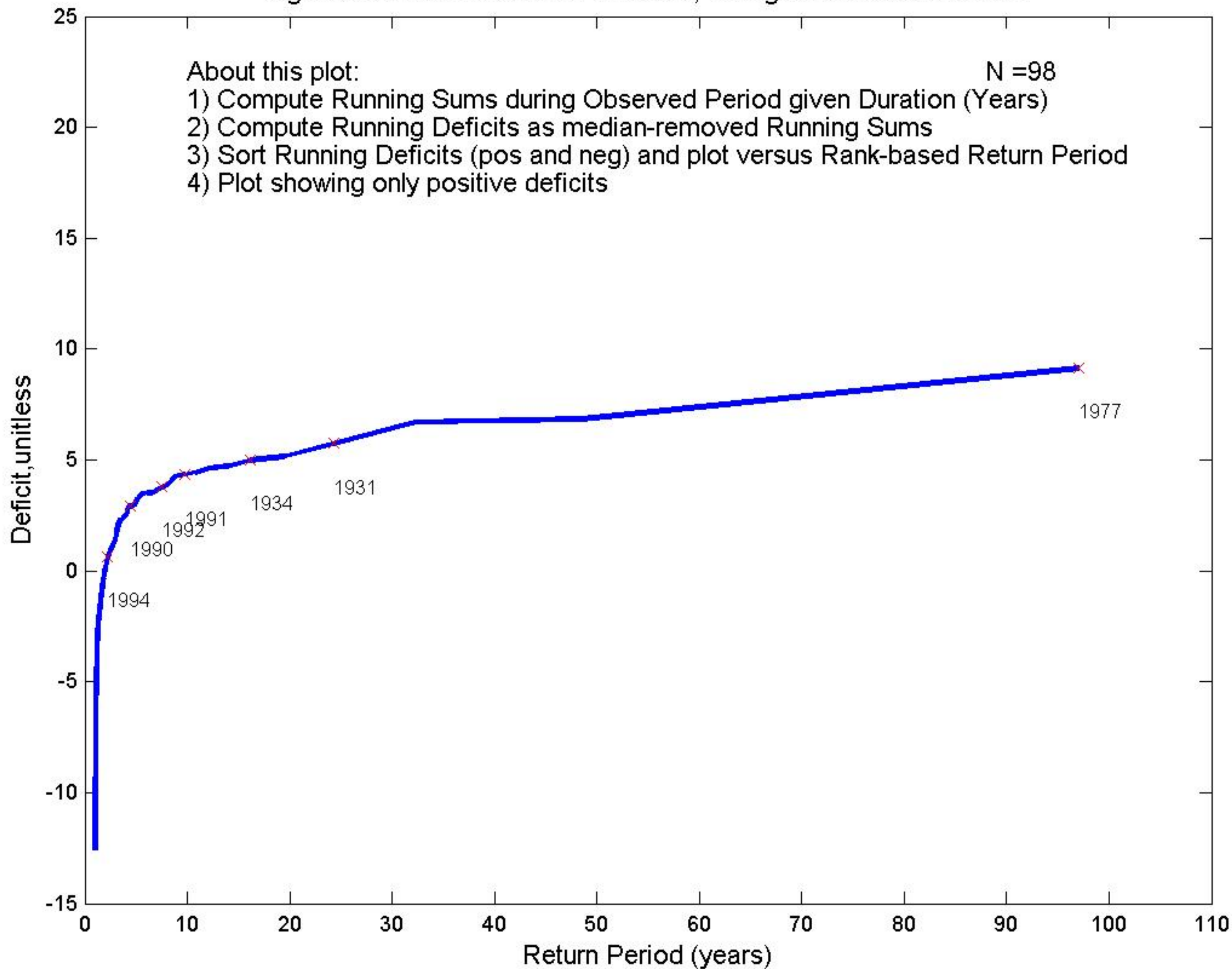
Fig.G2-Observed:Two-Year Duration, Drought End-Years Labeled
