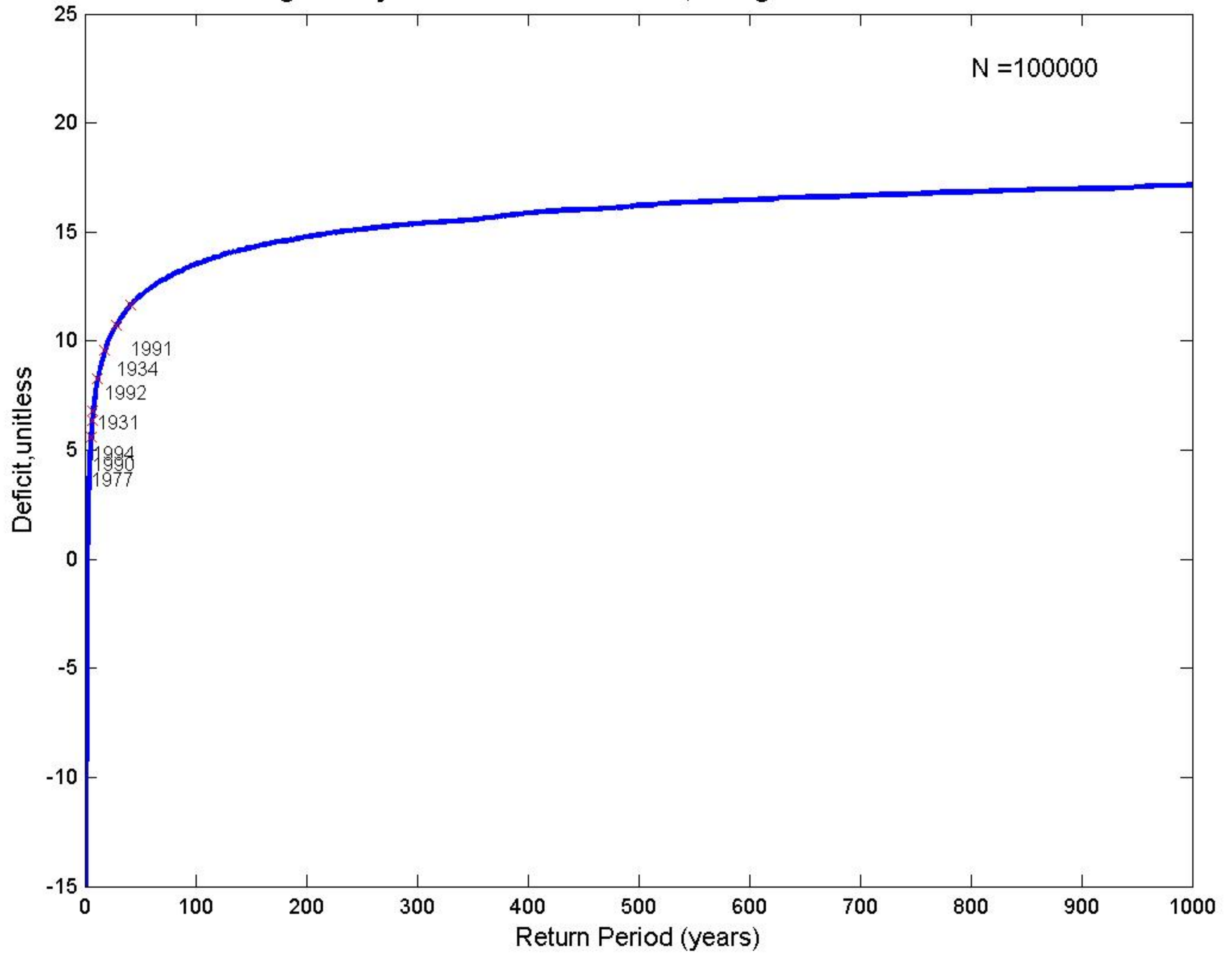
Fig.G18-Synthetic:Five-Year Duration, Drought End-Years Labeled
