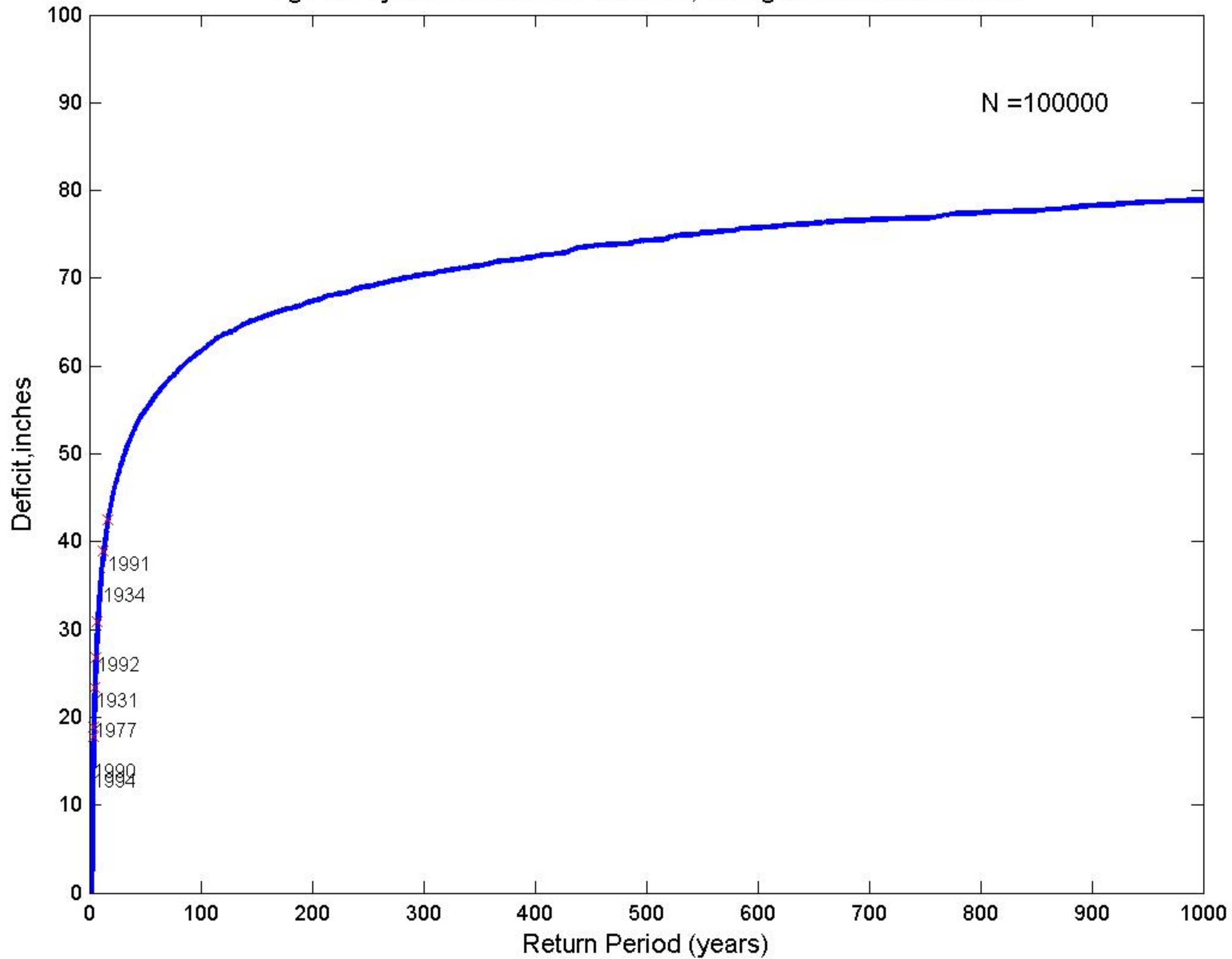
Fig.F18-Synthetic:Five-Year Duration, Drought End-Years Labeled
