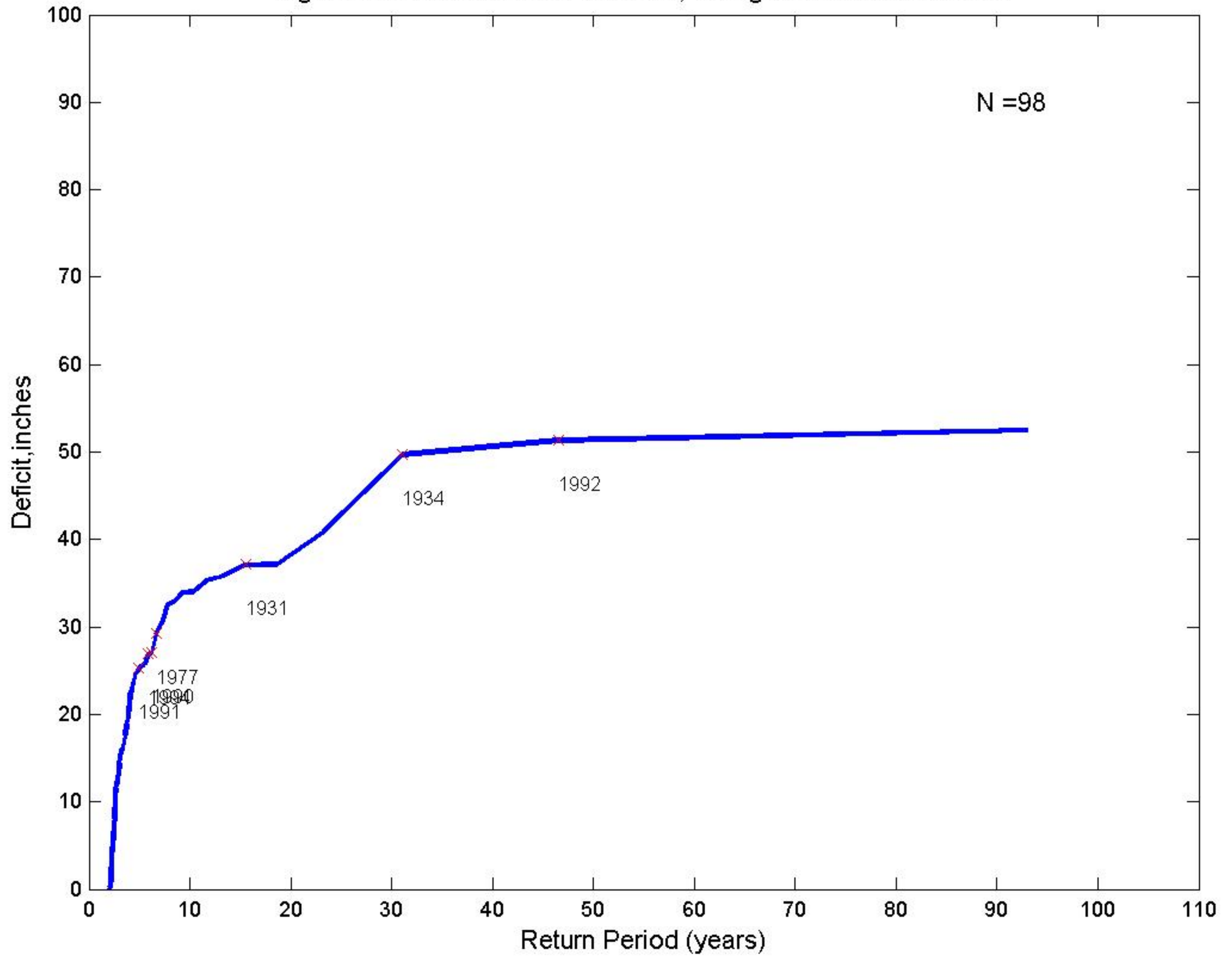
Fig.F6-Observed:Six-Year Duration, Drought End-Years Labeled
