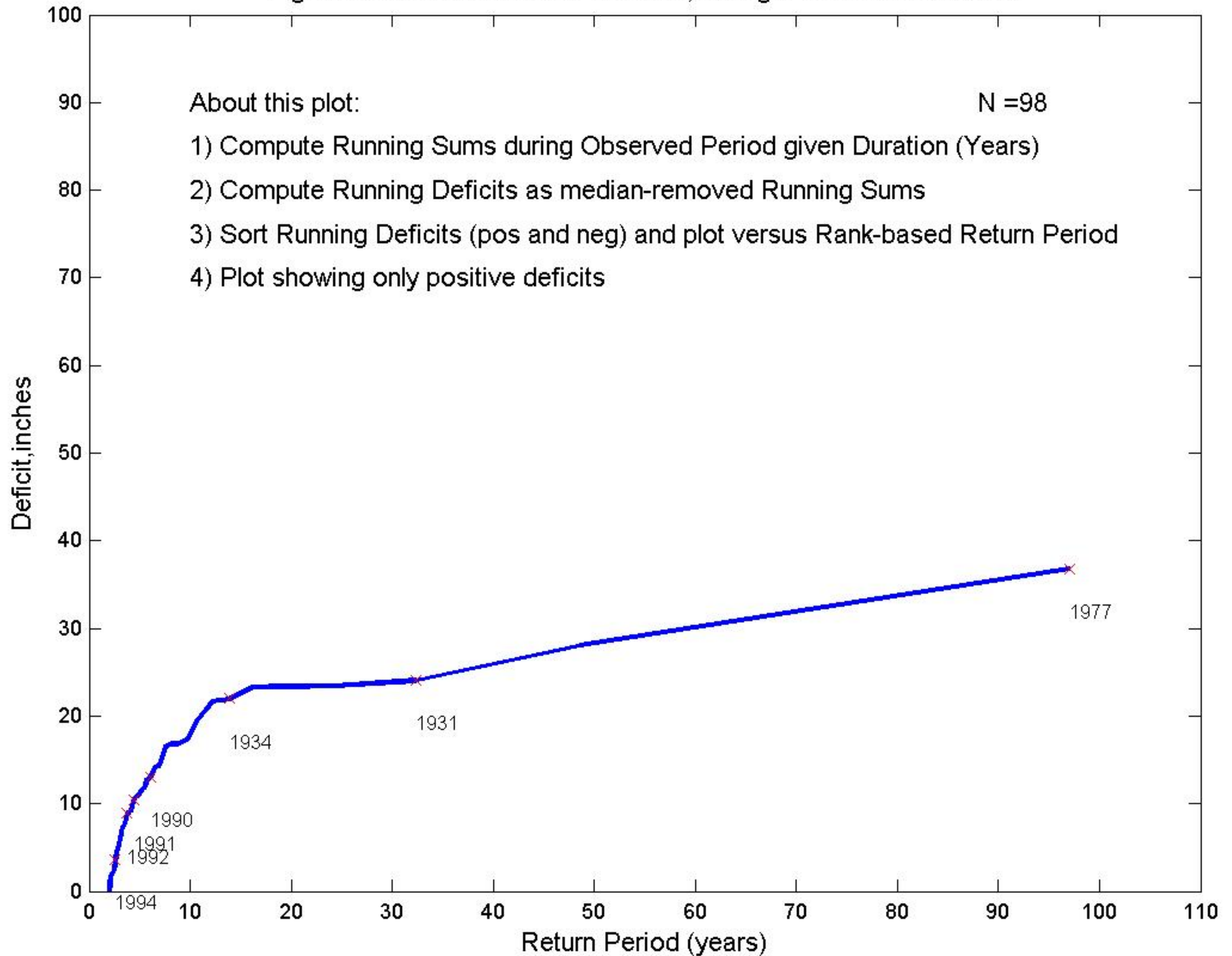
Fig.F2-Observed:Two-Year Duration, Drought End-Years Labeled
