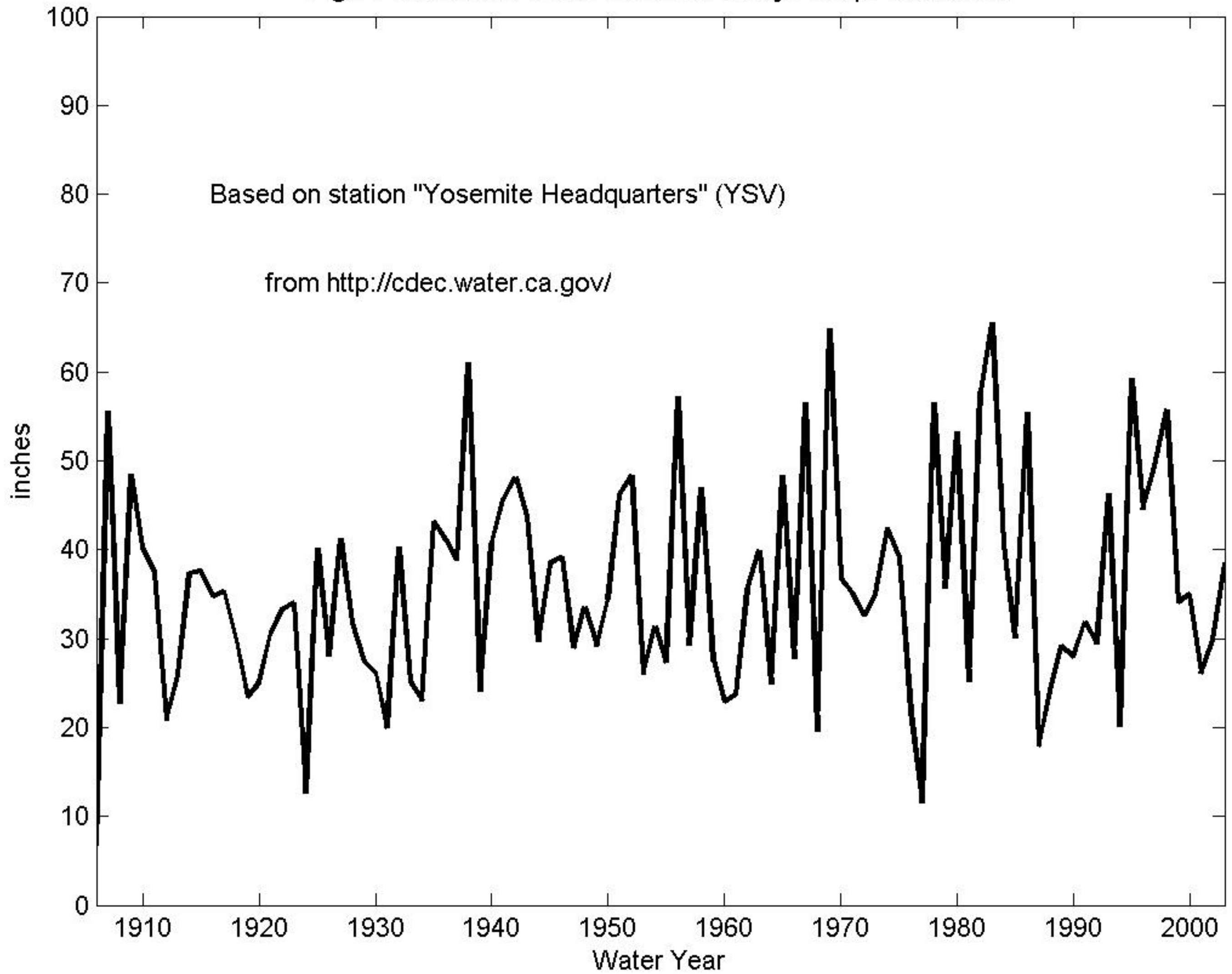
Fig.F1-Observed Annual Yosemite Valley Precip: 1906-2003
