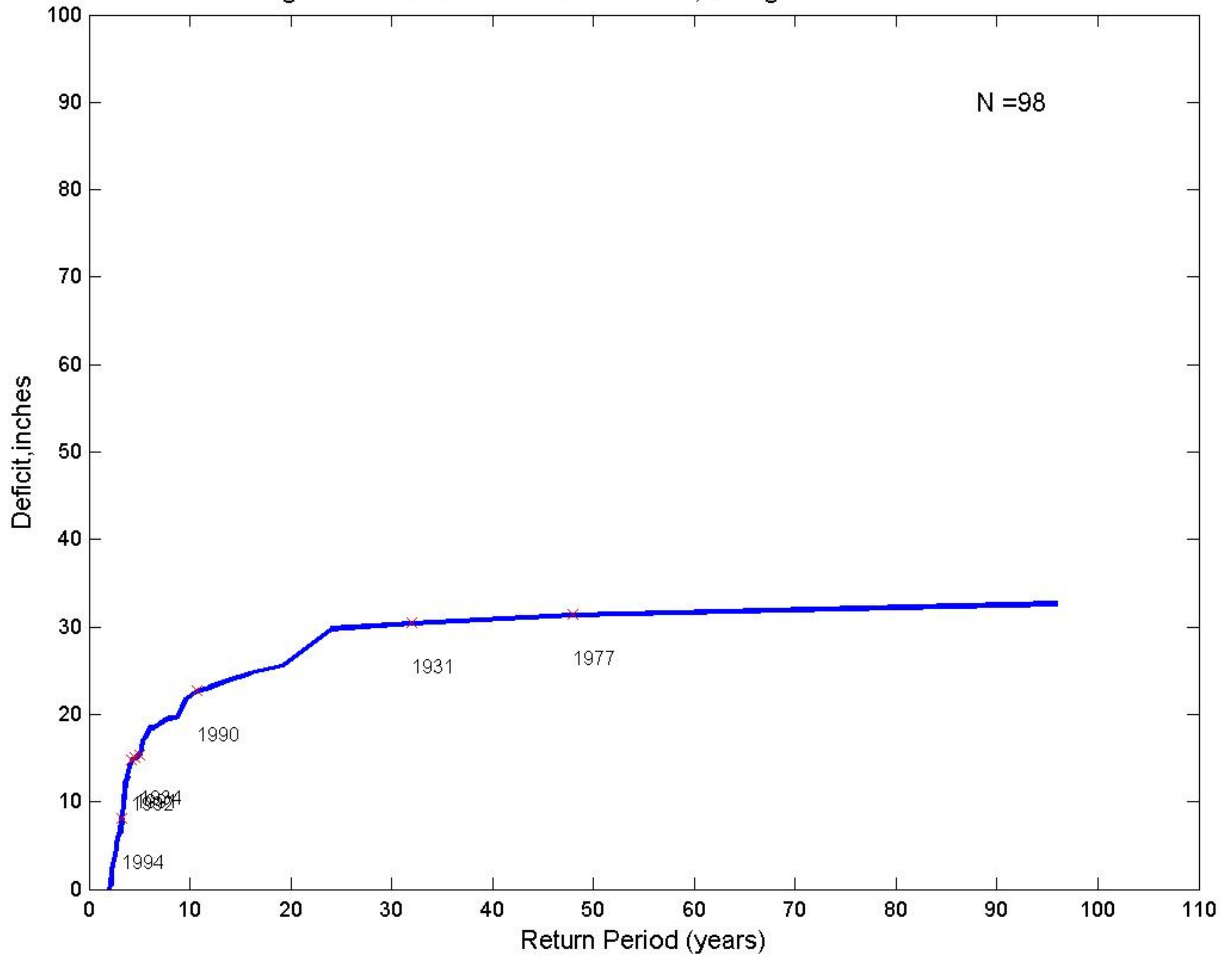
Fig.F3-Observed:Three-Year Duration, Drought End-Years Labeled
