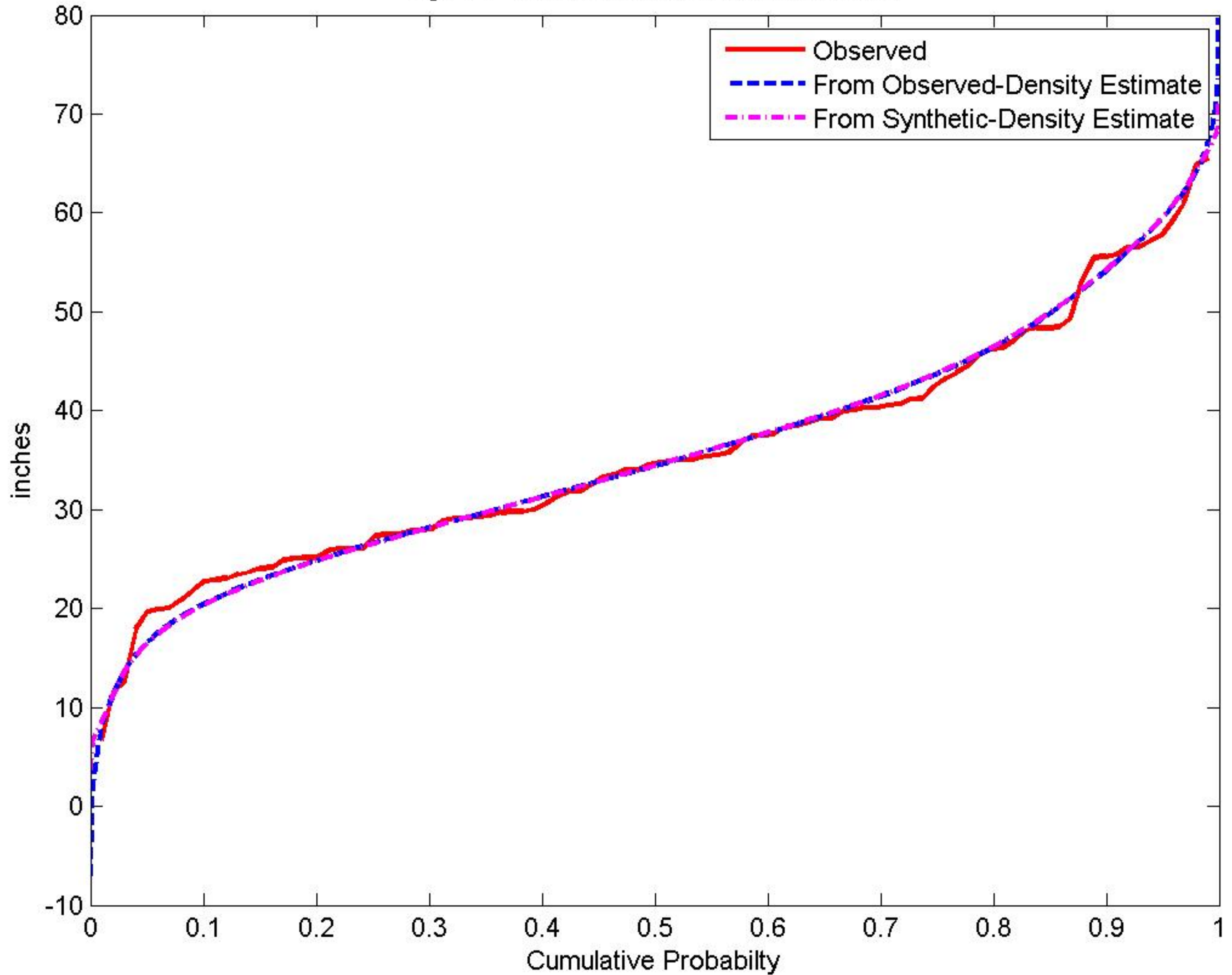
Fig.F14 - Cumulative Distribution Functions
