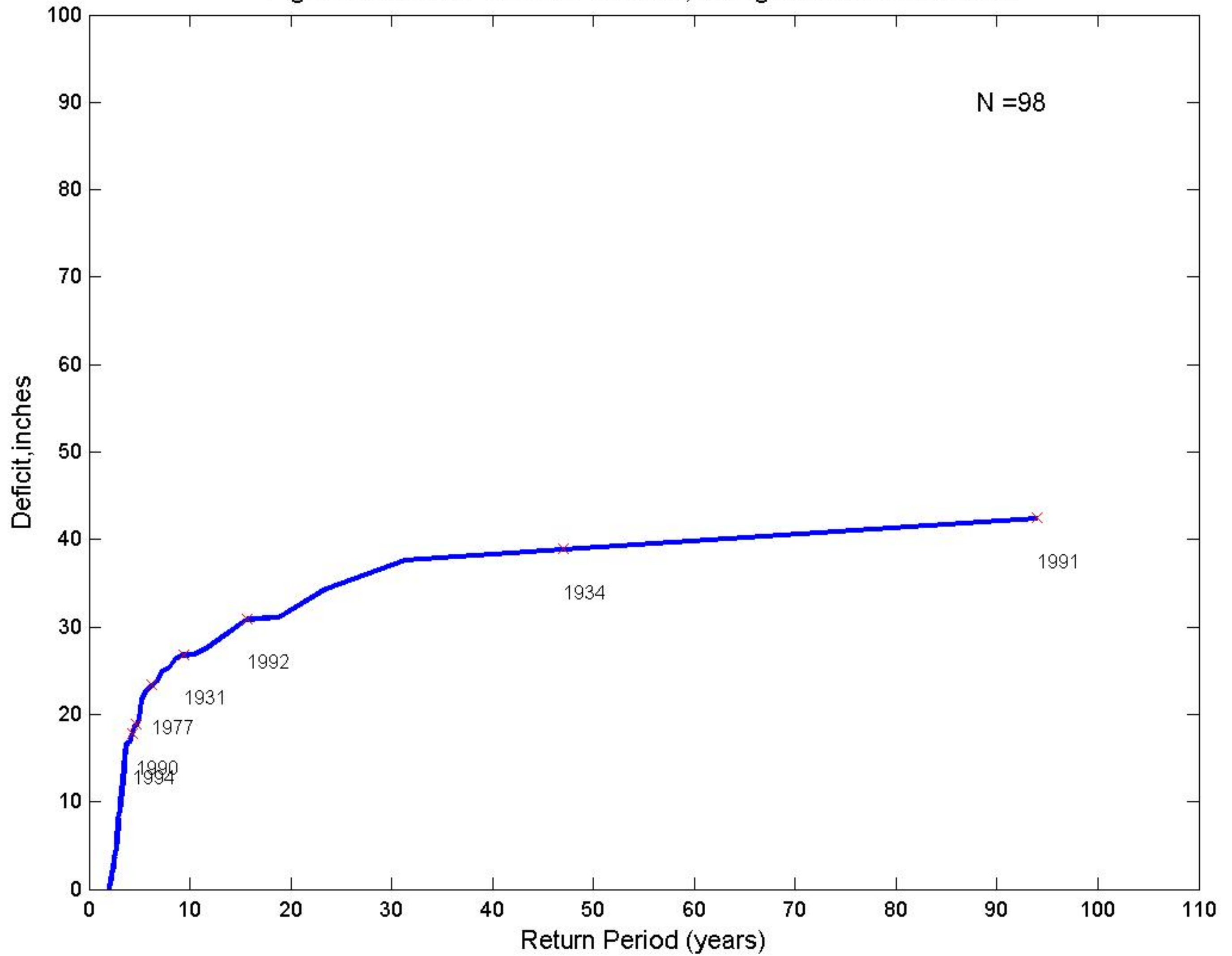
Fig.F5-Observed:Five-Year Duration, Drought End-Years Labeled
