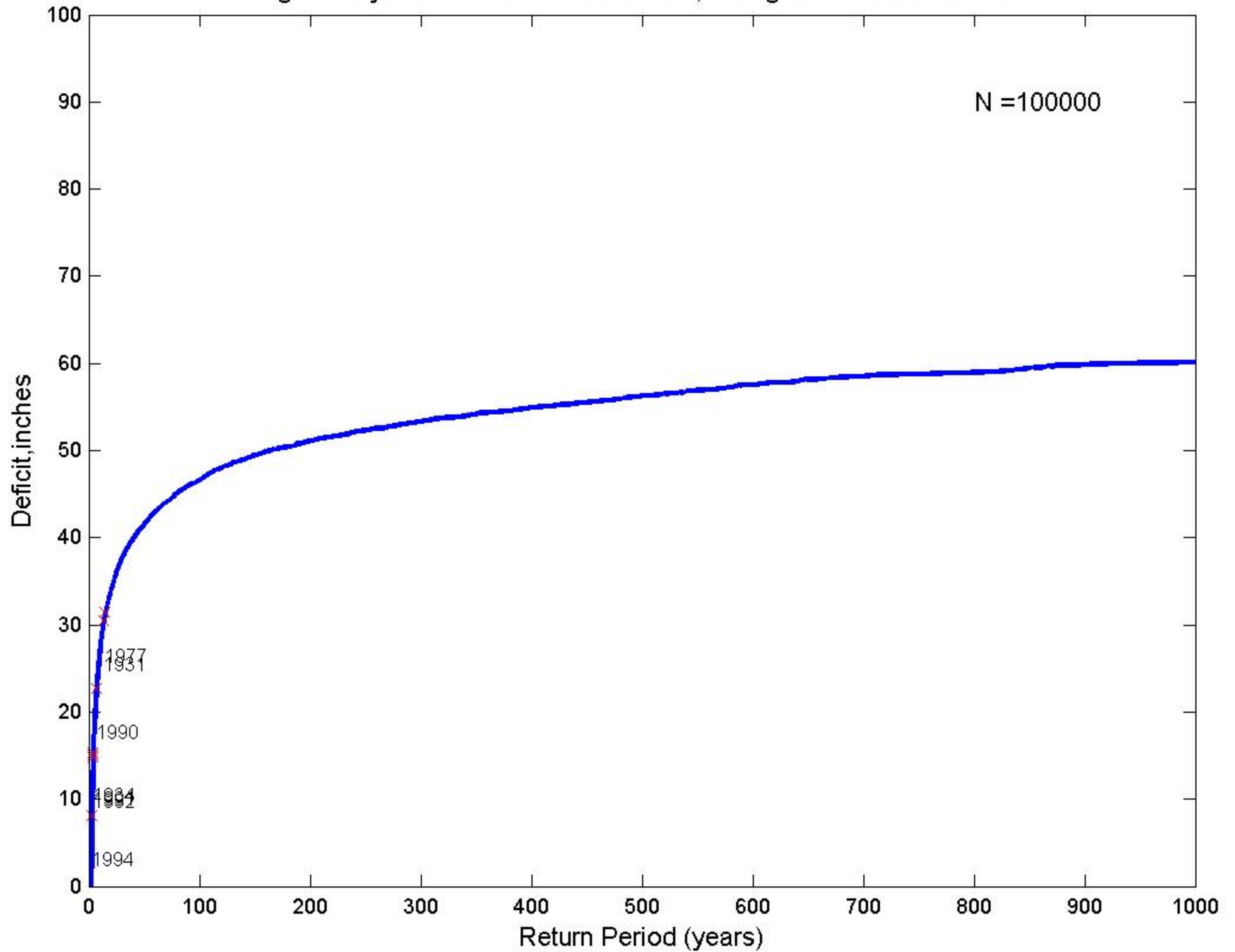
Fig.F16-Synthetic: Three-Year Duration, Drought End-Years Labeled
