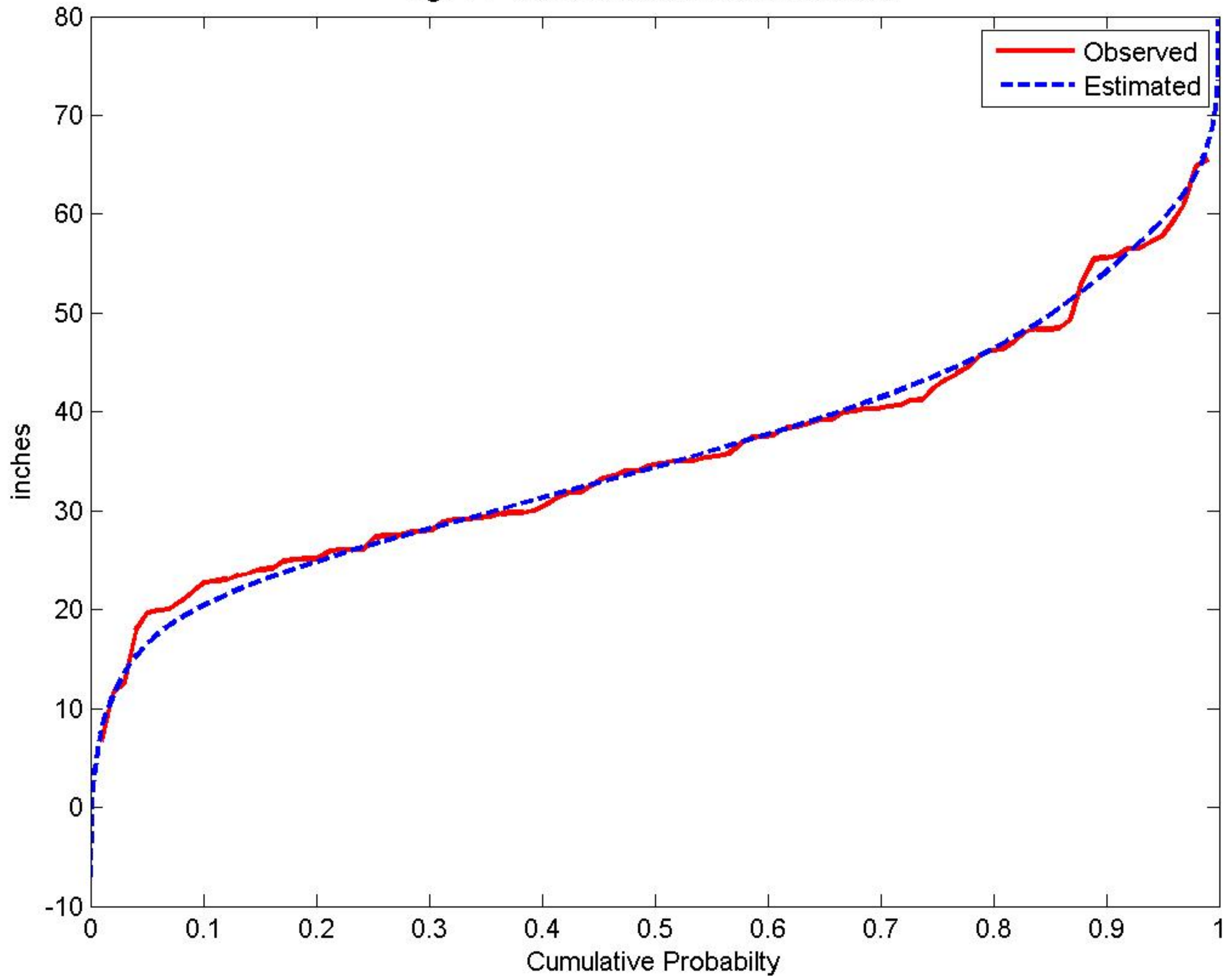
Fig.F11 - Cumulative Distribution Functions
