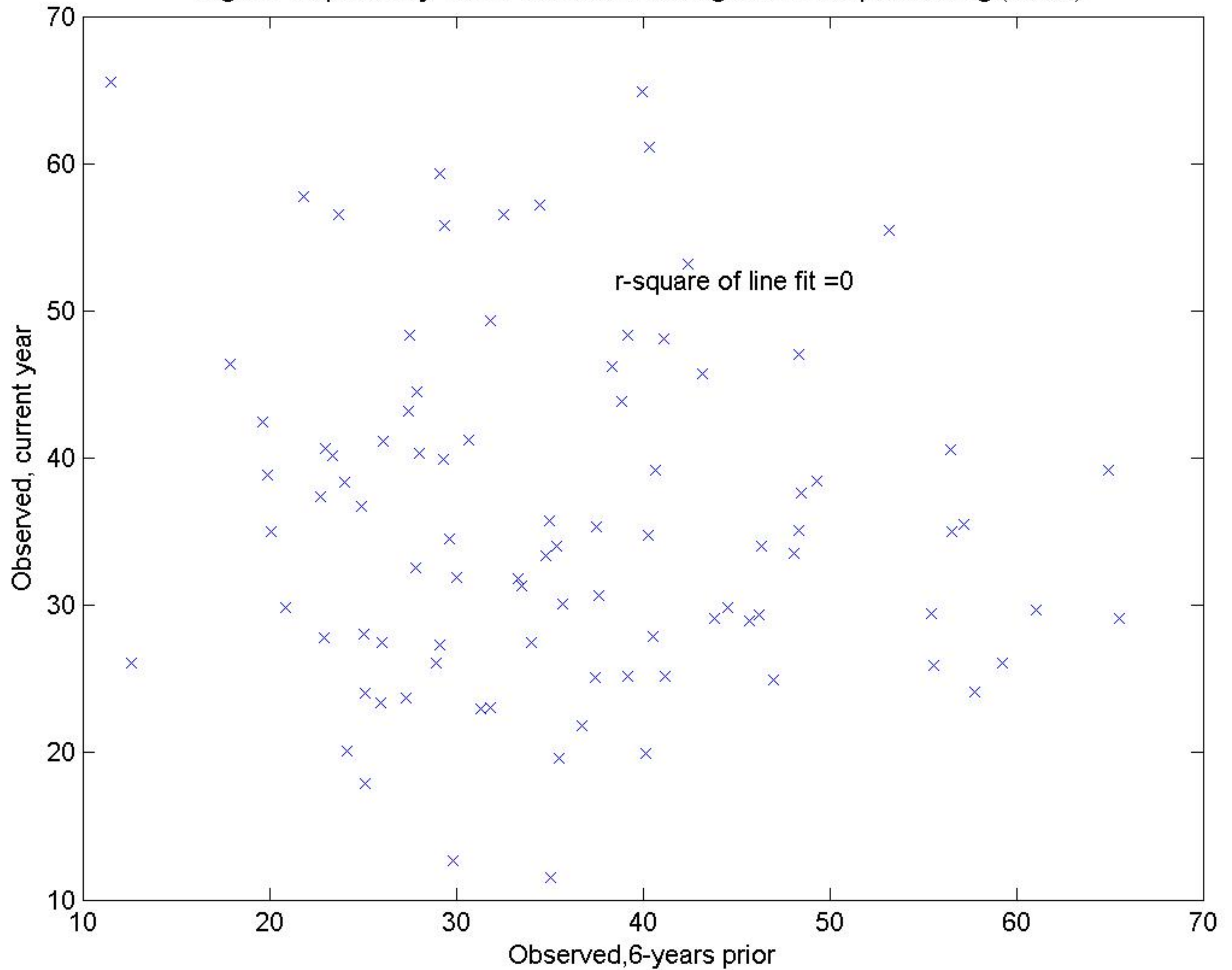
Fig.F8 - Explanatory Term: Consider Autoregression at specified lag (x-axis)
