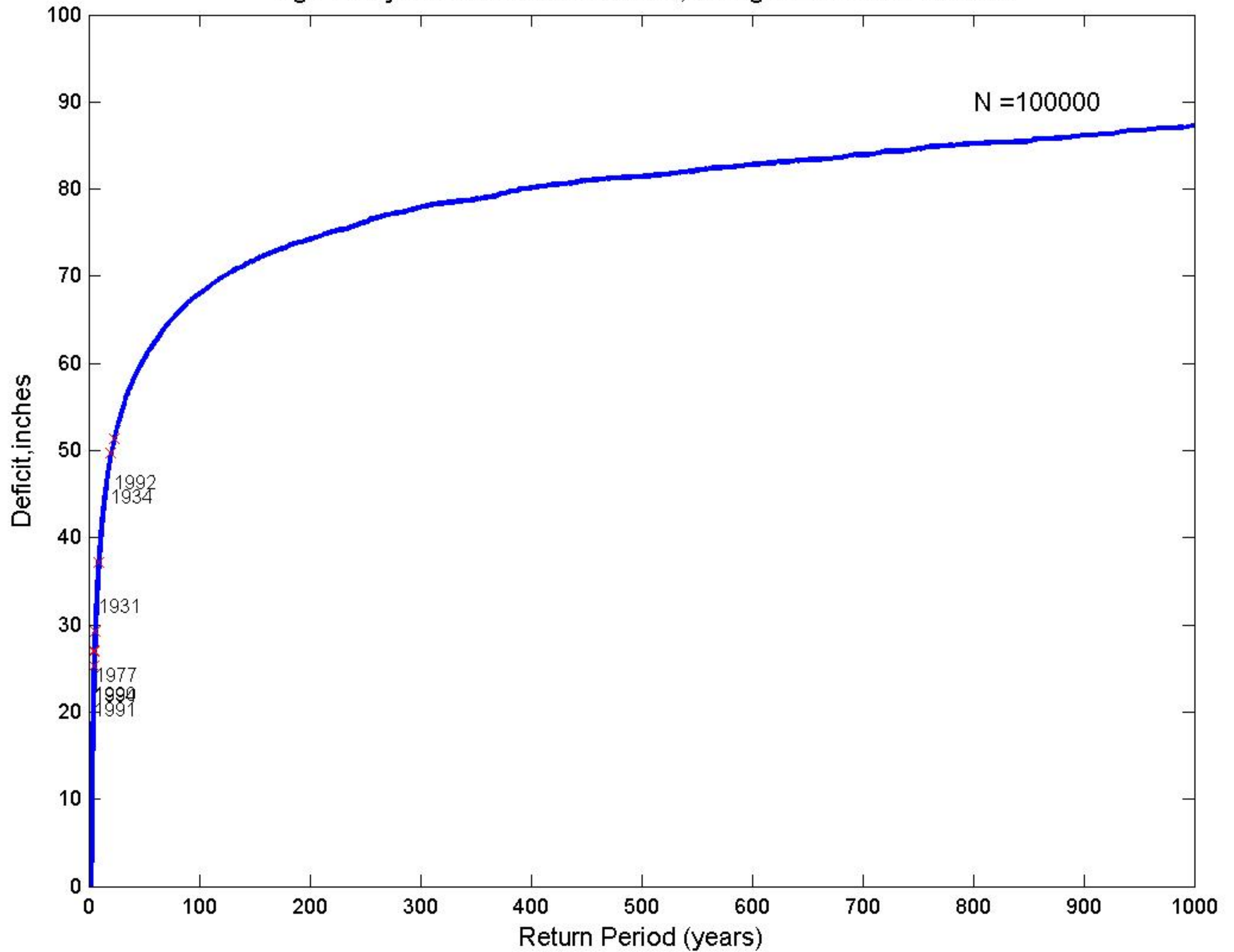
Fig.F19-Synthetic:Six-Year Duration, Drought End-Years Labeled
