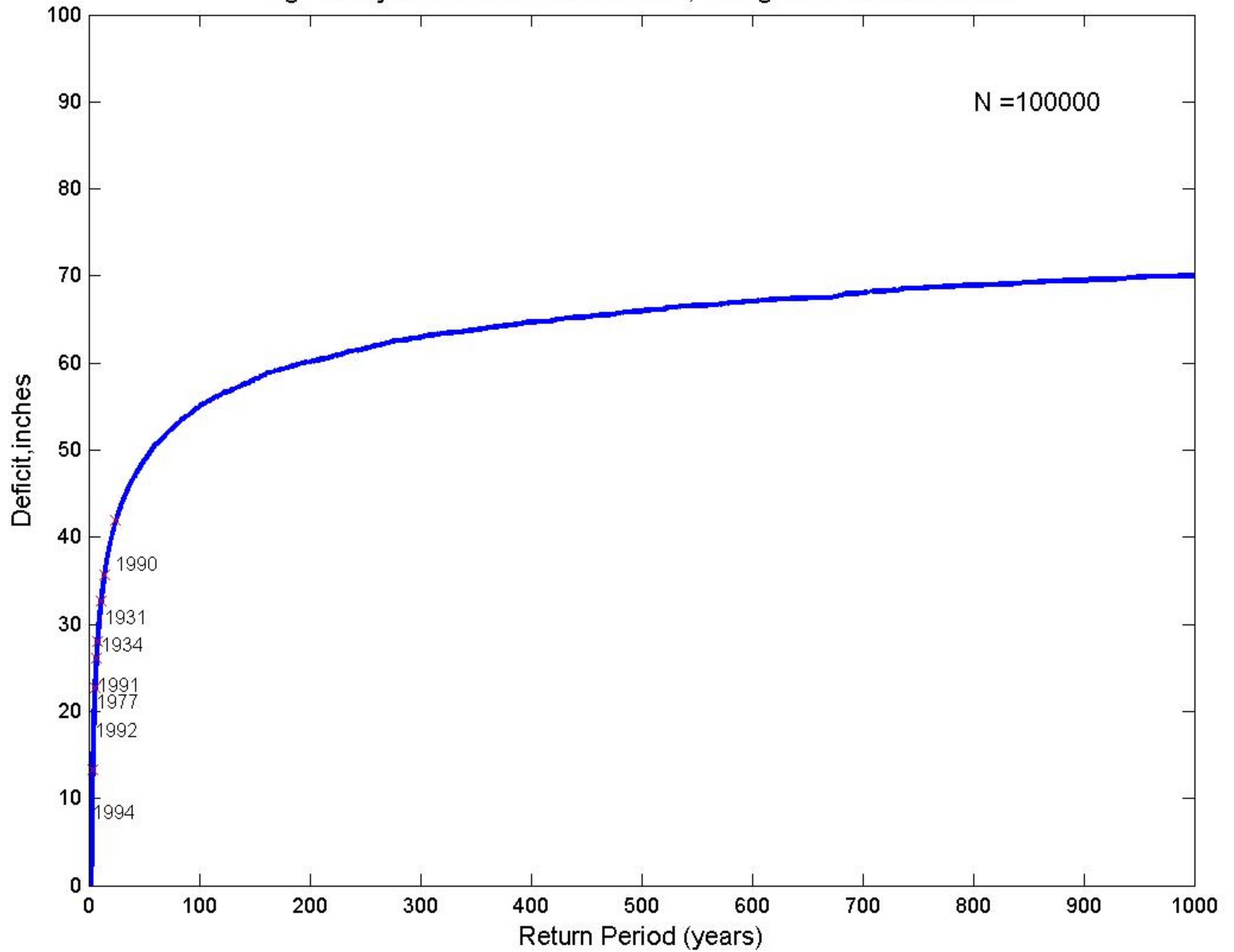
Fig.F17-Synthetic:Four-Year Duration, Drought End-Years Labeled
