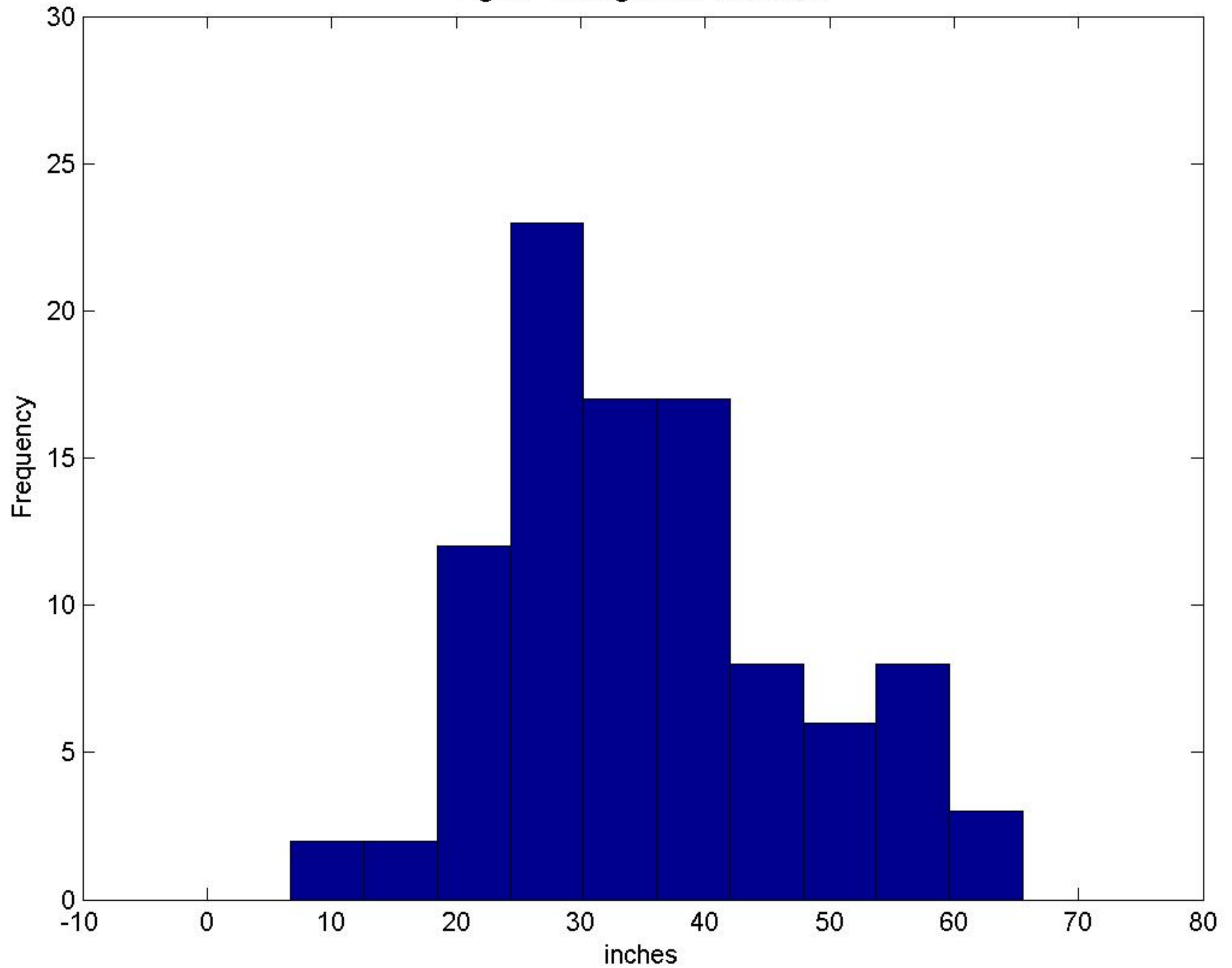
Fig.F9 - Histogram of Observed
