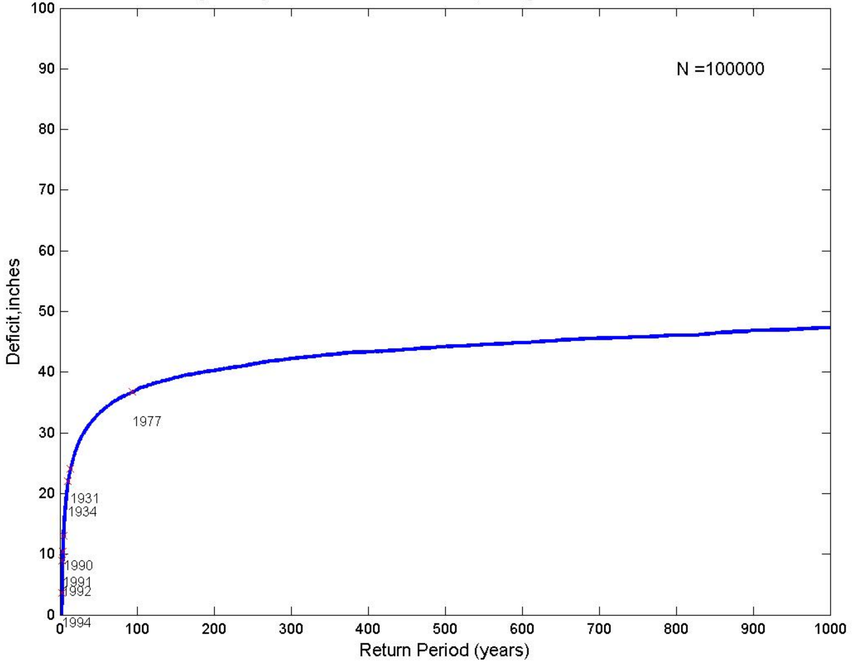
Fig.F15-Synthetic:Two-Year Duration, Drought End-Years Labeled
