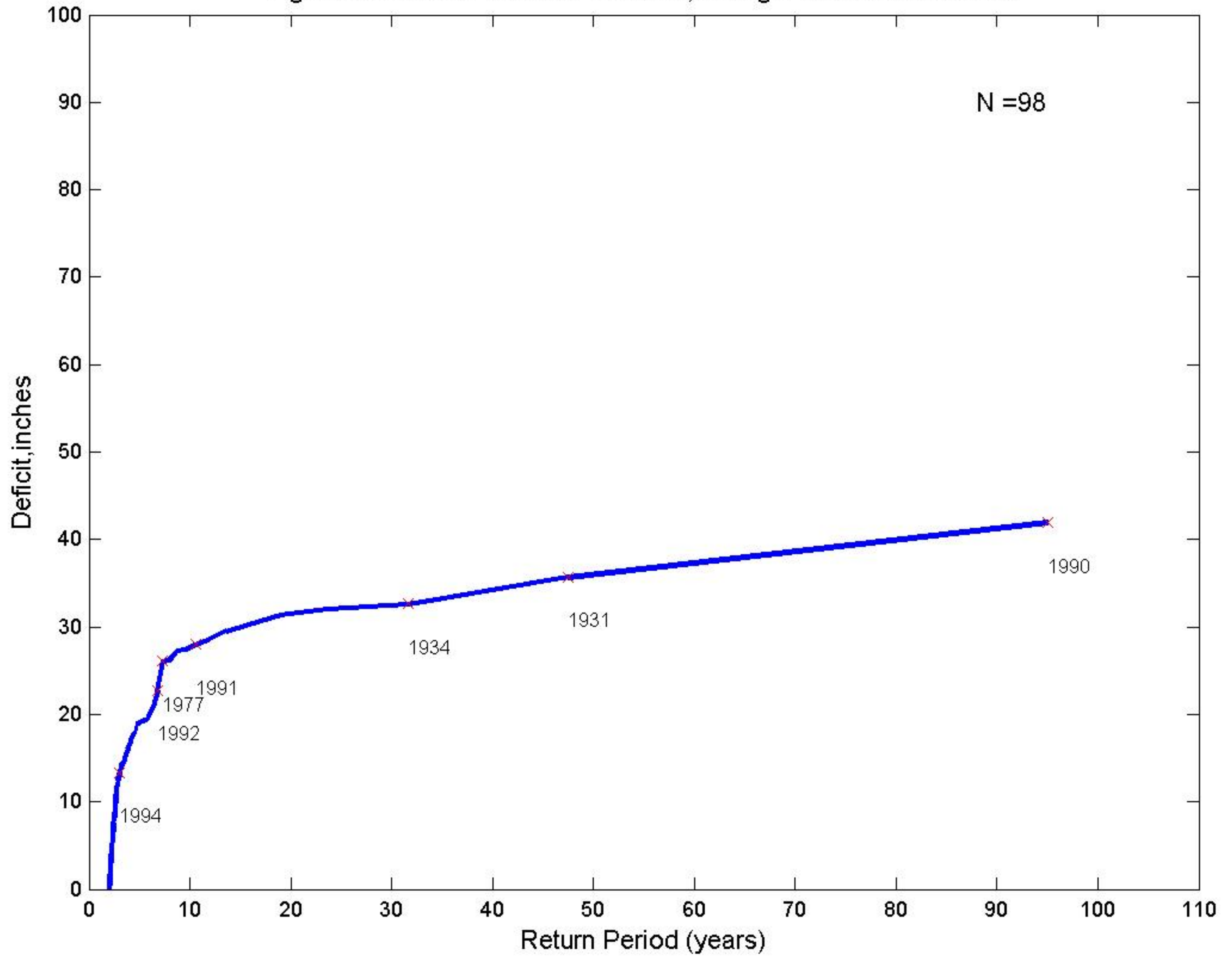
Fig.F4-Observed:Four-Year Duration, Drought End-Years Labeled
