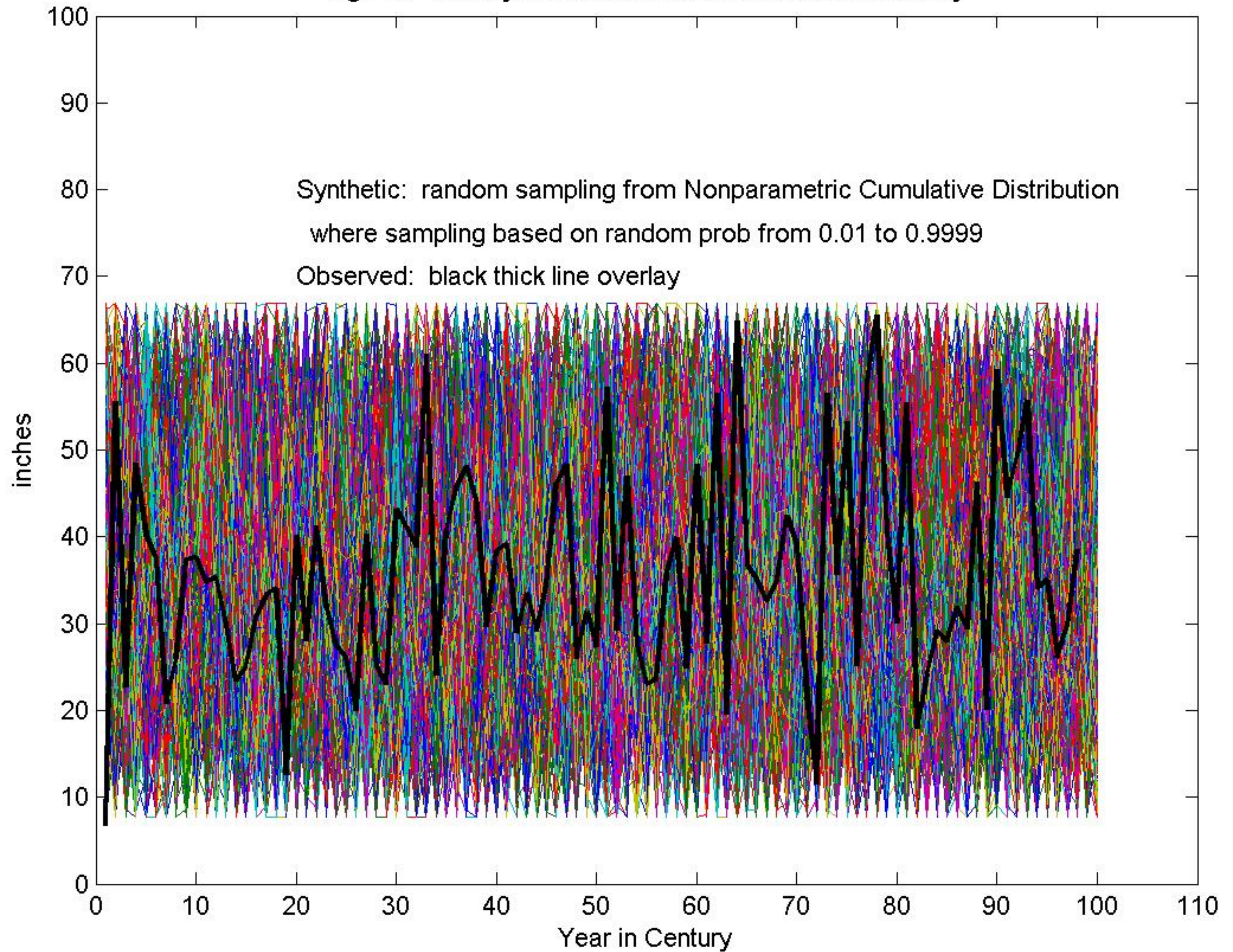
Fig.F12 - 200 Synthetic Centuries and Observed Overlay
