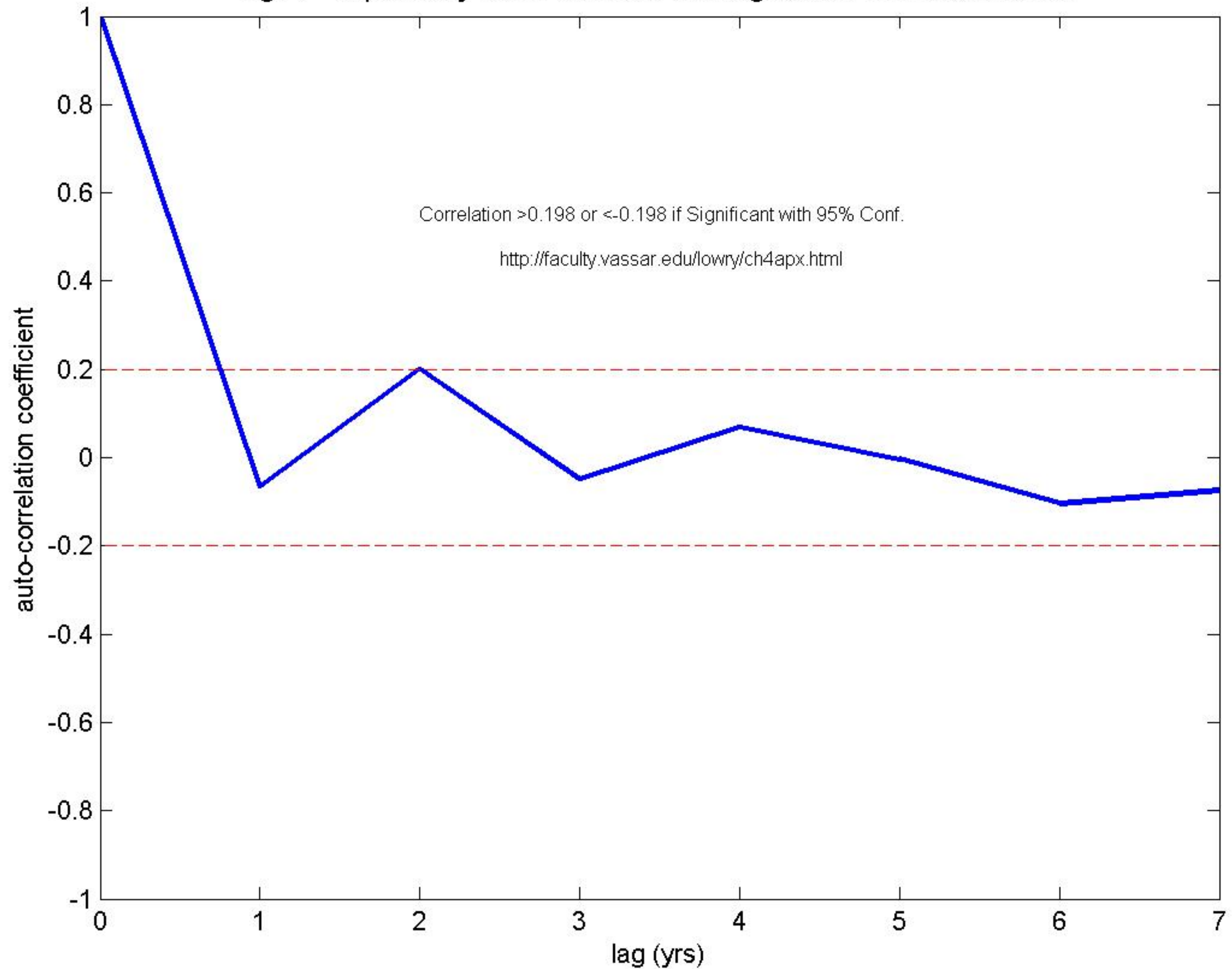
Fig.F7 - Explanatory Term: Consider Autoregression - Check Correlation
