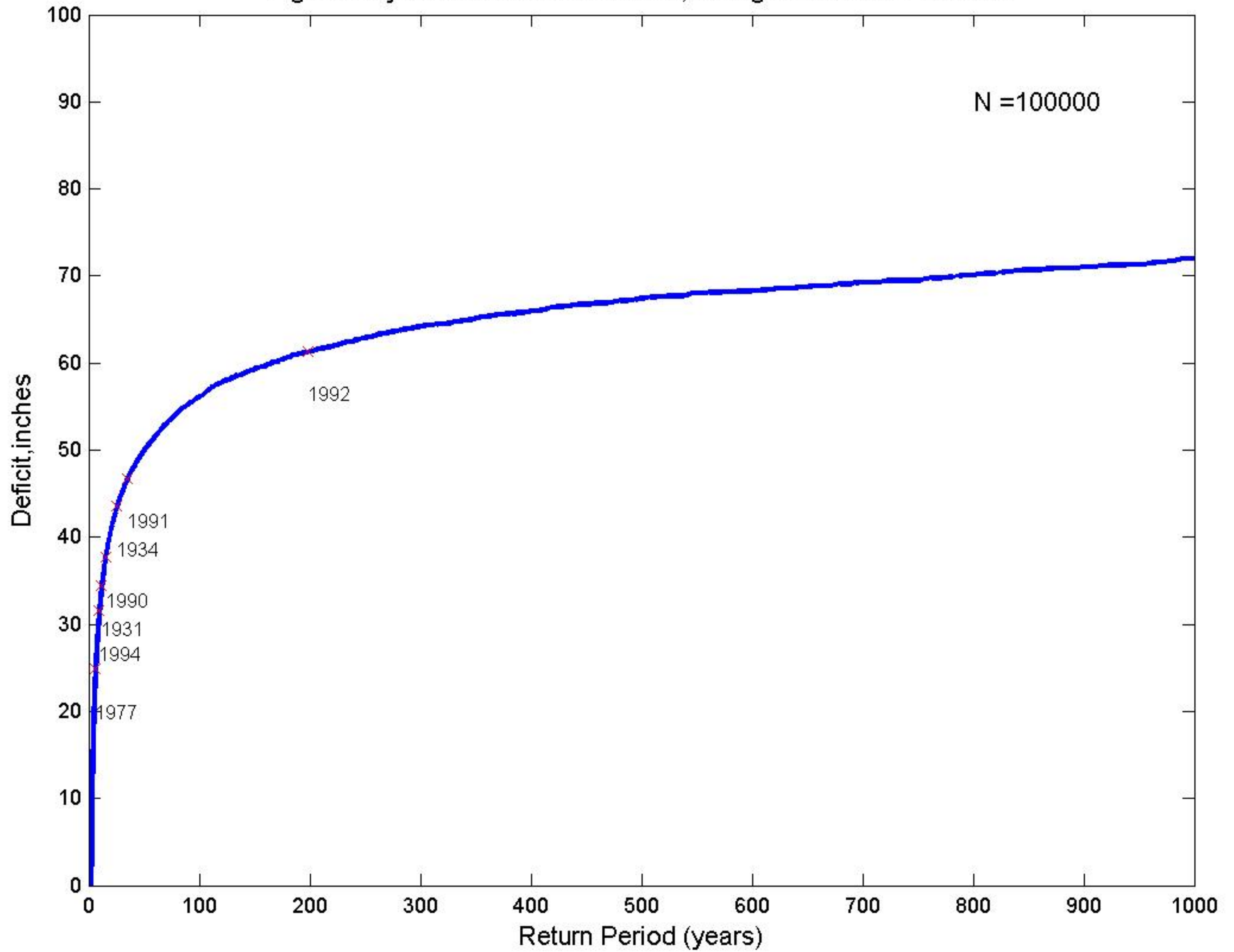
Fig.D19-Synthetic:Six-Year Duration, Drought End-Years Labeled
