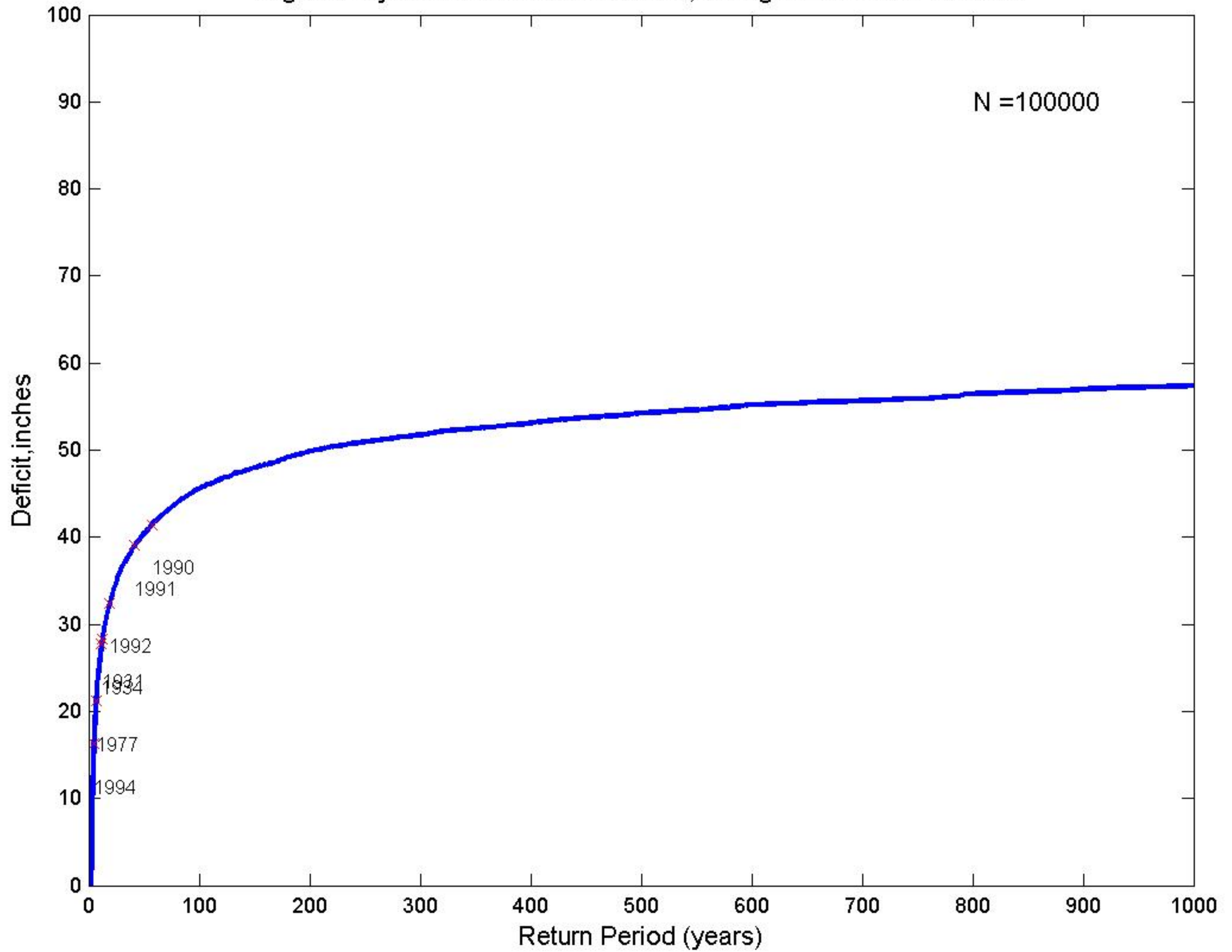
Fig.D17-Synthetic:Four-Year Duration, Drought End-Years Labeled
