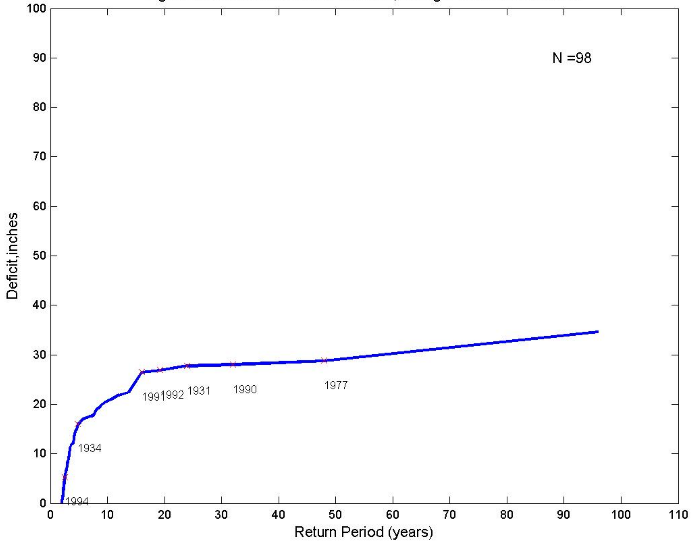
Fig.D3-Observed:Three-Year Duration, Drought End-Years Labeled
