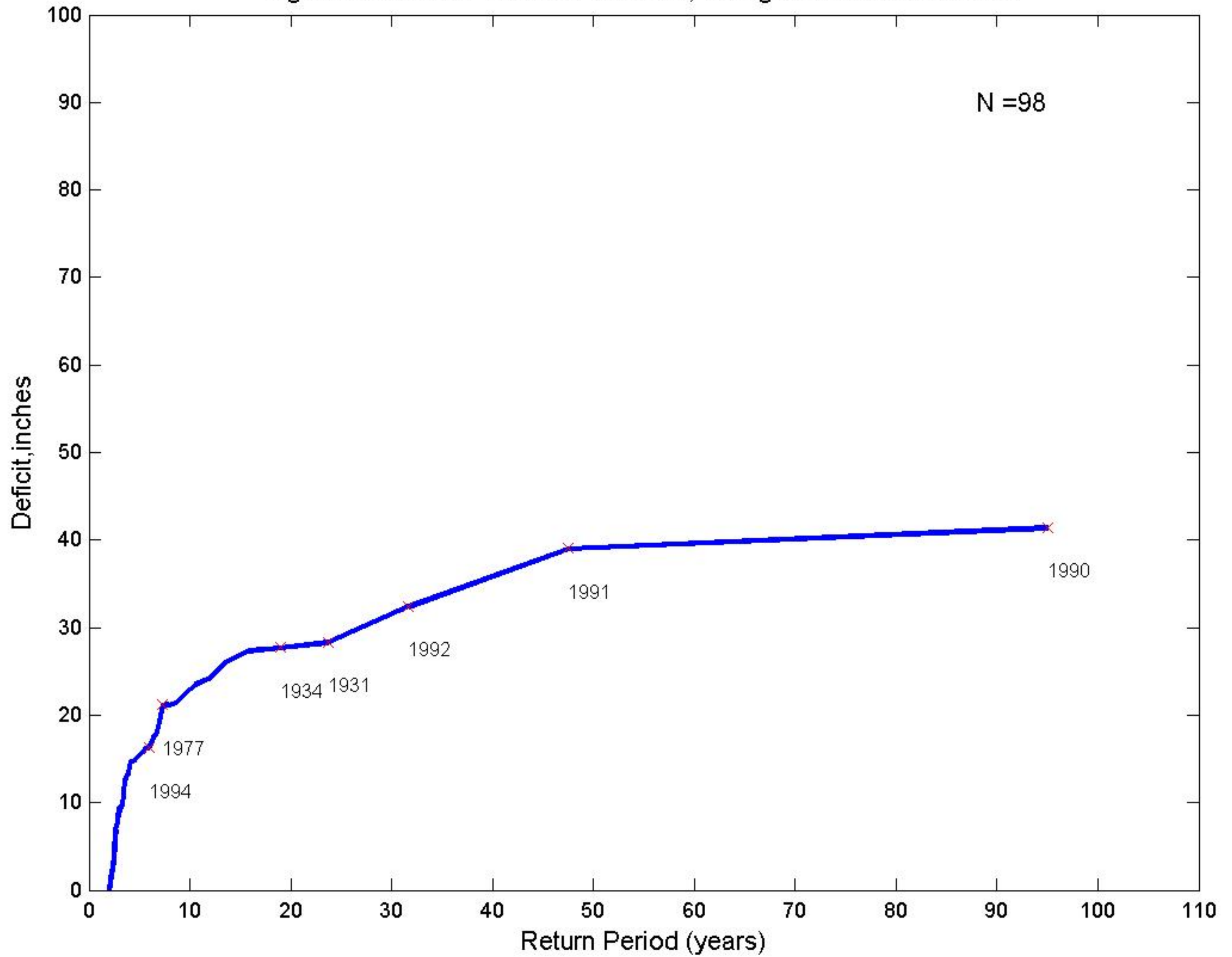
Fig.D4-Observed:Four-Year Duration, Drought End-Years Labeled
