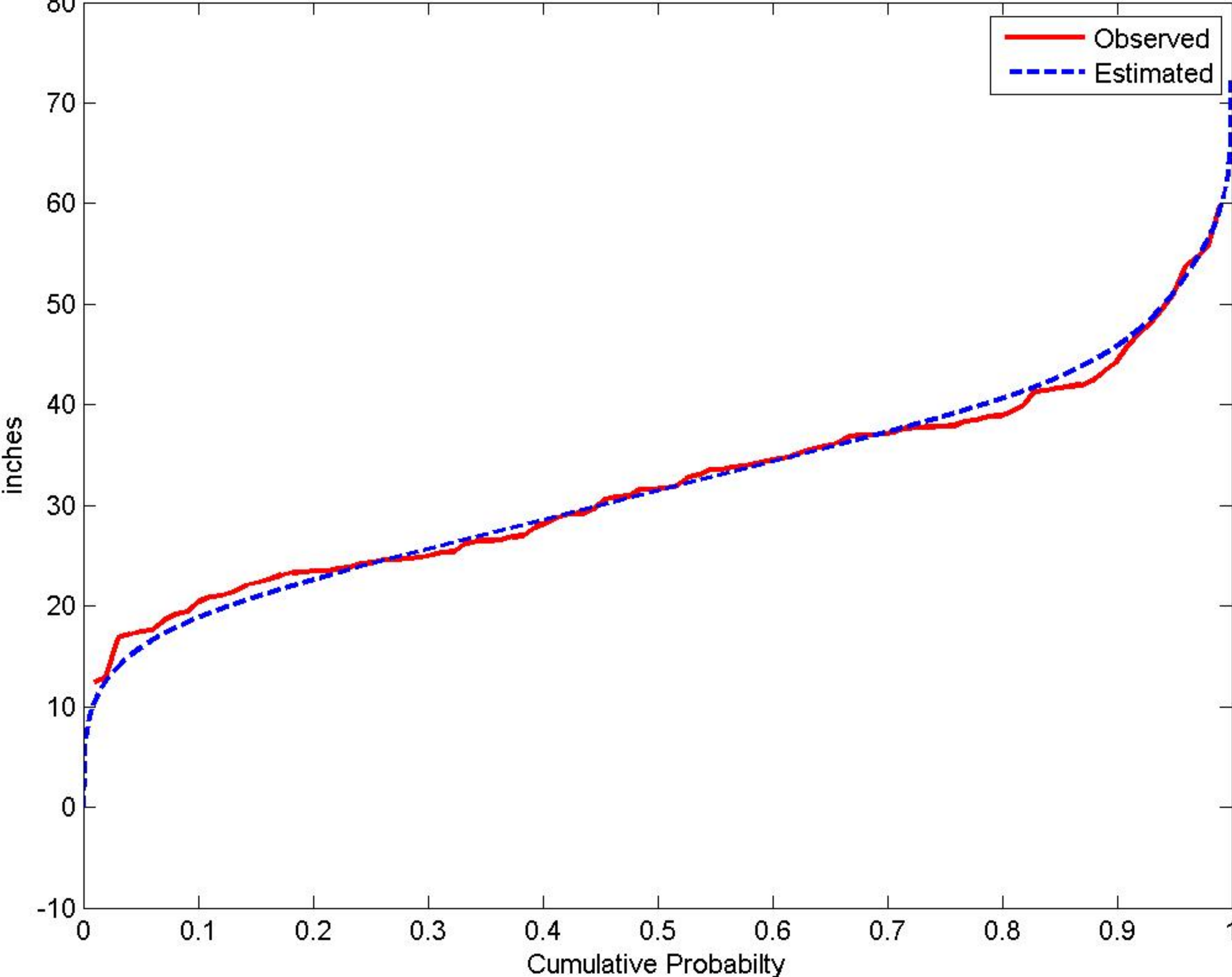
Fig.D11 - Cumulative Distribution Functions
