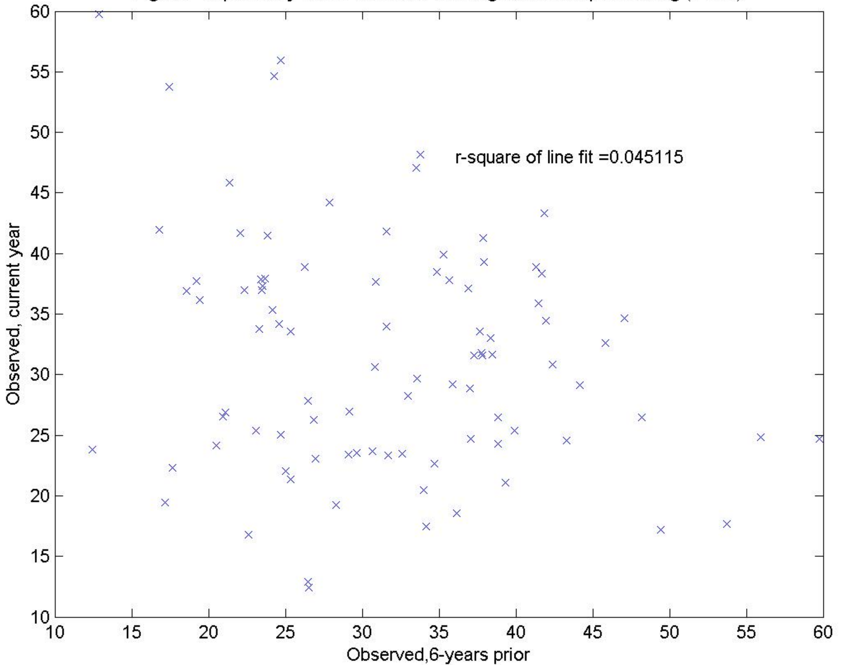
Fig.D8 - Explanatory Term: Consider Autoregression at specified lag (x-axis)
