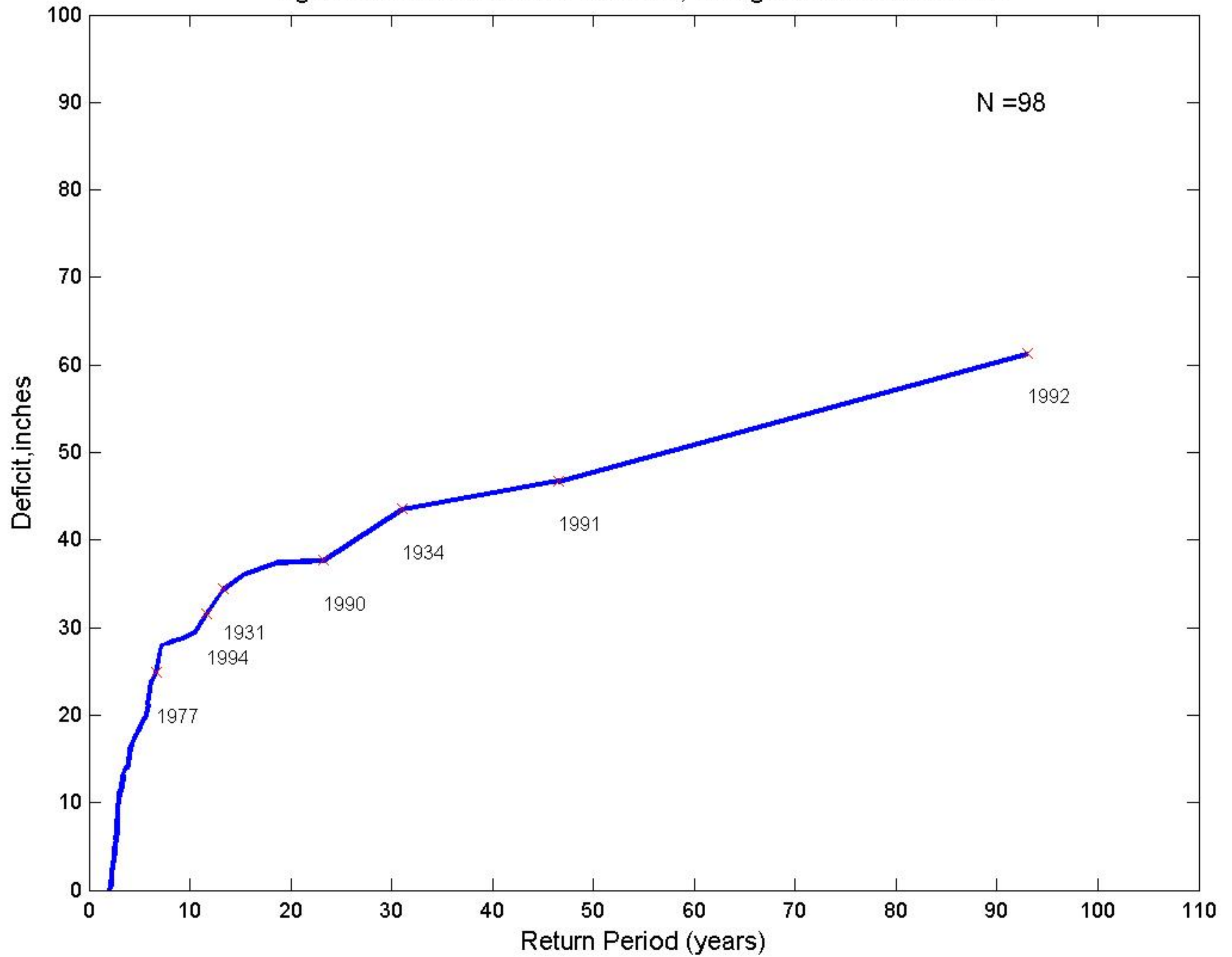
Fig.D6-Observed:Six-Year Duration, Drought End-Years Labeled
