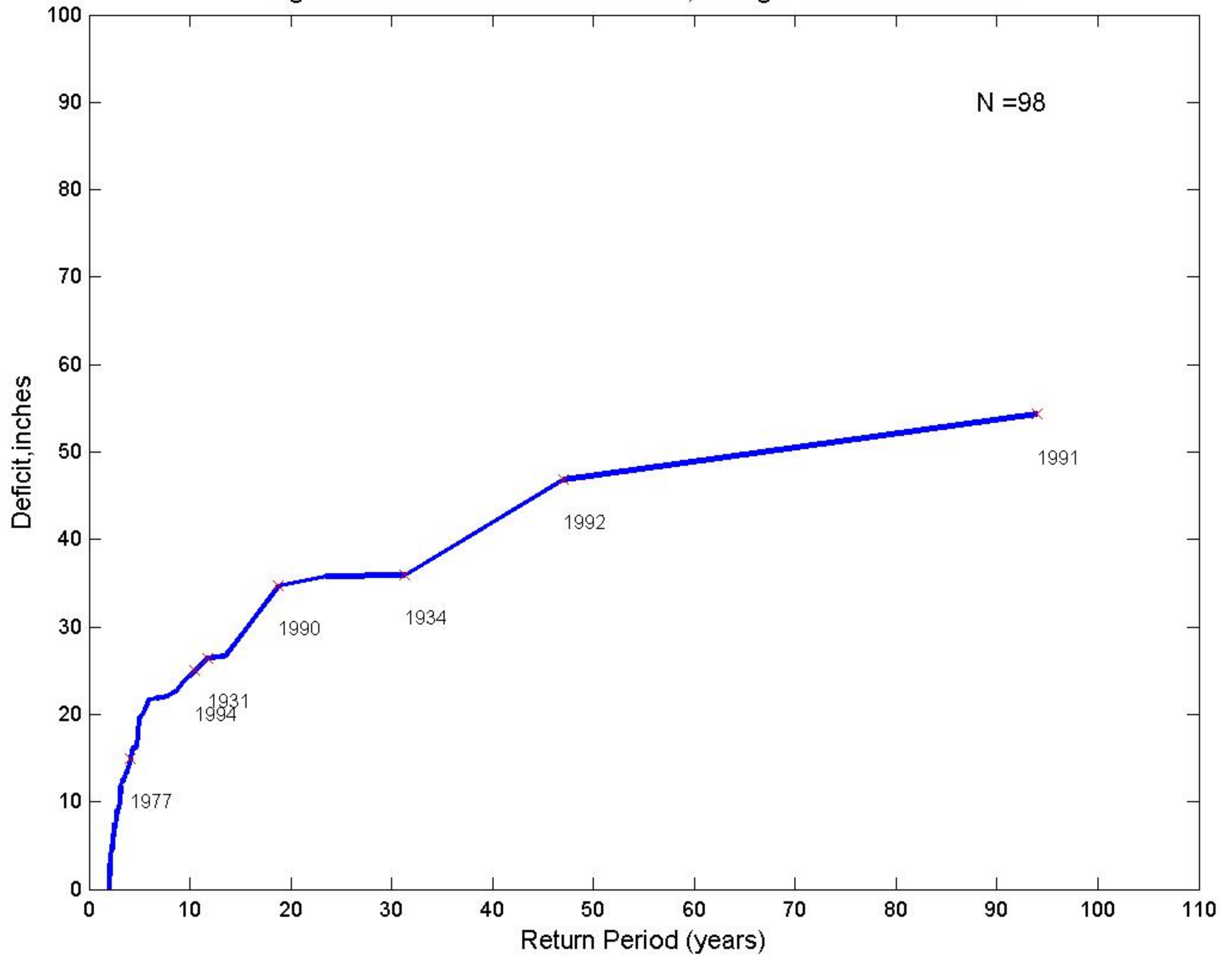
Fig.D5-Observed:Five-Year Duration, Drought End-Years Labeled
