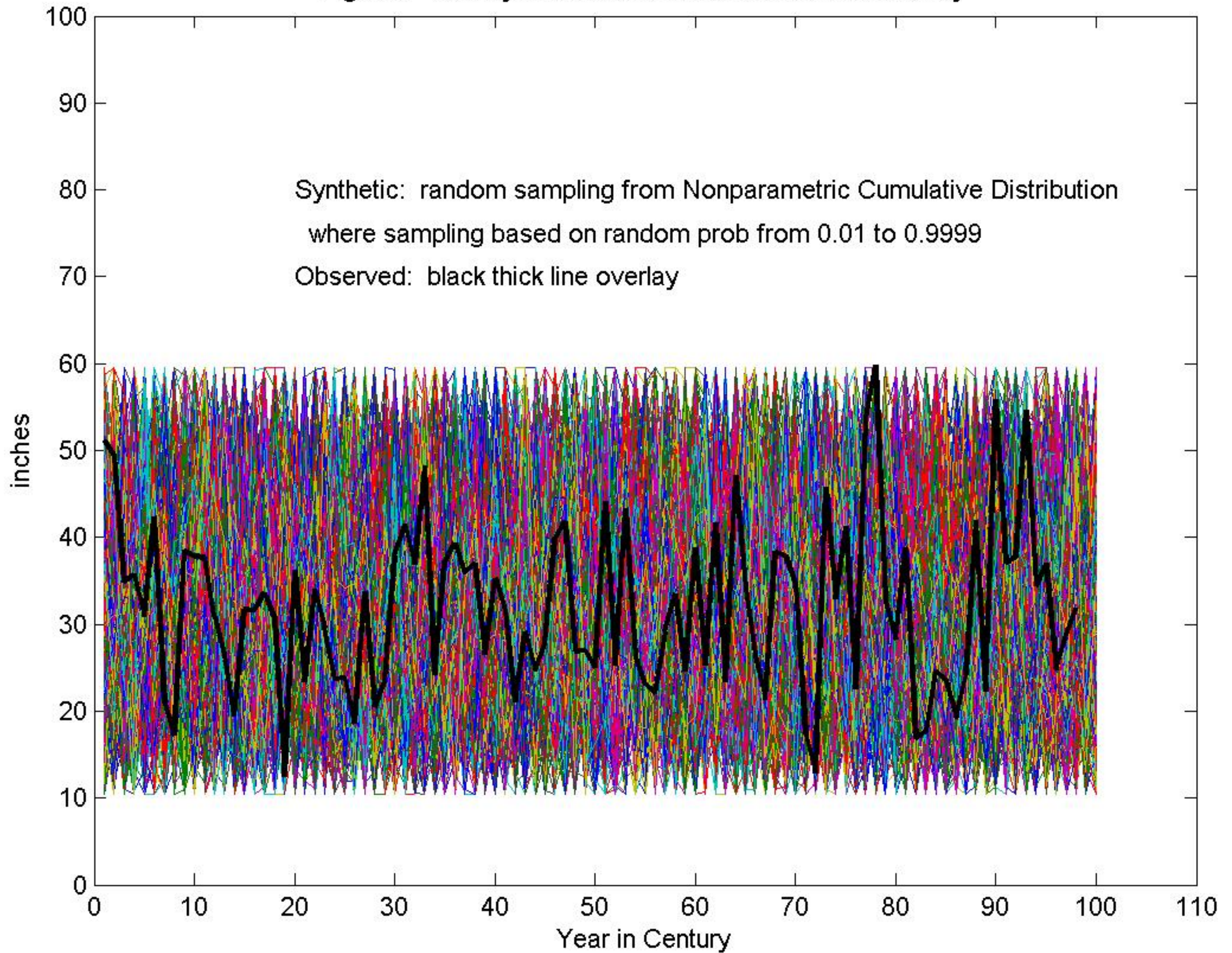
Fig.D12 - 200 Synthetic Centuries and Observed Overlay
