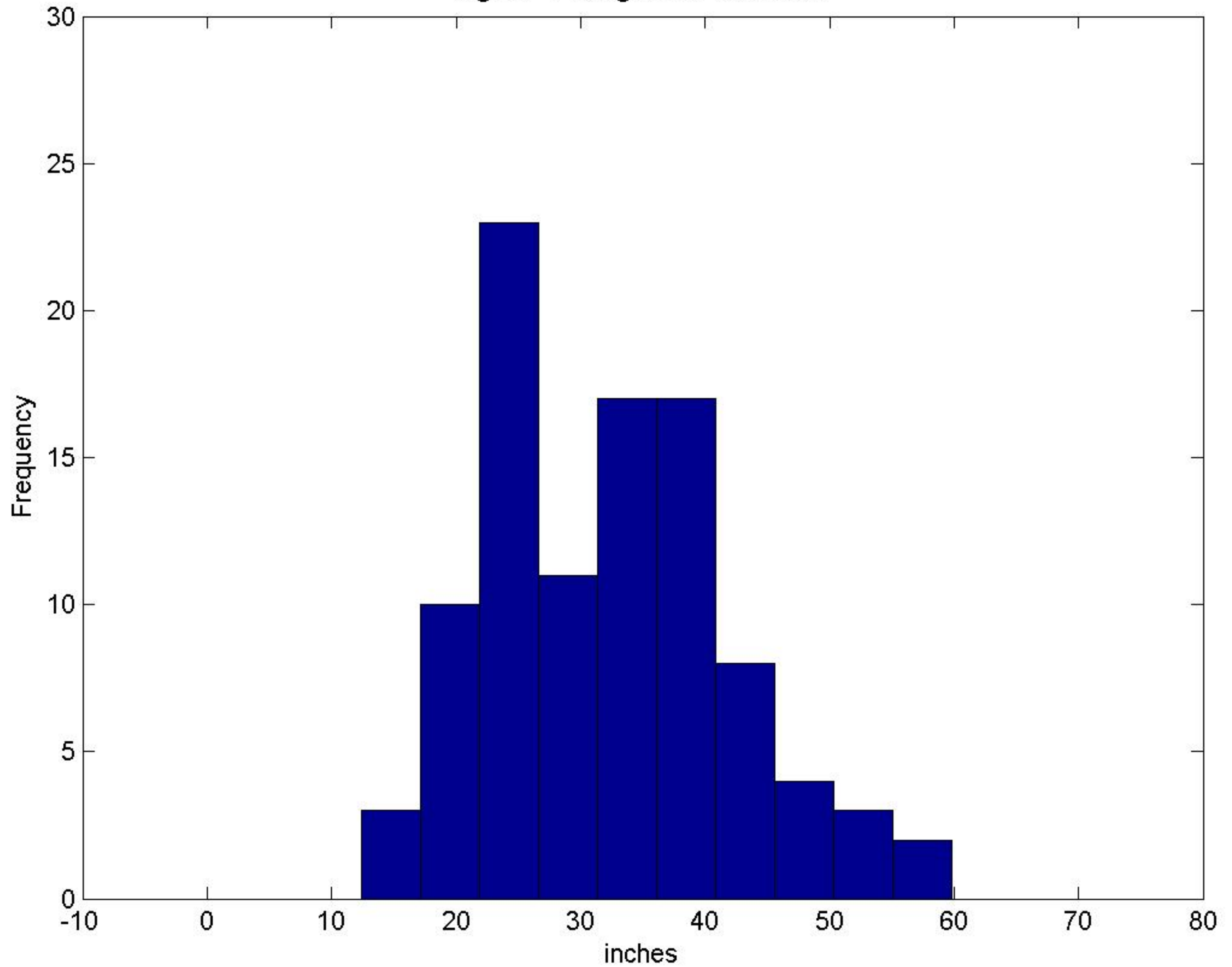
Fig.D9 - Histogram of Observed
