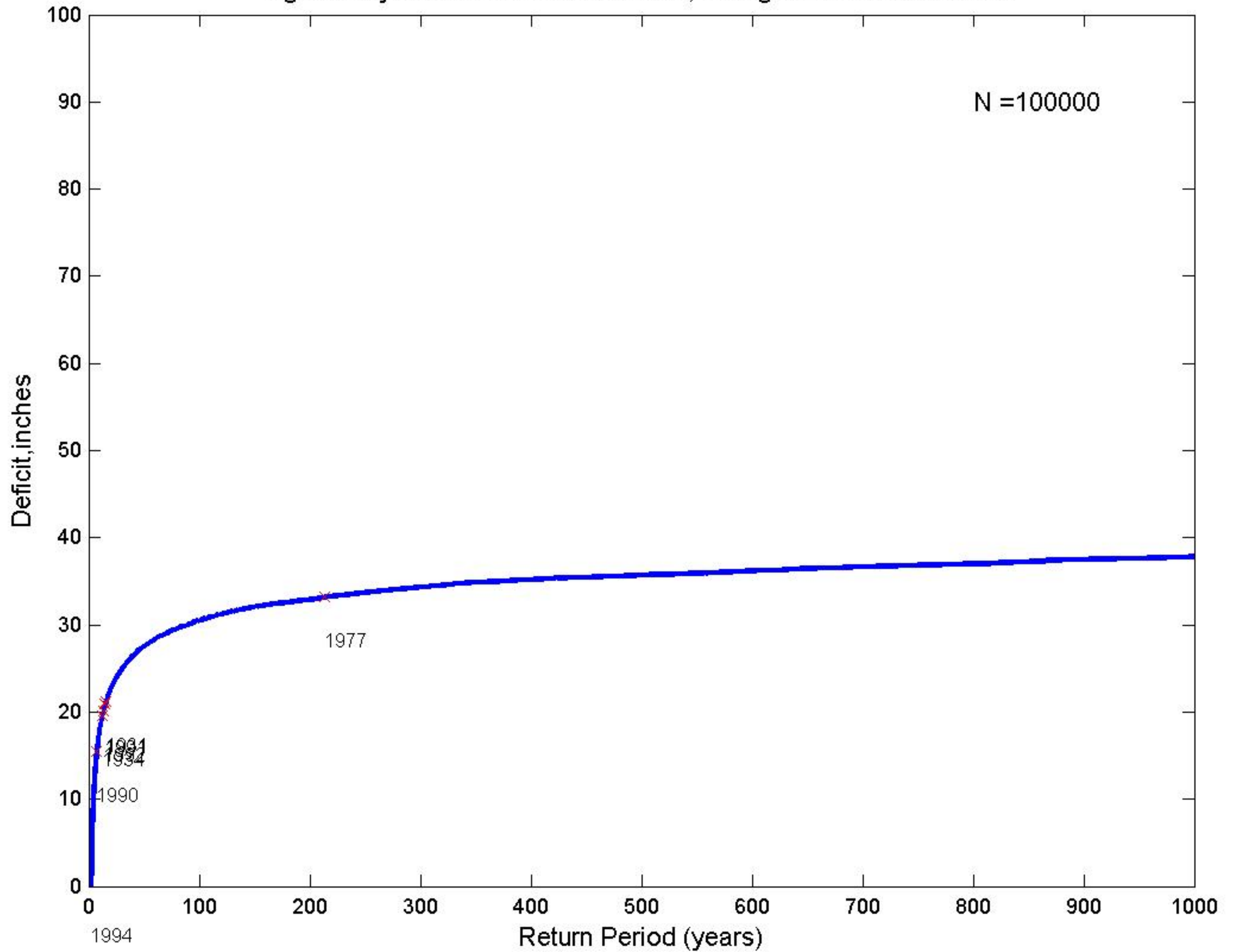
Fig.D15-Synthetic:Two-Year Duration, Drought End-Years Labeled
