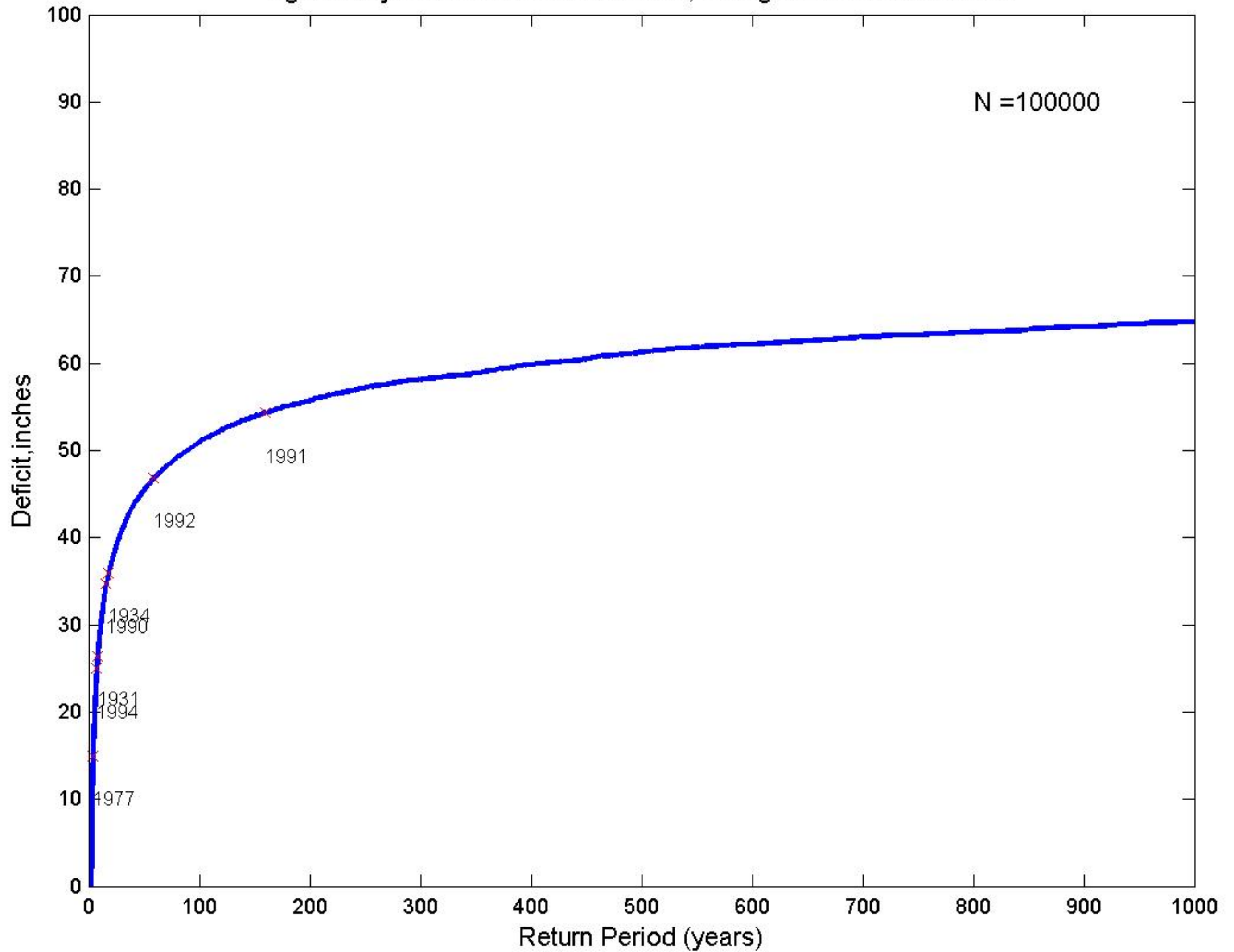
Fig.D18-Synthetic:Five-Year Duration, Drought End-Years Labeled
