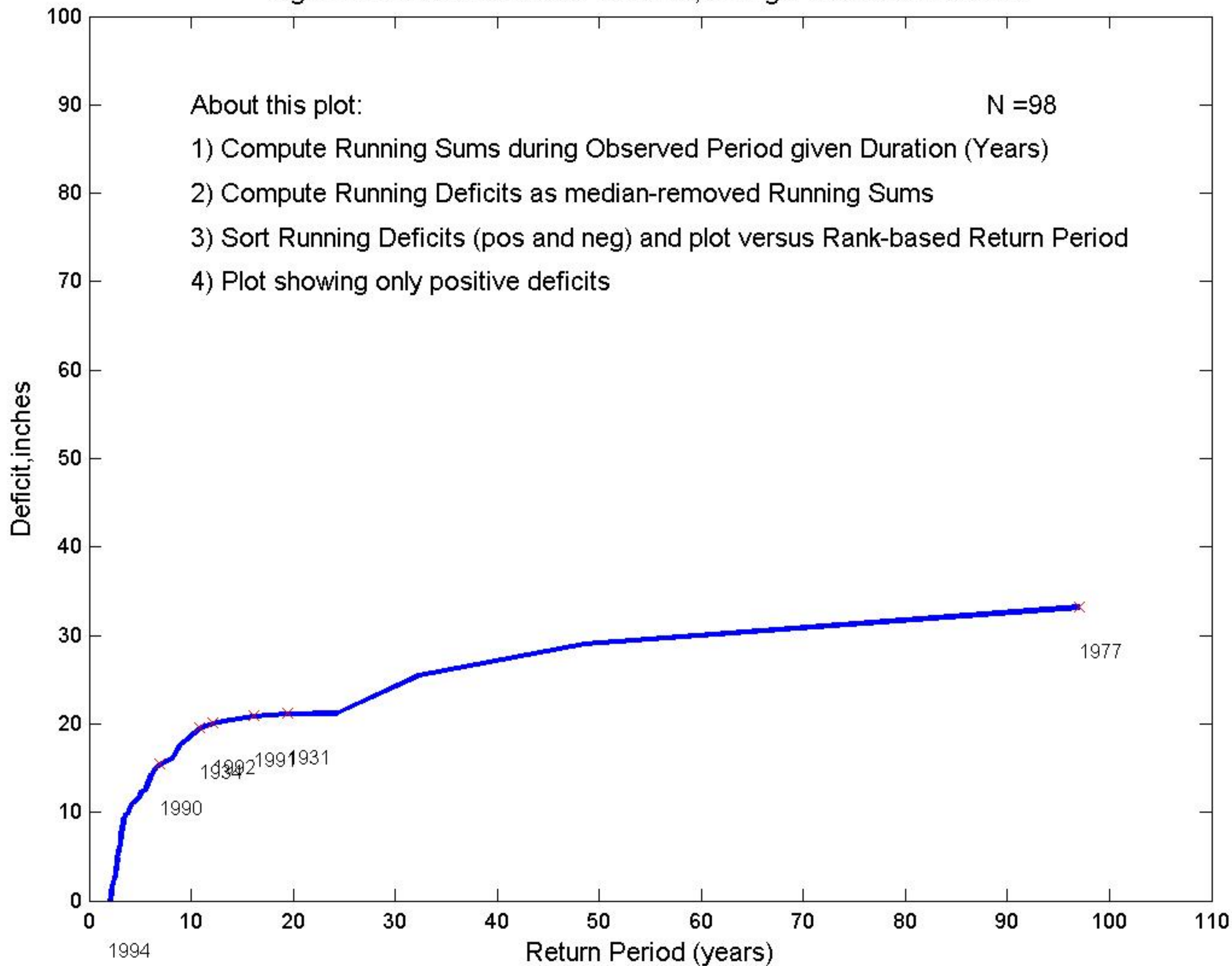
Fig.D2-Observed:Two-Year Duration, Drought End-Years Labeled
