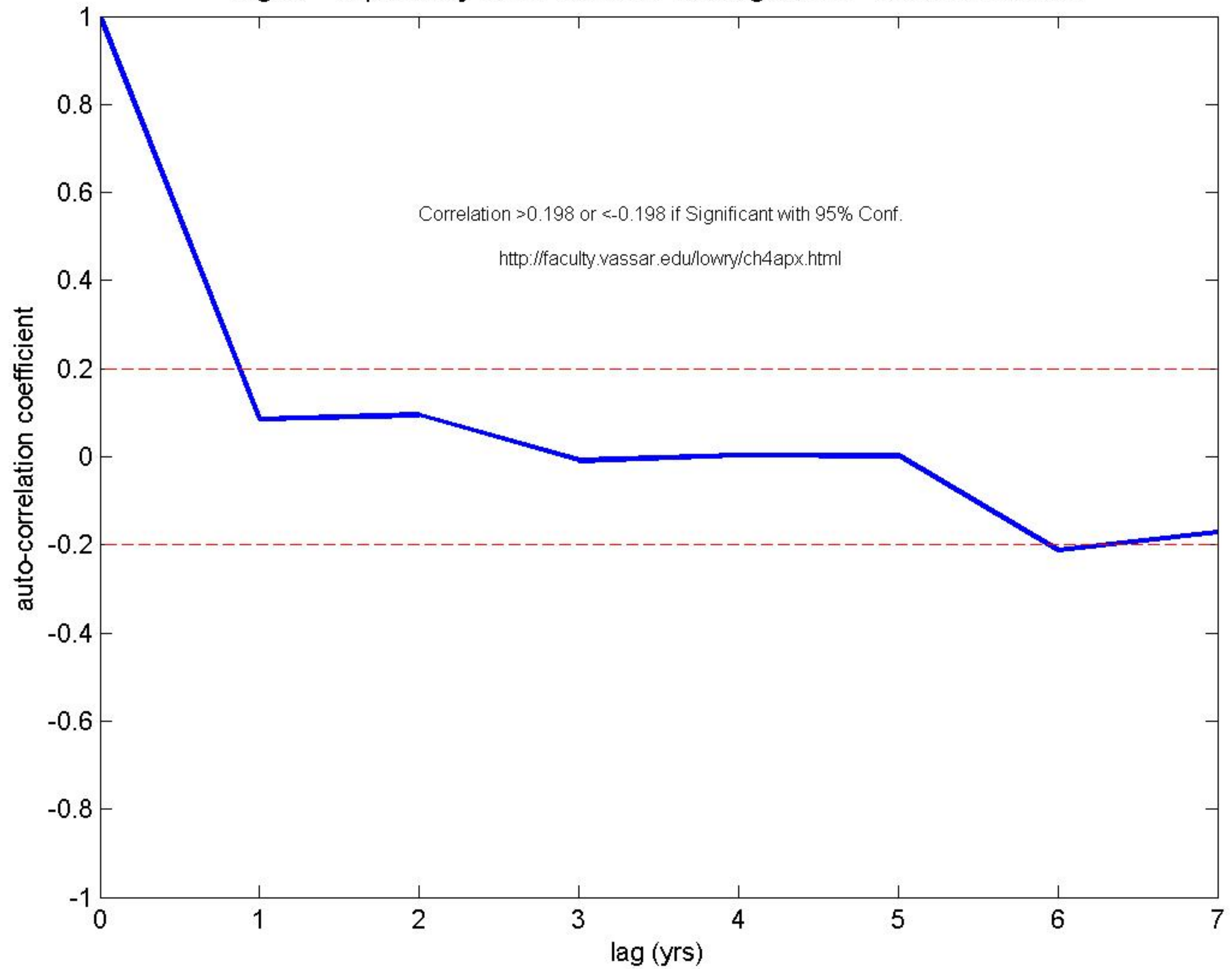
Fig.D7 - Explanatory Term: Consider Autoregression - Check Correlation
