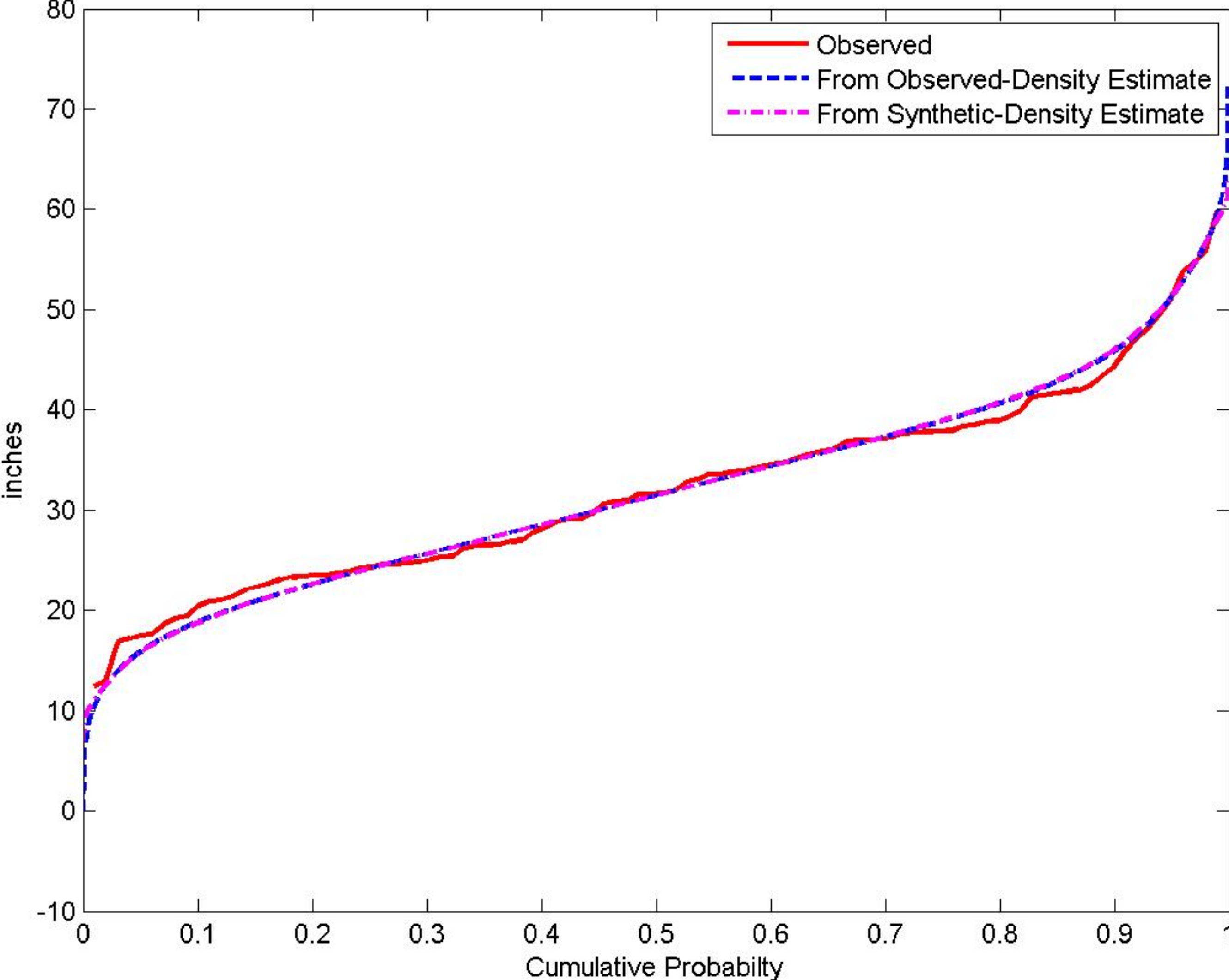
Fig.D14 - Cumulative Distribution Functions
