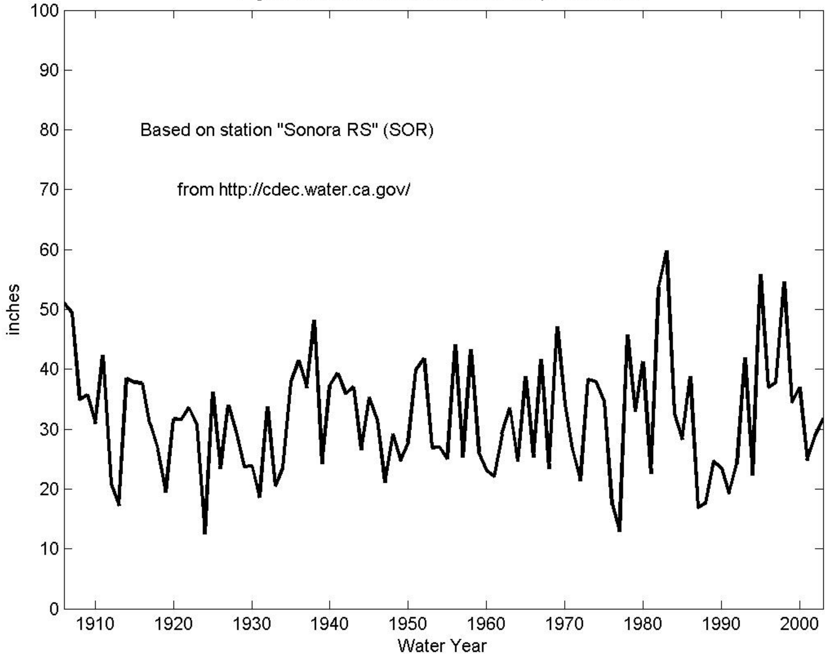
Fig.D1-Observed Annual Sonora Precip: 1906-2003
