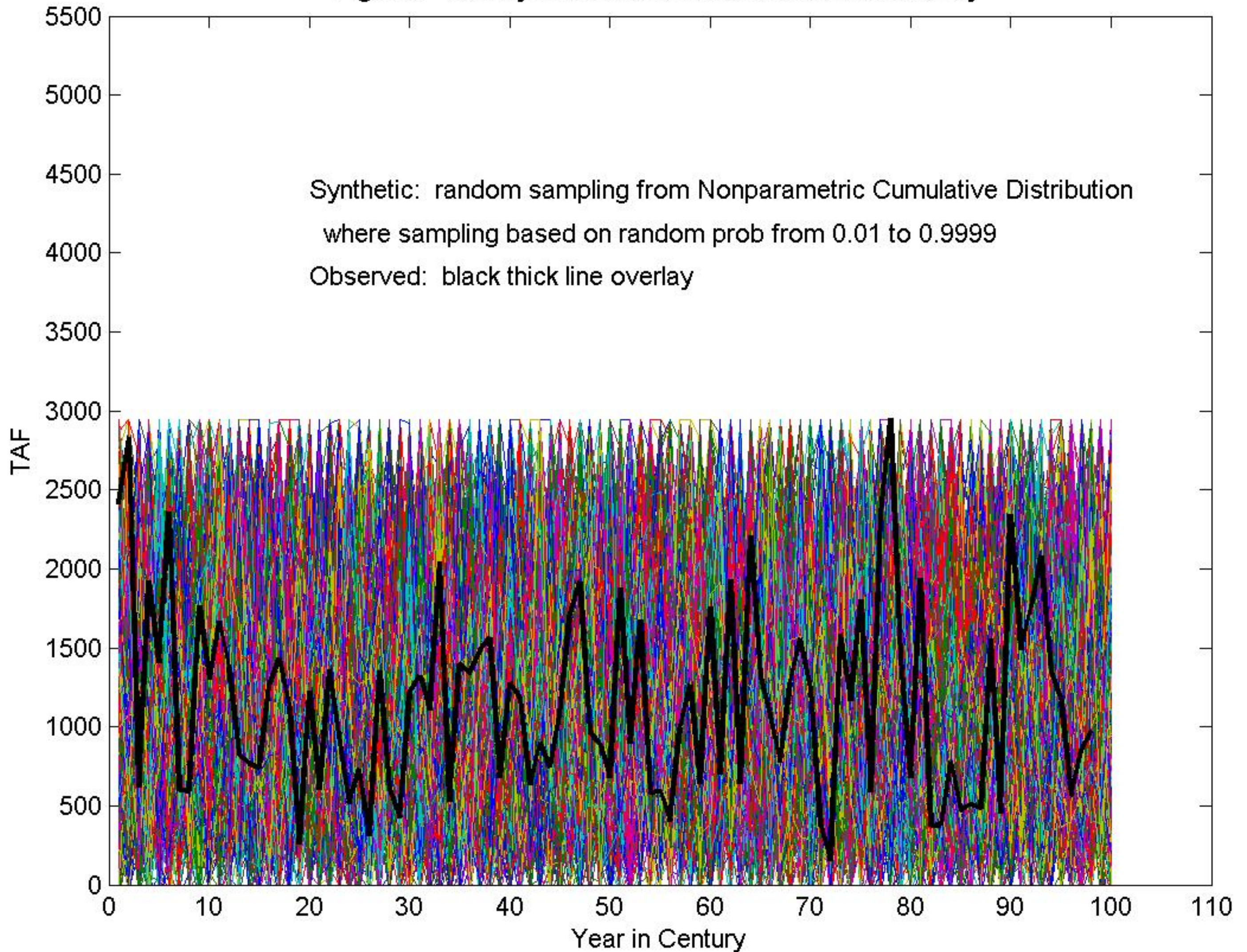
Fig.C12 - 200 Synthetic Centuries and Observed Overlay
