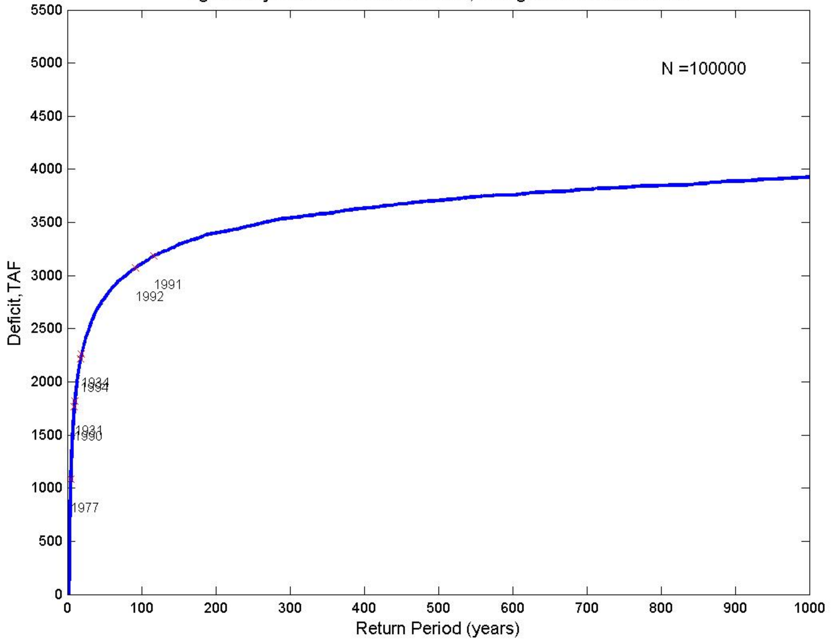
Fig.C18-Synthetic:Five-Year Duration, Drought End-Years Labeled
