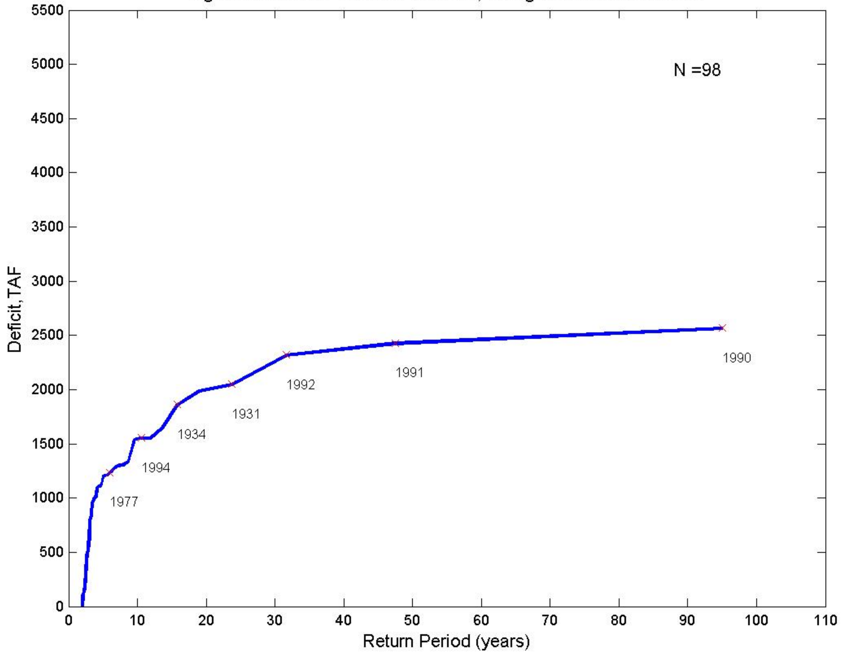
Fig.C4-Observed:Four-Year Duration, Drought End-Years Labeled
