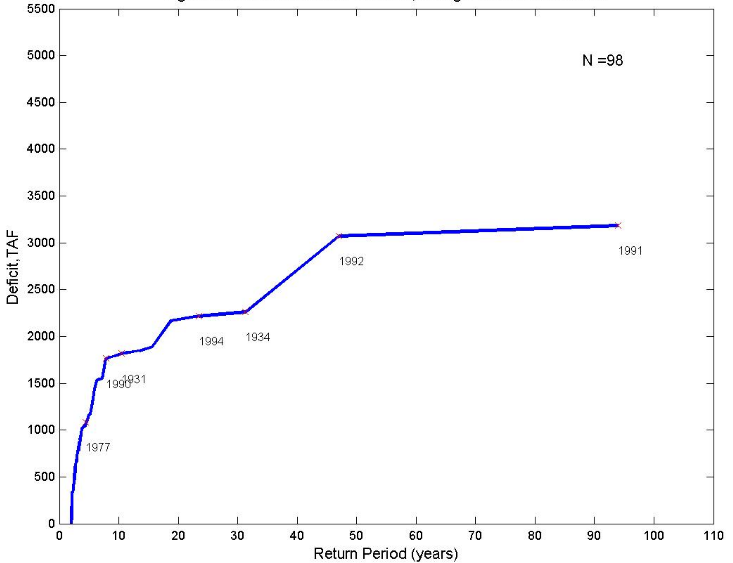
Fig.C5-Observed:Five-Year Duration, Drought End-Years Labeled
