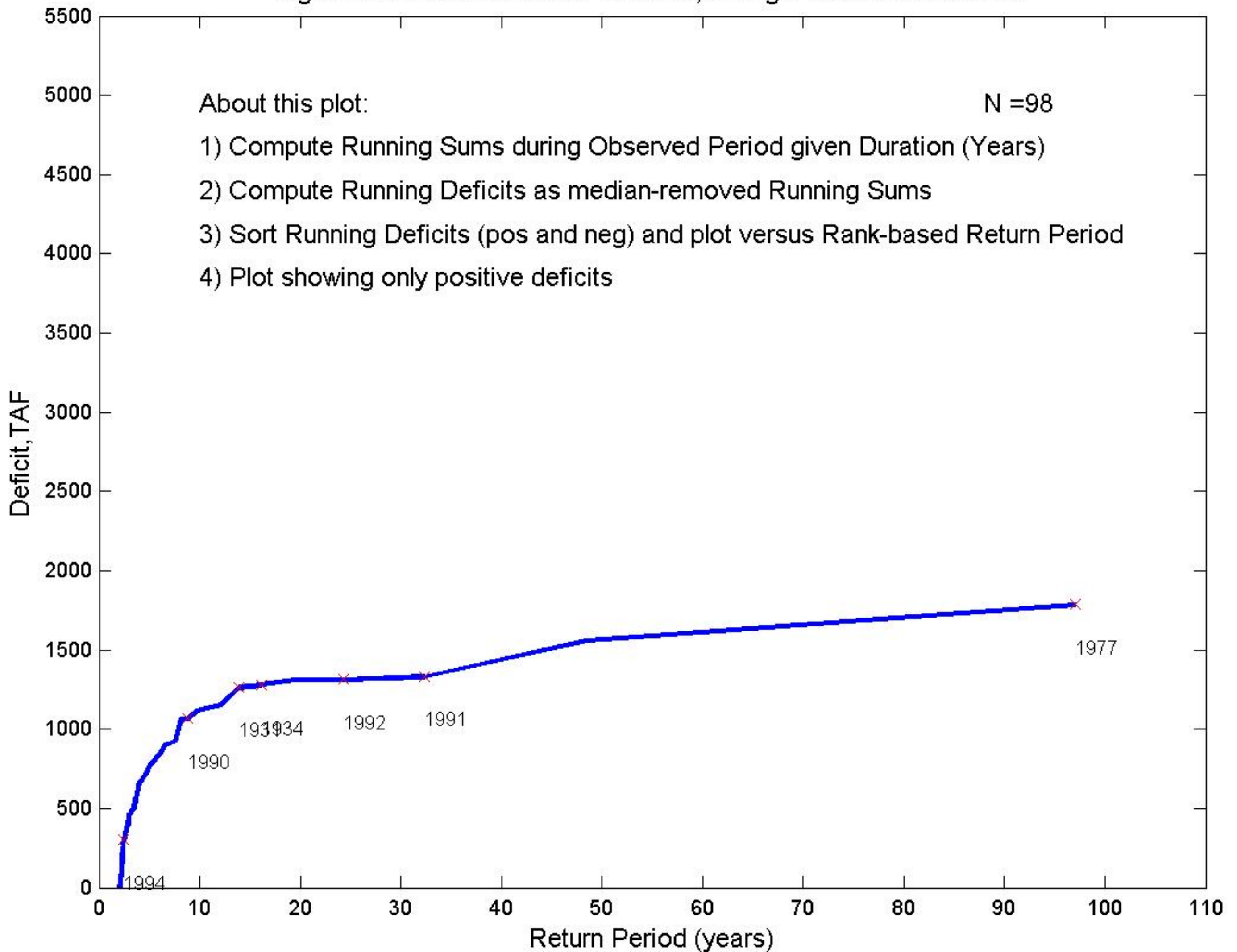
Fig.C2-Observed:Two-Year Duration, Drought End-Years Labeled
