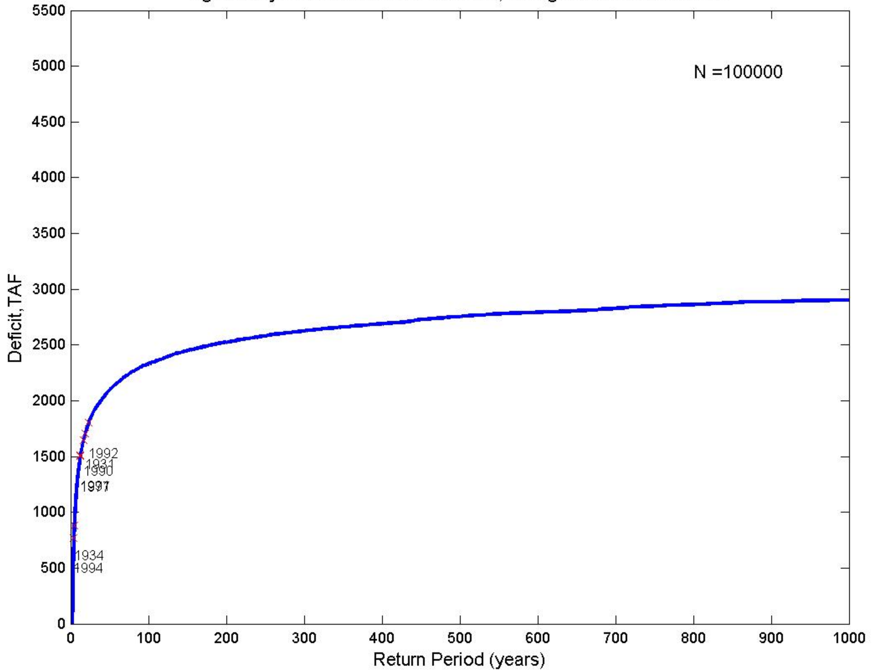
Fig.C16-Synthetic: Three-Year Duration, Drought End-Years Labeled
