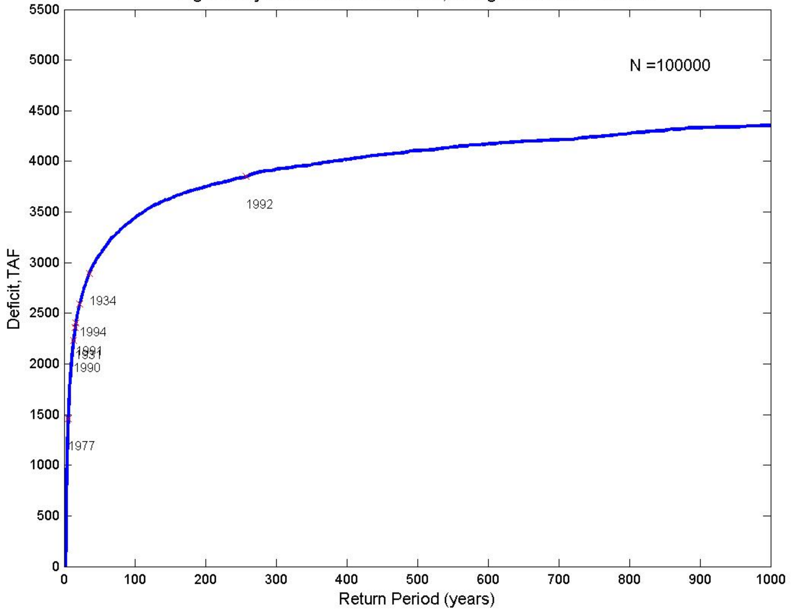
Fig.C19-Synthetic:Six-Year Duration, Drought End-Years Labeled
