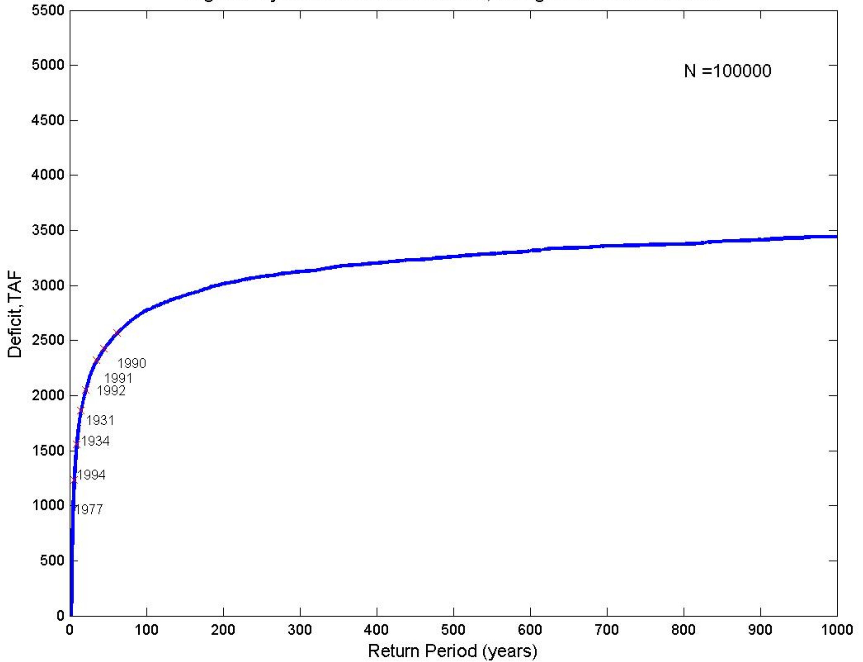
Fig.C17-Synthetic:Four-Year Duration, Drought End-Years Labeled
