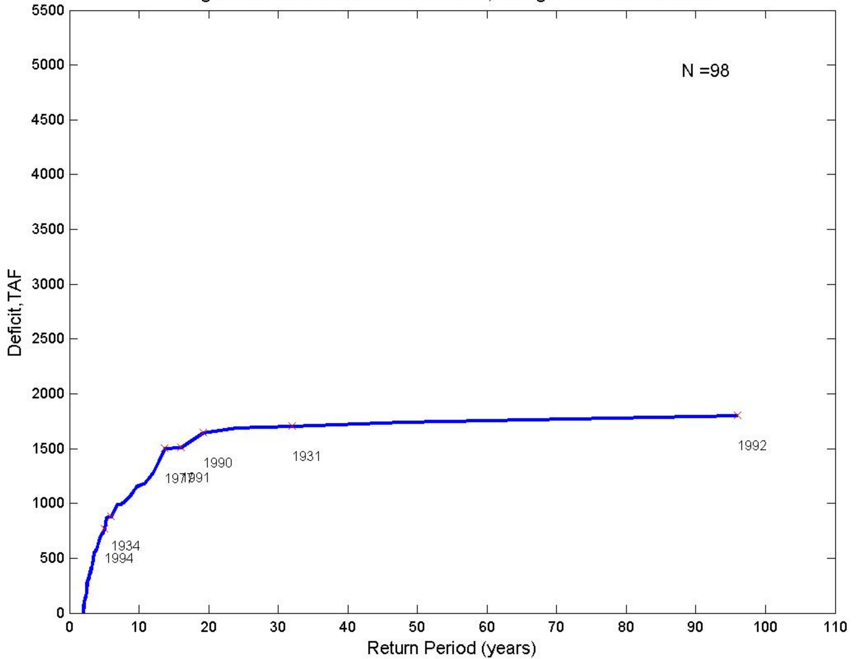
Fig.C3-Observed:Three-Year Duration, Drought End-Years Labeled
