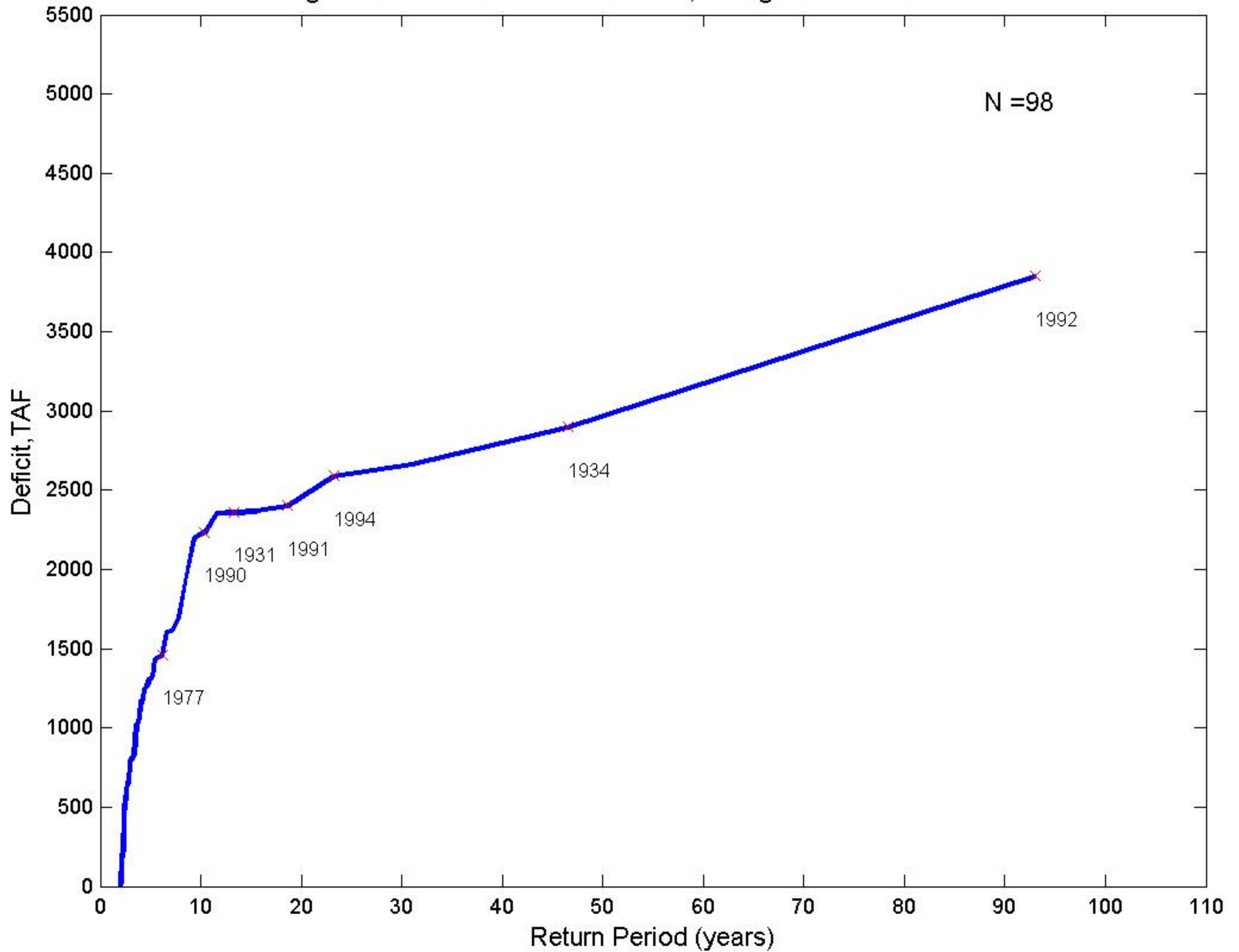
Fig.C6-Observed:Six-Year Duration, Drought End-Years Labeled
