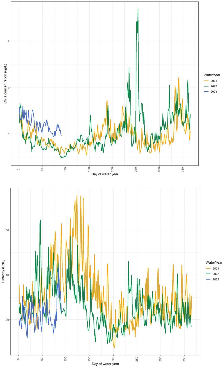
Figure 40 Comparison of chlorophyll concentration and turbidity at USGS continuous monitoring station at CM72 in the low-exchange zone of the ship channel. Missing data interval coincides with COVID-19 shut down period. Data are provisional.
