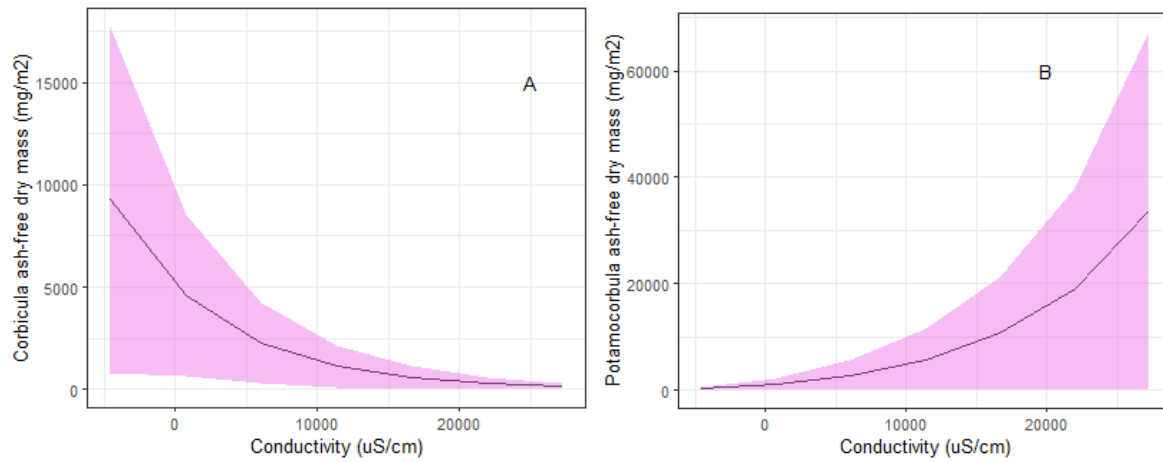
Figure 29 Salinity as a driver of A) Corbicula fluminea and B) Potamocorbula amurensis biomass in Suisun Marsh 2018-2021
