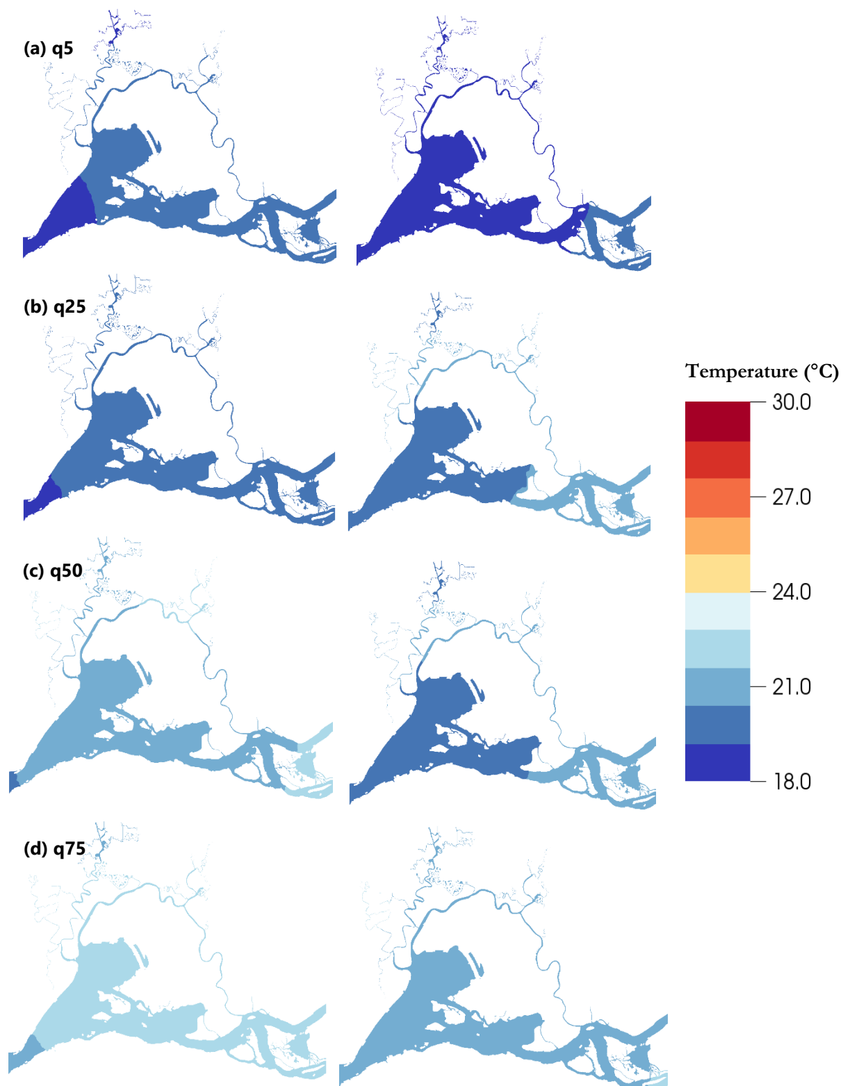
Figure 47. Sample monthly averaged temperature quantiles (5 th , 25 th , 50 th , 75 th ) for August (left) and September (right)
