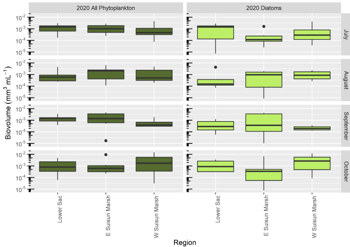
Figure 25 Estimated biovolume of all phytoplankton (left) and diatoms (right) based on samples collected during 2020 by the Environmental Monitoring Program, Summer Townet Survey, and Fall Midwater Trawl Survey. Sample sizes range 4-7 for each month by year combination.
