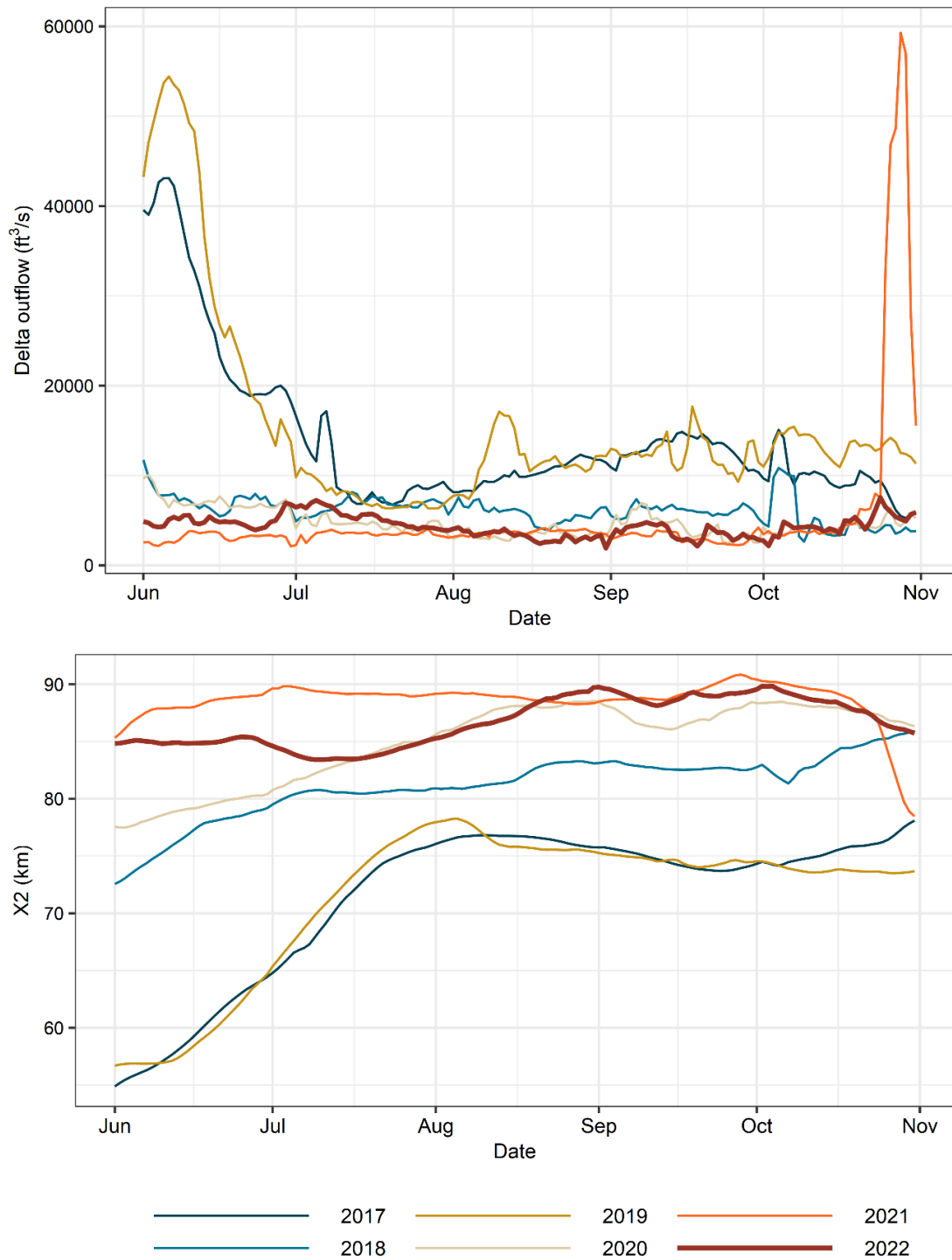
Figure 4 Top: Modeled daily Delta outflow from DWR Dayflow model from 2017 to 2021, plotted alongside 2022 Net Delta Outflow Index (NDOI) from DWR. Bottom: Modeled daily X2 from DWR Dayflow model (with the exception of 2022), plotted alongside calculated X2 for 2022 using X2 equation used in Dayflow and NDOI data (bottom). Dark red bold line indicates the year 2022.
