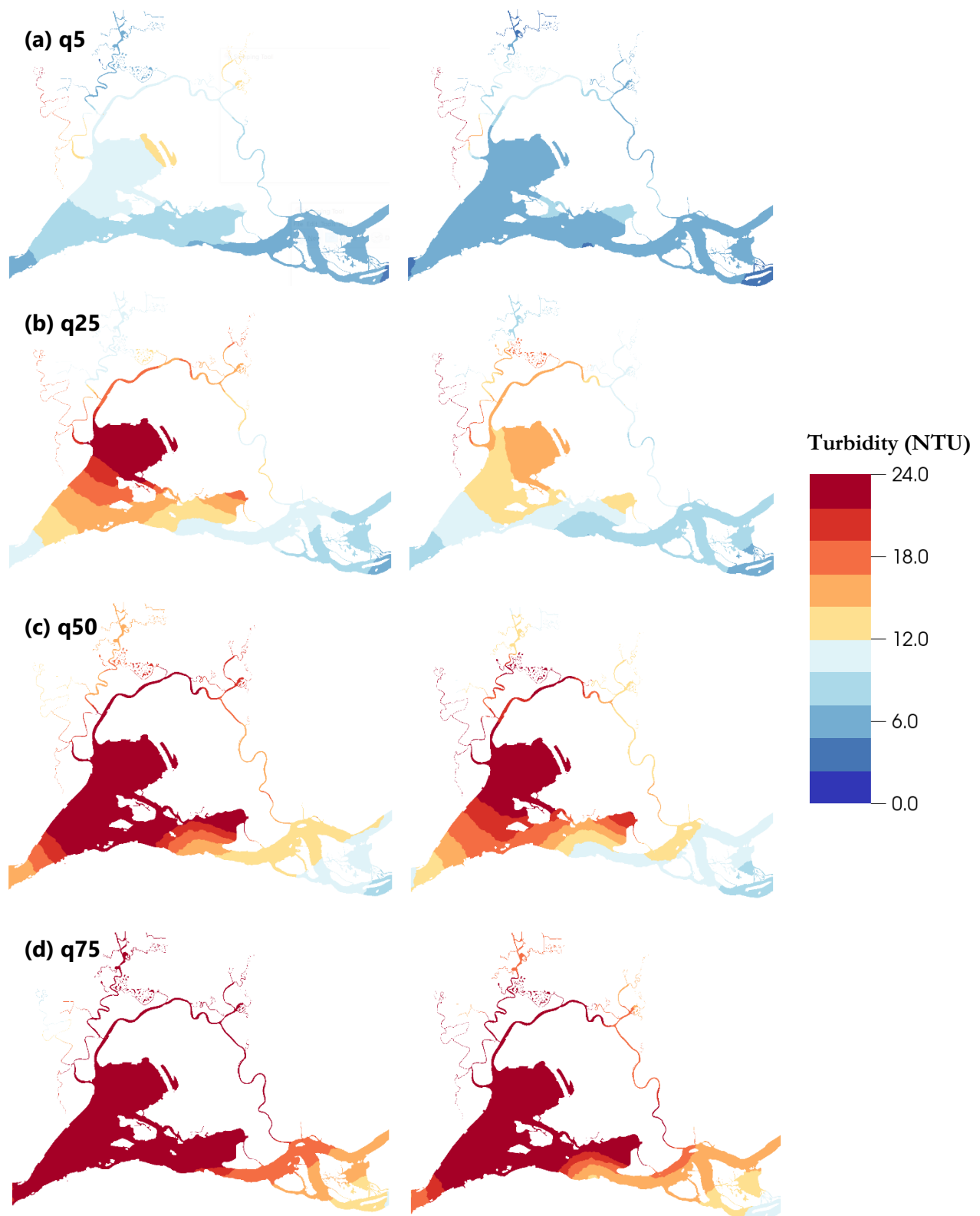
Figure 46. Sample monthly averaged turbidity quantiles (5 th , 25 th , 50 th , 75 th ) for August (left) and September (right)
