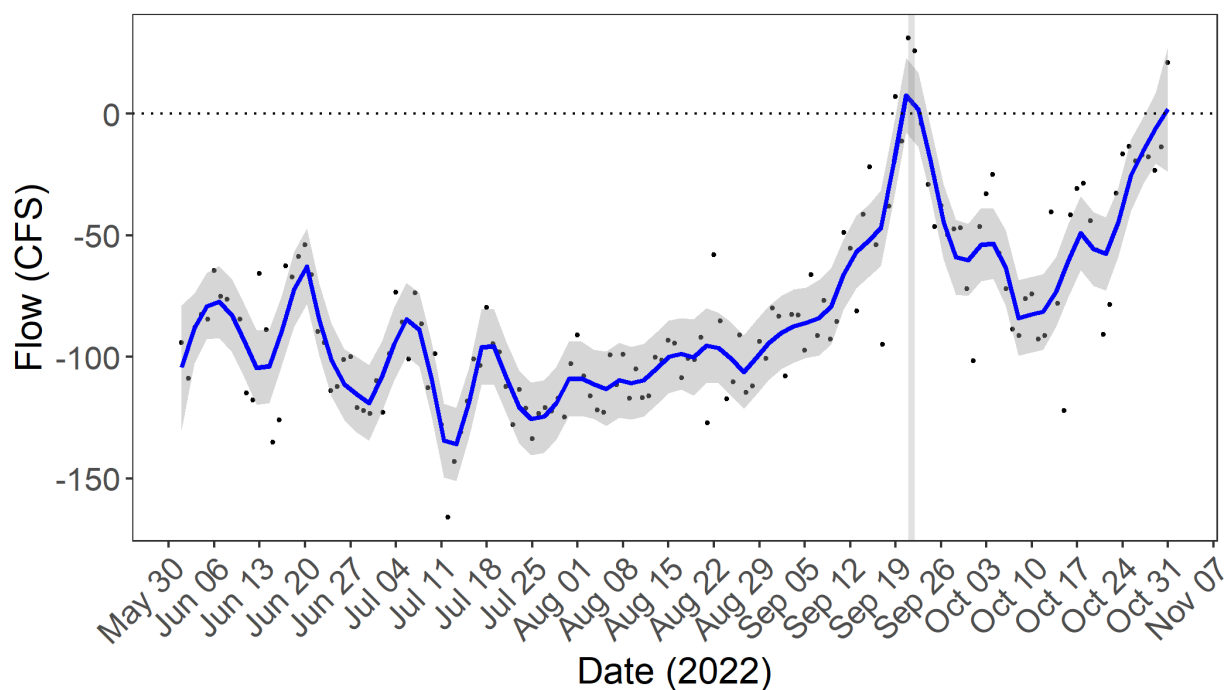
Figure 32 CDEC flow data from Lisbon Weir in the Yolo Bypass Toe Drain (station LIS) from June 1st through October 31st, 2022, taken at 15-minute intervals. Blue line indicates LOESS smoothing line \pm 1 SE of daily average flow. Points represent daily average flow, the horizontal dashed line at 0 CFS indicate the threshold for positive flow (downstream), and the grey box highlights the two-day non-managed flow pulse that occurred September 21st and September 22, 2022, during which daily average flow was 31.1 CFS. Data from CDEC are provisional, did not undergo QA/QC and are subject to change.
