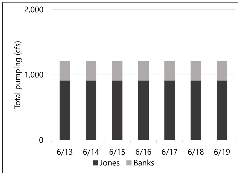
FIGURE A2. Daily forecasted pumping: Jones and Banks (cfs) for Baseline.
