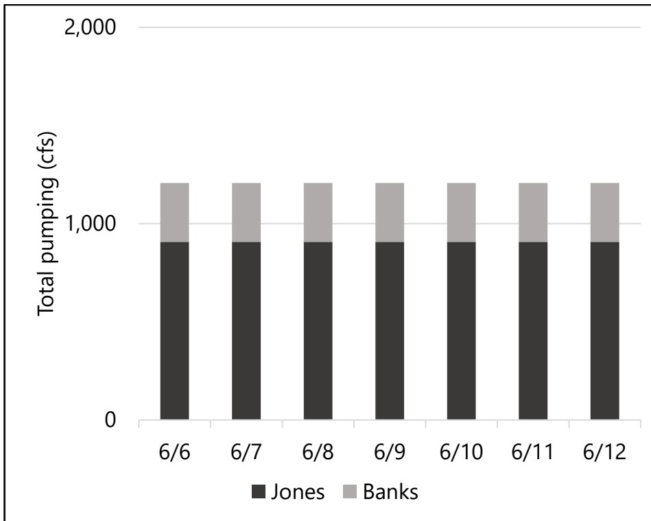
FIGURE A2. Daily forecasted pumping: Jones and Banks (cfs) for Baseline.
