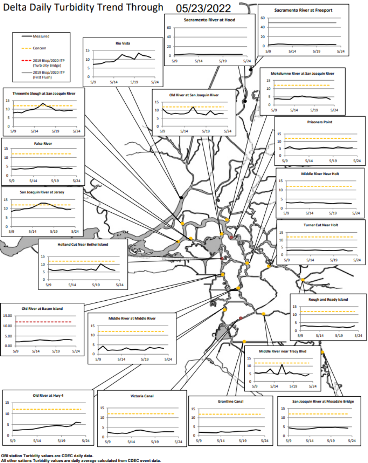
FIGURE 2. Delta Daily Turbidity Trends Through 05/23/2022
