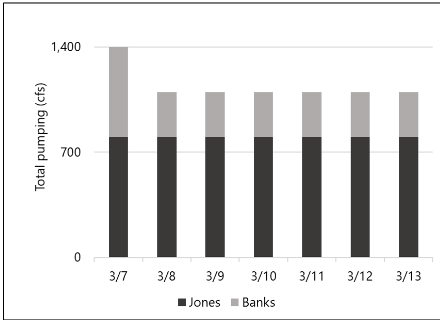
FIGURE A2a. Daily forecasted pumping: Jones and Banks (cfs) for (a) Baseline.
