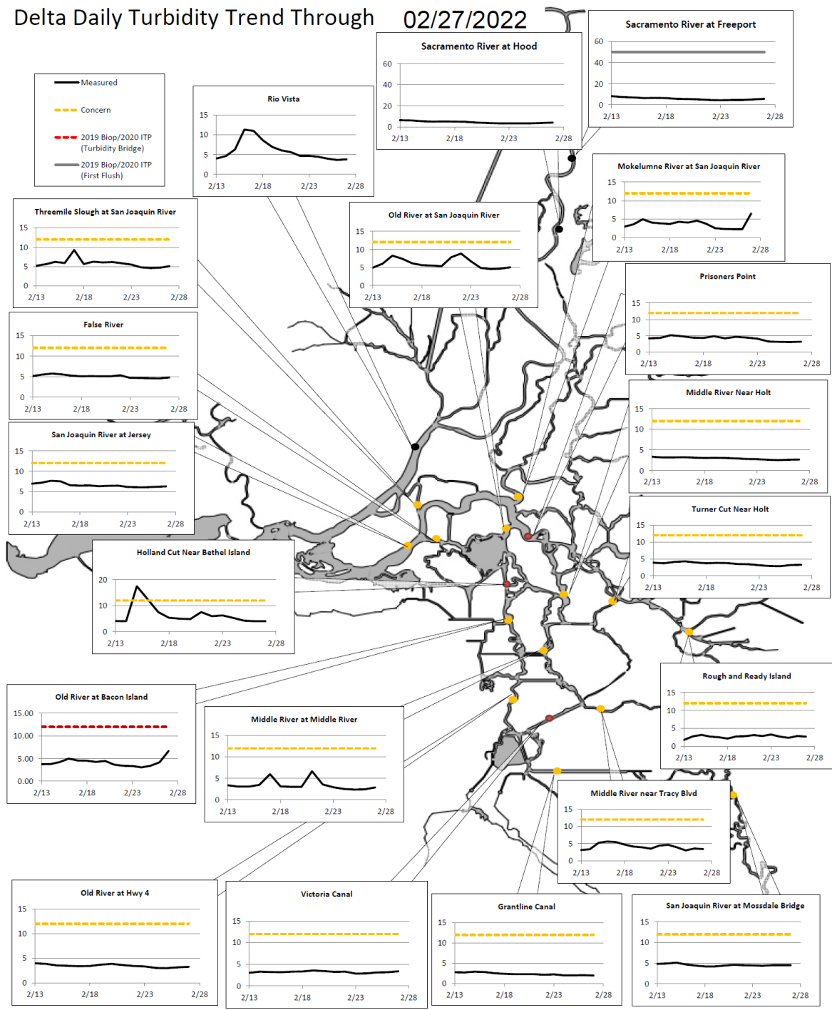
Figure 2. Delta Daily Turbidity Trends Through 02/27/2022
