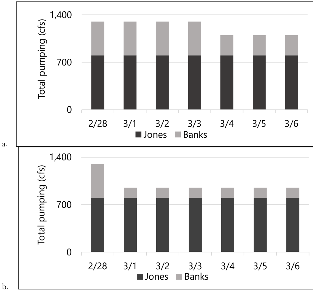
FIGURE A2a-c. Daily forecasted pumping: Jones and Banks (cfs) for (a) Baseline, and (b) Scenario 1.
