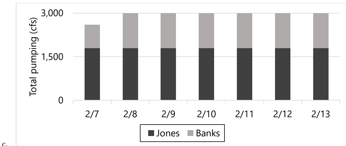
FIGURE A2a-c. Daily forecasted pumping: Jones and Banks (cfs) for (a) Baseline, (b) Scenario 1, and (c) Scenario 2.
