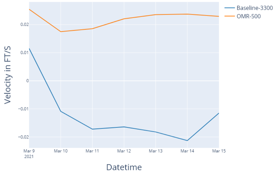
Figure A8: Slightly upstream of Head of Old River (CHAN006)
