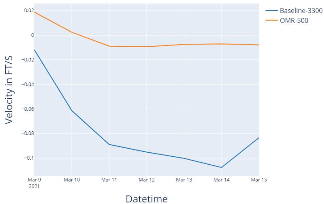
Figure A12: South Delta along Middle River (CHAN107 – Old River-Bacon Isl.)
