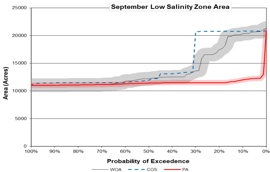
Figure 5.16-36. Mean Modeled Low Salinity Zone Area, September.
