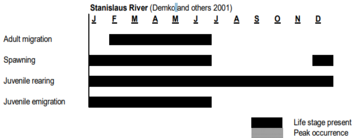
Figure 5.10-26. Stanislaus River Weir O. mykiss Passage (FishBio 2012)
