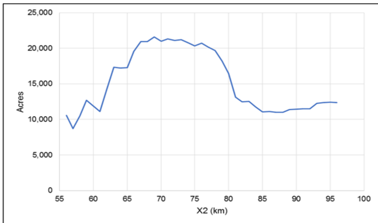
Figure 5.16-52: Acres of low salinity zone (1-6ppt) versus X2 in kilometers from the Golden Gate Bridge
