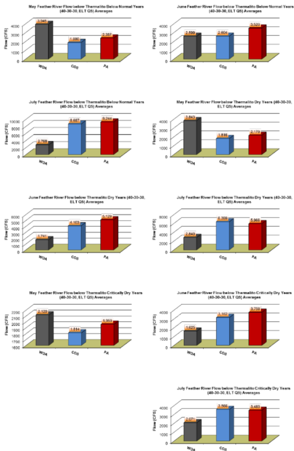
Figure 5.12-43. CalSim II estimates of Feather River Flow below the Thermalito Afterbay in May-July under the WOA, Proposed Action, and COS Scenarios.
