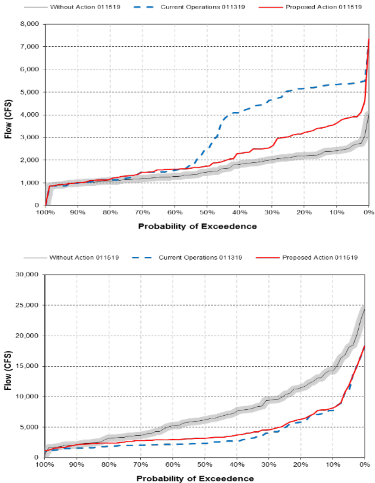
Figure 5.8-30. CalSimII estimates of Feather River flow below the Thermalito Afterbay in September-November and December-February under the WOA (Without Action), COS (Current Operations), and PA (Proposed Action) scenarios.
