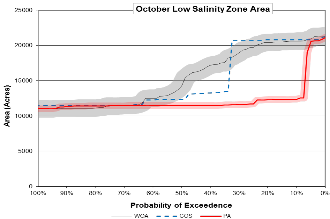
Figure 5.16-37. Mean Modeled Low Salinity Zone Area, October.
