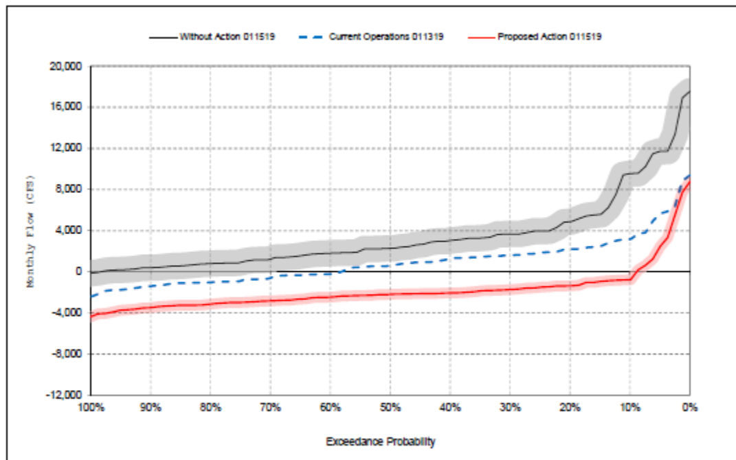
Figure 5.16-45. Mean Modeled Old and Middle River Flows, April.
