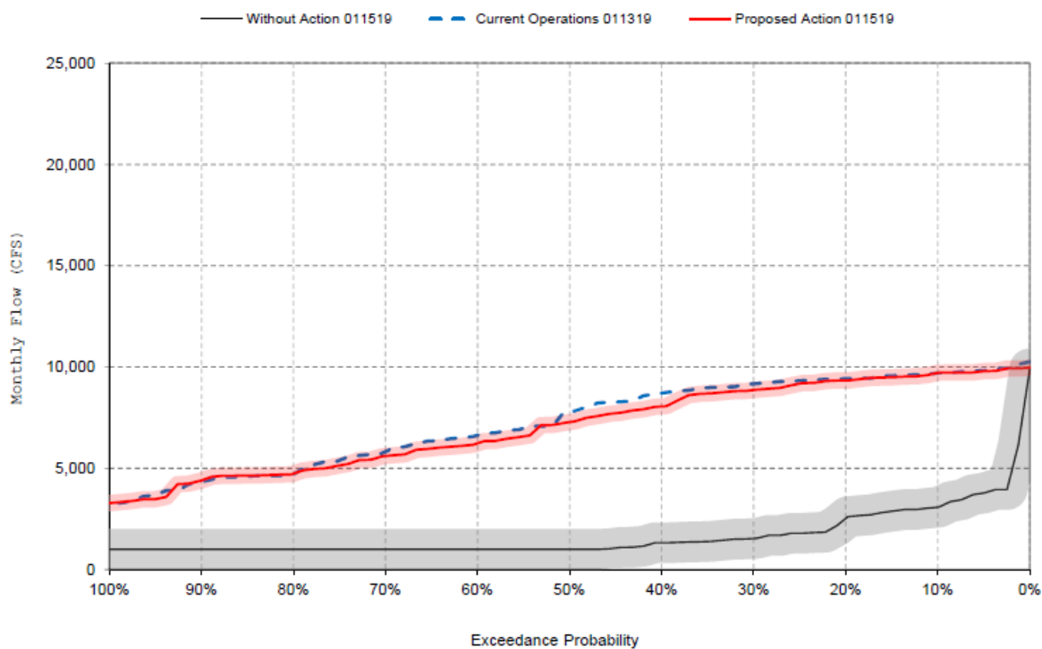
Figure 5.8-16. Modeled Sacramento River Flows at Wilkins Slough, July
