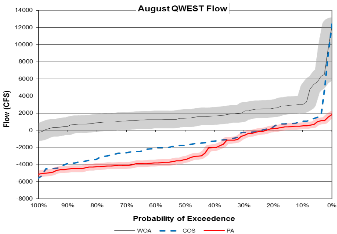
Figure 5.16-17. Mean Modeled QWEST Flow, August
