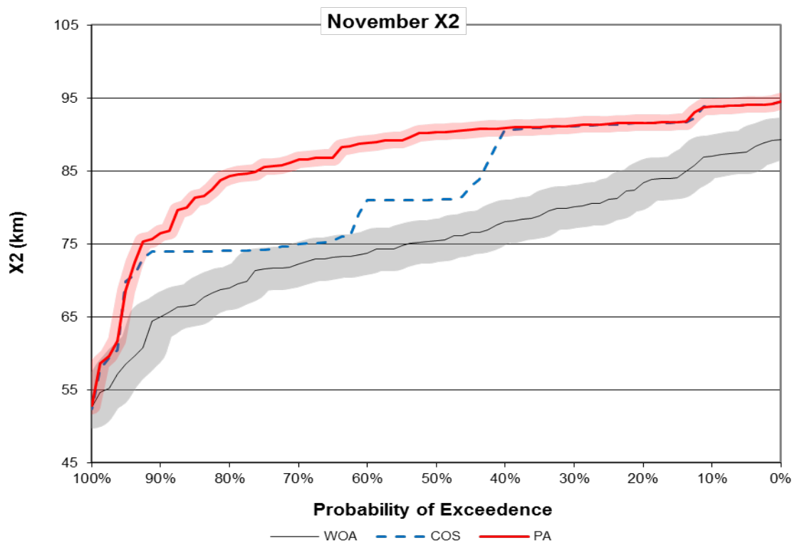
Figure 5.16-35. Mean Modeled X2 from CalSim, November.
