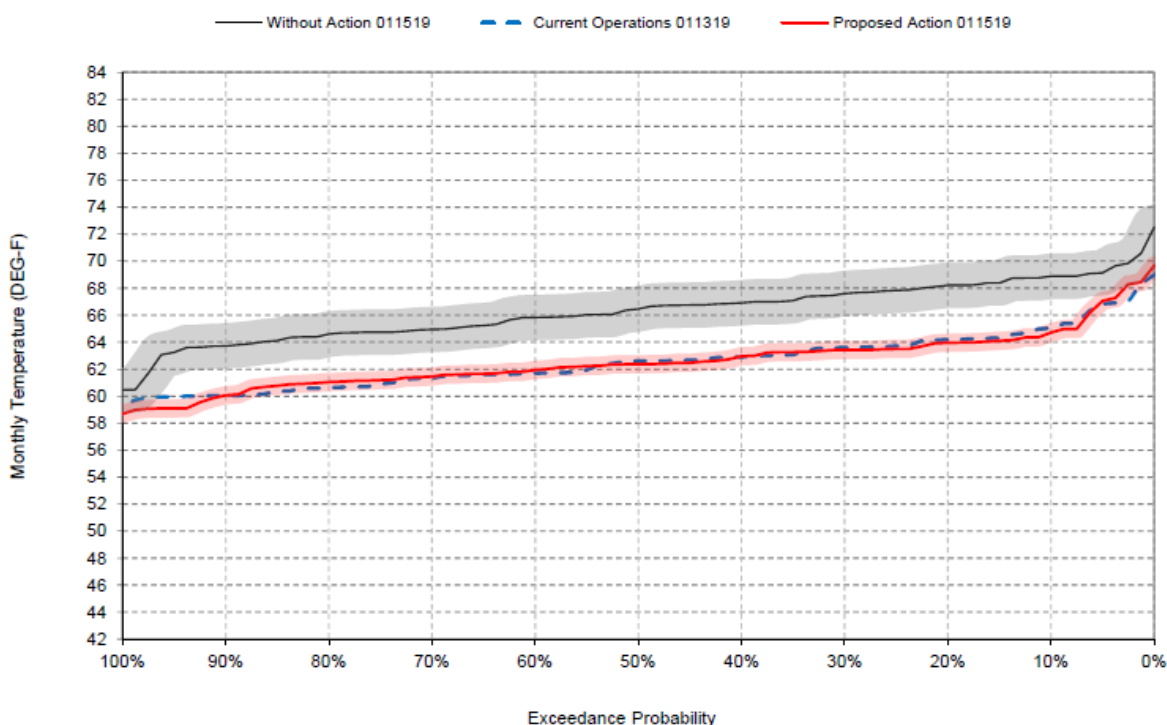
Figure 5.8-10. HEC-5Q Sacramento River Water Temperatures at Keswick Dam under the WOA and COS scenarios, October
