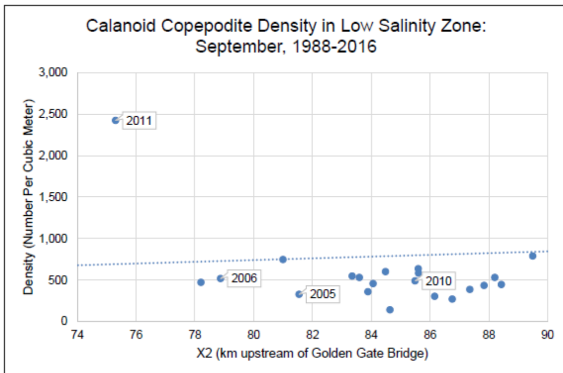
Figure 5.16-30. Mean September Calanoid Copepod Copepodite Density in the Low Salinity Zone (Salinity = 1 to 6) from Environmental Monitoring Program Zooplankton Survey Data (Clarke-Bumpus Net) versus Mean X2 from 1988-2016.
