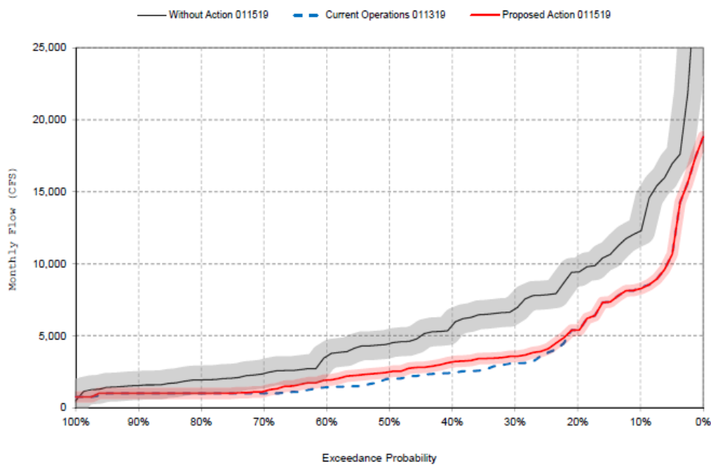
Figure 5.10-10. CalSimII estimates of Feather River flow below the Thermalito Afterbay in May under the WOA, COS, and proposed action.
