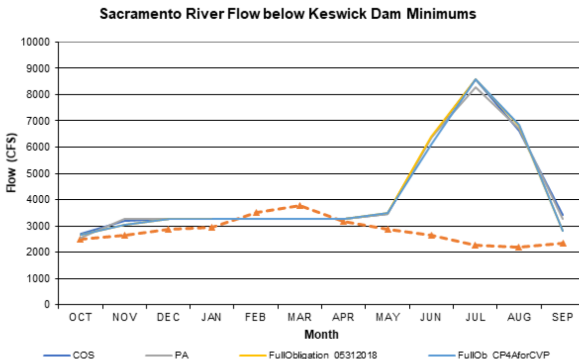
Figure 5.6-40. CalSim II Sacramento River Flows below Keswick Dam all scenarios
