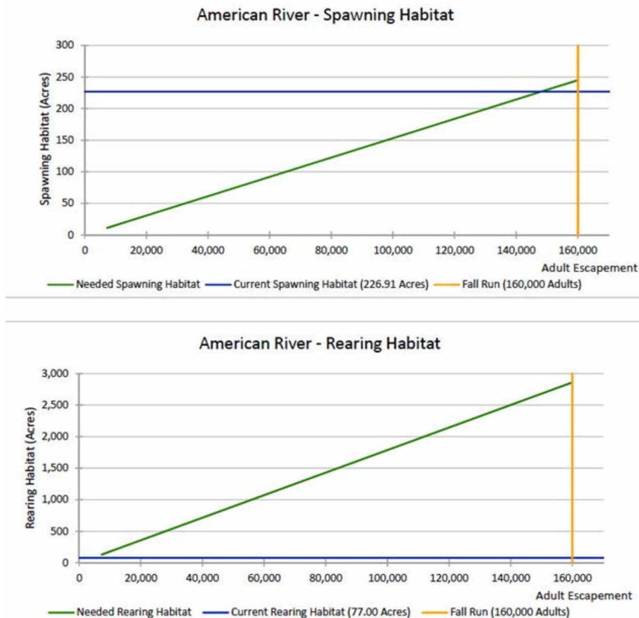
Figure 5.14-21. Estimated Chinook spawning and rearing habitat needed in the lower American River to support the range of escapement sizes (CVPIA 2018).
