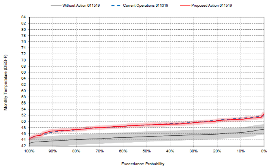
Figure 5.10-24: Exceedance Probability of January Temperatures below Goodwin Dam
