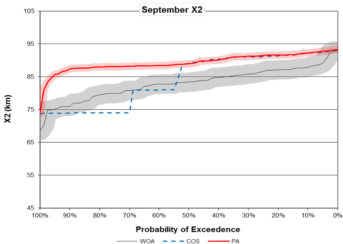
Figure 5.16-33. Mean Modeled X2 from CalSim, September
