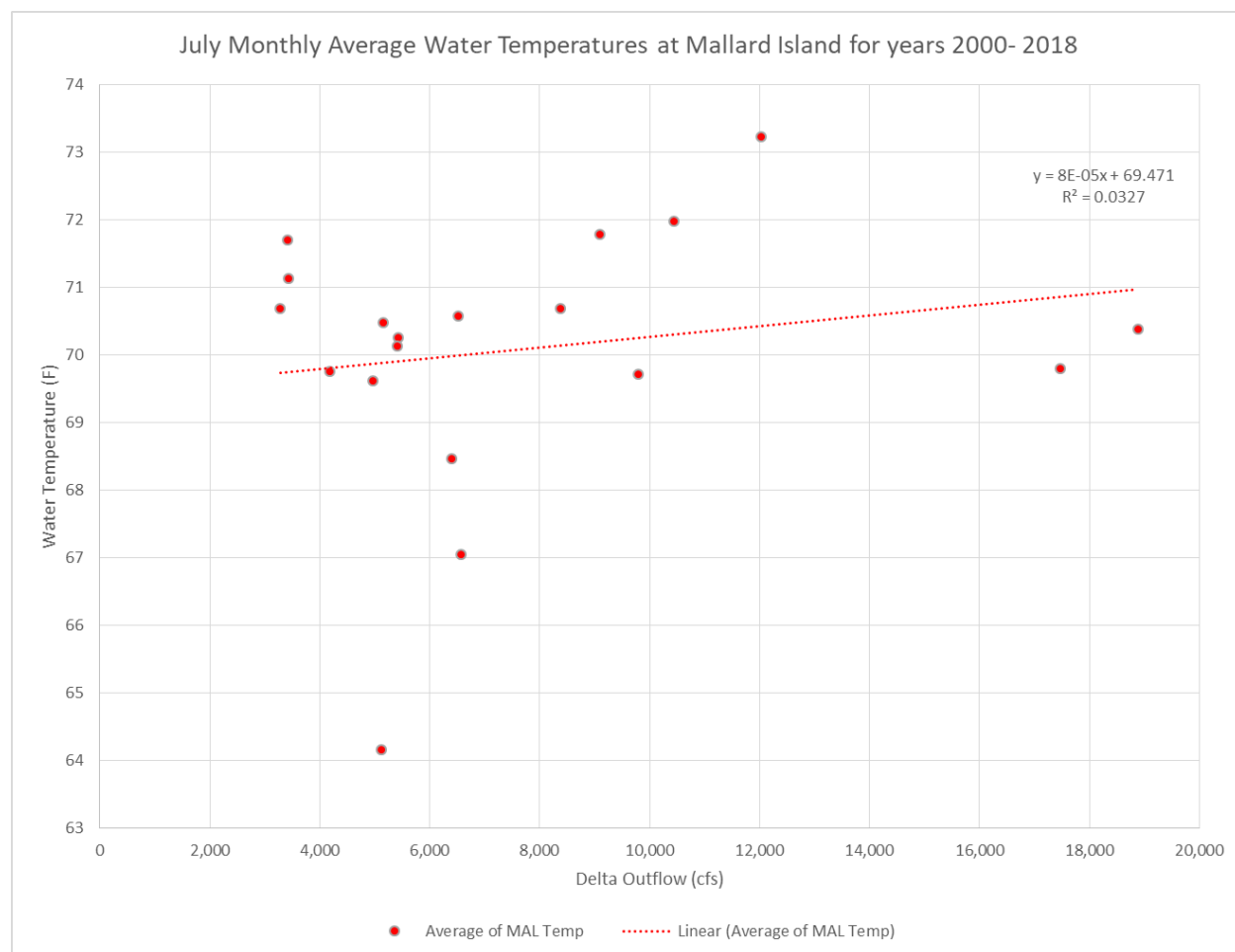
Figure 5.16-50. Average monthly July temperature at Mallard Island versus Delta outflow, 2000 – 2018.
