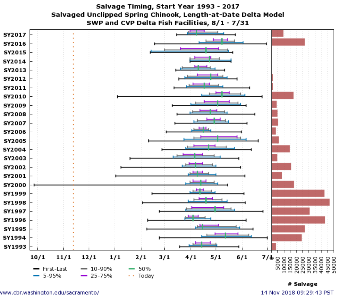
Figure 5.8-50. Salvage of Spring-run Chinook Salmon from 2009 - 2018.
