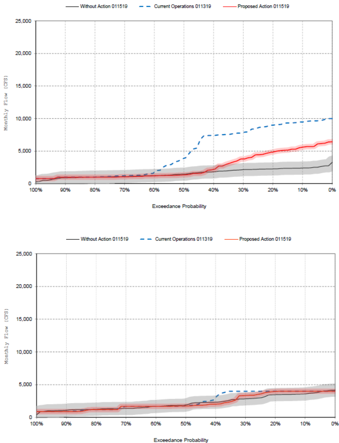
Figure 5.8-31. CalSimII estimates of Feather River flow below the Thermalito Afterbay in September and October under the WOA (Without Action), COS (Current Operations), and PA (Proposed Action) scenarios.
