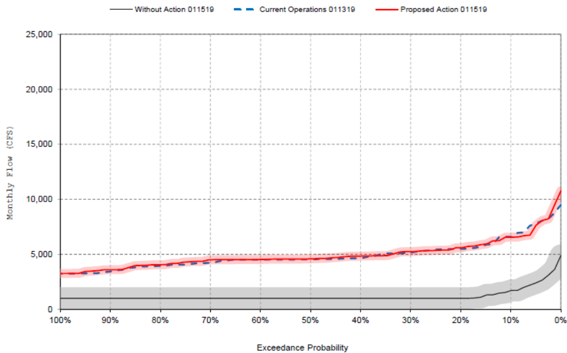
Figure 5.8-17. Modeled Sacramento River Flows at Wilkins Slough, August
