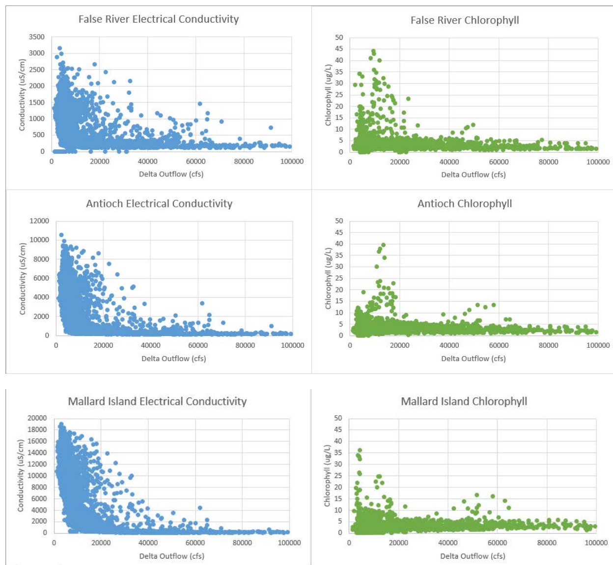
Figure 5.16-49. Raw daily electrical conductivity and chlorophyll from the sensors at False River, Antioch, and Mallard Island from 2007 onwards.
