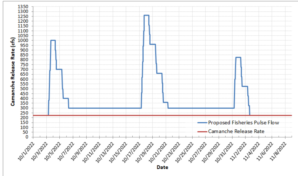
Figure A1. October 2022 Mokelumne River Pulse Flow plan (source: 2022 Camanche Pulse Flow Plan_Schedule; tab: Pulse Flow – Hourly INPUT)
