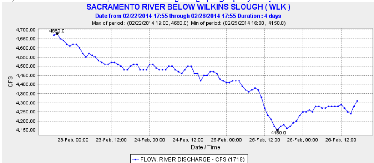
Figure 8: Real time Sacramento River discharges at Wilkins Slough for the week of February 23, 2014. Available at: http://cdec.water.ca.gov/cgi-progs/queryDaily?WLK
