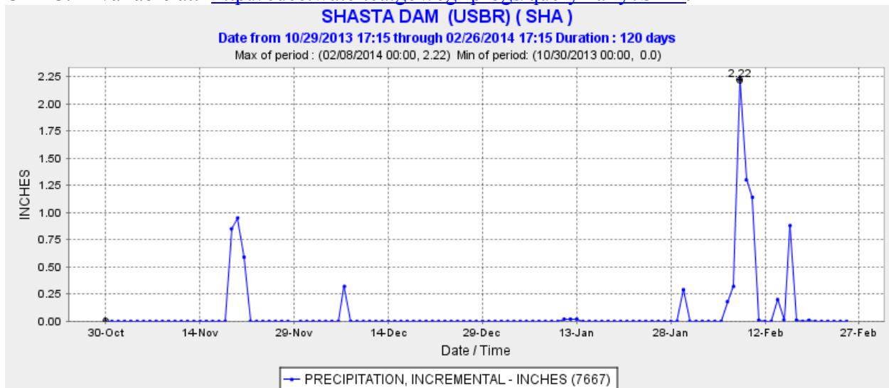
Figure 6: Shasta Dam (SHA) incremental precipitation for the water year 2014 (to date) from CDEC. Available at: http://cdec.water.ca.gov/cgi-progs/queryDaily?SHA .
