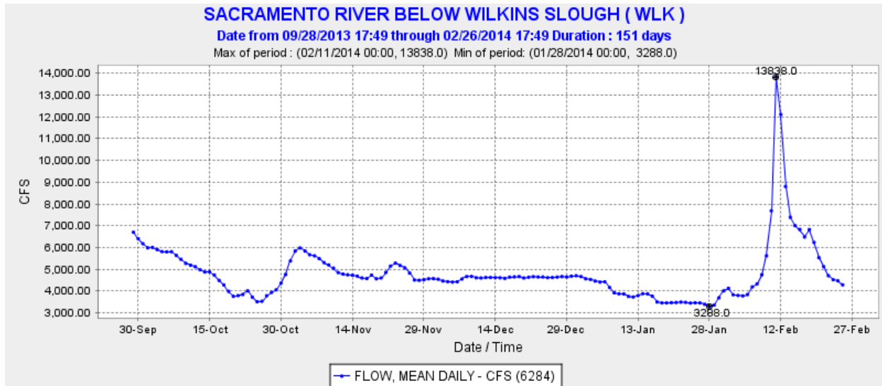
Figure 7: Daily Sacramento River discharges as measured at Wilkins Slough measured in cubic feet per second (cfs) for water year 2014. Available at: http://cdec.water.ca.gov/jspplot/jspPlotServlet.jsp?sensor_no=6284&end=02%2F26%2F2014+17%3A49&geom=medium&interval=151&cookies=cdec01 .
