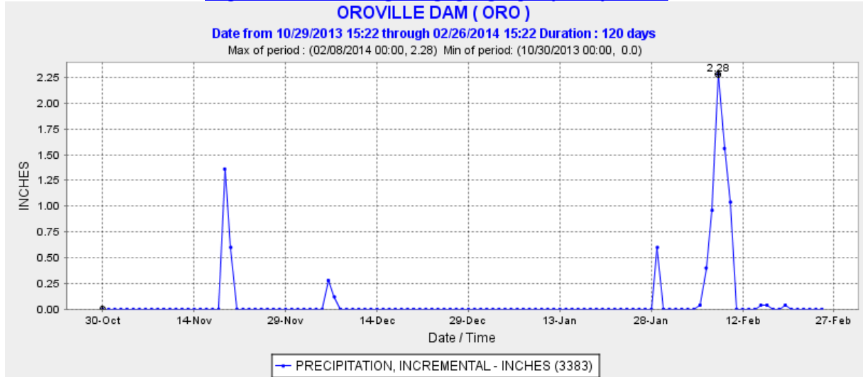
Figure 5: Oroville Dam (ORO) incremental precipitation for the water year 2014 (to date) from CDEC. Available at: http://cdec.water.ca.gov/cgi-progs/queryDaily?ORO .
