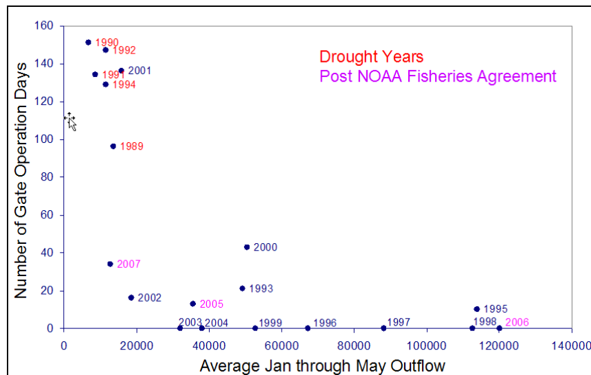
1 2 Figure 0-10 SMSCG operation frequency versus outflow since 1988.
