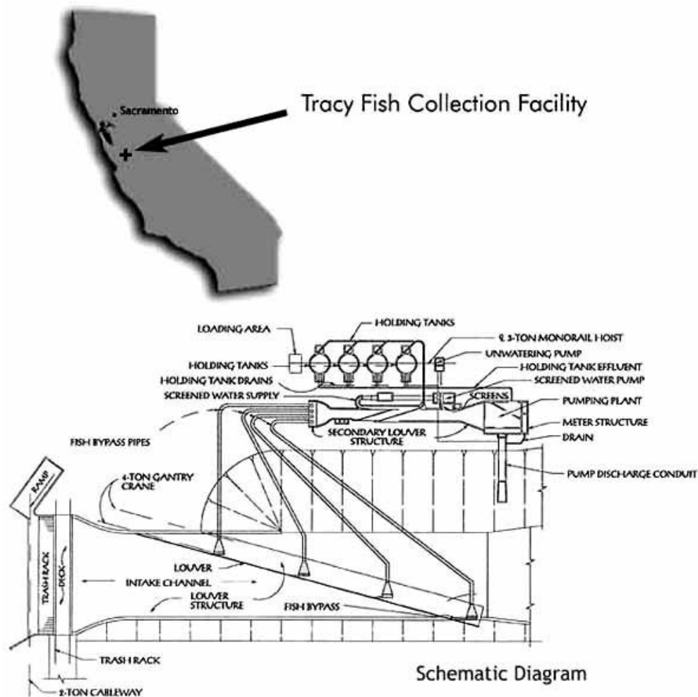
21 Figure 2-8 Tracy Fish Collection Facility Diagram
