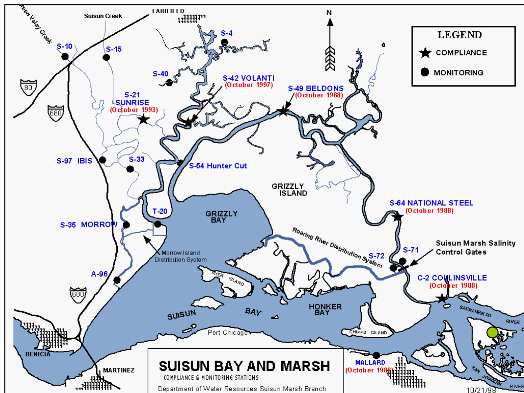
6 7 Figure 0-8 Compliance and monitoring stations and salinity control facilities in Suisun Marsh.
