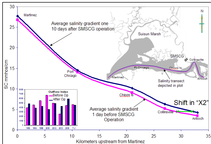
14 Figure 0-9 Average of seven years salinity response to SMSCG gate operation in Montezuma 15 Slough and Suisun Bay.
