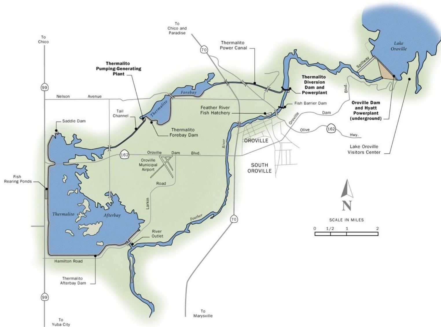
Figure 2-73 Oroville Facilities on the Feather River
