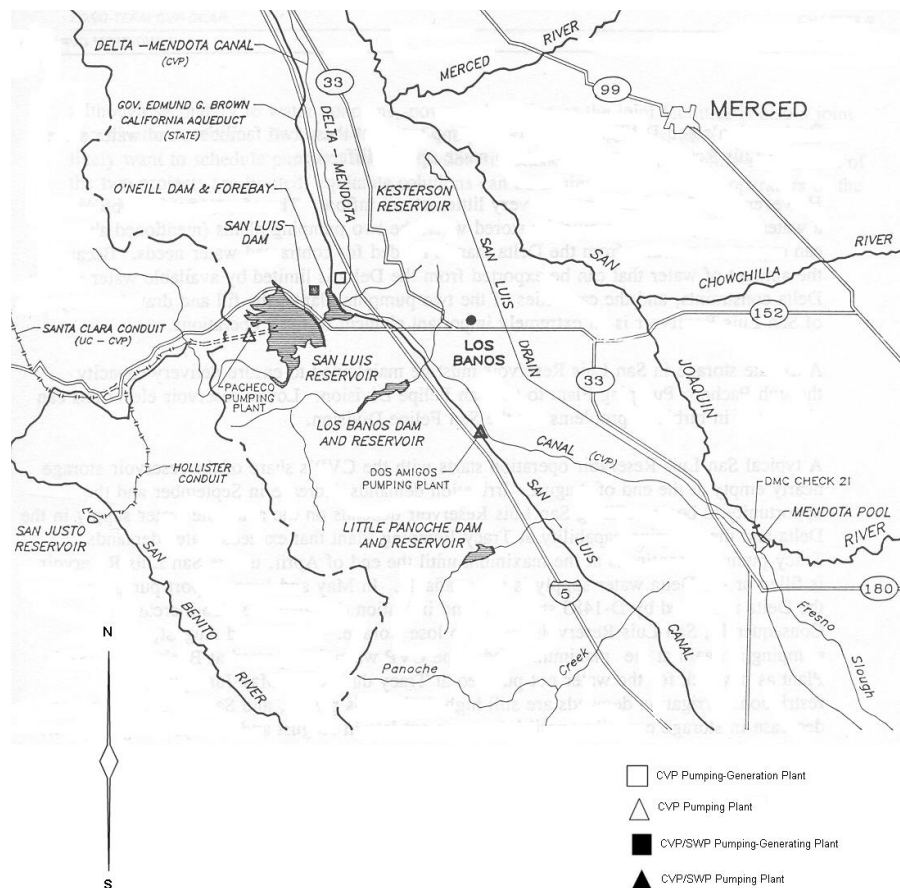
19 20 Figure 2-10 West San Joaquin Division and San Felipe Division
