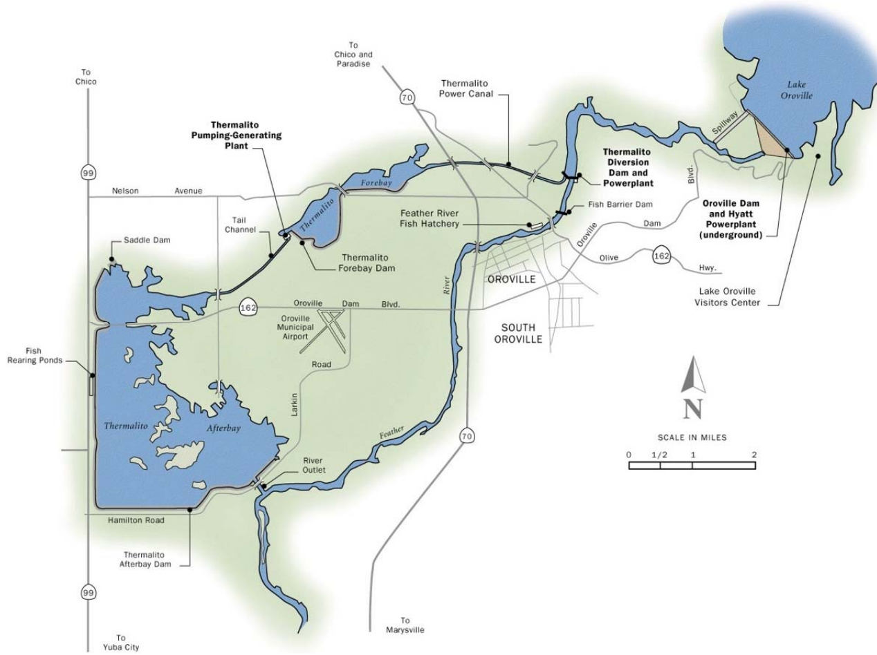
Figure 2-743 Oroville Facilities on the Feather River
