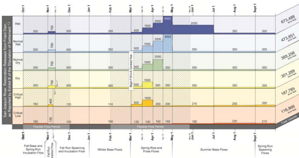
Figure 2-15 Settlement Flow Target Releases from Friant Dam
