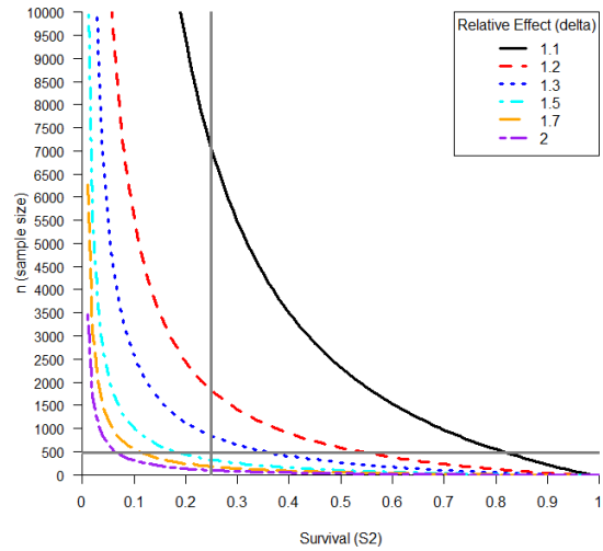
Figure A2A8. Sample sizes ( n ) necessary versus survival ( S_2 ) to achieve 80% power to detect a relative effect of size \delta in a one-tailed test with a single replicate ( \alpha=0.10 ). Survival and detection parameters are: S_1=0.55 , p_1=0.75 , p_{2a}=p_{2b}=0.85 . The cross-bars indicate the assumed survival via salvage for a high survival year, and the observed sample size in 2011 (steelhead).
