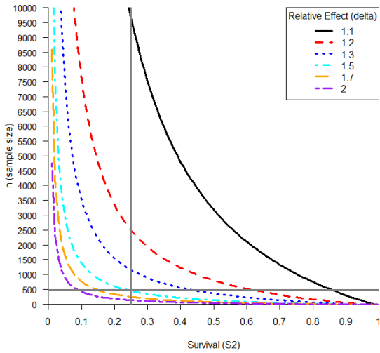
Figure A2A7. Sample sizes ( n ) necessary versus survival ( S_2 ) to achieve 80% power to detect a relative effect of size \delta in a one-tailed test with a single replicate ( \alpha=0.05 ). Survival and detection parameters are: S_1=0.55 , p_1=0.75 , p_{2a}=p_{2b}=0.85 . The cross-bars indicate the assumed survival via salvage for a high survival year, and the observed sample size in 2011 (steelhead).
