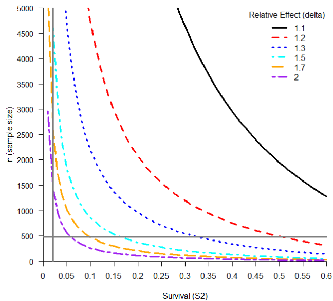
Figure A2A6. Sample sizes ( n ) necessary versus survival ( S_2 ) to achieve 80% power to detect a relative effect of size delta ( \delta ) in a one-tailed test with a single replicate ( \alpha=0.10 ). Survival and detection parameters are: S_1=0.50 , p_1=0.95 , p_{2a}=p_{2b}=0.90 . The cross-bars indicate the observed survival and sample size in 2011 (Chinook salmon).
