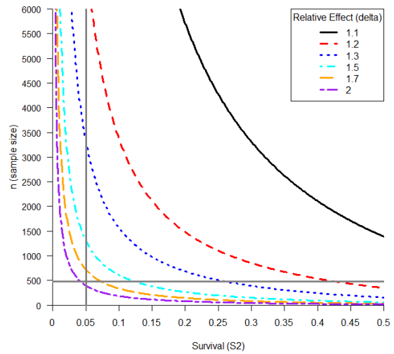
Figure A2A14. Sample sizes ( n ) necessary versus survival ( S_2 ) to achieve 80% power to detect a relative effect of size \delta in a one-tailed test with a single replicate ( \alpha=0.10 ). Survival and detection parameters are: S_1=0.70 , p_1=0.95 , p_{2a}=p_{2b}=0.90 . The cross-bars indicate the assumed survival via salvage for a low survival year, and the observed sample size in 2011 (Chinook).
