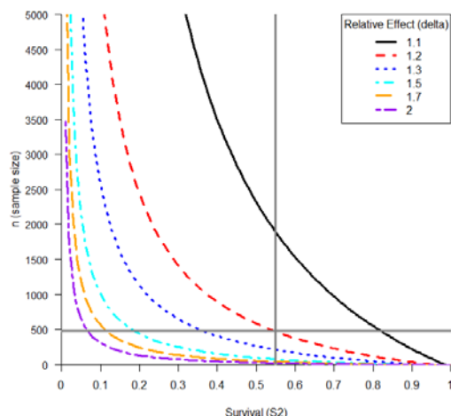
Figure A1. Sample sizes ( n ) necessary versus survival ( S_2 ) to achieve 80% power to detect a relative effect of size \delta in a one-tailed test with a single replicate ( \alpha=0.10 ). Survival and detection parameters are: S_1=0.55 , p_1=0.75 , p_{2a}=p_{2b}=0.88 . The cross-bars indicate the observed survival and sample size in 2011 (steelhead).
