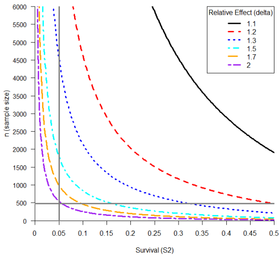
Figure A2A13. Sample sizes ( n ) necessary versus survival ( S_2 ) to achieve 80% power to detect a relative effect of size \delta in a one-tailed test with a single replicate ( \alpha=0.05 ). Survival and detection parameters are: S_1=0.70 , p_1=0.95 , p_{2a}=p_{2b}=0.90 . The cross-bars indicate the assumed survival via salvage for a low survival year, and the observed sample size in 2011 (Chinook).
