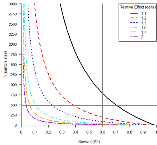
Figure A2A12. Sample sizes ( n ) necessary versus survival ( S_2 ) to achieve 80% power to detect a relative effect of size delta ( \delta ) in a one-tailed test with a single replicate ( \alpha=0.10 ). Survival and detection parameters are: S_1=0.95 , p_1=0.85 , p_{2a}=p_{2b}=0.85 . The cross-bars indicate the assumed survival via salvage for a high survival year, and the observed sample size in 2011 (steelhead).
