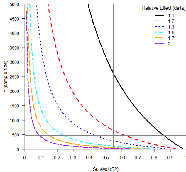
Figure A2A1. Sample sizes ( n ) necessary versus survival ( S_2 ) to achieve 80% power to detect a relative effect of size \delta in a one-tailed test with a single replicate ( \alpha=0.05 ). Survival and detection parameters are: S_1=0.55 , p_1=0.75 , p_{2a}=p_{2b}=0.85 . The cross-bars indicate the observed survival and sample size in 2011 (steelhead).
