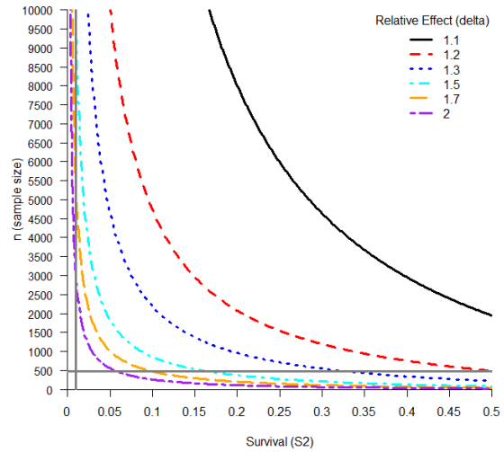
Figure A2A10. Sample sizes ( n ) necessary versus survival ( S_2 ) to achieve 80% power to detect a relative effect of size delta ( \delta ) in a one-tailed test with a single replicate ( \alpha=0.10 ). Survival and detection parameters are: S_1=0.50 , p_1=0.95 , p_{2a}=p_{2b}=0.90 . The cross-bars indicate the assumed survival via salvage for a low survival year, and the observed sample size in 2011 (Chinook).
