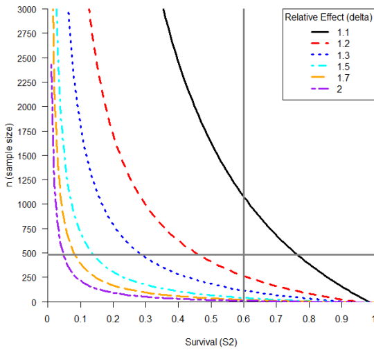
Figure A2A11. Sample sizes ( n ) necessary versus survival ( S_2 ) to achieve 80% power to detect a relative effect of size delta ( \delta ) in a one-tailed test with a single replicate ( \alpha=0.05 ). Survival and detection parameters are: S_1=0.95 , p_1=0.85 , p_{2a}=p_{2b}=0.85 . The cross-bars indicate the assumed survival via salvage for a high survival year, and the observed sample size in 2011 (steelhead).
