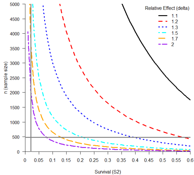
Figure A2A5. Sample sizes ( n ) necessary versus survival ( S_2 ) to achieve 80% power to detect a relative effect of size delta ( \delta ) in a one-tailed test with a single replicate ( \alpha=0.05 ). Survival and detection parameters are: S_1=0.50 , p_1=0.95 , p_{2a}=p_{2b}=0.90 . The cross-bars indicate the observed survival and sample size in 2011 (Chinook salmon).
