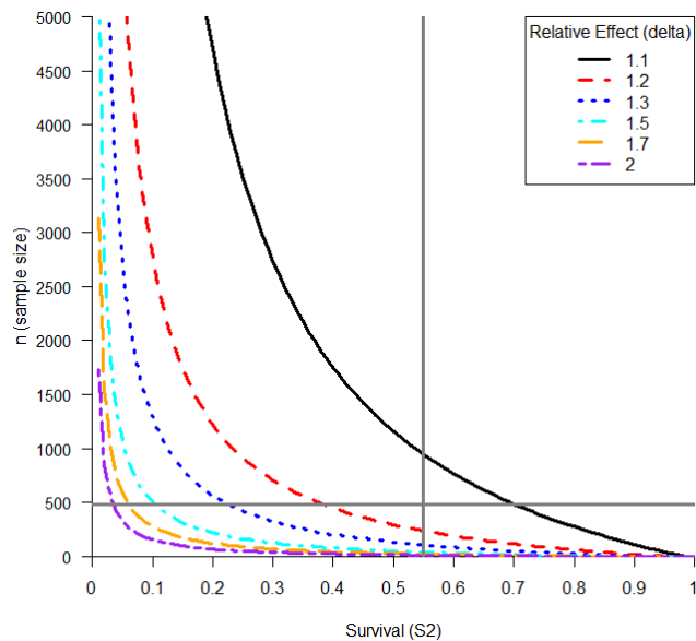
Figure A2A4. Sample sizes ( n ) necessary versus survival ( S_2 ) to achieve 80% power to detect a relative effect of size \delta in a one-tailed test with two replicates ( \alpha=0.10 ). Survival and detection parameters are: S_1=0.55 , p_1=0.75 , p_{2a}=p_{2b}=0.88 . The cross-bars indicate the observed survival and sample size in 2011 (steelhead).
