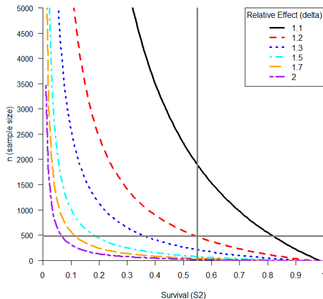
Figure A2A2. Sample sizes ( n ) necessary versus survival ( S_2 ) to achieve 80% power to detect a relative effect of size \delta in a one-tailed test with a single replicate ( \alpha=0.10 ). Survival and detection parameters are: S_1=0.55 , p_1=0.75 , p_{2a}=p_{2b}=0.88 . The cross-bars indicate the observed survival and sample size in 2011 (steelhead).
