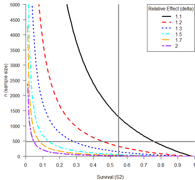
Figure A2A3. Sample sizes ( n ) necessary versus survival ( S_2 ) to achieve 80% power to detect a relative effect of size \delta in a one-tailed test with two replicates ( \alpha=0.05 ). Survival and detection parameters are: S_1=0.55 , p_1=0.75 , p_{2a}=p_{2b}=0.88 . The cross-bars indicate the observed survival and sample size in 2011 (steelhead).
