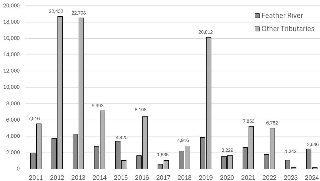
Figure 2. Annual spring-run Chinook Salmon escapement estimates. (2024 values are preliminary; PFMC 2025 )
