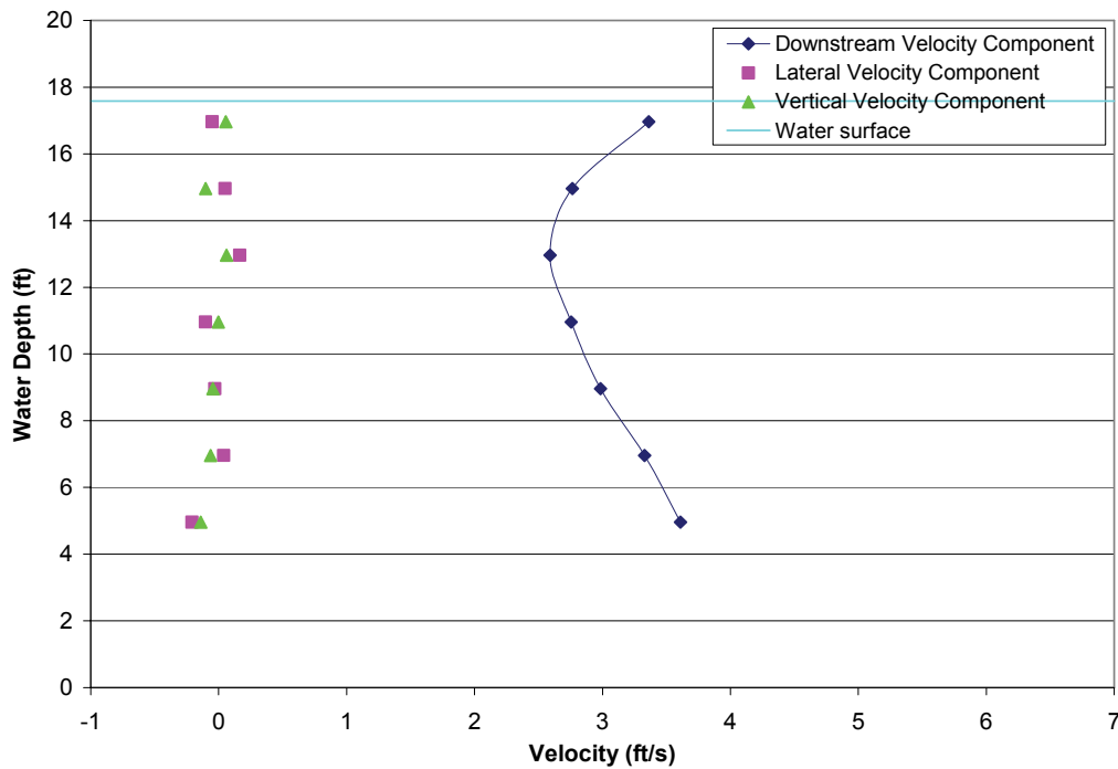
FIGURE A2-1.—Test 2-1, bypass 1 intake profile with all bypasses open, measured bypass ratio = N/A, bypass ratio with facility instruments = 0.86, high tide, water depth = 17.59 ft, trashrack differential = 0.76 ft, louvers differential = 0.72 ft.
