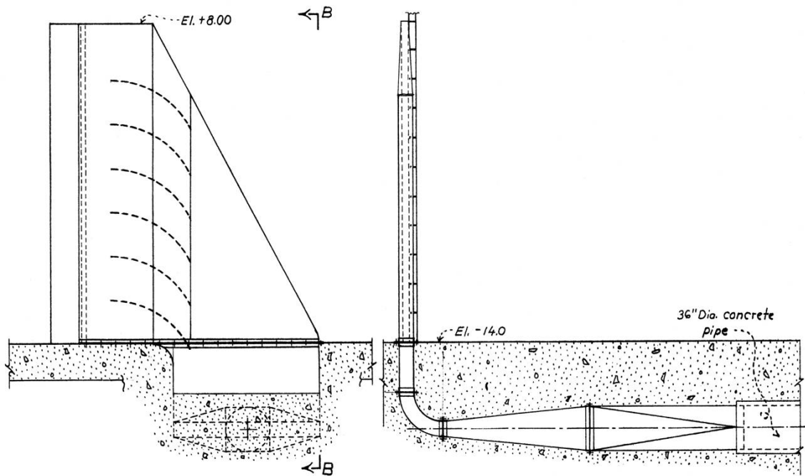
FIGURE 3.—Original bypass intake design using internal curved vanes from 1956.
