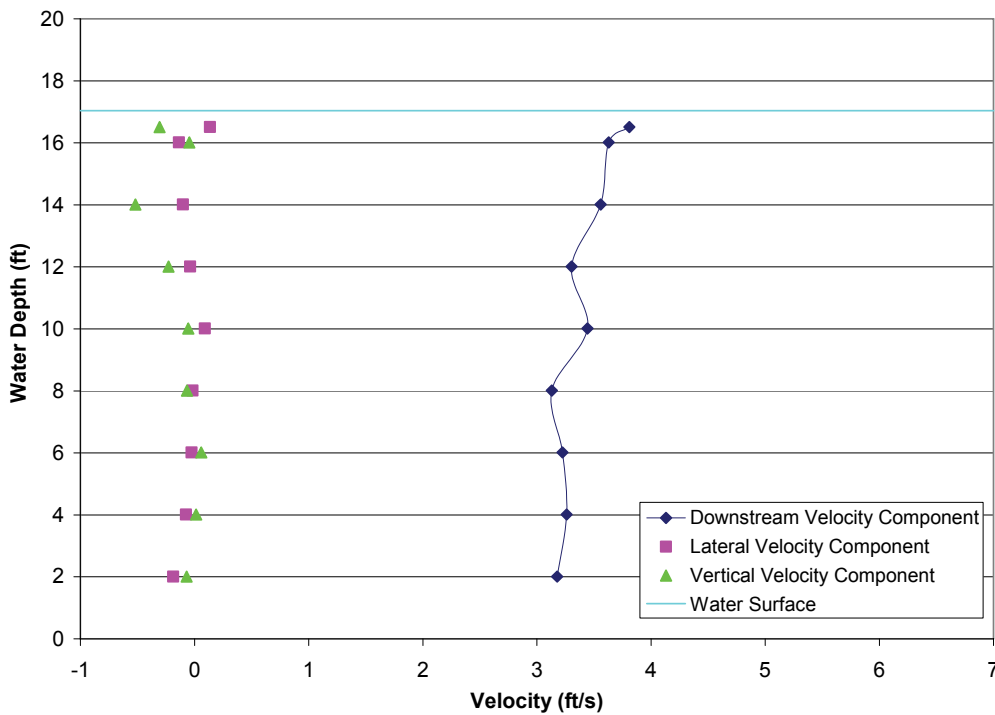
FIGURE A2-11.—Test 3-2, bypass 2 intake profile with all bypasses open, measured bypass ratio = 1.02, bypass ratio with facility instruments = 0.79, outgoing tide, water depth = 17.04 ft, trashrack differential = 1.11 ft, louvers differential = 0.55 ft.
