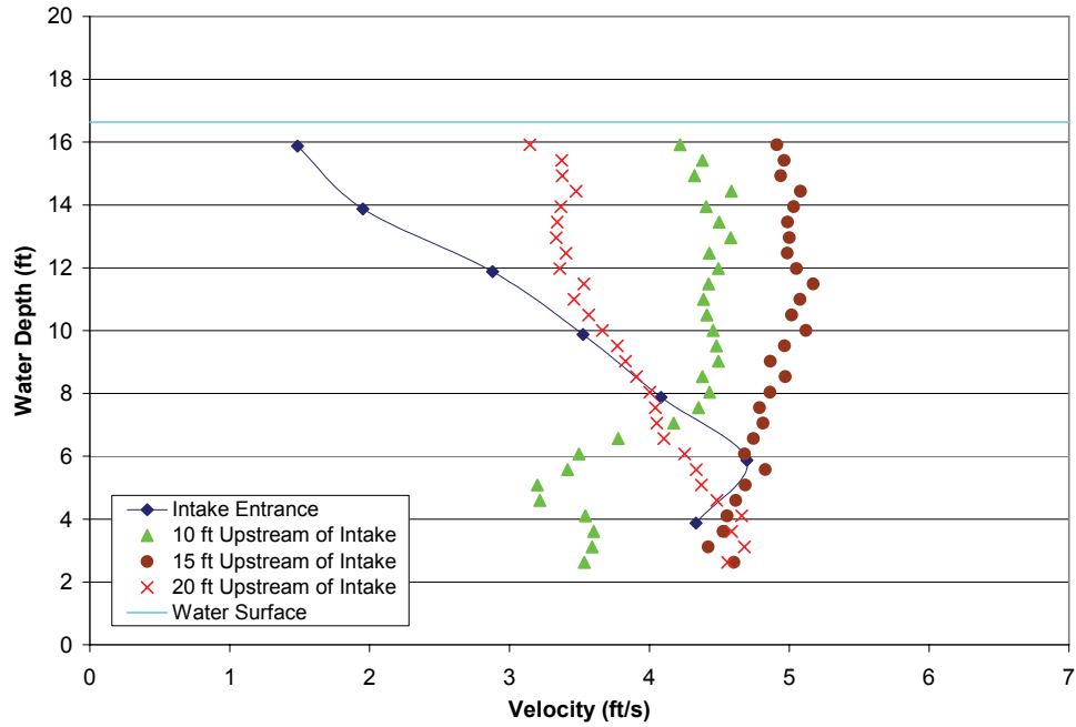
FIGURE A1-4.—Test 1B, bypass 1 approach velocity profiles away from louvers with all bypasses open, measured bypass ratio = 0.80, bypass ratio with facility instruments = 0.69, incoming tide, water depth = 16.64 ft, recently cleaned trashrack and louvers.
