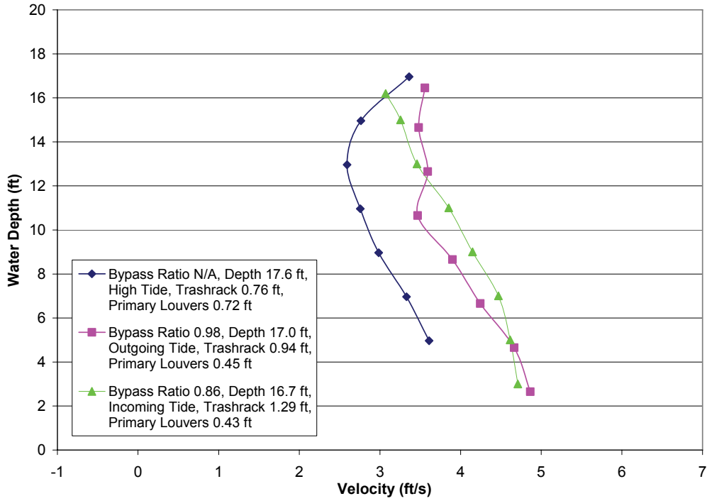
FIGURE 16.—Velocity profiles in the replacement primary bypass 1 intake entrance.
