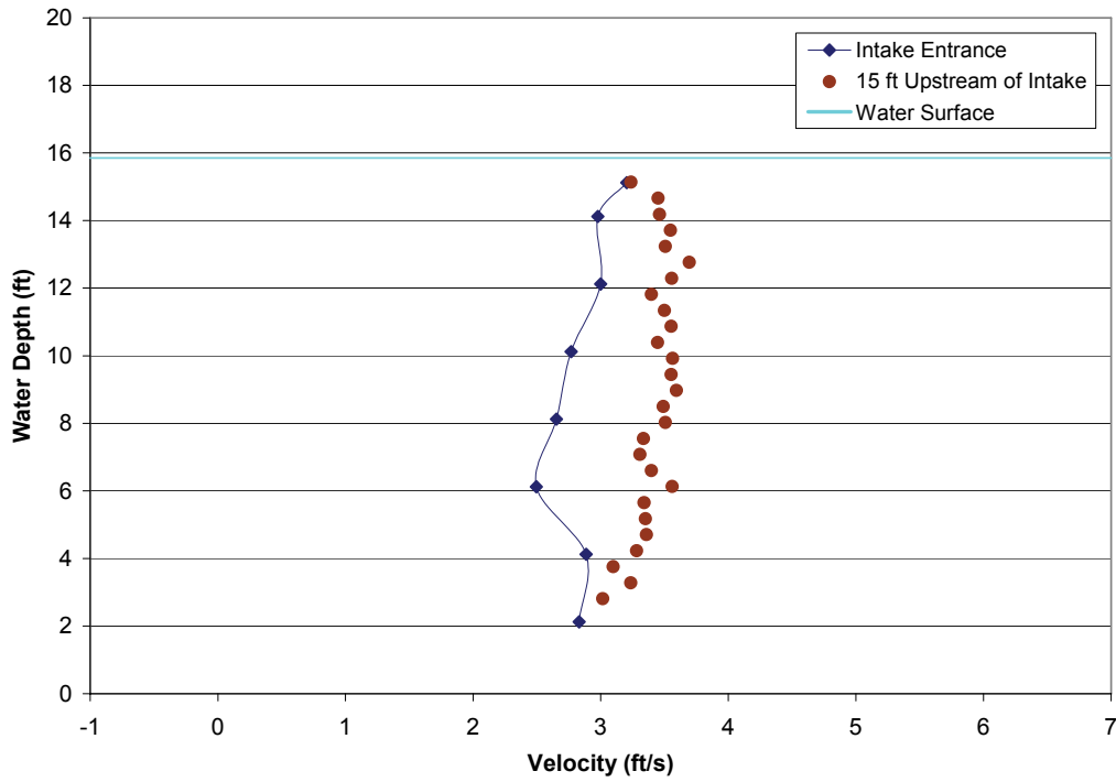
FIGURE A2-30.—Test 1C, bypass 4 approach velocity profiles with bypass 1 and 2 closed, measured bypass ratio = 0.88, bypass ratio with facility instruments = 0.94, outgoing tide, water depth = 15.85 ft, trashrack differential = 1.52 ft, louvers differential = 0.59 ft.
