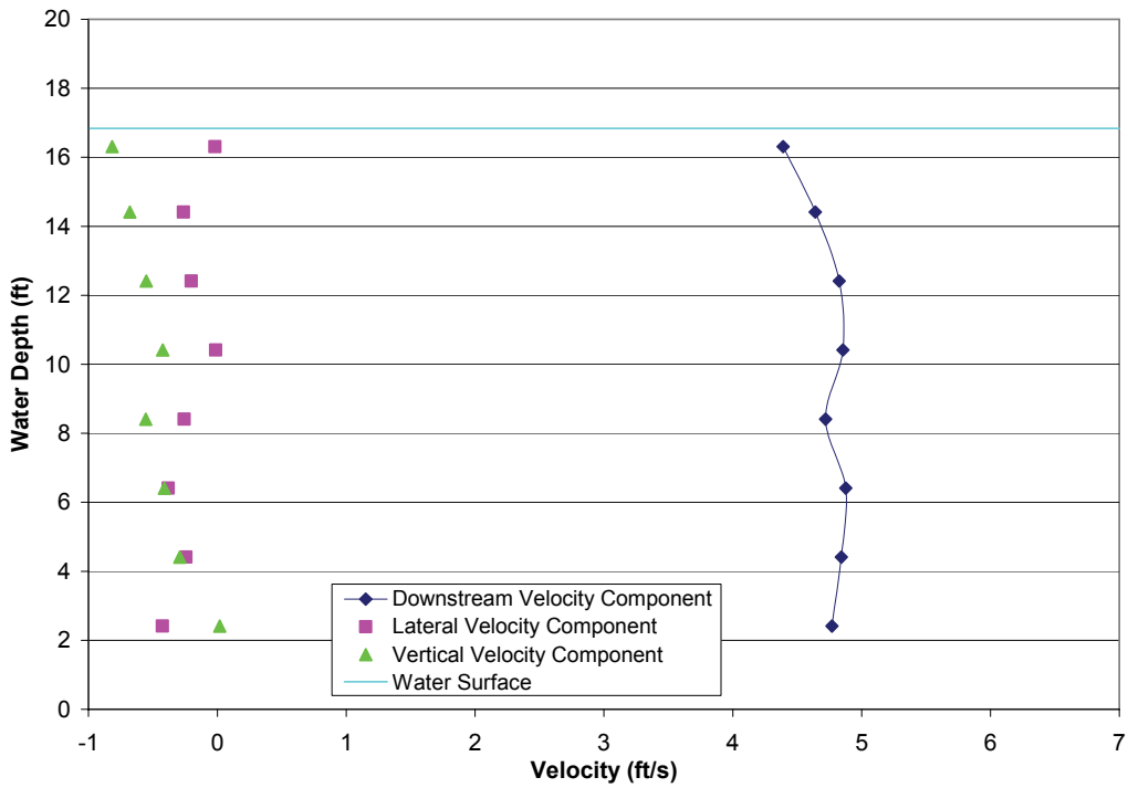
FIGURE A2-33.—Test 5A, bypass 4 intake profile with bypass 1 and 2 closed, measured bypass ratio = 1.24, bypass ratio with facility instruments = 1.41, outgoing tide, water depth = 16.84 ft, trashrack differential = 1.09 ft, louvers differential = 0.56 ft.
