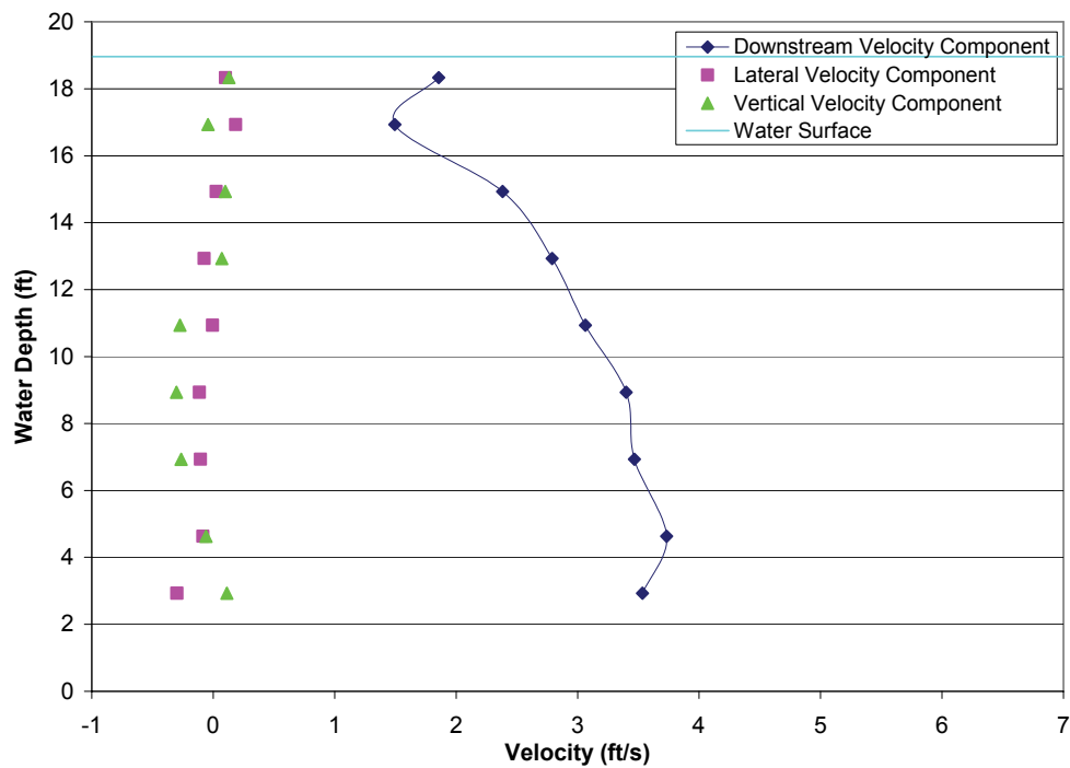
FIGURE A2-21.—Test 4-3, bypass 3 intake profile with all bypasses open, measured bypass ratio = 0.98, bypass ratio with facility instruments = 0.74, incoming tide, water depth = 18.96 ft, trashrack differential = 1.07 ft, louvers differential = 0.37 ft.
