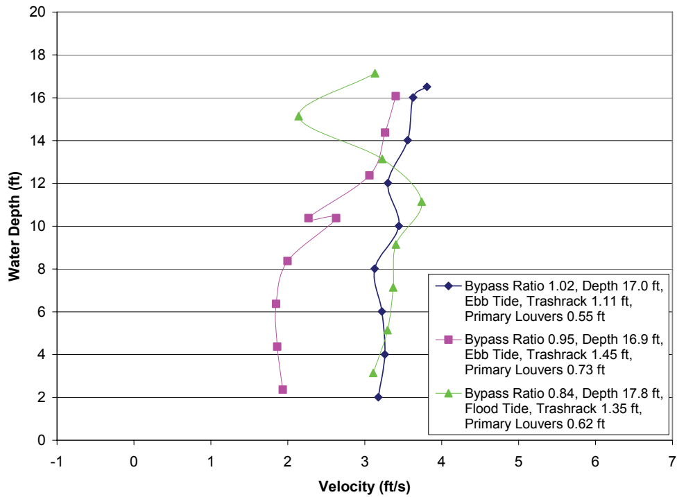
FIGURE 17.—Velocity profiles in the replacement primary bypass 2 intake entrance.
