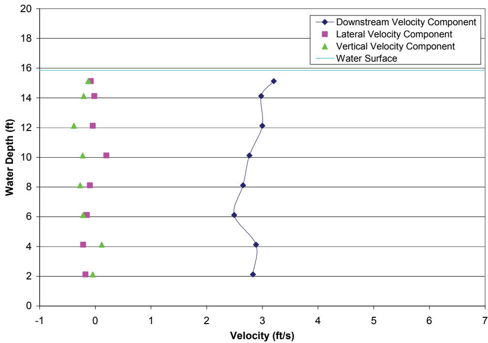
FIGURE A2-29.—Test 1C, bypass 4 intake profile with bypass 1 and 2 closed, measured bypass ratio = 0.88, bypass ratio with facility instruments = 0.94, outgoing tide, water depth = 15.85 ft, trashrack differential = 1.52 ft, louvers differential = 0.59 ft.
