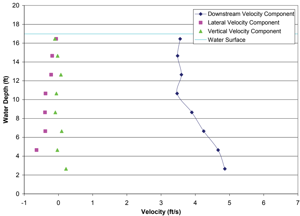
FIGURE A2-9.—Test 3-1, bypass 1 intake profile with all bypasses open, measured bypass ratio = 0.98, bypass ratio with facility instruments = 1.27, outgoing tide, water depth = 16.98 ft, trashrack differential = 0.94 ft, louvers differential = 0.45 ft.
