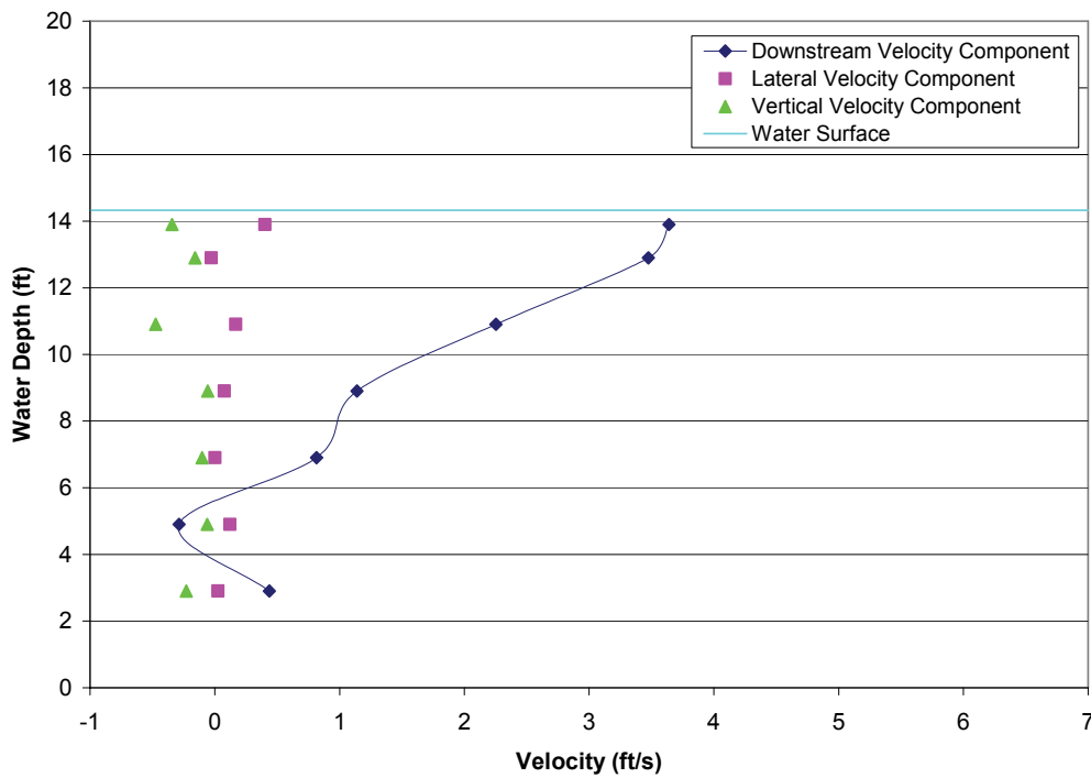
FIGURE A2-7.—Test 2-4, bypass 4 intake profile with all bypasses open, measured bypass ratio = 0.37, bypass ratio with facility instruments = N/A, outgoing tide, water depth = 14.33 ft, trashrack differential = 2.98 ft, louvers differential = 1.19 ft.
