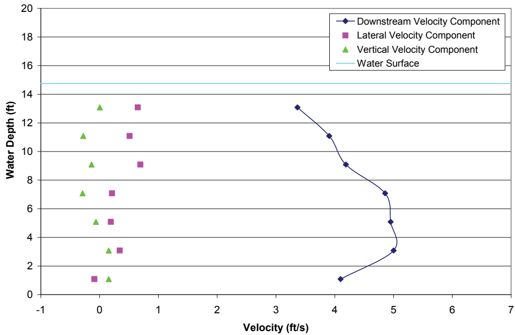
FIGURE A1-1.—Test 1A, bypass 1 intake profile with all bypasses open, measured bypass ratio = N/A, bypass ratio with facility instruments = N/A, incoming tide, water depth = 14.75 ft, recently cleaned trashrack and louvers.
