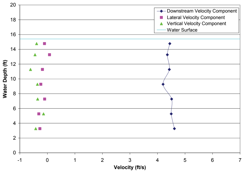
FIGURE A2-31.—Test 1D, bypass 4 intake profile with bypass 1, 2, and 3 closed, measured bypass ratio = 1.32, bypass ratio with facility instruments = 0.97, outgoing tide, water depth = 15.40 ft, trashrack differential = 1.81 ft, louvers differential = 0.49 ft.
