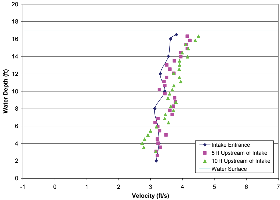
FIGURE 21.—Example of a profile collected with a bypass ratio near 1.0. Test 3-2, collected at bypass 2 with a measured bypass ratio of 1.02, shows similarly shaped approach profiles with a slight deceleration of flow into the intake.
