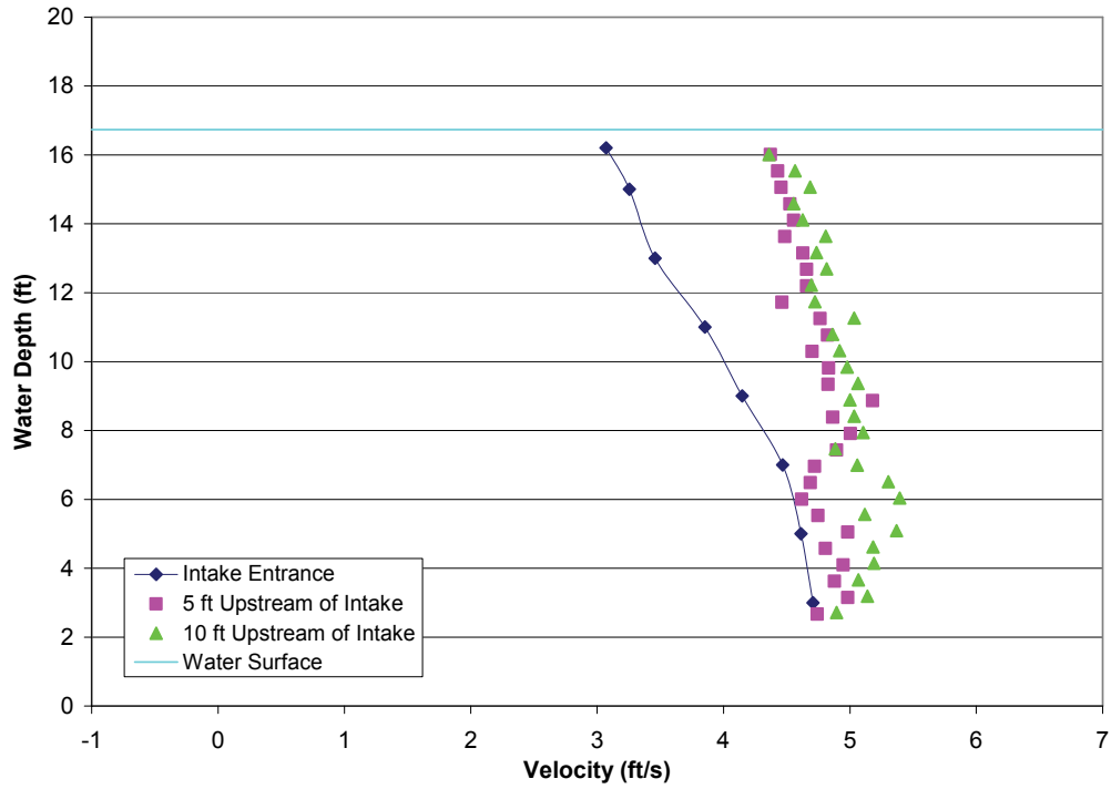
FIGURE A2-18.—Test 4-1, bypass 1 approach velocity profiles with all bypasses open, measured bypass ratio = 0.86, bypass ratio with facility instruments = 1.17, incoming tide, water depth = 16.73 ft, trashrack differential = 1.29 ft, louvers differential = 0.43 ft.
