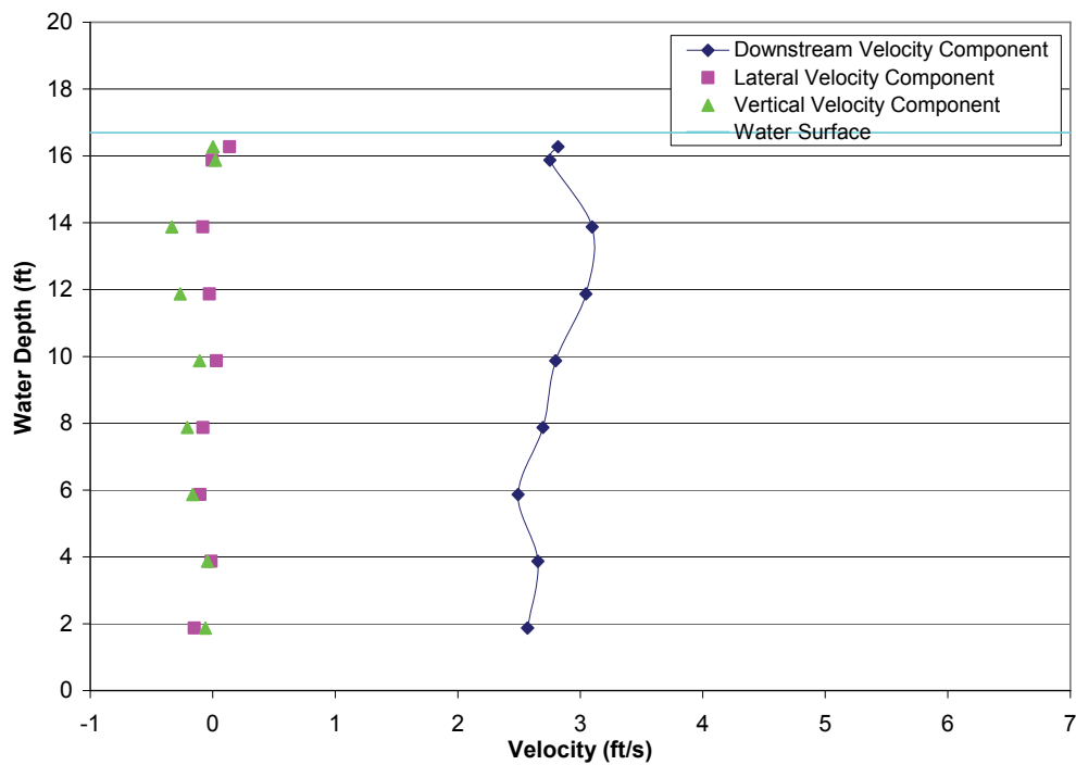
FIGURE A2-23.—Test 4-4, bypass 4 intake profile with all bypasses open, measured bypass ratio = 0.87, bypass ratio with facility instruments = 0.90, high tide, water depth = 16.70 ft, trashrack differential = 1.27 ft, louvers differential = 0.49 ft.
