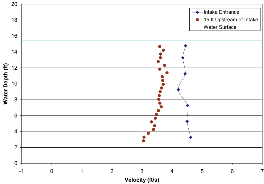
FIGURE A2-32.—Test 1D, bypass 4 approach velocity profiles with bypass 1, 2, and 3 closed, measured bypass ratio = 1.32, bypass ratio with facility instruments = 0.97, outgoing tide, water depth = 15.40 ft, trashrack differential = 1.81 ft, louvers differential = 0.49 ft.
