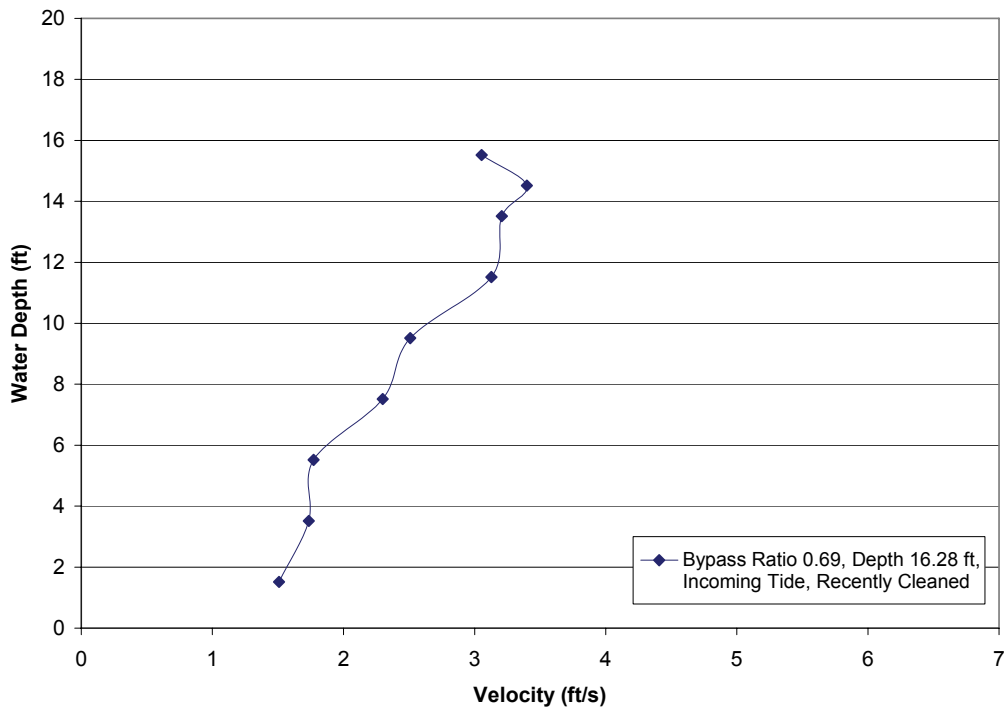
FIGURE 15.—Velocity profiles in the original primary bypass 4 intake entrance.
