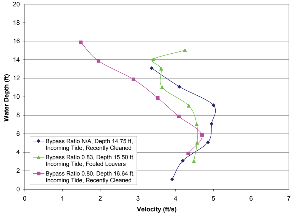
FIGURE 14.—Velocity profiles in the original primary bypass 1 intake entrance.
