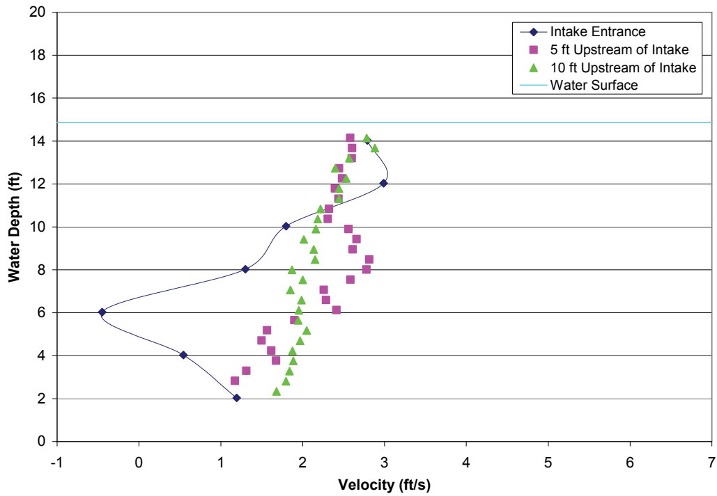
FIGURE A2-6.—Test 2-3, bypass 3 approach velocity profiles with all bypasses open, measured bypass ratio = 0.69, bypass ratio with facility instruments = N/A, outgoing tide, water depth = 14.86 ft, trashrack differential = 3.03 ft, louvers differential = 0.74 ft.
