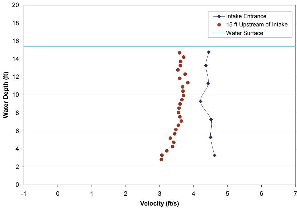
FIGURE 22.—Example of a profile collected with a bypass ratio greater than 1.0. Test 1D, collected at bypass 4 with a measured bypass ratio of 1.32, shows an acceleration of flow into the intake.
