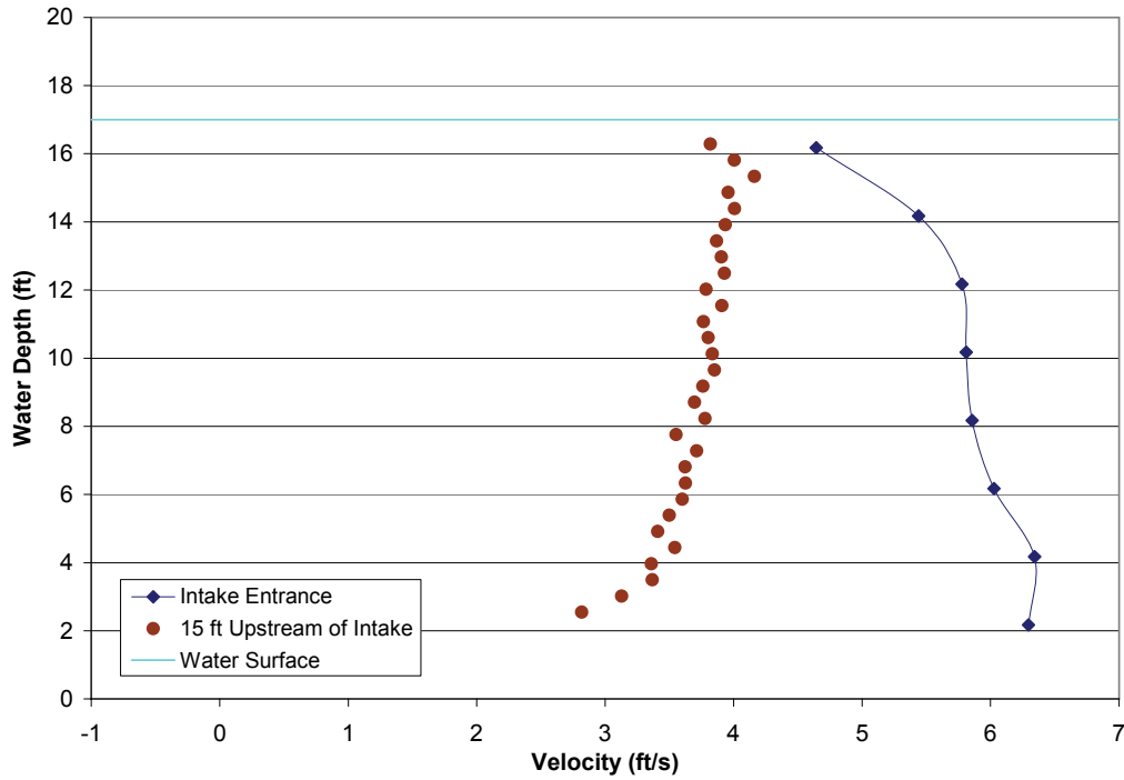
FIGURE A2-36.—Test 5B, bypass 4 approach velocity profiles with bypass 1, 2, and 3 closed, measured bypass ratio = 1.63, bypass ratio with facility instruments = 1.86, outgoing tide, water depth = 17.00 ft, trashrack differential = 0.80 ft, louvers differential = 0.59 ft.
