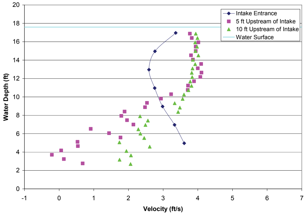
FIGURE A2-2.—Test 2-1, bypass 1 approach velocity profiles with all bypasses open, measured bypass ratio = N/A, bypass ratio with facility instruments = 0.86, high tide, water depth = 17.59 ft, trashrack differential = 0.76 ft, louvers differential = 0.72 ft.
