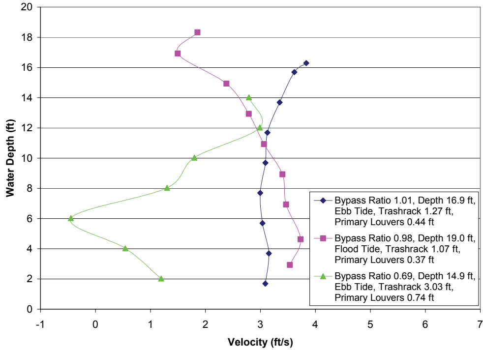
FIGURE 18.—Velocity profiles in the replacement primary bypass 3 intake entrance.
