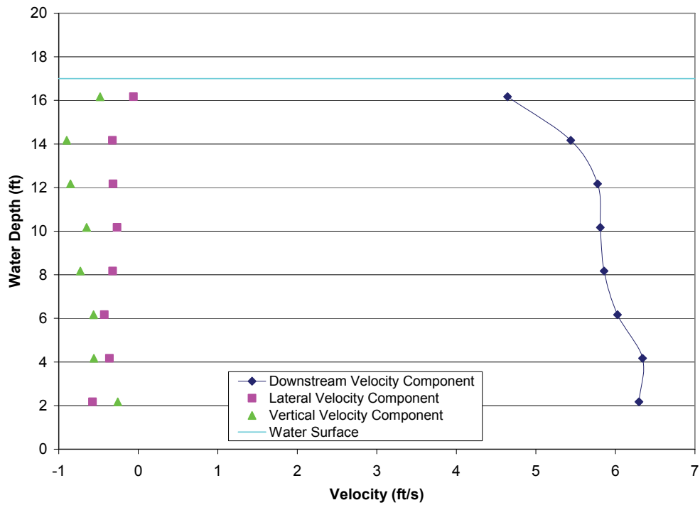
FIGURE A2-35.—Test 5B, bypass 4 intake profile with bypass 1, 2, and 3 closed, measured bypass ratio = 1.63, bypass ratio with facility instruments = 1.86, outgoing tide, water depth = 17.00 ft, trashrack differential = 0.80 ft, louvers differential = 0.59 ft.
