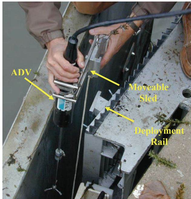
FIGURE 6.—The ADV was attached to a moveable sled to vertically position the instrument along the rail.
