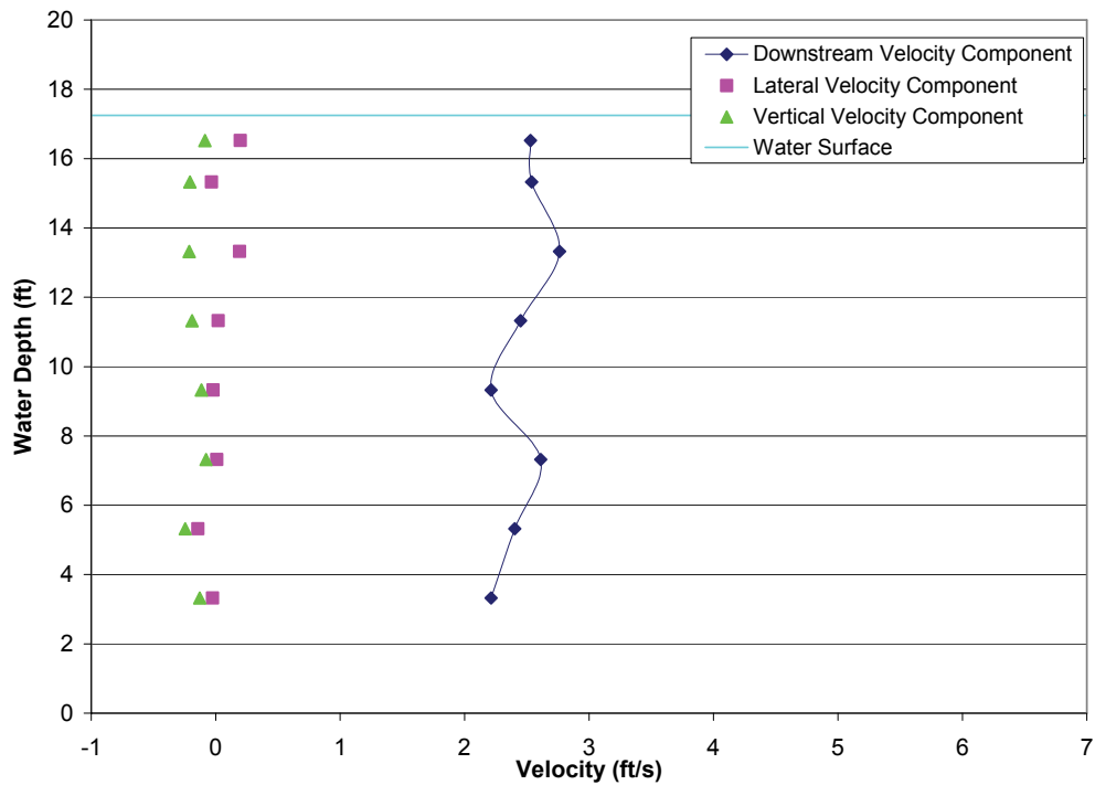
FIGURE A2-15.—Test 3-4, bypass 4 intake profile with all bypasses open, measured bypass ratio = 0.75, bypass ratio with facility instruments = 0.71, incoming tide, water depth = 17.25 ft, trashrack differential = 2.01 ft, louvers differential = 0.70 ft.
