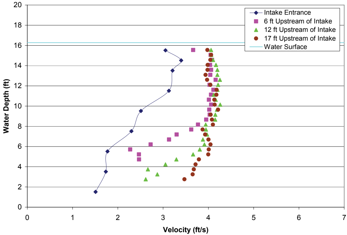
FIGURE A1-10.—Test 4A, bypass 4 approach velocity profiles away from louvers with all bypasses open, measured bypass ratio = 0.69, bypass ratio for facility instruments = 0.46, incoming tide, water depth = 16.28 ft, recently cleaned trashrack and louvers.
