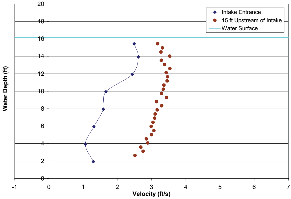
FIGURE A2-28.—Test 1B, bypass 4 approach velocity profiles with bypass 1 closed, measured bypass ratio = 0.61, bypass ratio with facility instruments = 0.64, outgoing tide, water depth = 16.16 ft, trashrack differential = 1.50 ft, louvers differential = 0.5 ft.
