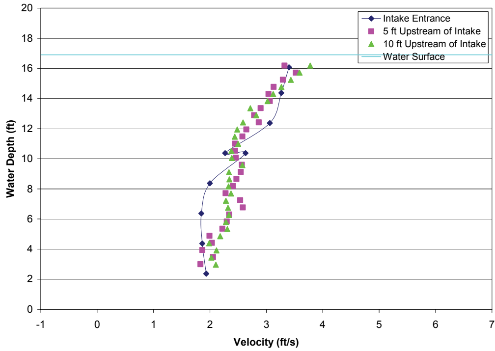
FIGURE A2-4.—Test 2-2, bypass 2 approach velocity profiles with all bypasses open, measured bypass ratio = 0.95, bypass ratio with facility instruments = 0.68, outgoing tide, water depth = 16.90 ft, trashrack differential = 1.45 ft, louvers differential = 0.73 ft.
