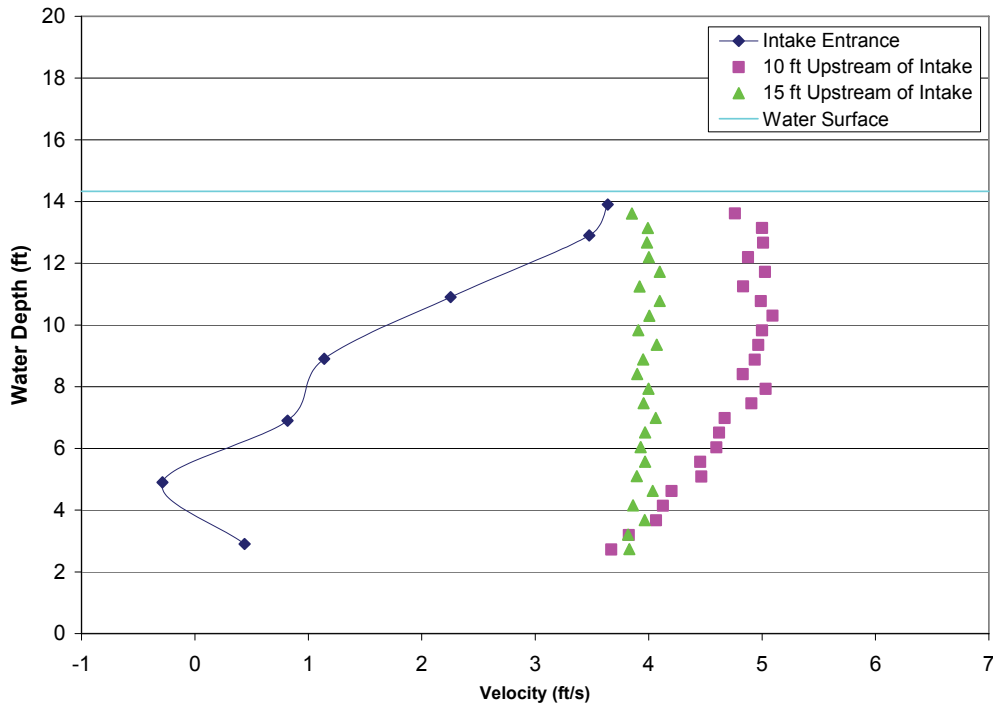
FIGURE A2-8.—Test 2-4, bypass 4 approach velocity profiles with all bypasses open, measured bypass ratio = 0.37, bypass ratio with facility instruments = N/A, outgoing tide, water depth = 14.33 ft, trashrack differential = 2.98 ft, louvers differential = 1.19 ft.
