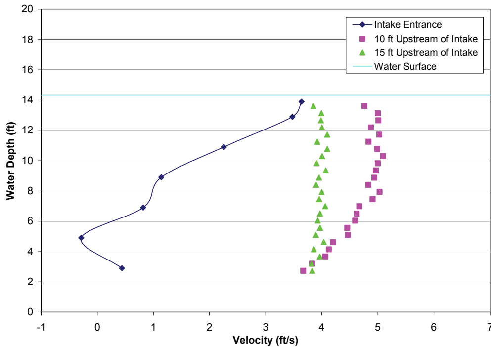
FIGURE 20.—Example of a profile collected with a bypass ratio of less than 1.0. Test 2-4, collected at bypass 4 with a measured bypass ratio of 0.37, shows significant slowing in the approach velocity fields and reverse flows at the intake entrance.
