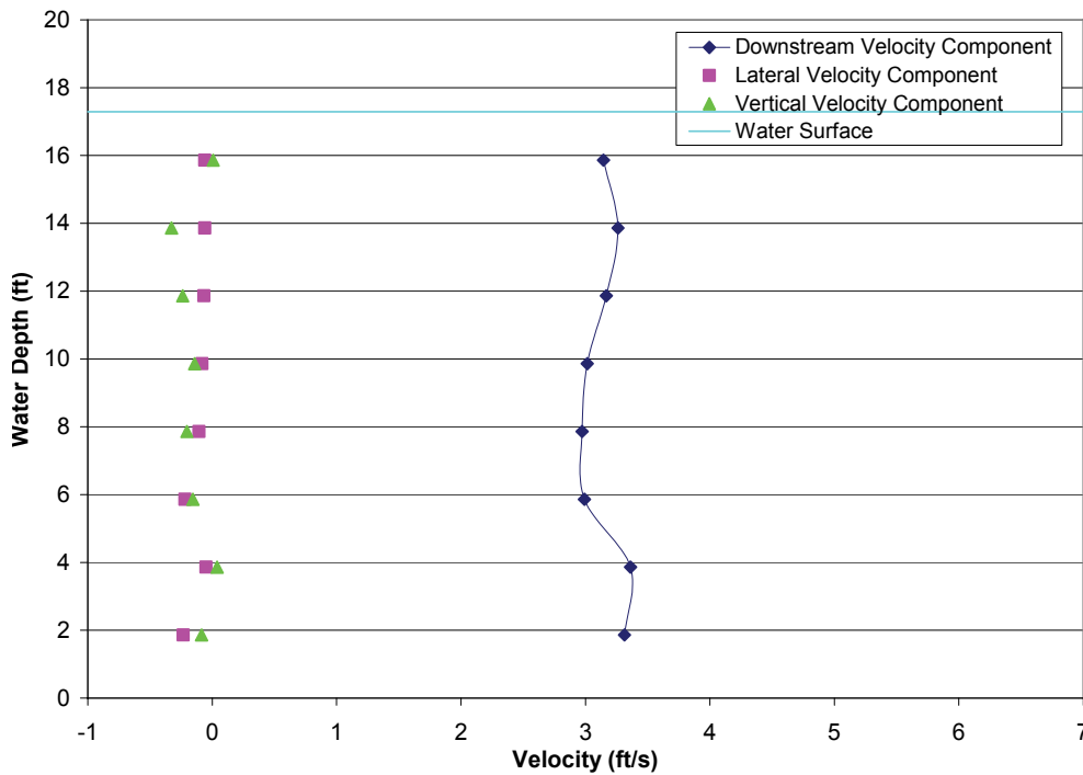
FIGURE A2-25.—Test 1A, bypass 4 intake profile with all bypasses open, measured bypass ratio = 1.05, bypass ratio with facility instruments = 1.02, outgoing tide, water depth = 17.29 ft, trashrack differential = 1.06 ft, louvers differential = 0.45 ft.
