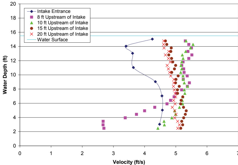
FIGURE A1-7.—Test 1C, bypass 1 approach velocity profiles away from louvers with all bypasses open, measured bypass ratio = 0.83, bypass ratio with facility instruments = 0.68, incoming tide, water depth = 15.50 ft, fouled louver panel 1, clean trashrack.
