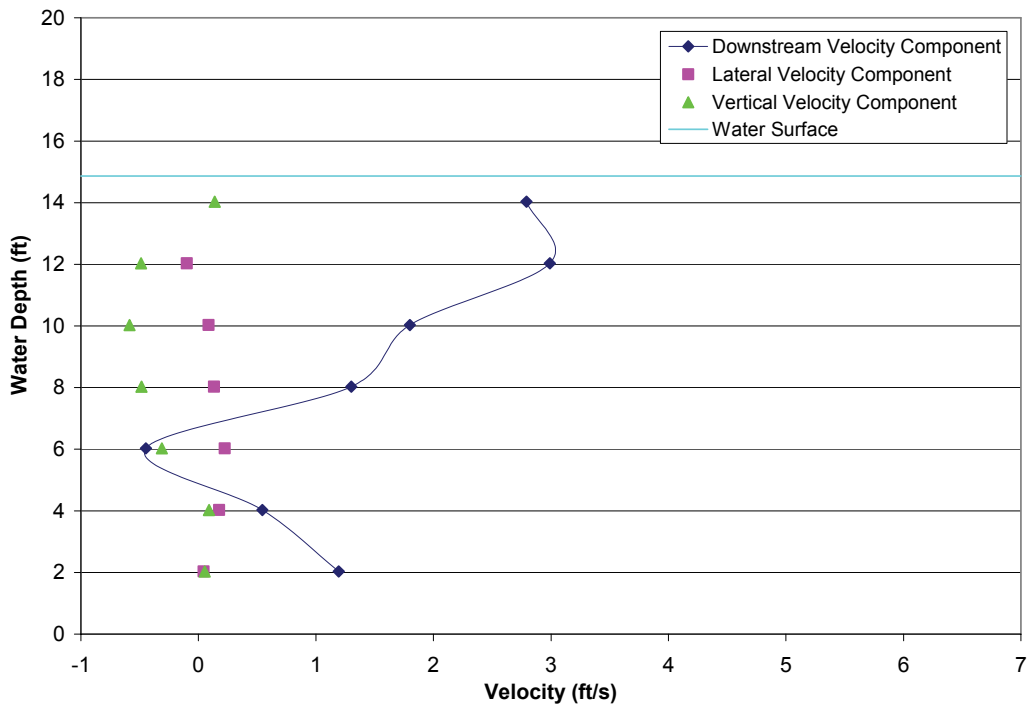
FIGURE A2-5.—Test 2-3, bypass 3 intake profile with all bypasses open, measured bypass ratio = 0.69, bypass ratio with facility instruments = N/A, outgoing tide, water depth = 14.86 ft, trashrack differential = 3.03 ft, louvers differential = 0.74 ft.
