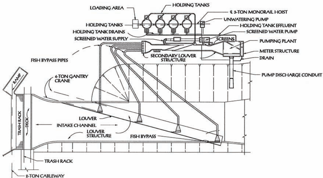
FIGURE 1.—Plan view schematic of Tracy Fish Collection Facility.
