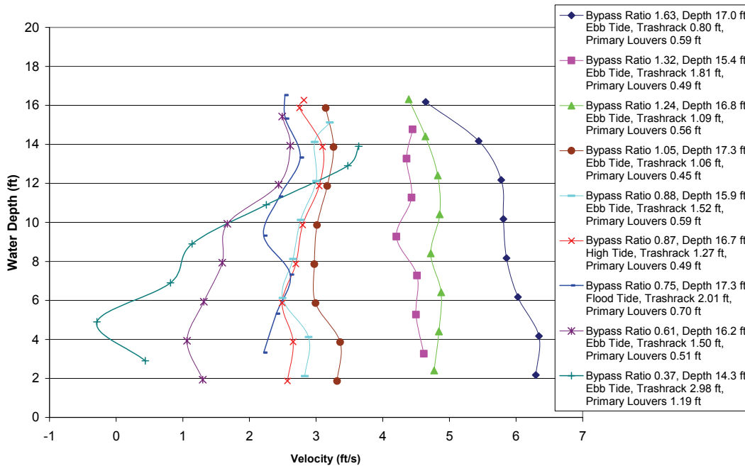
FIGURE 19.—Velocity profiles in the replacement primary bypass 4 intake entrance.
