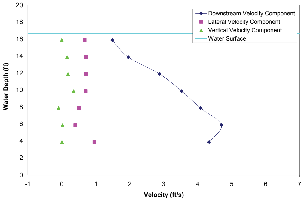
FIGURE A1-3.—Test 1B, bypass 1 intake profiles with all bypasses open, measured bypass ratio = 0.80, bypass ratio with facility instruments = 0.69, incoming tide, water depth = 16.64 ft, recently cleaned trashrack and louvers.
