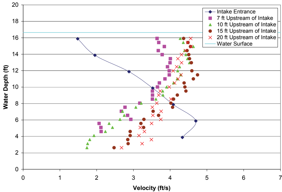
FIGURE A1-5.—Test 1B, bypass 1 approach velocity profiles against the louvers with all bypasses open, measured bypass ratio = 0.80, bypass ratio with facility instruments = 0.69, incoming tide, water depth = 16.64 ft, recently cleaned trashrack and louvers.
