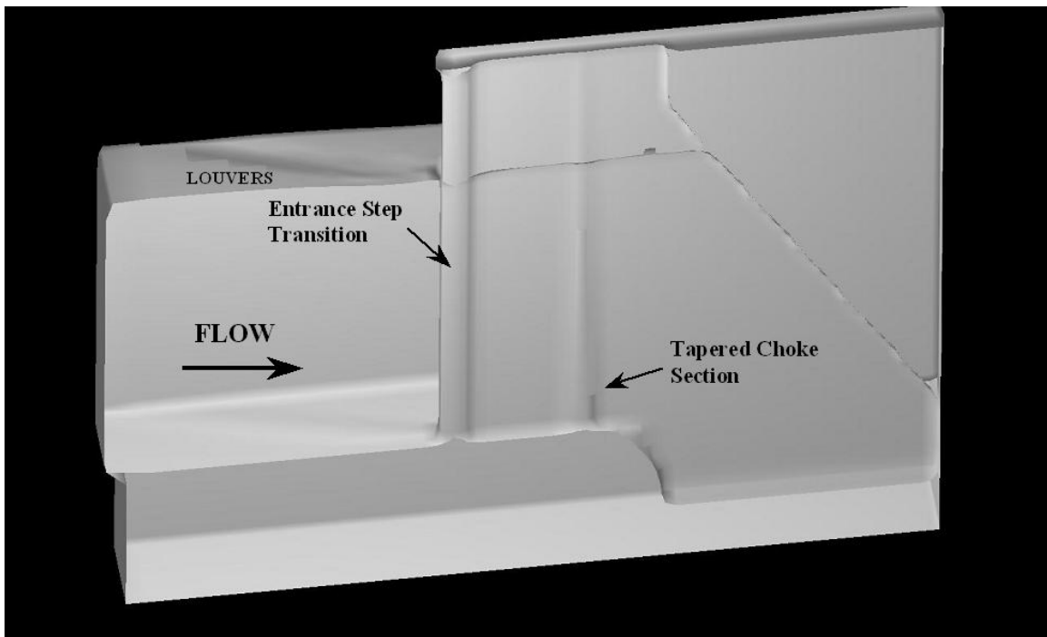
FIGURE 4.—Replacement bypass intake design using a tapered choke section (Kubitschek, 2003).
