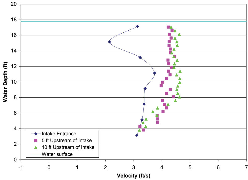
FIGURE A2-20.—Test 4-2, bypass 2 approach velocity profiles with all bypasses open, measured bypass ratio = 0.84, bypass ratio with facility instruments = 0.72, incoming tide, water depth = 17.77 ft, trashrack differential = 1.35 ft, louvers differential = 0.62 ft.
