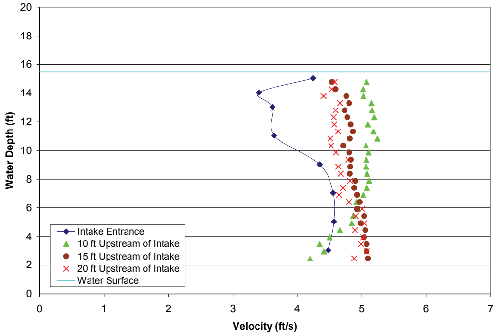
FIGURE A1-7.—Test 1C, bypass 1 approach velocity profiles away from louvers with all bypasses open, measured bypass ratio = 0.83, bypass ratio with facility instruments = 0.68, incoming tide, water depth = 15.50 ft, fouled louver panel 1, clean trashrack.
