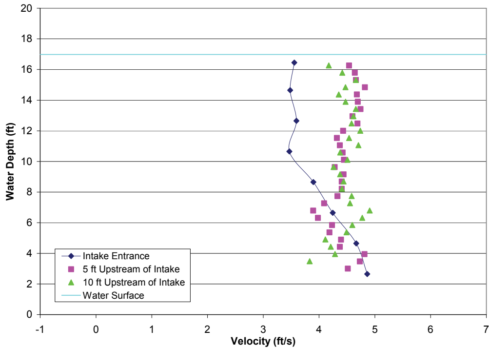
FIGURE A2-10.—Test 3-1, bypass 1 approach velocity profiles with all bypasses open, measured bypass ratio = 0.98, bypass ratio with facility instruments = 1.27, outgoing tide, water depth = 16.98 ft, trashrack differential = 0.94 ft, louvers differential = 0.45 ft.
