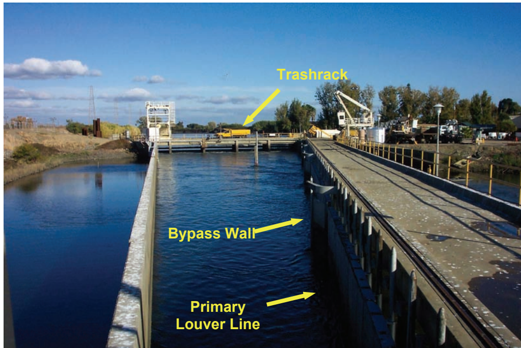
FIGURE 2.—Features in the primary channel looking upstream.
