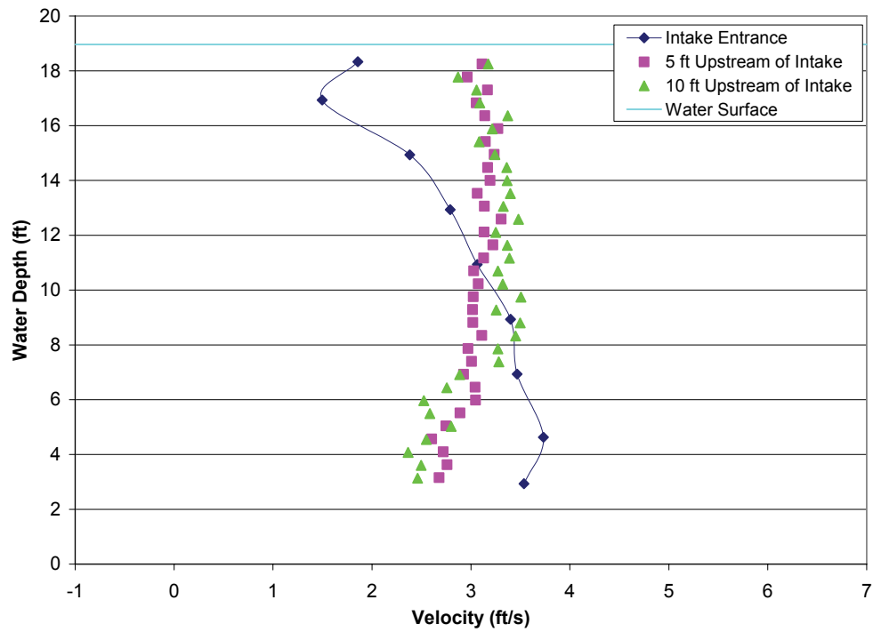
FIGURE A2-22.—Test 4-3, bypass 3 approach velocity profiles with all bypasses open, measured bypass ratio = 0.98, bypass ratio with facility instruments = 0.74, incoming tide, water depth = 18.96 ft, trashrack differential = 1.07 ft, louvers differential = 0.37 ft.
