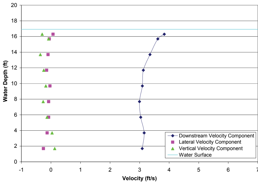
FIGURE A2-13.—Test 3-3, bypass 3 intake profile with all bypasses open, measured bypass ratio = 1.01, bypass ratio with facility instruments = 0.39, outgoing tide, water depth = 16.92 ft, trashrack differential = 1.27 ft, louvers differential = 0.44 ft.
