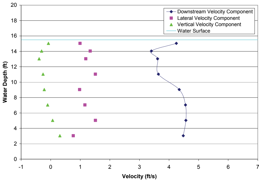
FIGURE A1-6.—Test 1C, bypass 1 intake profile with all bypasses open, measured bypass ratio = 0.83, bypass ratio with facility instruments = 0.68, incoming tide, water depth = 15.50 ft, fouled louver panel 1, clean trashrack.
