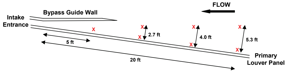
FIGURE 10.—Schematic of velocity profile locations (indicated by X ) upstream from the intake entrance. Profiles were measured against the louver panel face and several feet away from the louvers.
