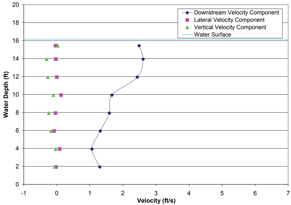
FIGURE A2-27.—Test 1B, bypass 4 intake profile with bypass 1 closed, measured bypass ratio = 0.61, bypass ratio with facility instruments = 0.64, outgoing tide, water depth = 16.16 ft, trashrack differential = 1.50 ft, louvers differential = 0.51 ft.
