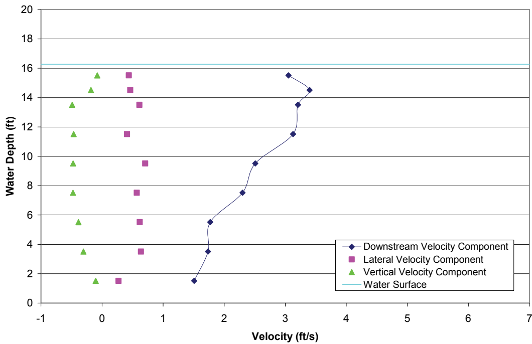
FIGURE A1-9.—Test 4A, bypass 4 intake profile with all bypasses open, measured bypass ratio = 0.69, bypass ratio for facility instruments = 0.46, incoming tide, water depth = 16.28 ft, recently cleaned trashrack and louvers.
