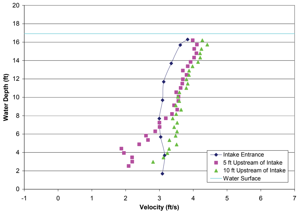
FIGURE A2-14.—Test 3-3, bypass 3 approach velocity profiles with all bypasses open, measured bypass ratio = 1.01, bypass ratio with facility instruments = 0.39, outgoing tide, water depth = 16.92 ft, trashrack differential = 1.27 ft, louvers differential = 0.44 ft.
