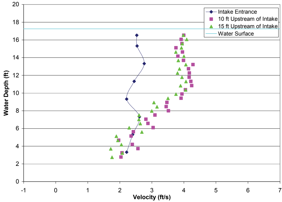
FIGURE A2-16.—Test 3-4, bypass 4 approach velocity profiles with all bypasses open, measured bypass ratio = 0.75, bypass ratio with facility instruments = 0.71, incoming tide, water depth = 17.25 ft, trashrack differential = 2.01 ft, louvers differential = 0.70 ft.
