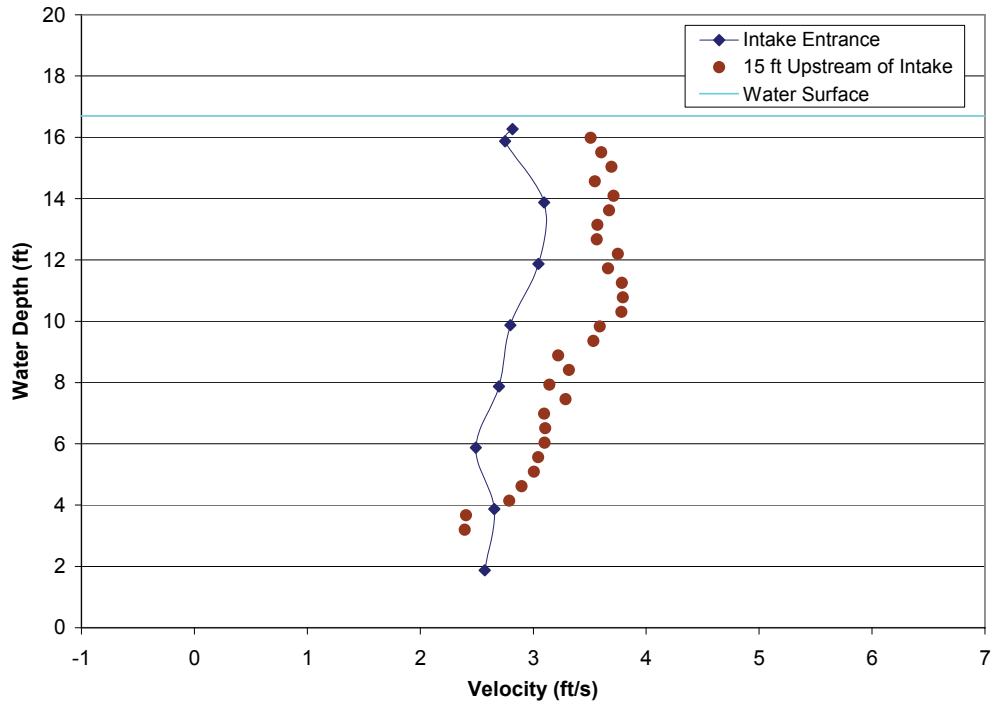
FIGURE A2-24.—Test 4-4, bypass 4 approach velocity profiles with all bypasses open, measured bypass ratio = 0.87, bypass ratio with facility instruments = 0.90, high tide, water depth = 16.70 ft, trashrack differential = 1.27 ft, louvers differential = 0.49 ft.
