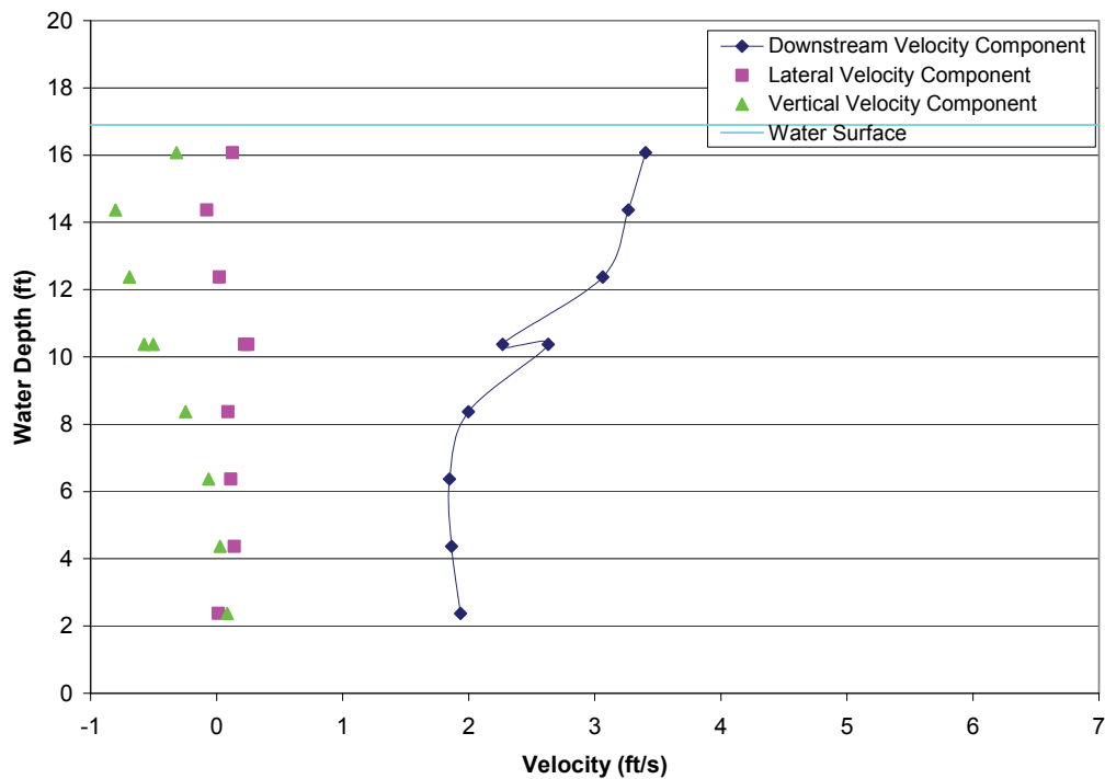
FIGURE A2-3.—Test 2-2, bypass 2 intake profile with all bypasses open, measured bypass ratio = 0.95, bypass ratio with facility instruments = 0.68, outgoing tide, water depth = 16.90 ft, trashrack differential = 1.45 ft, louvers differential = 0.73 ft.
