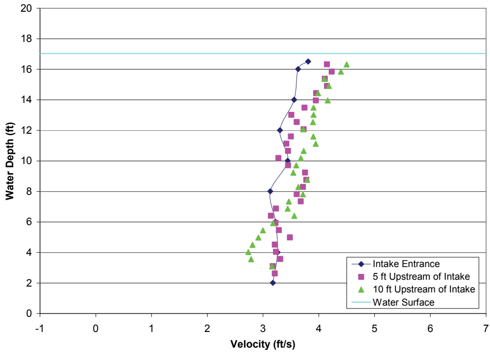
FIGURE A2-12.—Test 3-2, bypass 2 approach velocity profiles with all bypasses open, measured bypass ratio = 1.02, bypass ratio with facility instruments = 0.79, outgoing tide, water depth = 17.04 ft, trashrack differential = 1.11 ft, louvers differential = 0.55 ft.
