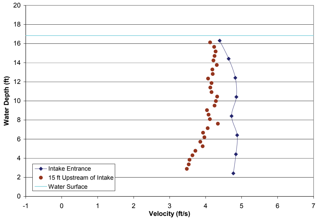
FIGURE A2-34.—Test 5A, bypass 4 approach velocity profiles with bypass 1 and 2 closed, measured bypass ratio = 1.24, bypass ratio with facility instruments = 1.41, outgoing tide, water depth = 16.84 ft, trashrack differential = 1.09 ft, louvers differential = 0.56 ft.
