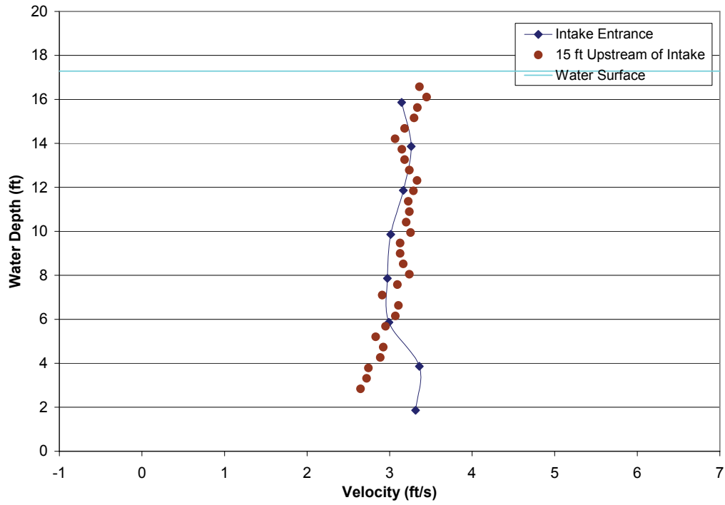
FIGURE A2-26.—Test 1A, bypass 4 approach velocity profiles with all bypasses open, measured bypass ratio = 1.05, bypass ratio with facility instruments = 1.02, outgoing tide, water depth = 17.29 ft, trashrack differential = 1.06 ft, louvers differential = 0.45 ft.
