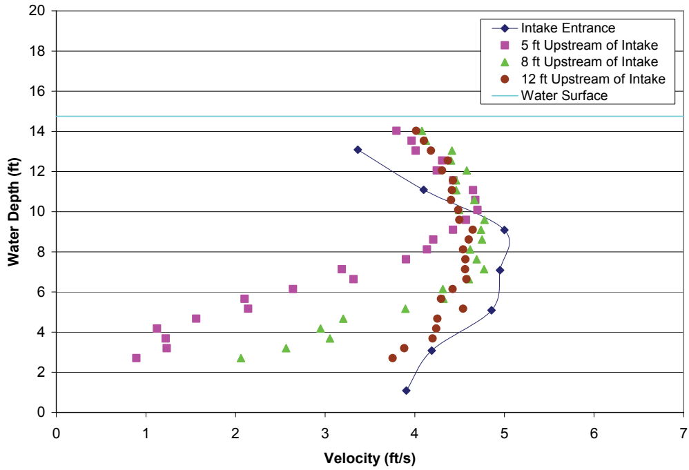
FIGURE A1-2.—Test 1A, bypass 1 approach velocity profiles against the louvers with all bypasses open, measured bypass ratio = N/A, bypass ratio with facility instruments = N/A, incoming tide, water depth = 14.75 ft, recently cleaned trashrack and louvers.
