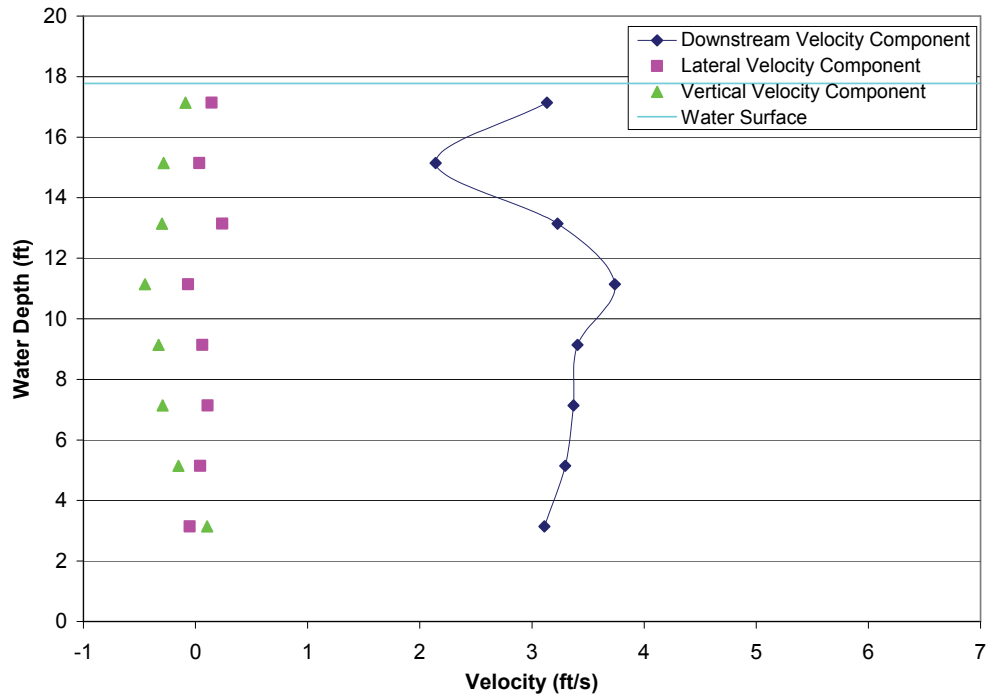
FIGURE A2-19.—Test 4-2, bypass 2 intake profile with all bypasses open, measured bypass ratio = 0.84, bypass ratio with facility instruments = 0.72, incoming tide, water depth = 17.77 ft, trashrack differential = 1.35 ft, louvers differential = 0.62 ft.
