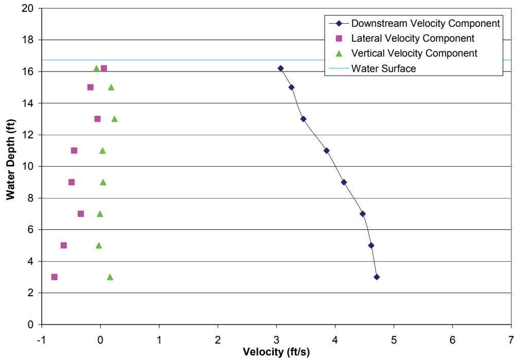
FIGURE A2-17.—Test 4-1, bypass 1 intake profile with all bypasses open, measured bypass ratio = 0.86, bypass ratio with facility instruments = 1.17, incoming tide, water depth = 16.73 ft, trashrack differential = 1.29 ft, louvers differential = 0.43 ft.
