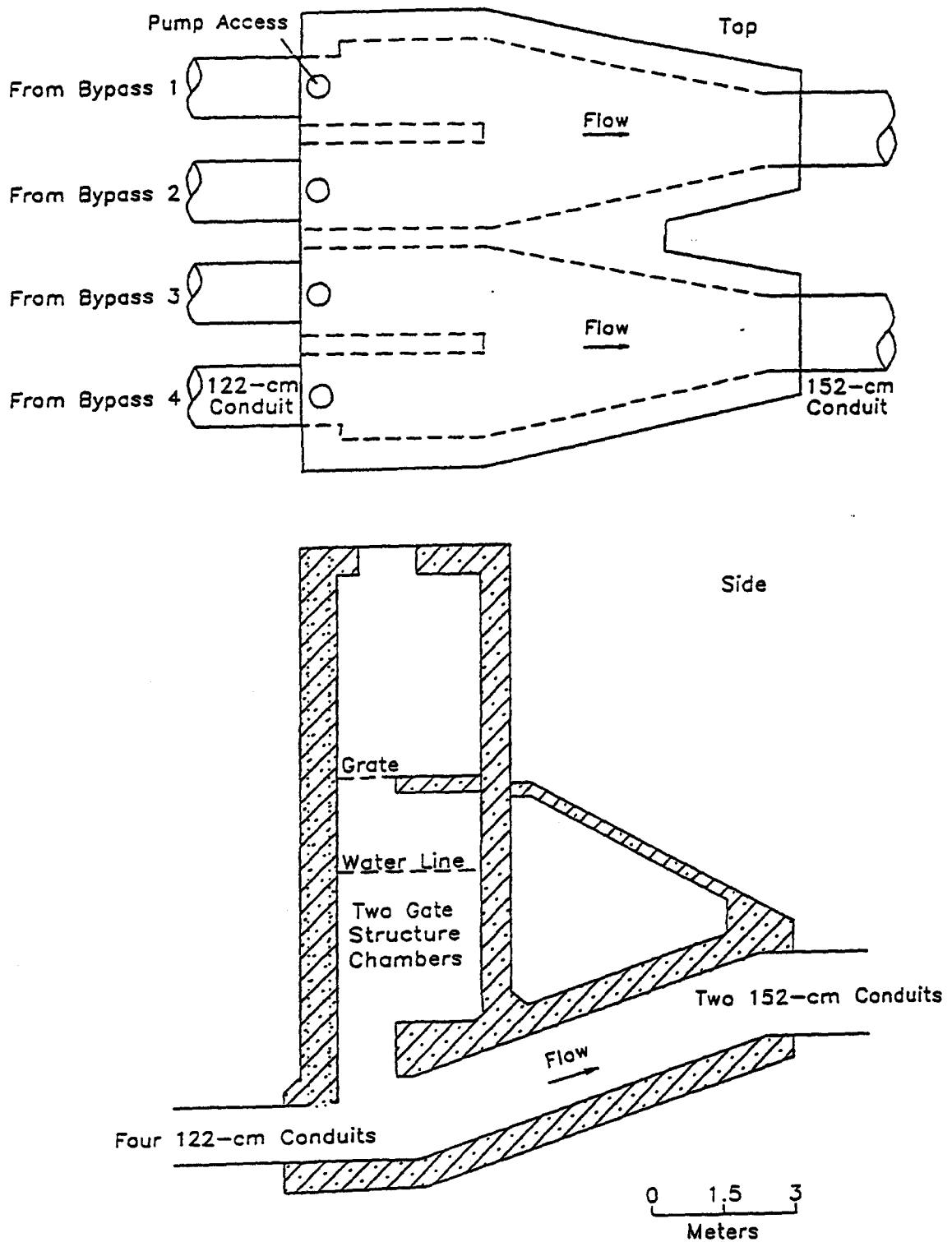
Figure 4.-Top and side view of gate structure including gate structure chambers.
