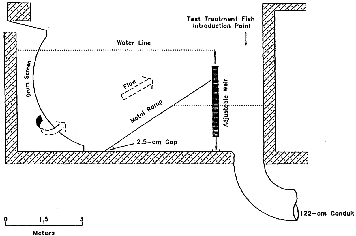
Figure 3.-Side view of one of four bypass entrances including test fish introduction site, metal ramp, adjustable weir, and 122-cm conduit opening. Gap between the floor and upstream end of the metal ramp (2.5 cm) is unique to bypass two.
