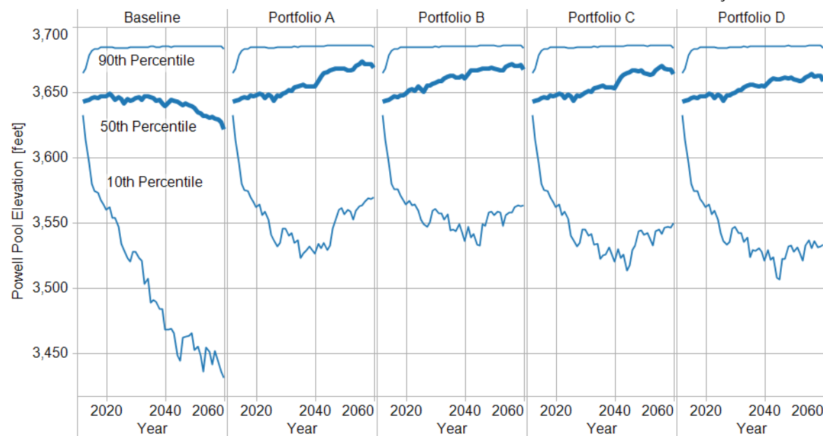
FIGURE G-22 10th, 50th, 90th Percentiles for Lake Powell End-of-December Pool Elevation for the Baseline and Four Dynamic Portfolios
