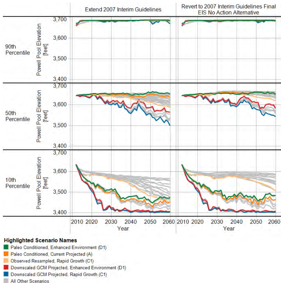
FIGURE G-4 10th, 50th, 90th Percentiles for Lake Powell End-of-December Pool Elevation
