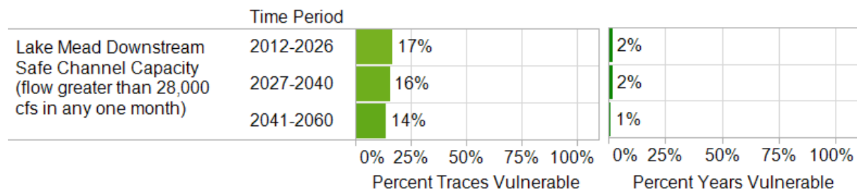
FIGURE G-12 Summary of Vulnerability Without Options and Strategies for Flood Control Indicator Metrics
