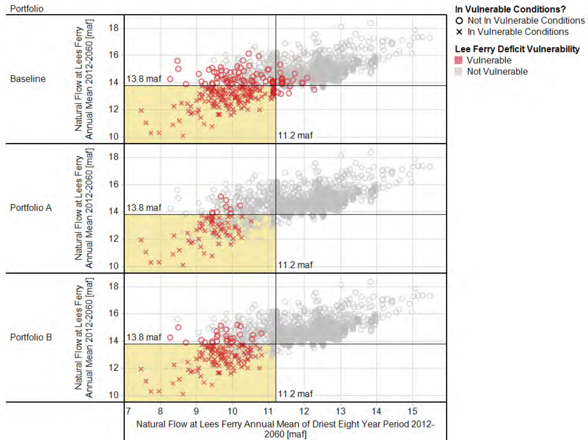
FIGURE G-32 Reduction in Vulnerable Traces with Selected Portfolios in Place, Lee Ferry Deficit Indicator Metric
