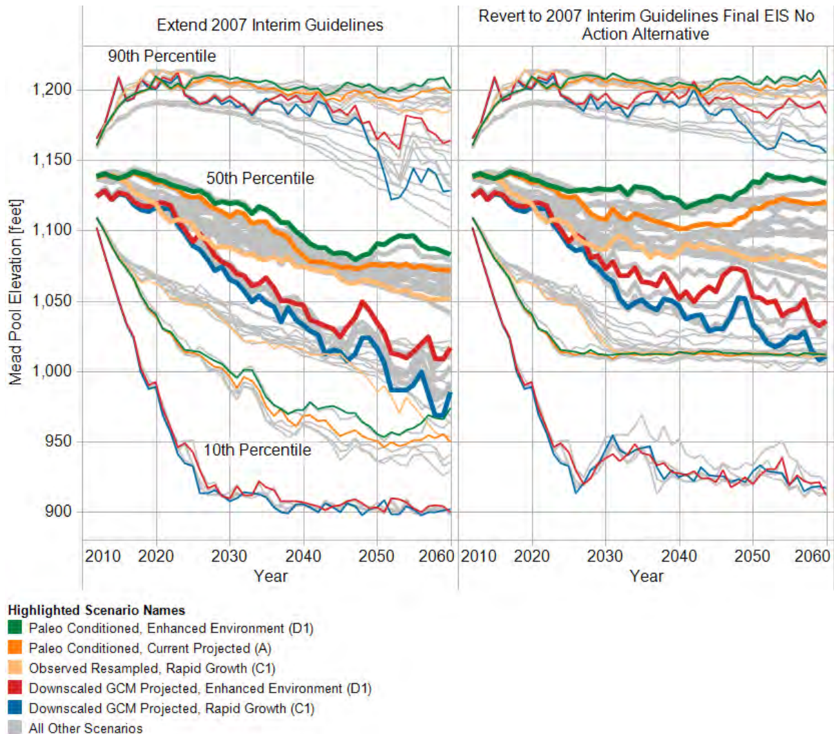
FIGURE G-6 10th, 50th, 90th Percentiles for Lake Mead End-of-December Pool Elevation
