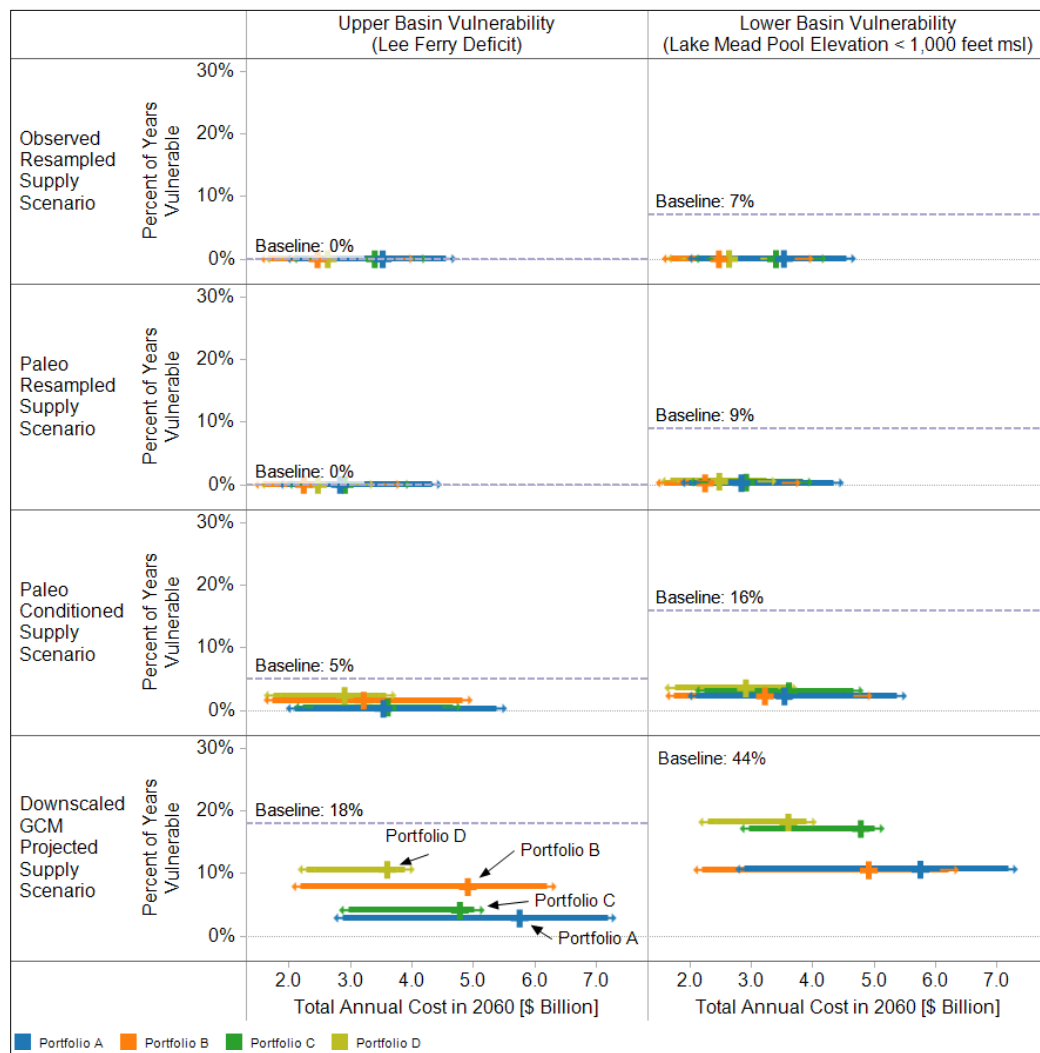
FIGURE G-51 Percent of Years Vulnerable for Upper Basin and Lower Basin Vulnerabilities from 2041–2060 and Range In Total Annual Cost In 2060 Across Supply Scenarios for Four Portfolios
