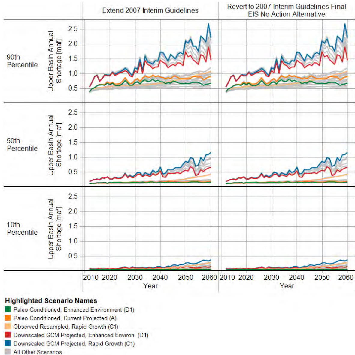
FIGURE G-3 10th, 50th, 90th Percentiles for Magnitude of Upper Basin Annual Shortage
