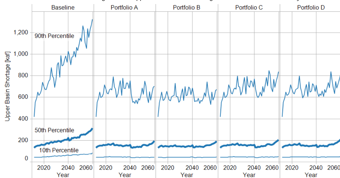
FIGURE G-21 10th, 50th, 90th Percentiles for Magnitude of Upper Basin Annual Shortage for the Baseline and Four Dynamic Portfolios
