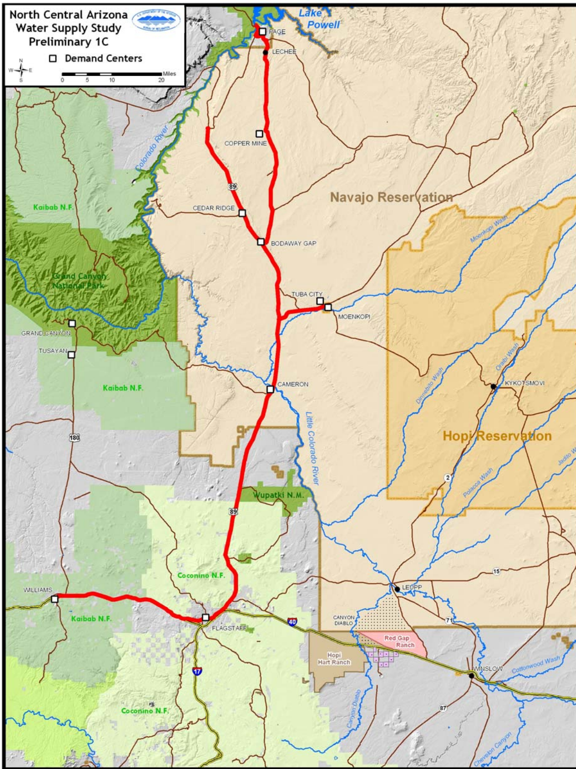
Figure IV.1-3. Lake Powell pipeline to Williams via Flagstaff.
