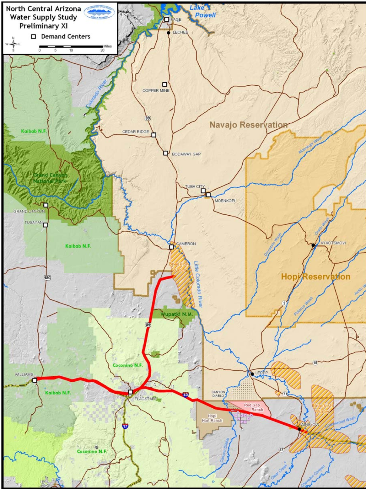
Figure IV.1-9. Low water quality C-Aquifer source to Williams and Flagstaff.
