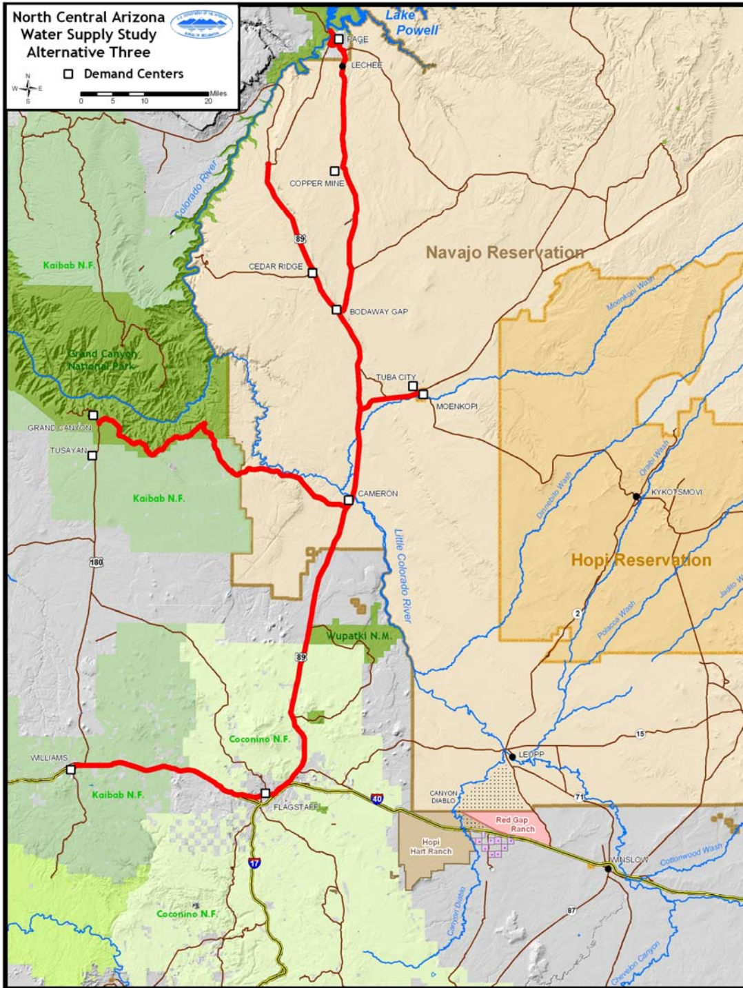
Figure IV.2-3. Alternative 3: Hopi/Navajo/Flagstaff/Williams/Grand Canyon/Tusayan Demand Centers –supplied via Lake Powell pipeline.
