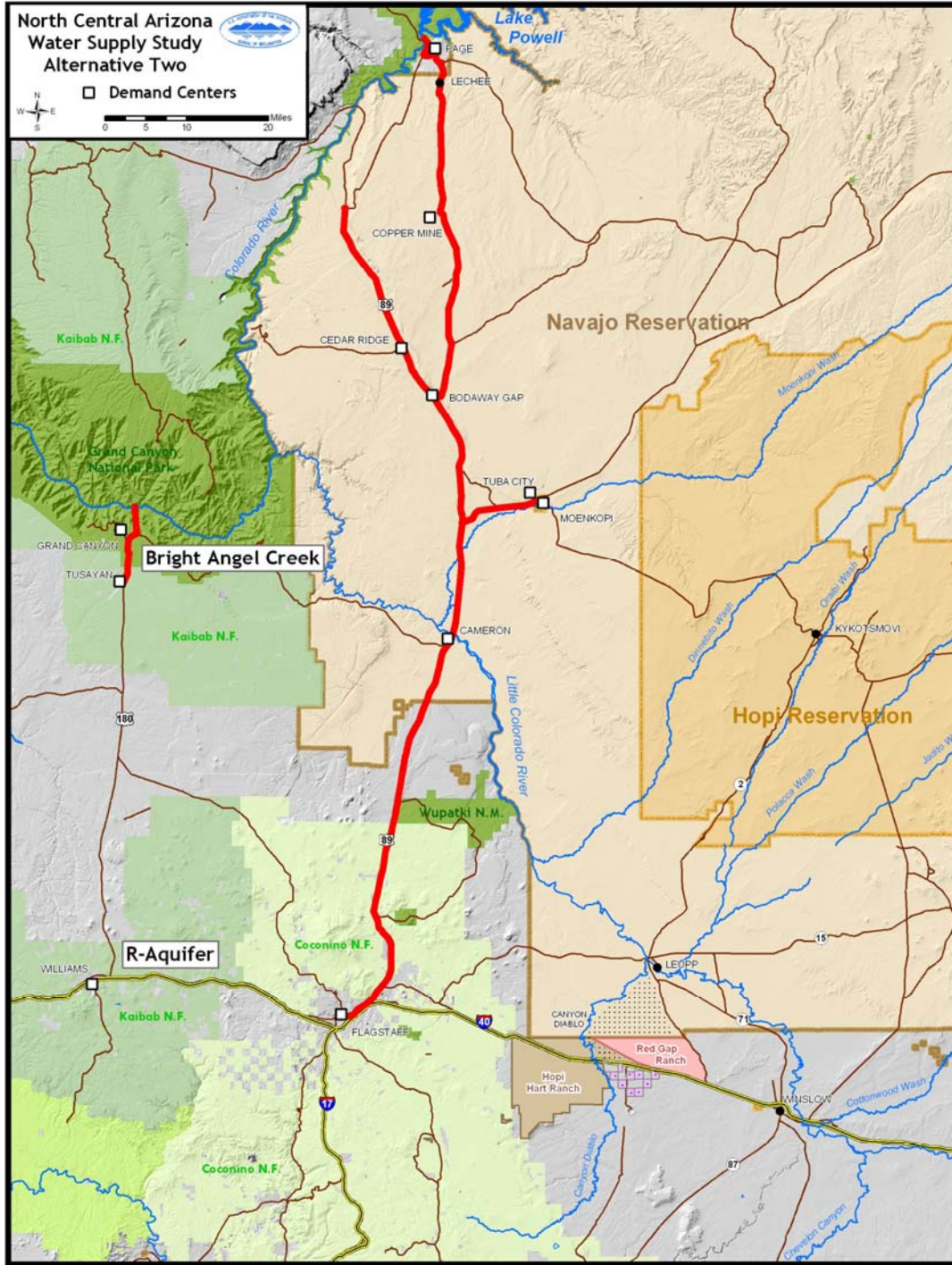
Figure IV.2-2. Alternative 2: Hopi/Navajo/Flagstaff Demand Centers – supplied via Lake Powell pipeline; Williams Demand Center – supplied from local R-M Aquifer wells; Grand Canyon/Tusayan Demand Center – supplied from Roaring Springs via pipeline diverting from Phantom Ranch infiltration gallery.
