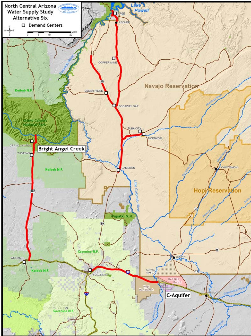
Figure IV.2-6. Alternative 6: Hopi/Navajo Demand Centers – supplied via Lake Powell pipeline; Flagstaff Demand Center – supplied via pipeline from C-Aquifer pipeline; Williams/Grand Canyon/Tusayan Demand Centers – supplied from Roaring Springs via pipeline diverting from Phantom Ranch infiltration gallery.
