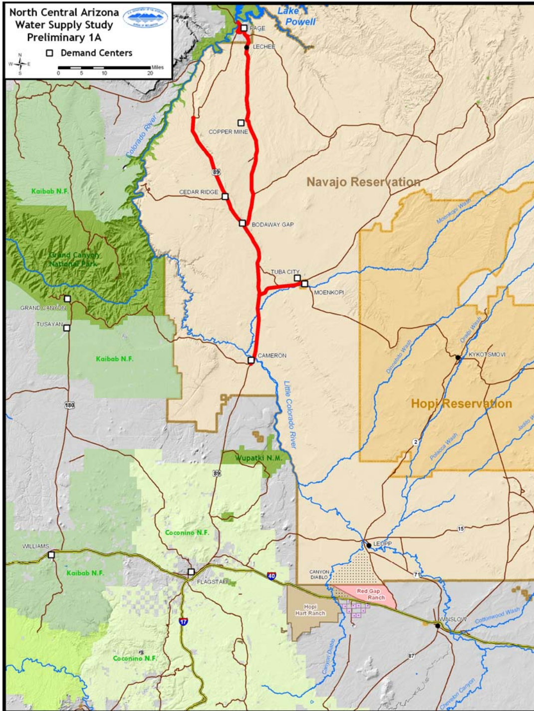
Figure IV.1-1. Lake Powell pipeline to Cameron.
