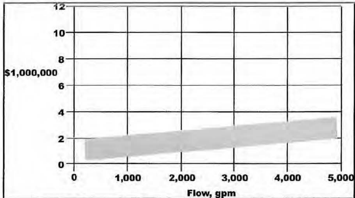
Figure 6.2 Coagulation/Filtration Arsenic Removal Capital Costs
