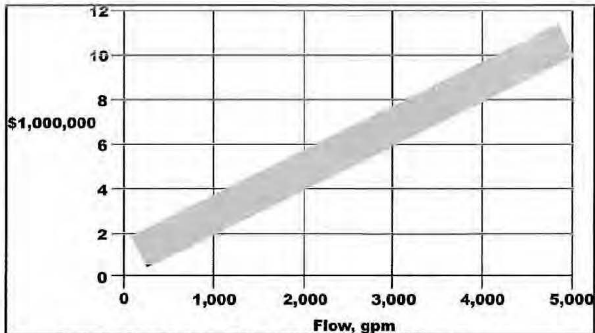
Figure 6.1 Ion Exchange Nitrate Removal Capital Costs
