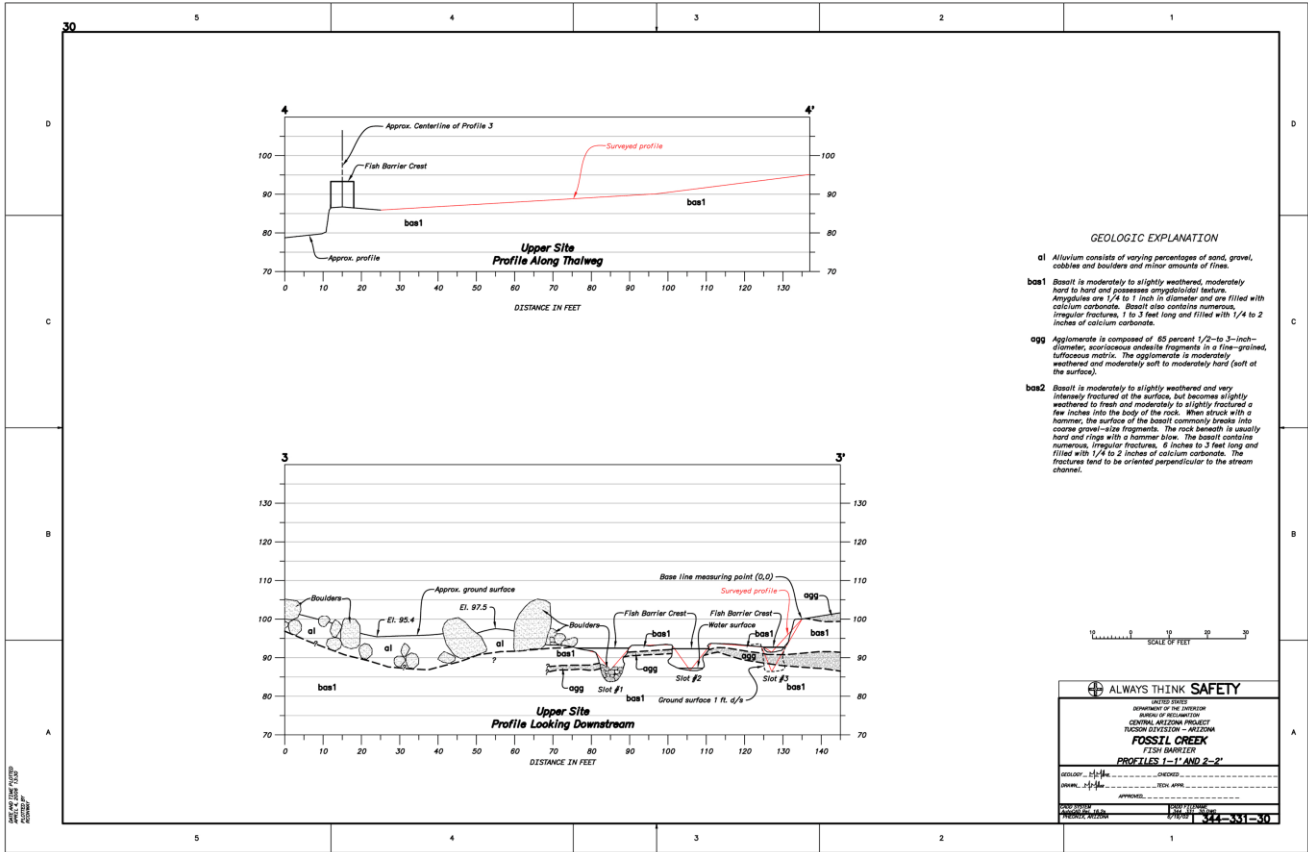
Figure 3. Upper site profile (along thalweg and looking downstream) of Fossil Creek fish barrier.
