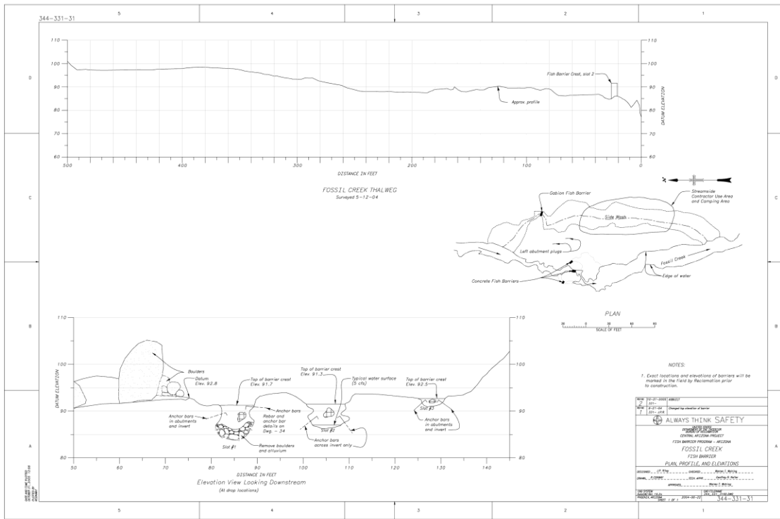
Figure 4. Elevation view of Fossil Creek fish barrier (looking downstream at drop location).
