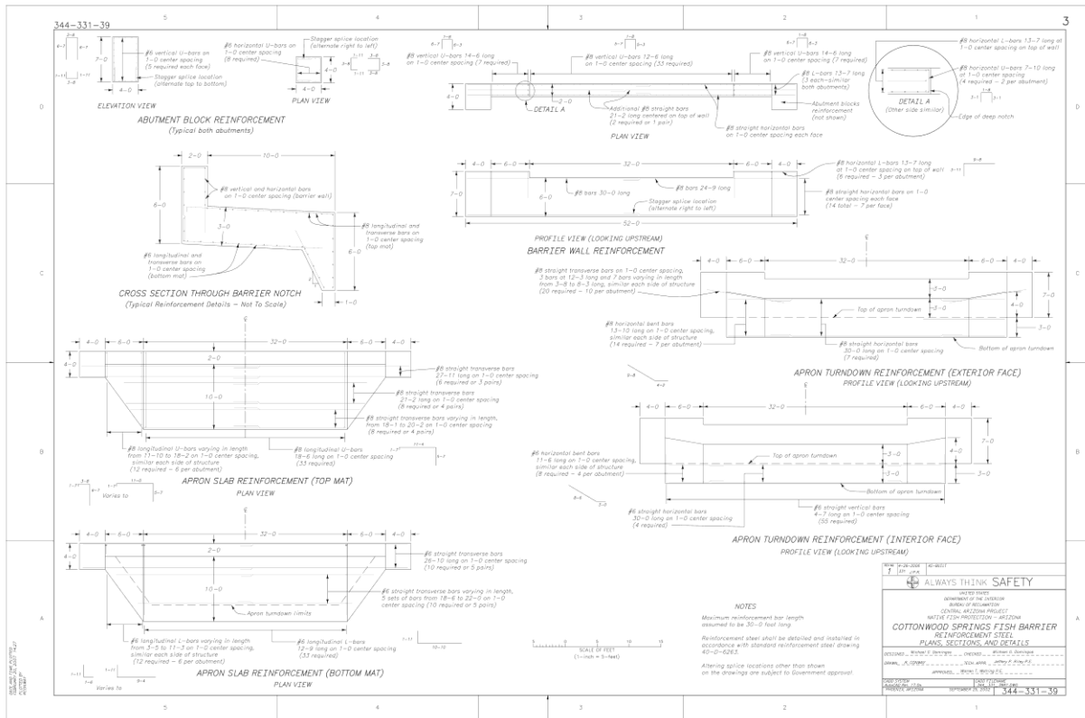
Figure 4. Reinforcement steel plans, sections, and details of Cottonwood Springs fish barrier.
