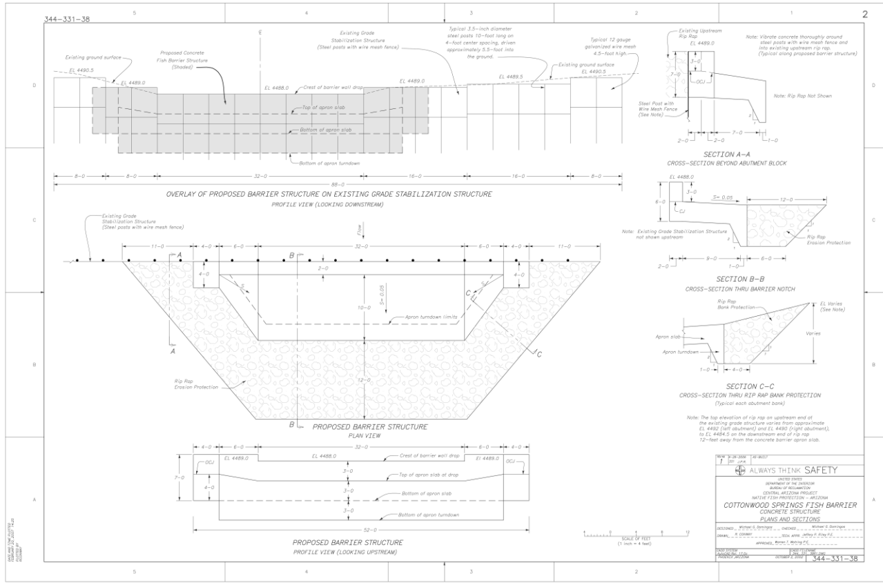
Figure 3. Concrete structure plans and sections of Cottonwood Springs fish barrier.
