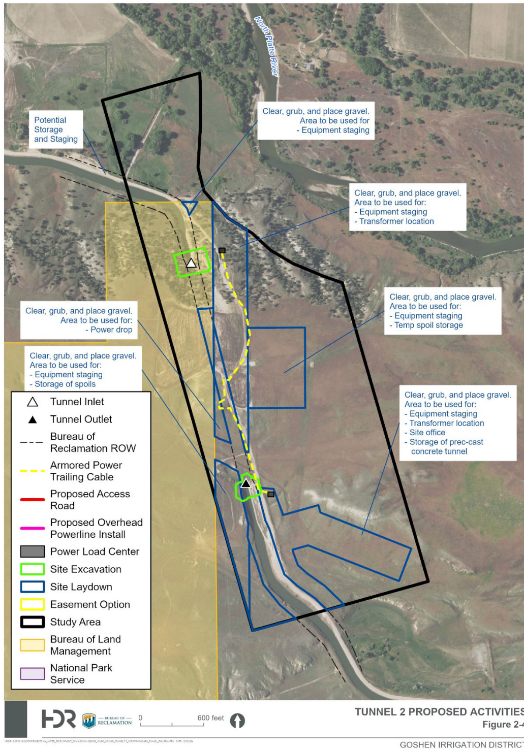
Figure 2-4. Proposed Activities, Tunnel No. 2
