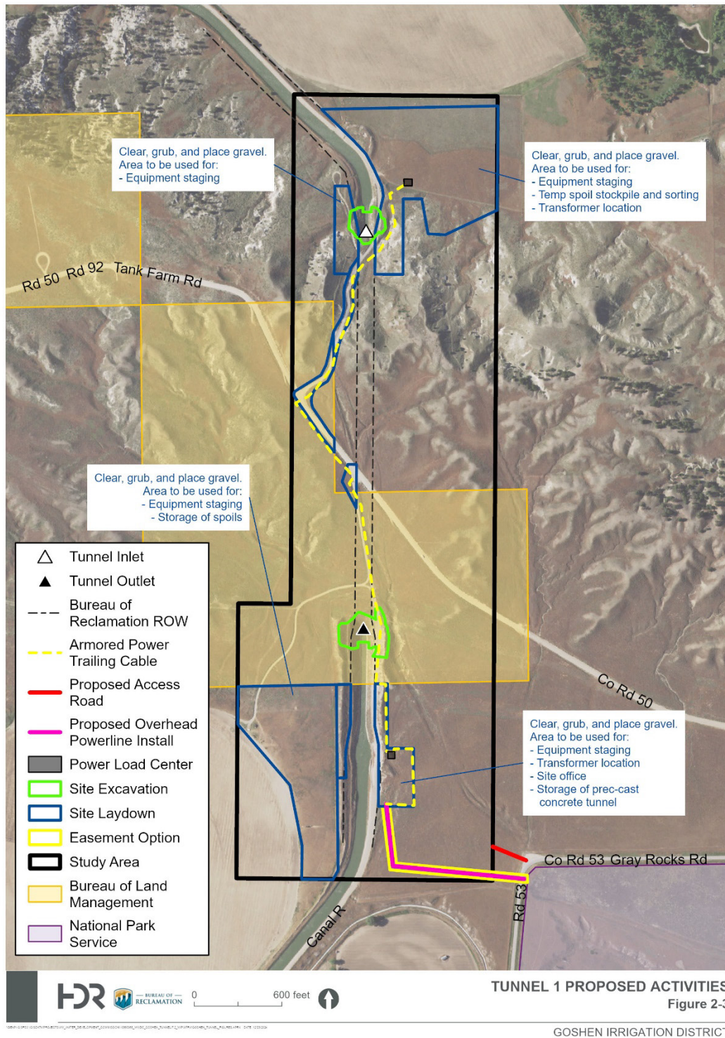
Figure 2-3. Proposed Activities, Tunnel No. 1
