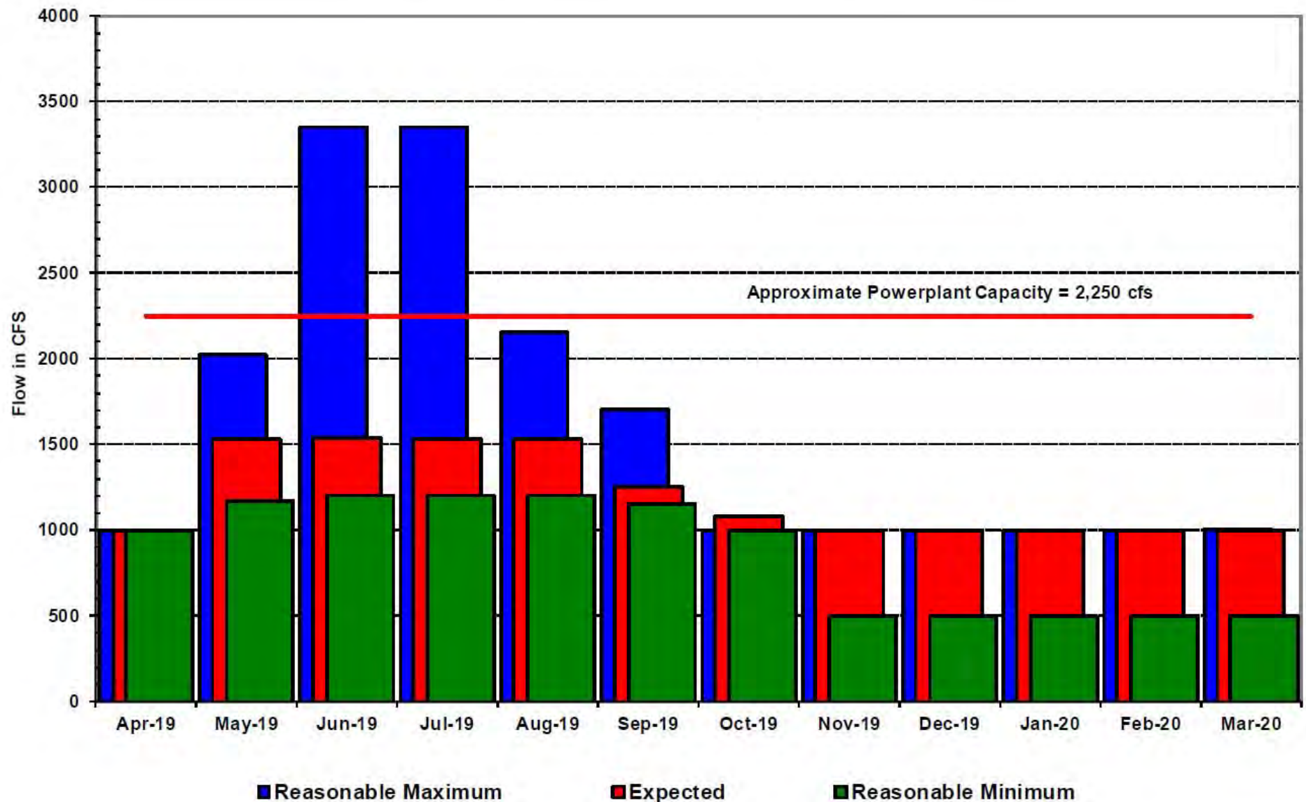
WIND RIVER FLOW BELOW BOYSEN DAM
