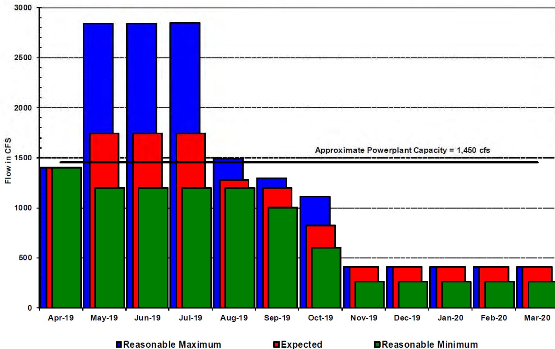
SHOSHONE RIVER FLOW BELOW BUFFALO BILL DAM
