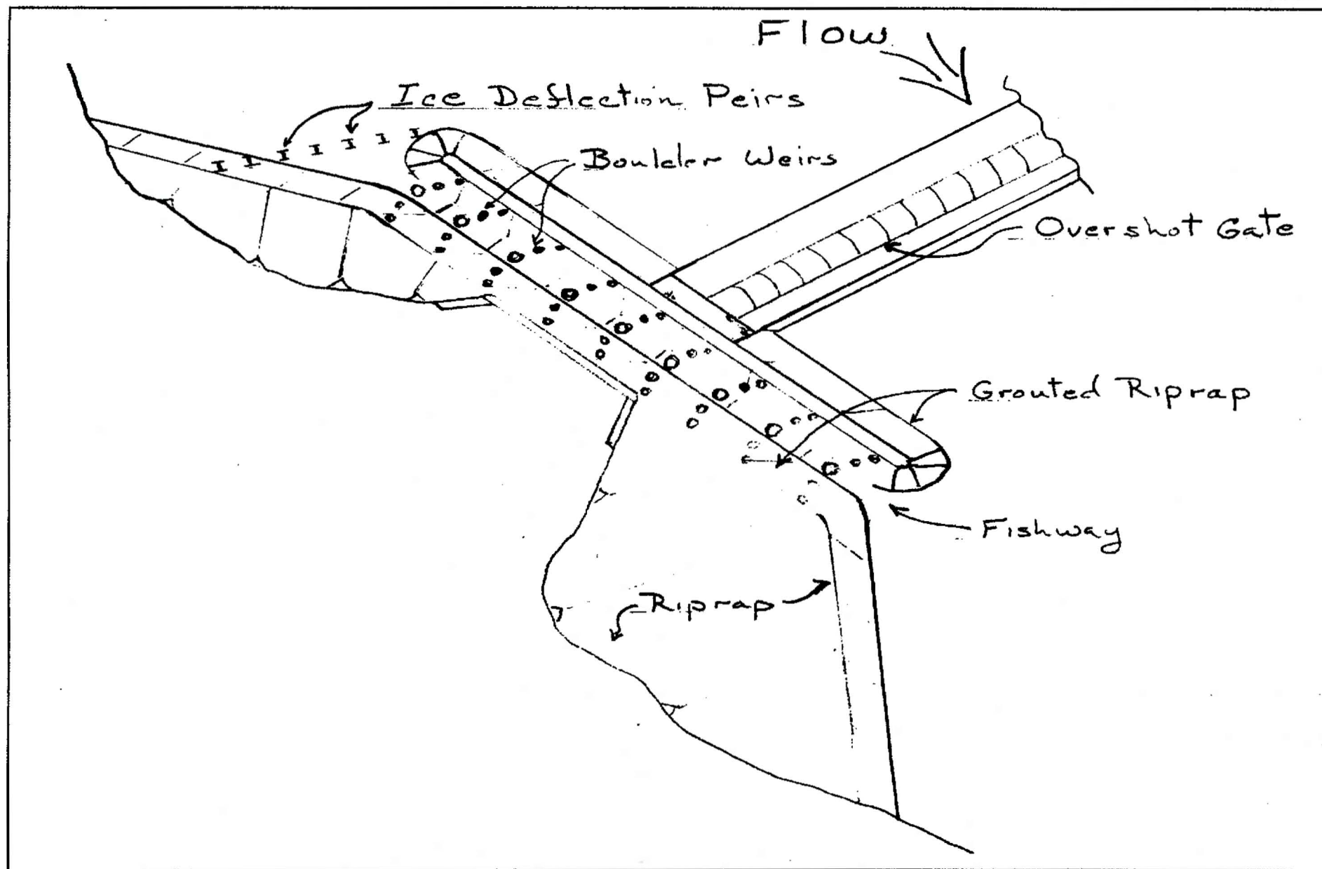
Figure 9 - Plan View of Fishway
